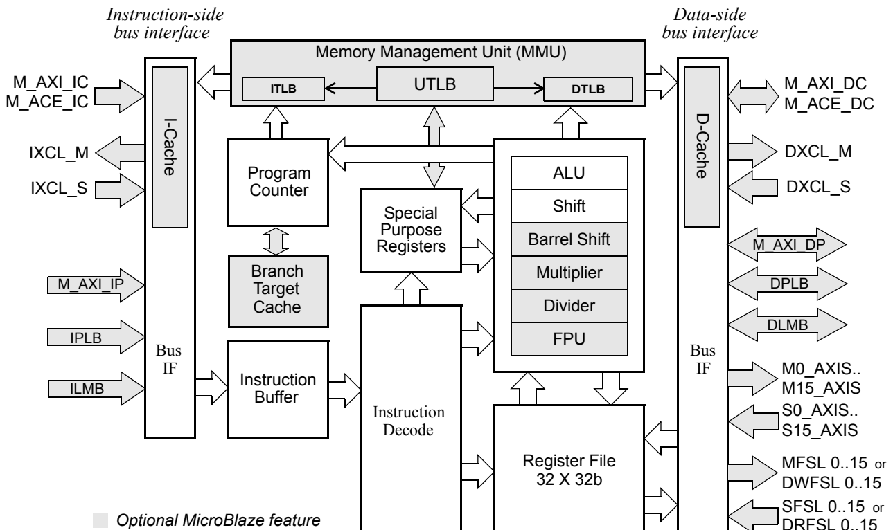
Figure 3-1: MicroBlaze Core Block Diagram
