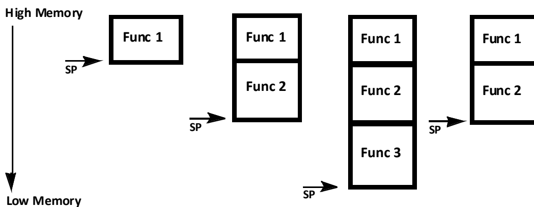
Figure 4-1: Stack Frame
