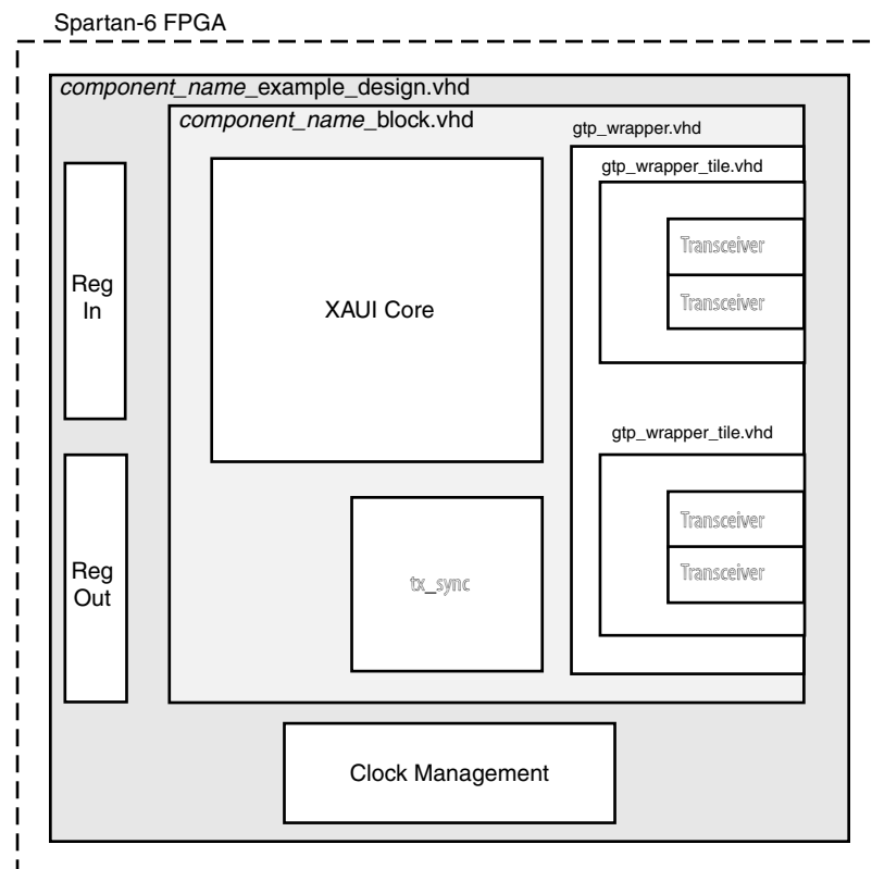
Figure 12-5: Example HDL Wrapper for XAUI (Spartan-6 FPGAs)
