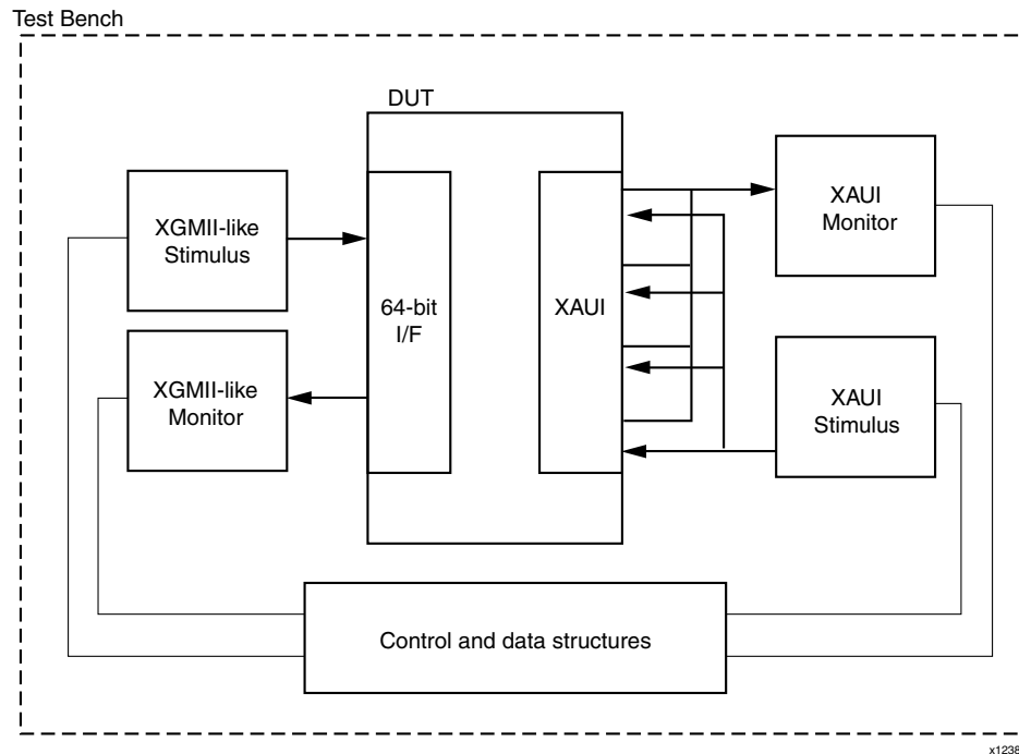
Figure 12-6: Demonstration Test Bench for XAUI without XGMII Interface
