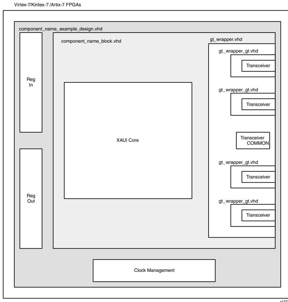
Figure 12-4: Example HDL Wrapper for XAUI (Virtex-7, Kintex-7, and Artix-7 FPGAs)
