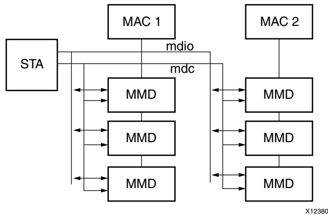
Figure 5-5: A Typical MDIO-Managed System
