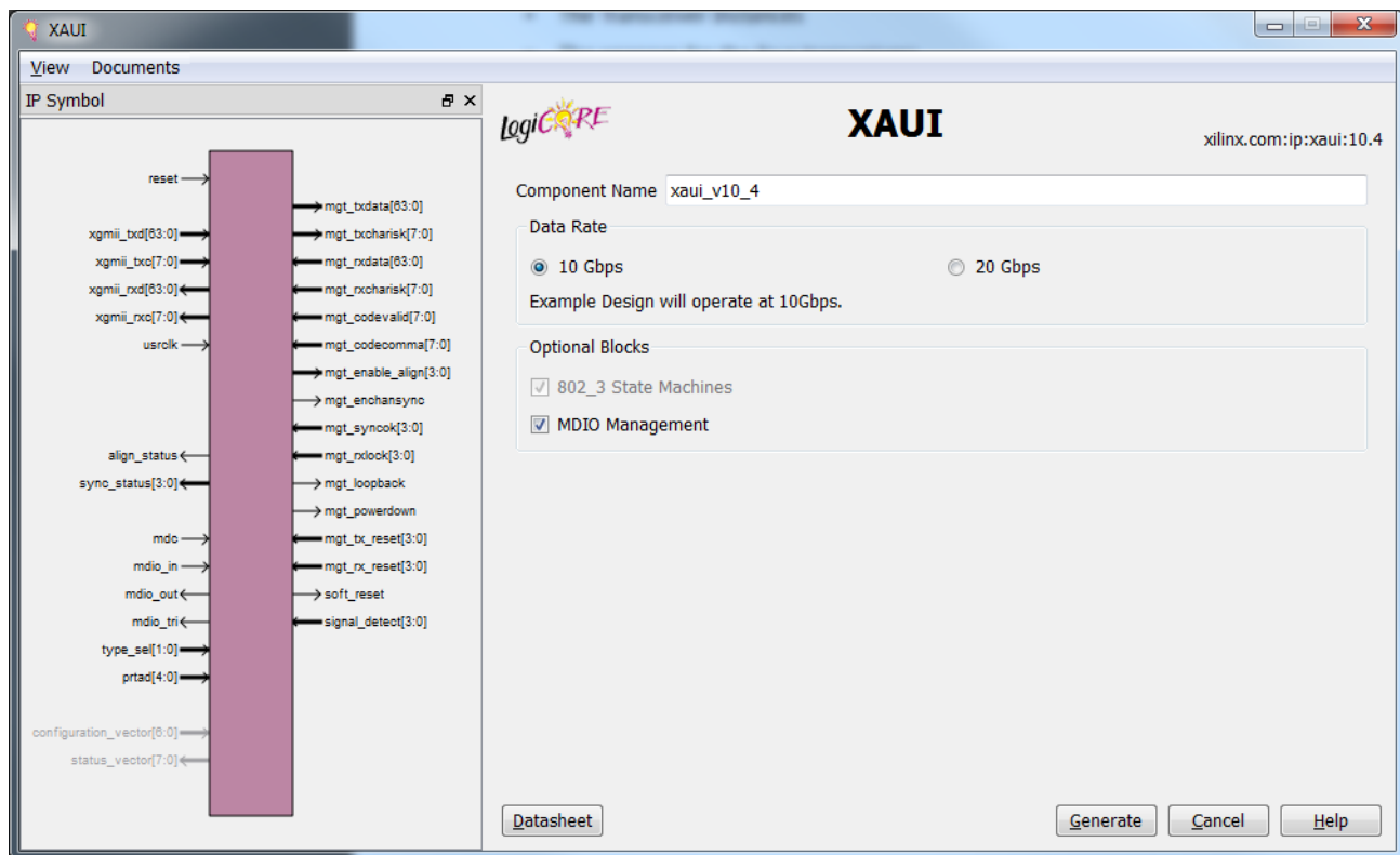
Figure 10-1: XAUI Main Screen
