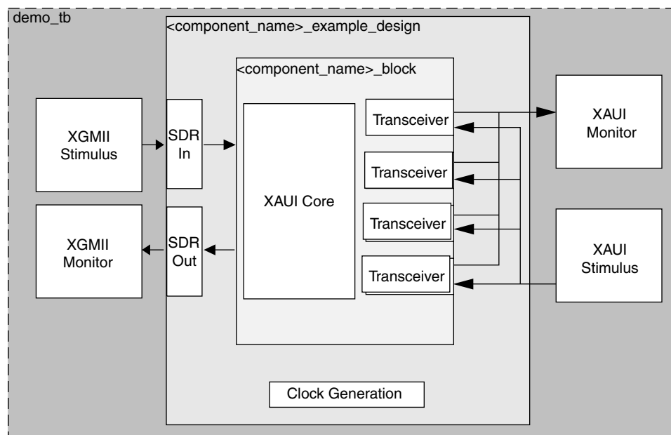
Figure 14-1: XAUI Example Design and Test Bench: Default Configuration
