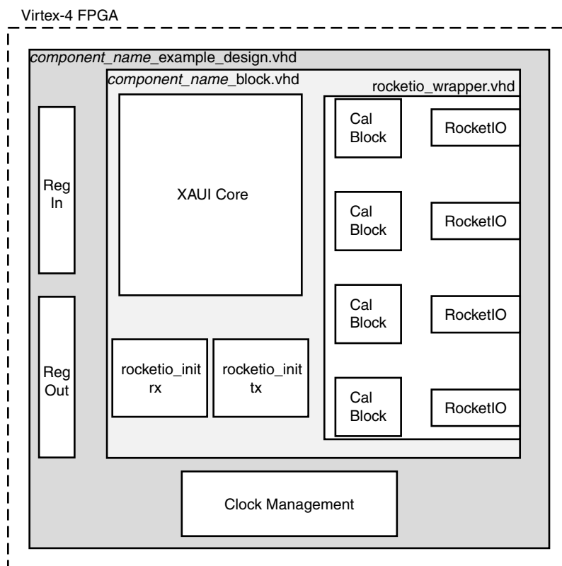
Figure 12-1: Example HDL Wrapper for XAUI without XGMII (Virtex-4 FPGAs)
