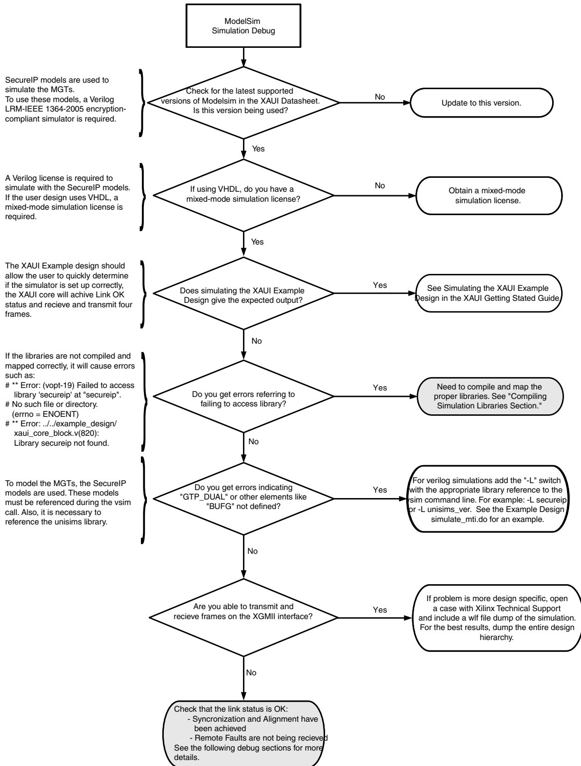
Figure C-1: ModelSim Debug Flow Diagram
