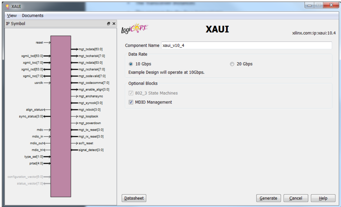
Figure 14-2: XAUI Main Screen
