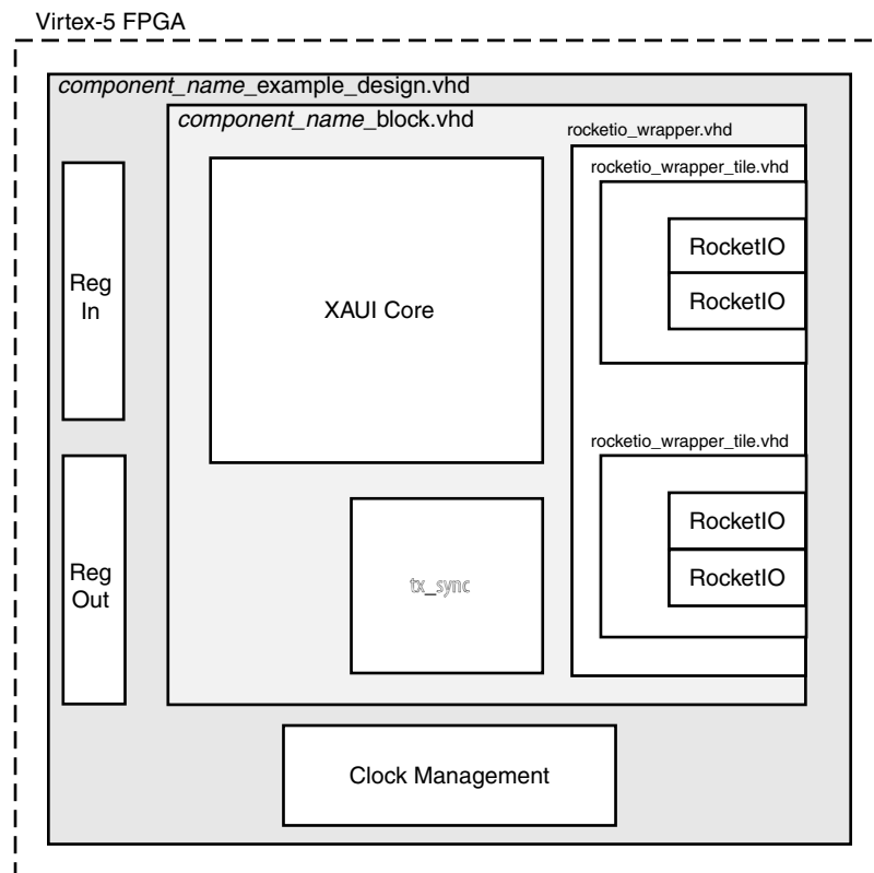
Figure 12-2: Example HDL Wrapper for XAUI without XGMII (Virtex-5 FPGAs)
