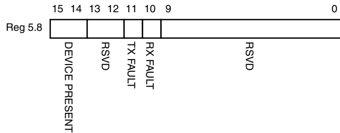
Figure 5-35: DTE XS Status 2 Register
