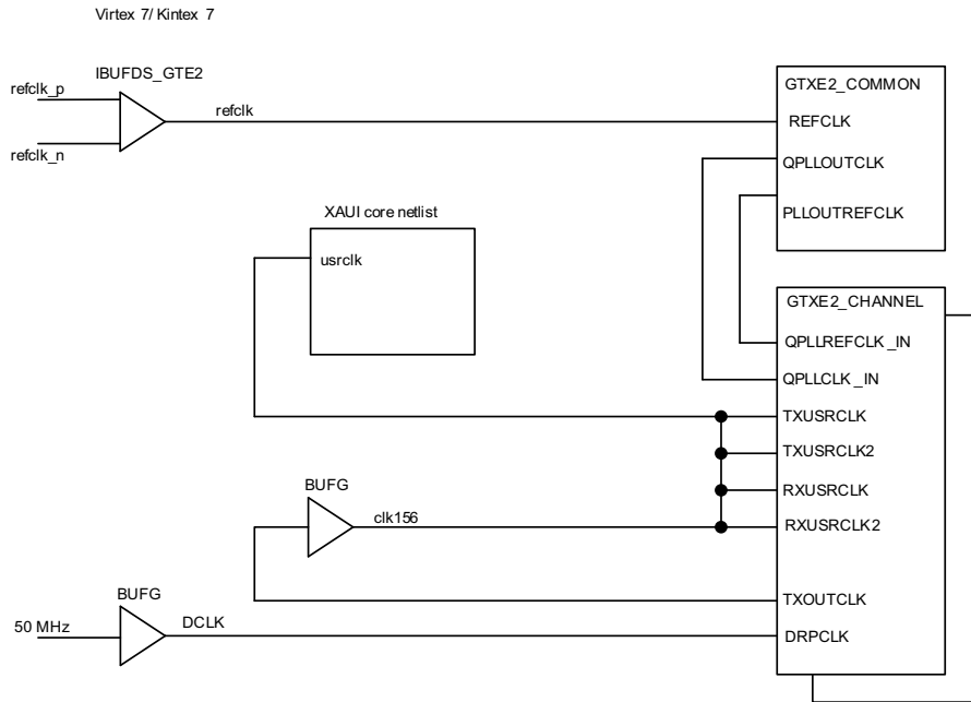
Figure 6-2: Clock Scheme for Internal Client-Side Interface: 7 Series GTX Transceivers
