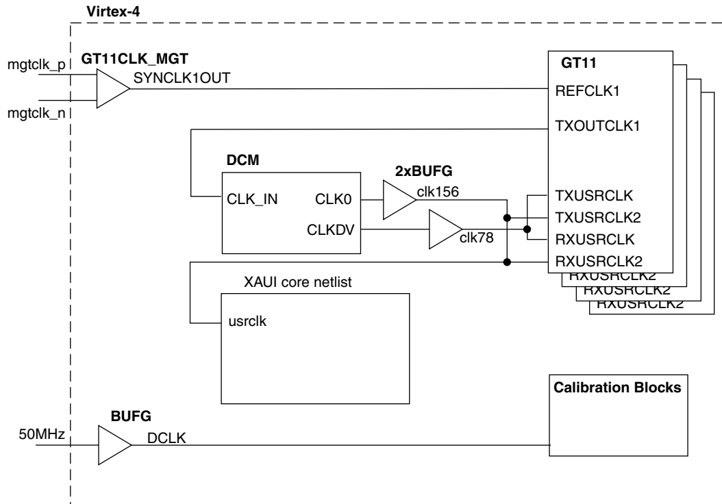
Figure 6-8: Clock Scheme for Internal Client-Side Interface: Virtex-4 FPGAs
