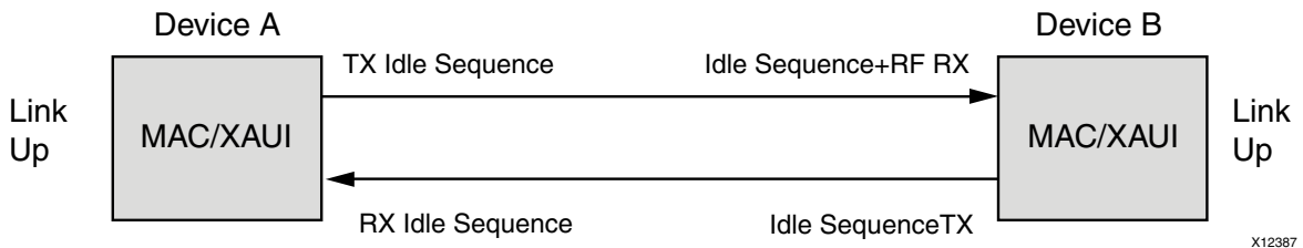
Figure C-6: Normal Operation
