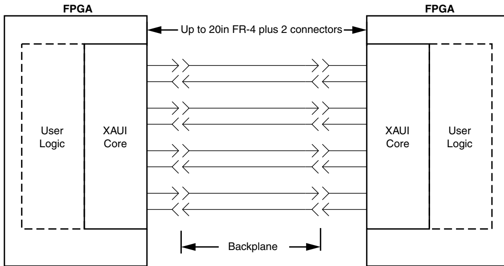
Figure 4-2: Typical Backplane Application for XAUI
