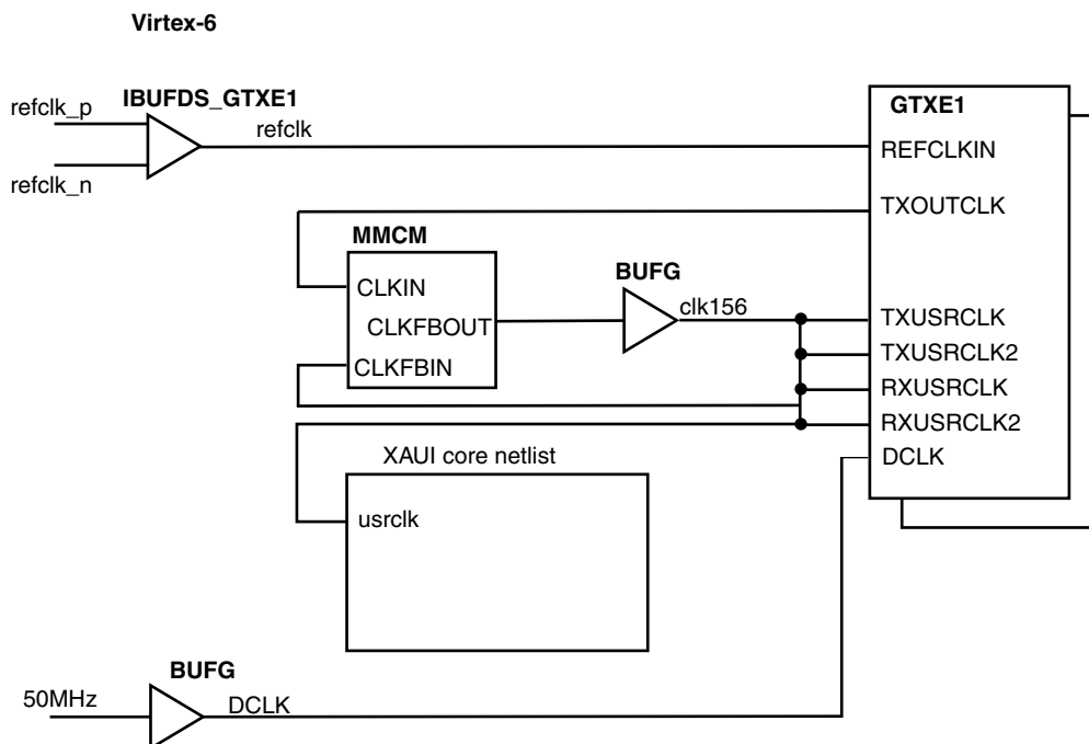
Figure 6-4: Clock Scheme for Internal Client-Side Interface: Virtex-6 FPGAs
