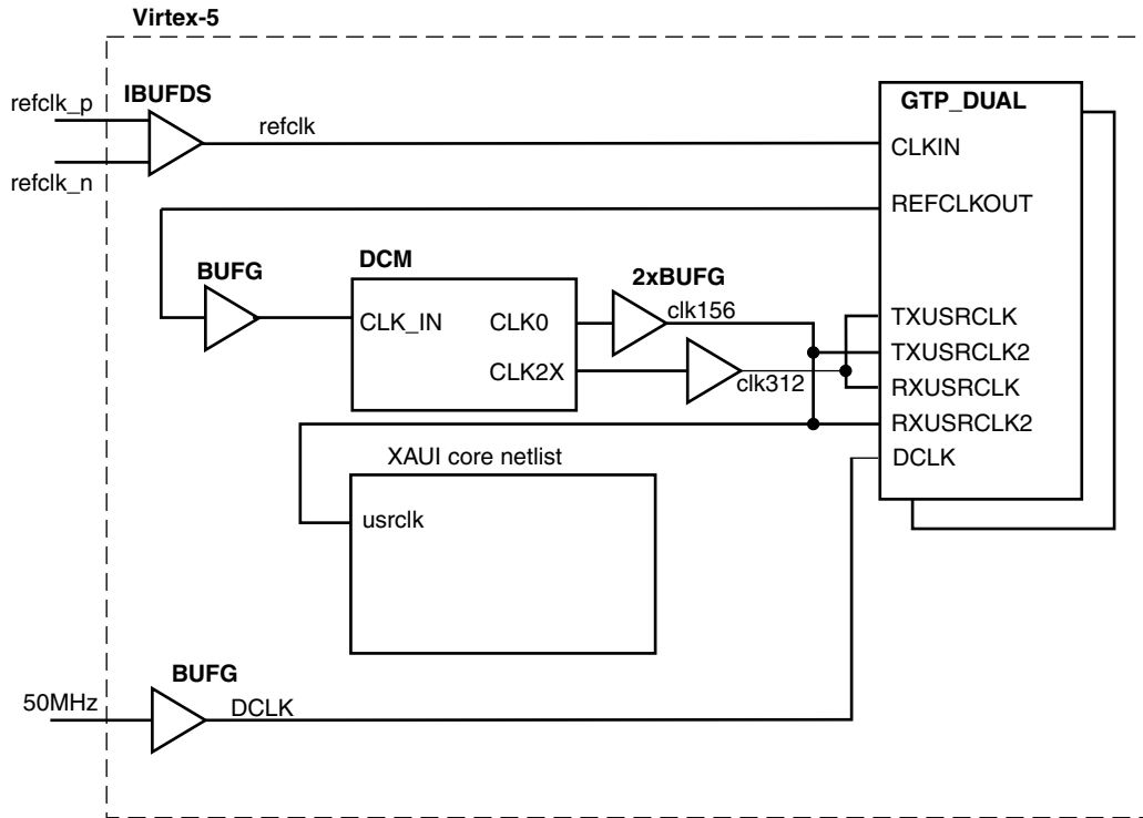
Figure 6-6: Clock Scheme for Internal Client-Side Interface: Virtex-5 LXT/SXT FPGAs
