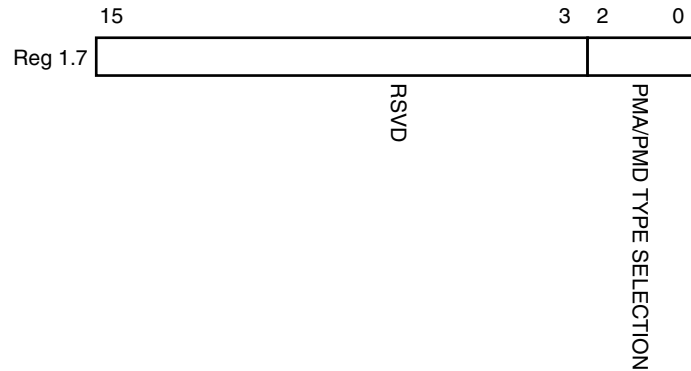
Figure 5-16: 10G PMA/PMD Control 2 Register
