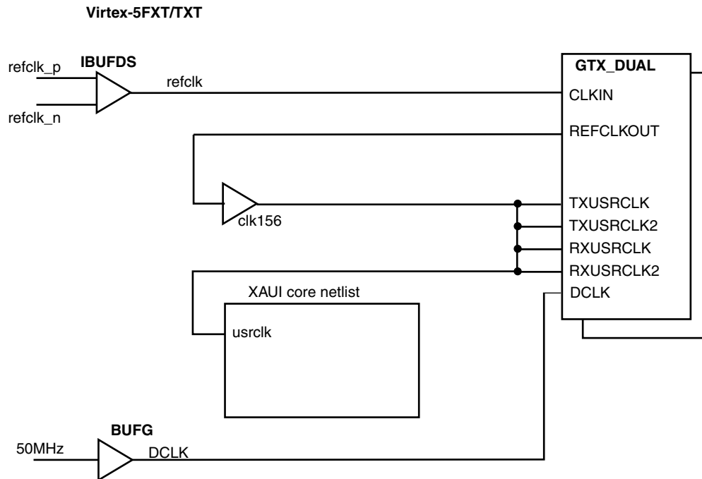
Figure 6-7: Clock Scheme for Internal Client-Side Interface: Virtex-5 FXT/TXT FPGAs
