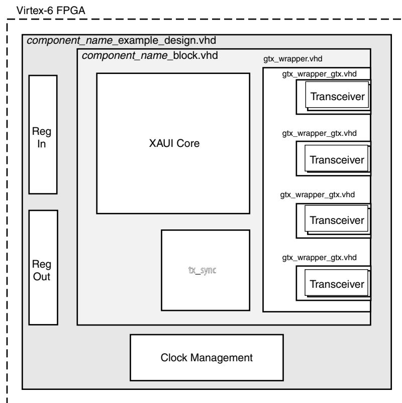
Figure 12-3: Example HDL Wrapper for XAUI without XGMII (Virtex-6 FPGAs)
