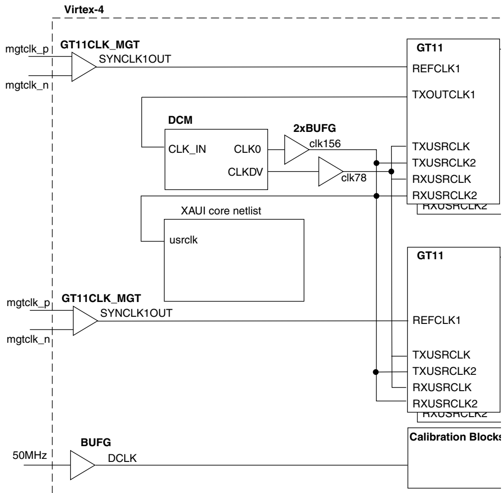
Figure 6-9: Clocking Using Two Columns
