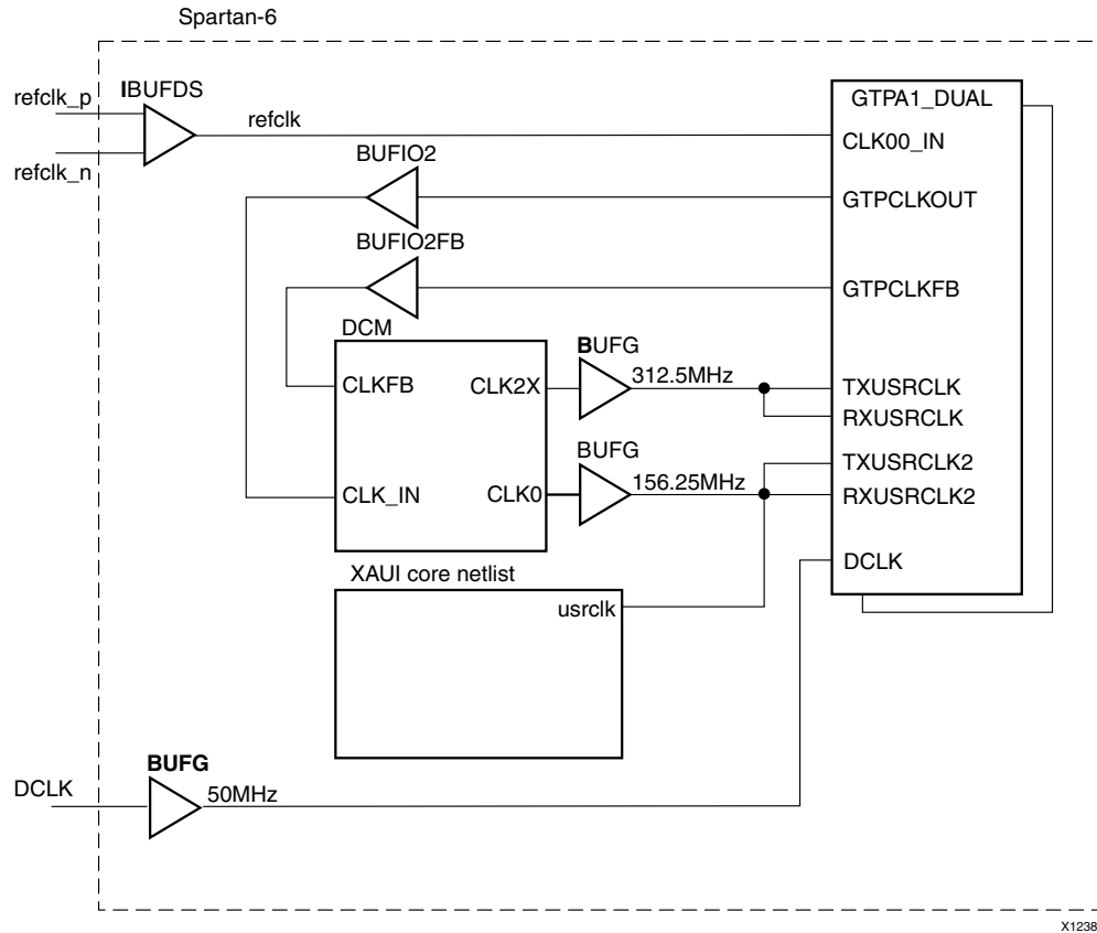
Figure 6-5: Clock Scheme for Internal Client-Side Interface: Spartan-6 LXT FPGAs
