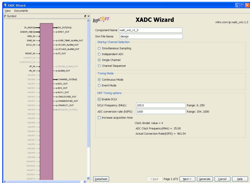
Figure 3-4: XADC Setup - Page 1
