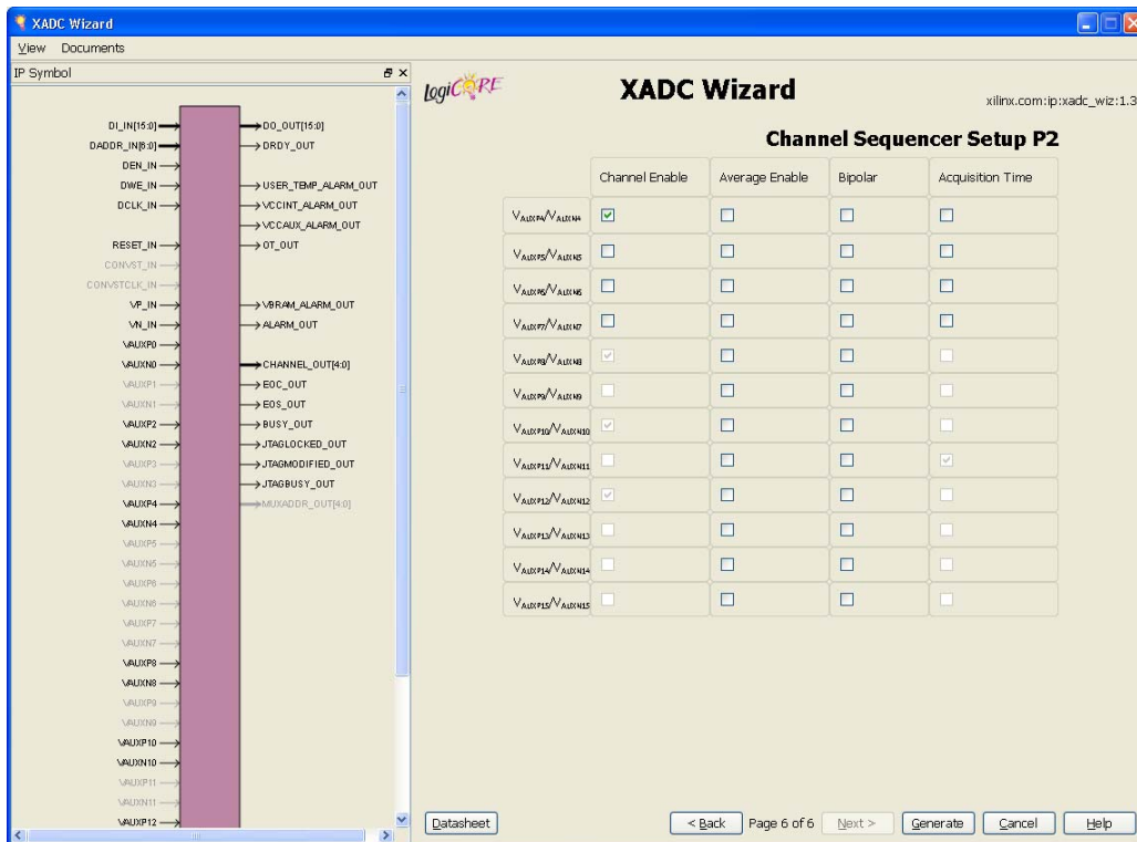
Figure 3-9: Channel Sequencer Setup P2 - Page 6
