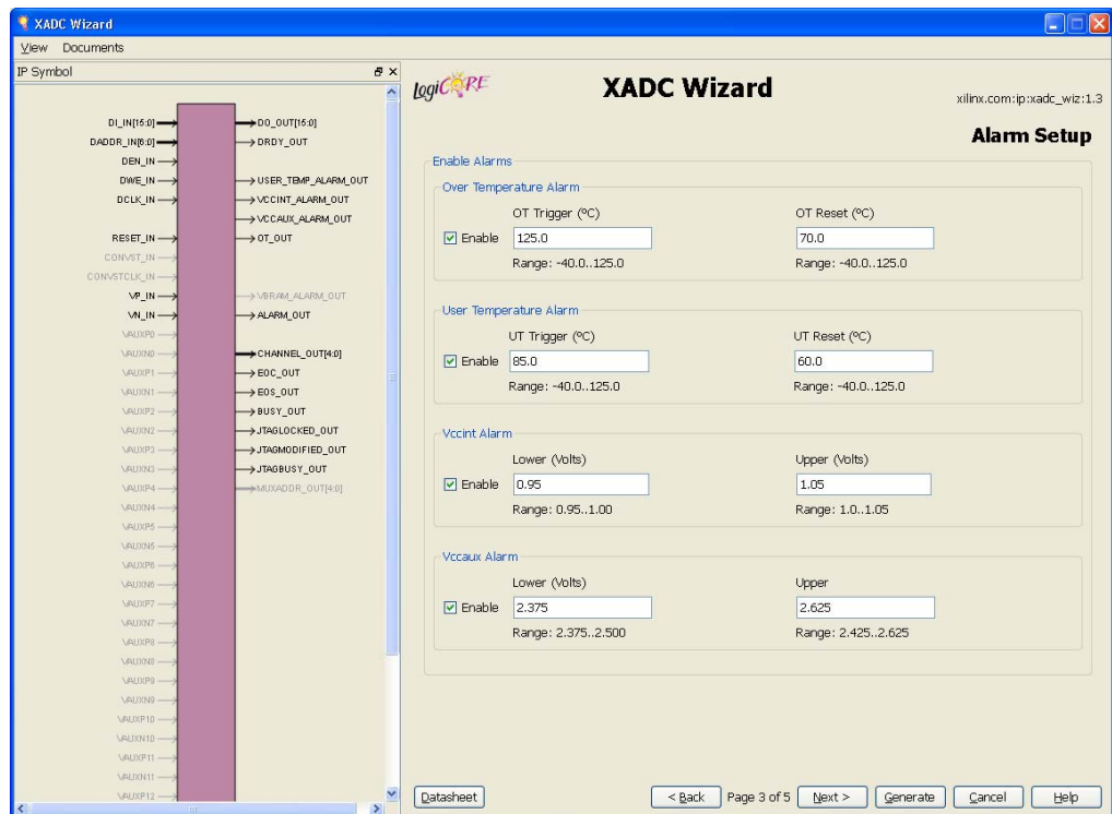
Figure 3-6: Alarm Setup - Page 3
