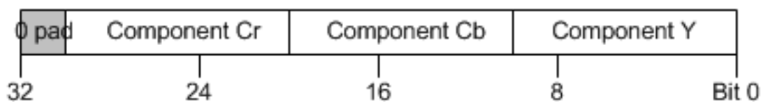
Figure 2-2: YCbCr 4:4:4 Data Encoding on s_axis_video_data and m_axis_video_data
