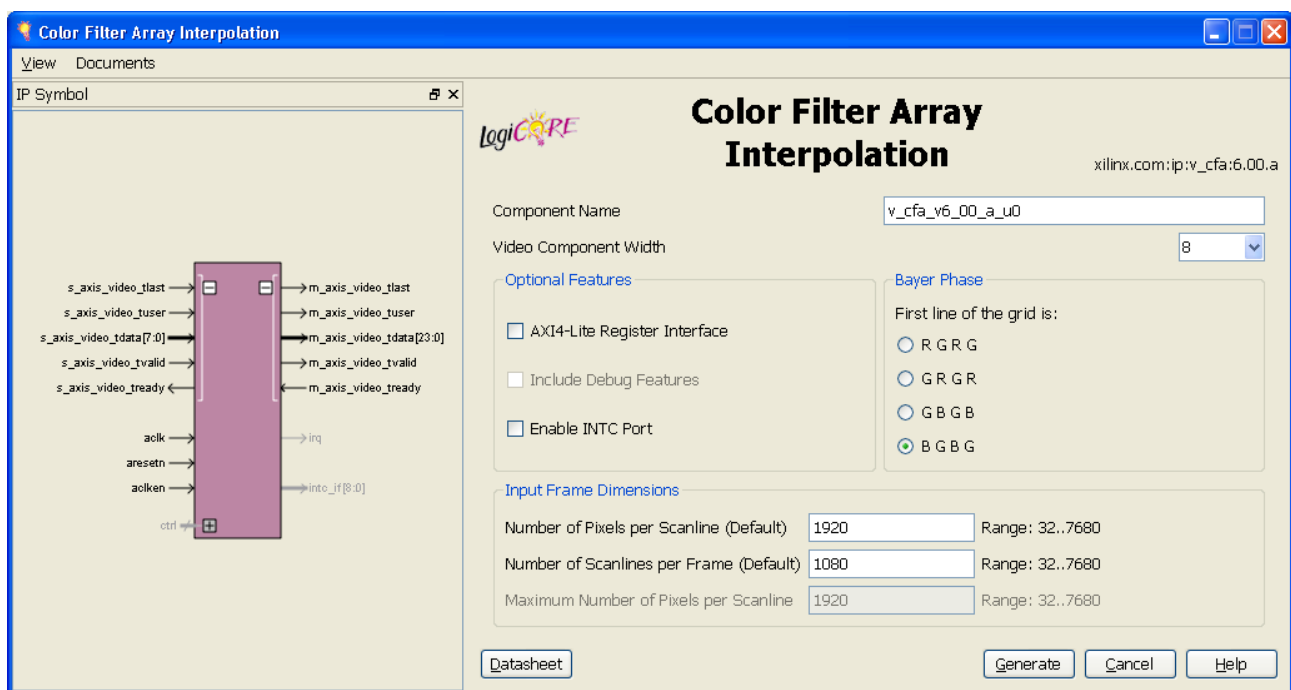
Figure 8-1: Color Filter Array Interpolation CORE Generator GUI
