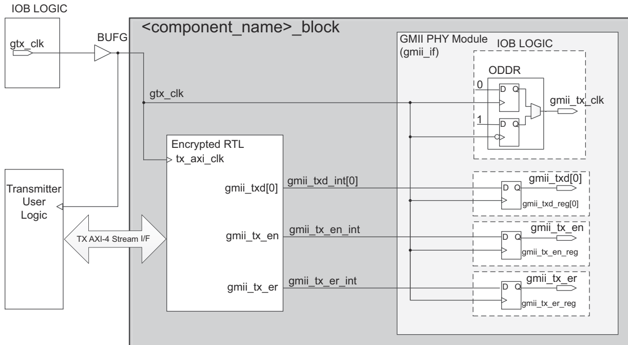
Figure 3-80: 1 Gb/s GMII Transmitter and Clock Logic
