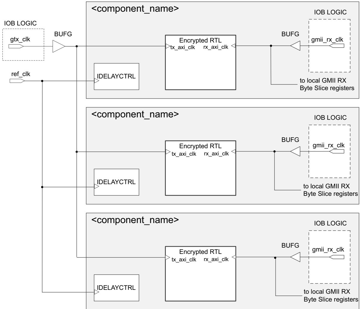
Figure 3-82: Clock Resource Sharing for 1 Gb/s GMII
