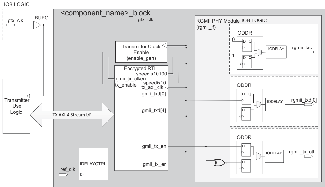
Figure 3-90: Tri-Speed RGMII Transmitter and Clock Logic
