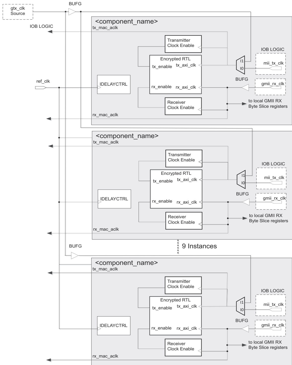
Figure 3-89: Clock Resource Sharing for Tri-Speed GMII with GTX Clock BUFG
