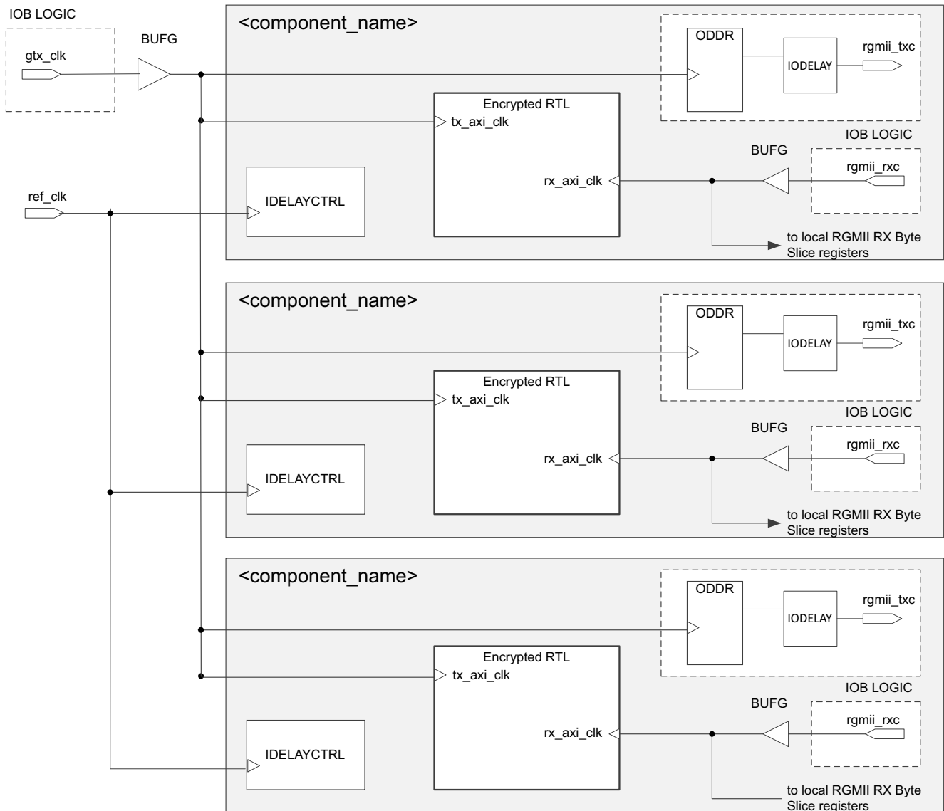
Figure 3-85: Clock Resource Sharing for 1 Gb/s RGMII
