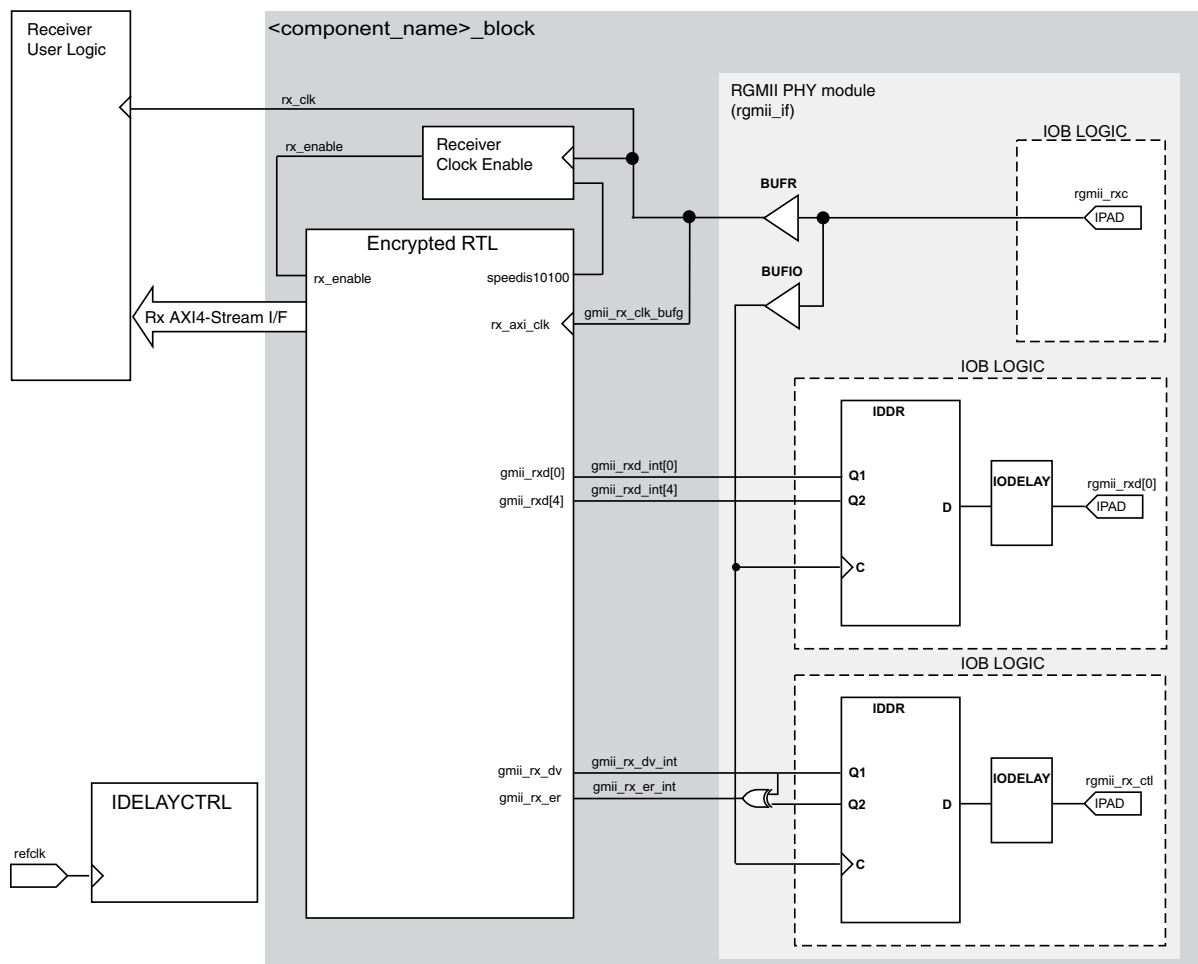
Figure 3-76: Tri-Speed RGMII Receiver and Clock Logic for 7 Series Devices
