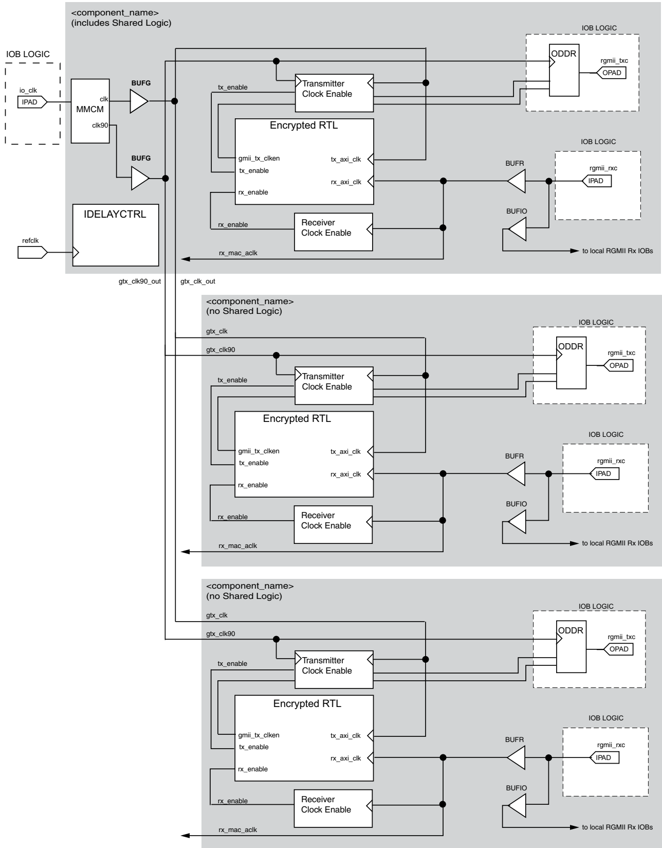
Figure 3-78: Clock Resource Sharing for Tri-Speed RGMII in 7 Series Devices Using HR I/O
