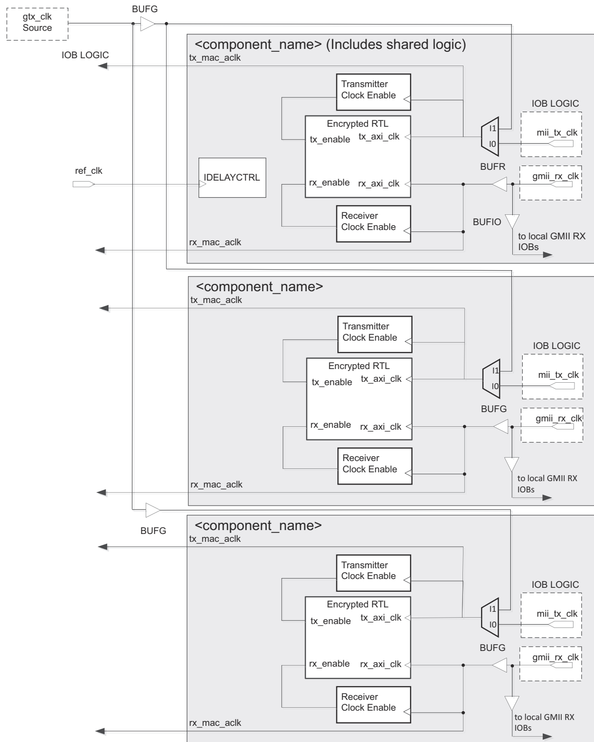
Figure 3-73: Clock Resource Sharing for Tri-Speed GMII in 7 Series Devices with GTX Clock BUFG
