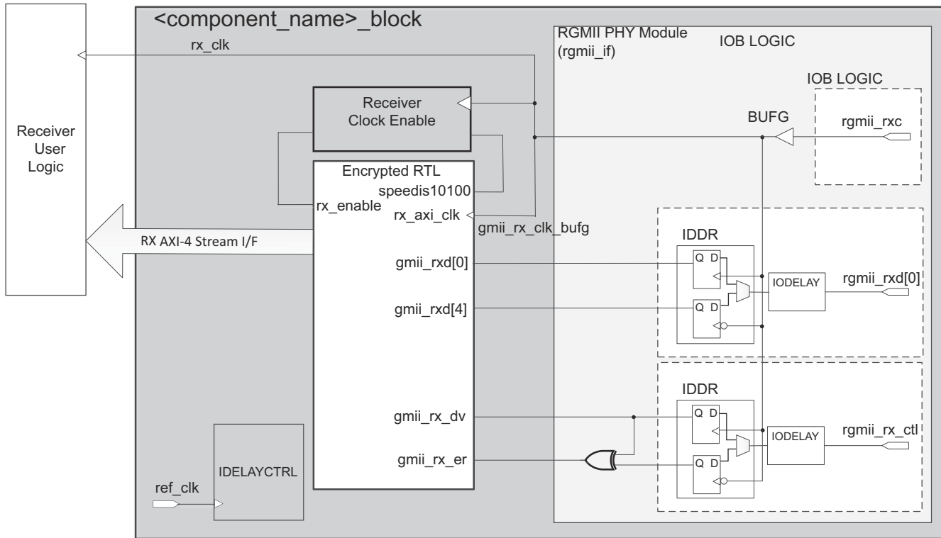
Figure 3-91: Tri-Speed RGMII Receiver and Clock Logic
