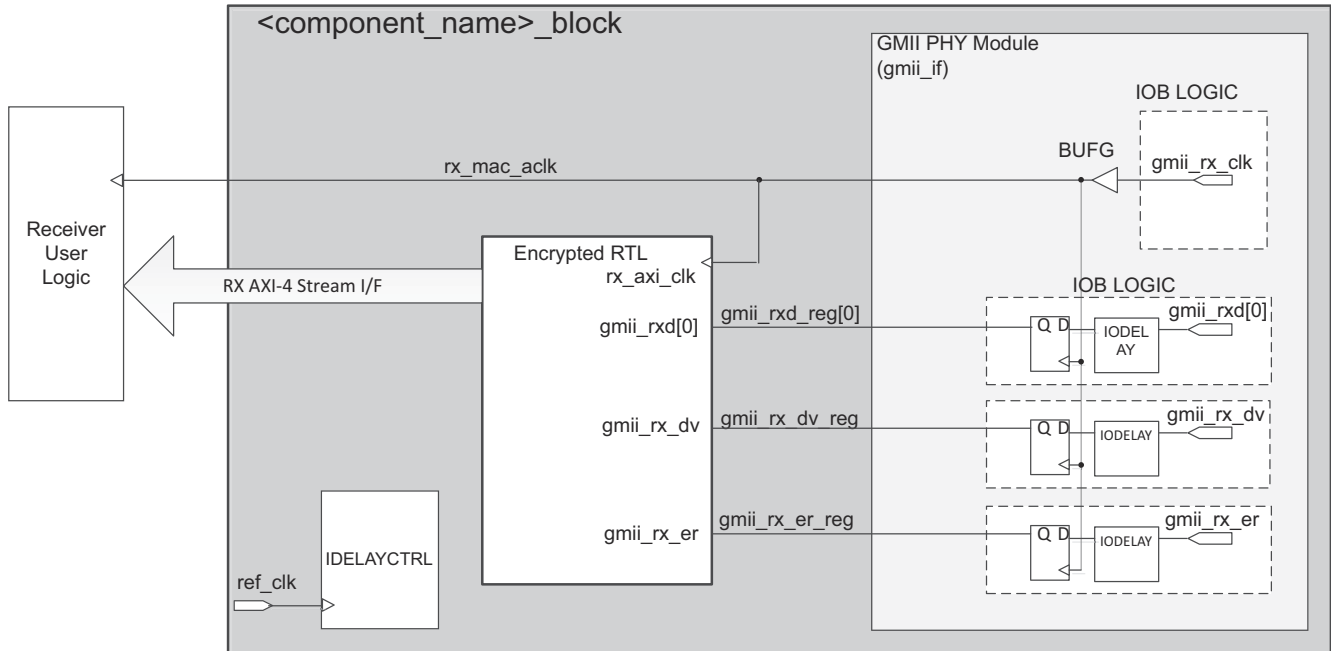
Figure 3-81: 1 Gb/s GMII Receiver and Clock Logic
