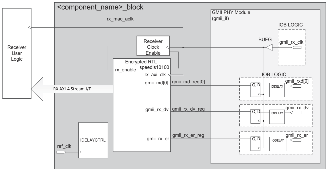
Figure 3-87: Tri-Speed GMII Receiver and Clock Logic
