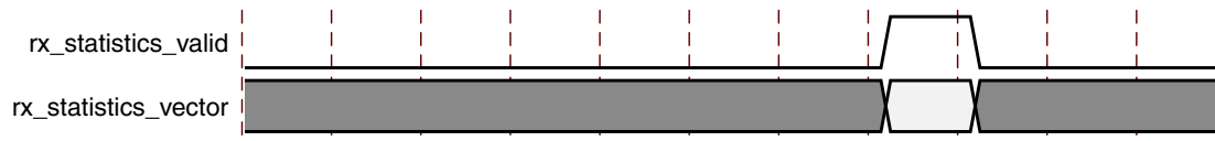
Figure 3-19: Receiver Statistics Vector Timing
