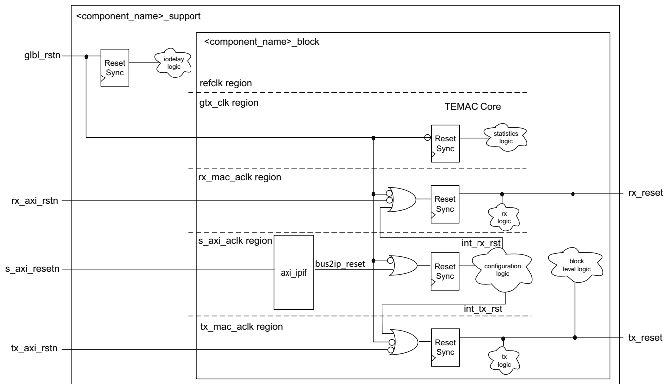
Figure 3-8: Reset Architecture
