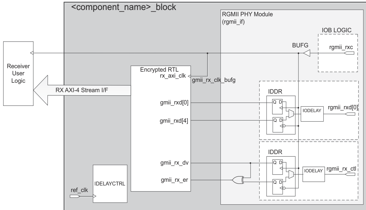
Figure 3-84: 1 Gb/s RGMII Receiver and Clock Logic
