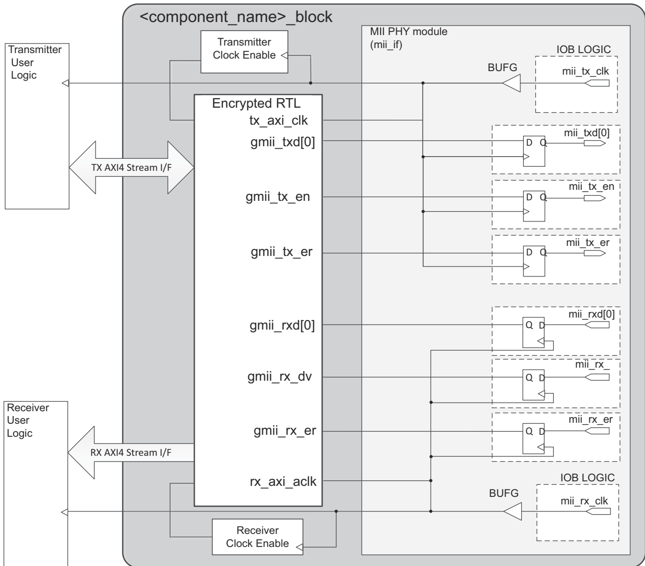
Figure 3-79: MII Transceiver, Receiver and Clock Logic for UltraScale Architecture-Based Devices
