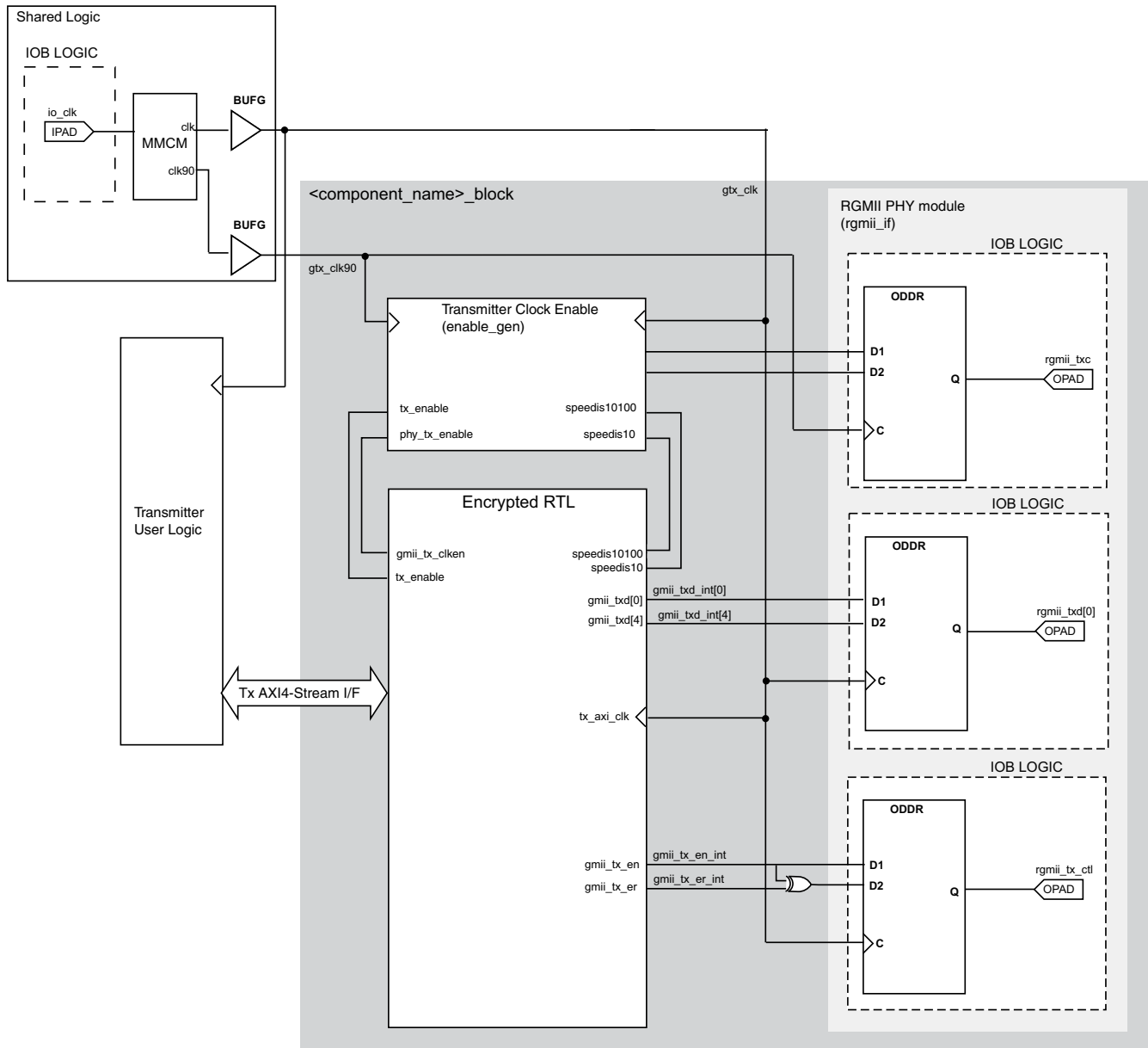
Figure 3-75: Tri-Speed RGMII Transmitter and Clock Logic for 7 Series Devices Using HR I/O
