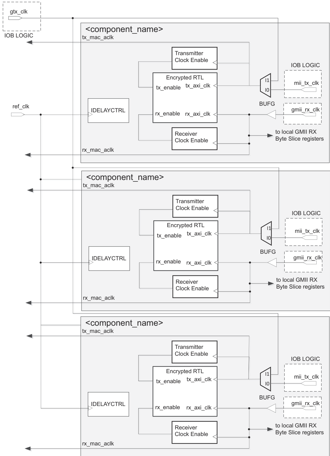
Figure 3-88: Clock Resource Sharing for Tri-Speed GMII
