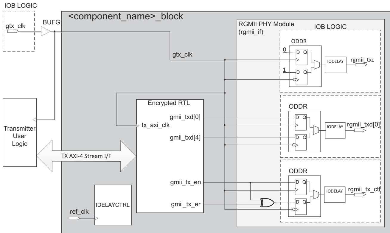
Figure 3-83: 1 Gb/s RGMII Transmitter and Clock Logic
