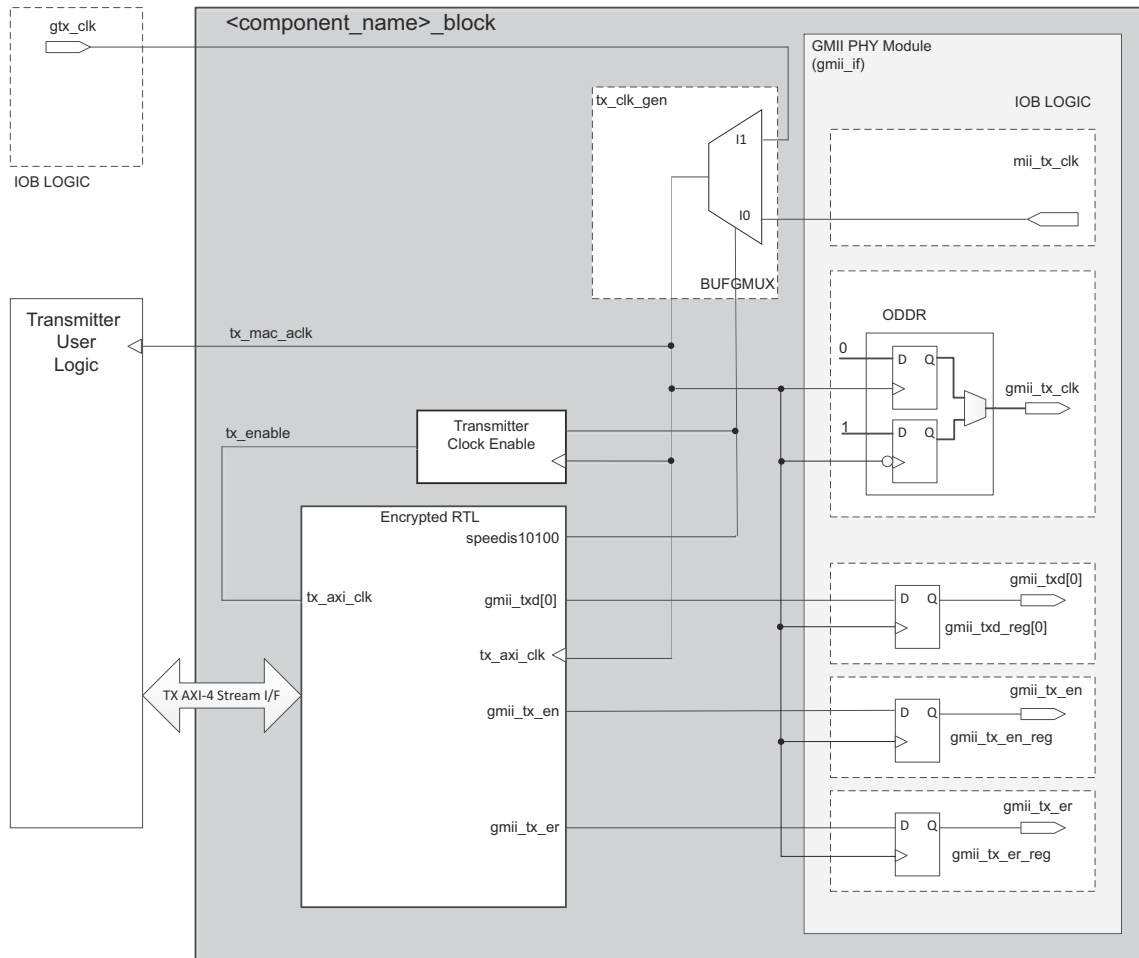
Figure 3-86: Tri-Speed GMII Transmitter and Clock Logic
