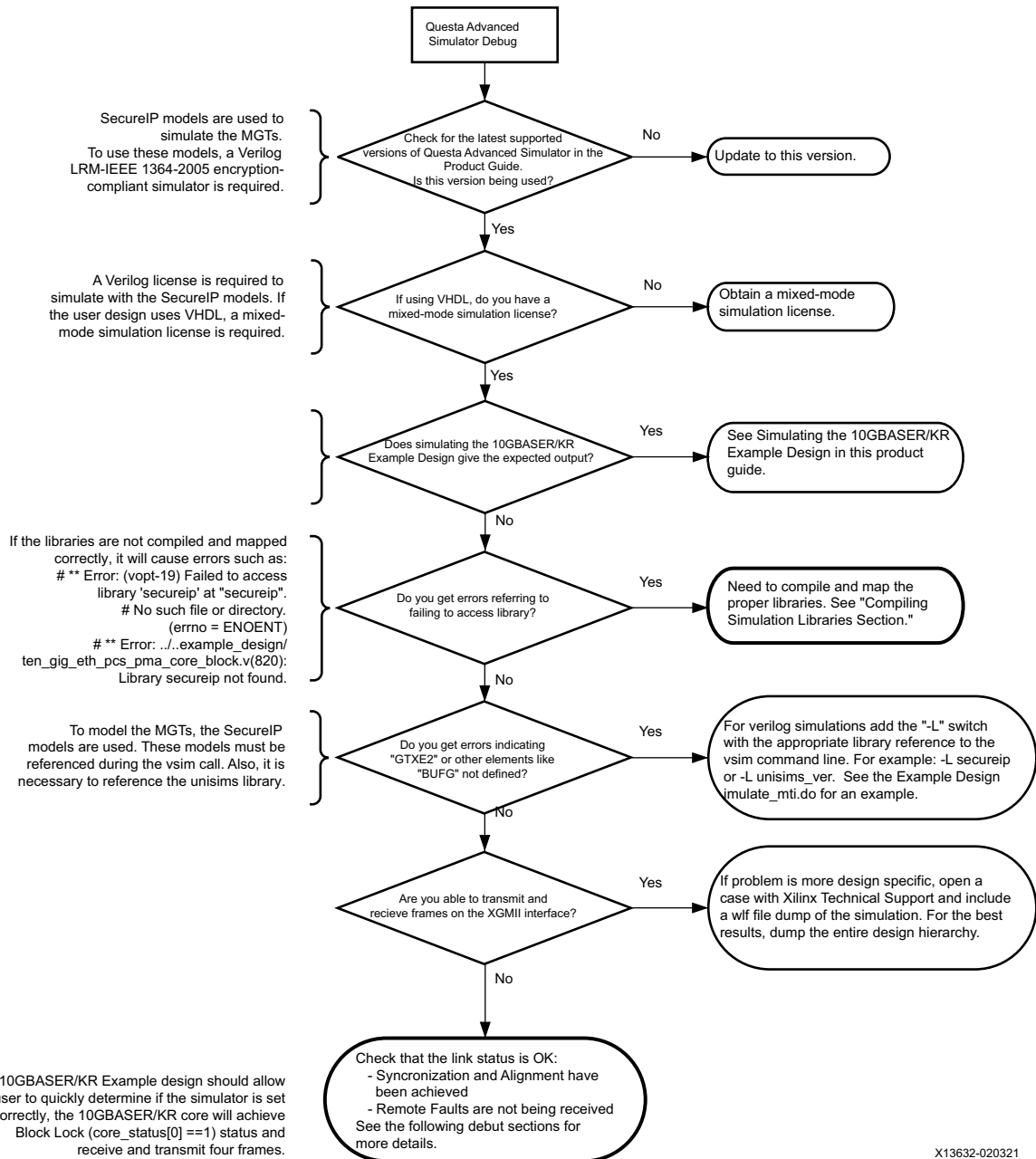
Figure C-1: Simulation Debug Flow
