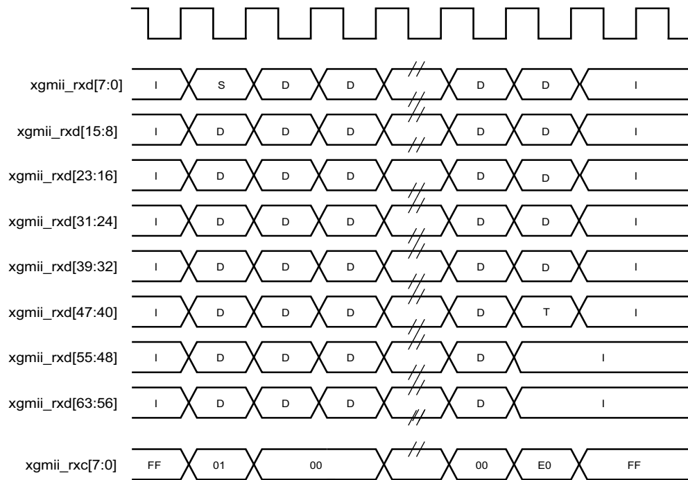
Figure 3-9: Frame Reception Across the 64-Bit XGMII Interface
