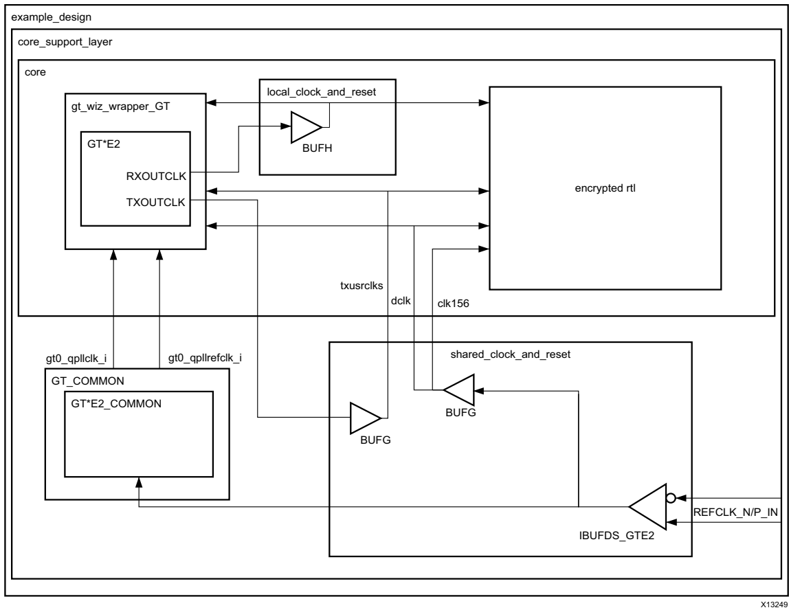
Figure 3-16: Clocking Scheme for Internal Client-Side Interface: 7 Series FPGAs
