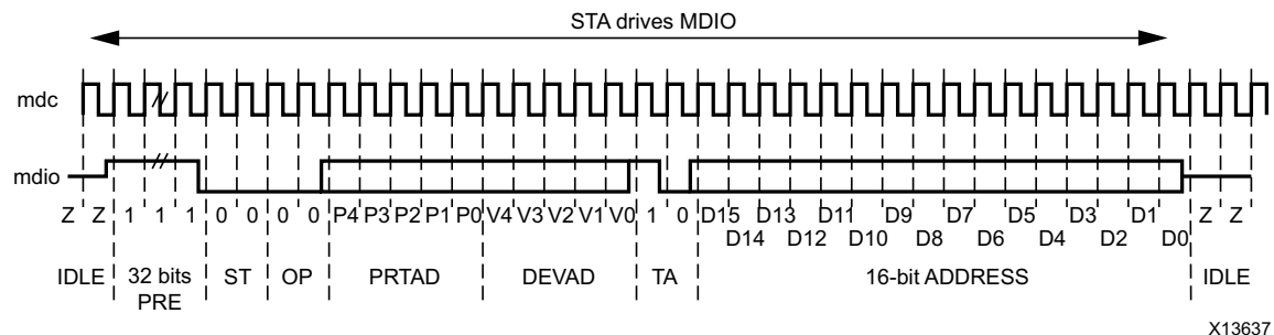
Figure 3-10: MDIO Set Address Transaction
