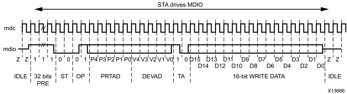
Figure 3-11: MDIO Write Transaction
