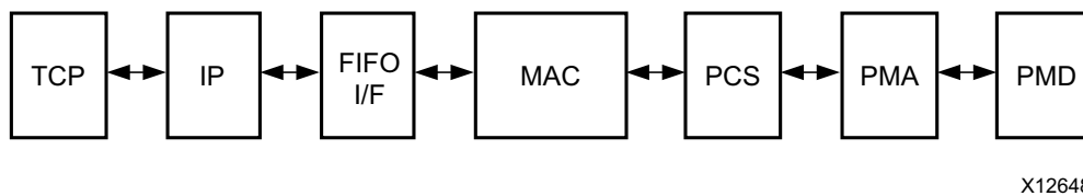
Figure 1-3: Typical Ethernet System Architecture
