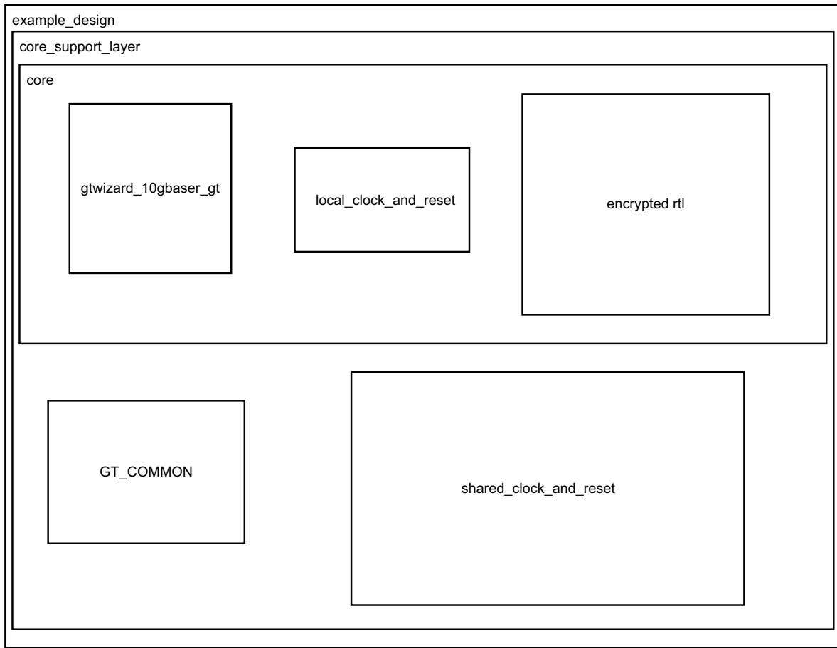
Figure 5-1: Example HDL Wrapper for 10GBASE-R/KR
