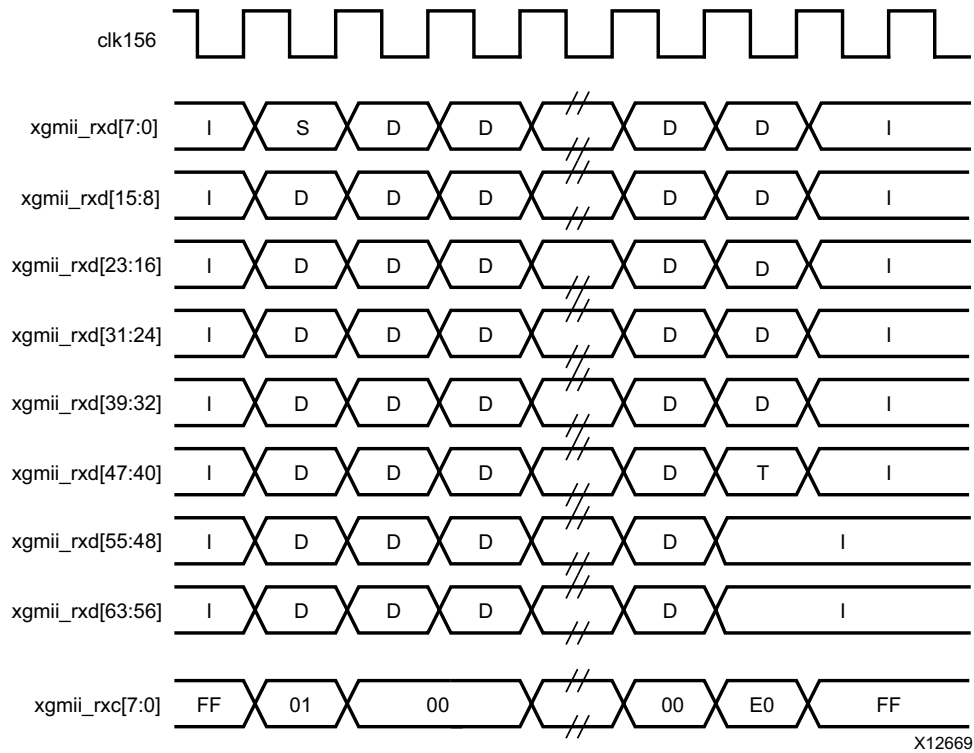
Figure 2-2: Receiving a Frame Through the Client-Side Interface
