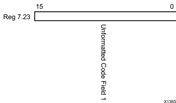
Figure 2-49: AN XNP Transmit Register 1
