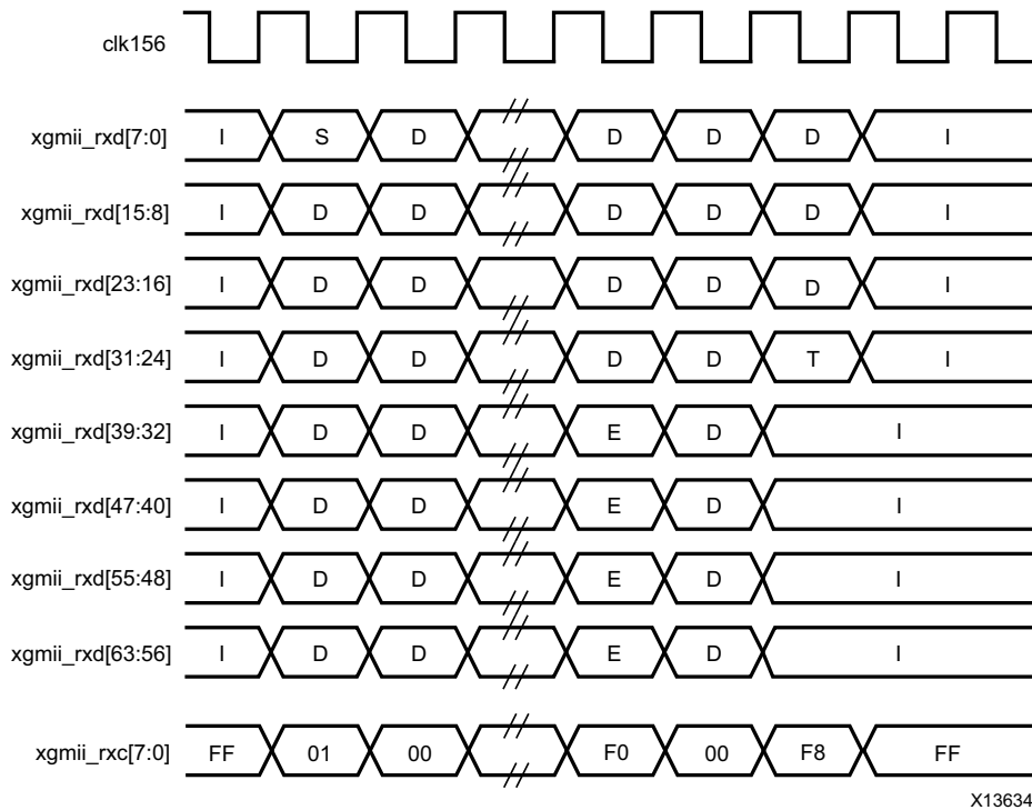
Figure 3-8: Frame Reception with Error Across the Internal 64-bit Client Interface
