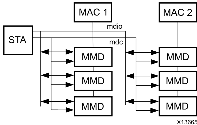
Figure 3-9: A Typical MDIO-Managed System
