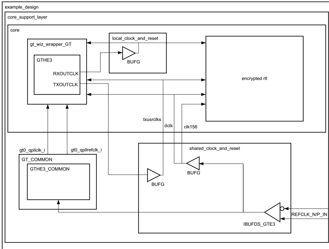
Figure 3-17: Clocking Scheme for Internal Client-Side Interface: UltraScale Devices
