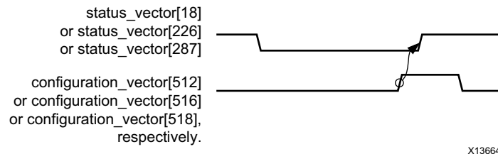
Figure 3-15: Setting the Latching-Low Bits
