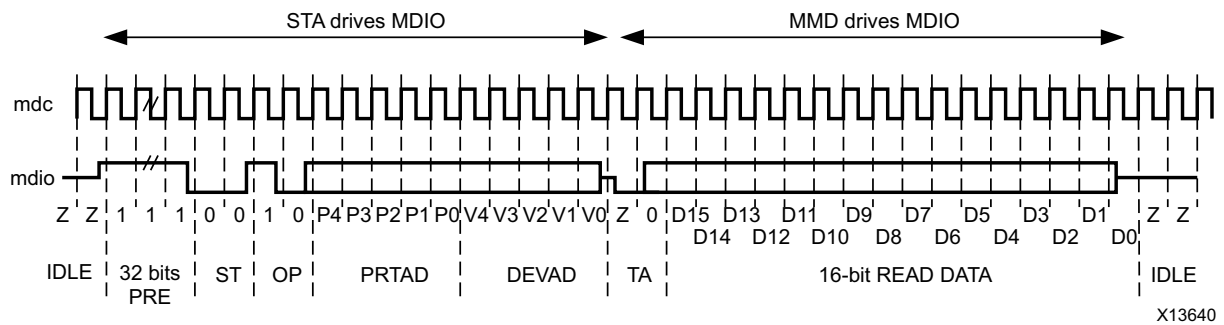
Figure 3-13: MDIO Read-and-increment Transaction
