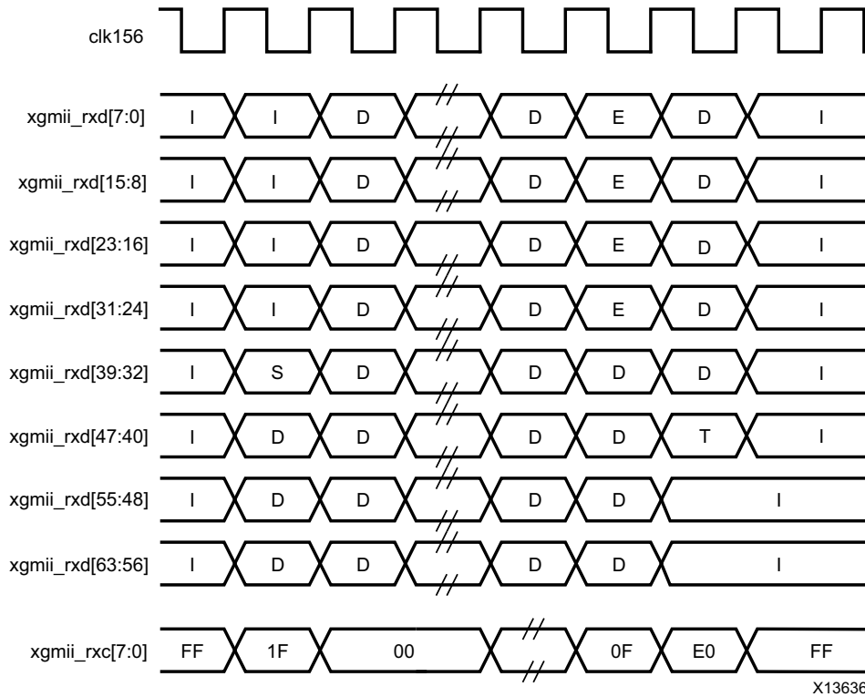
Figure 3-6: Frame Transmission with Error Across Internal 64-bit Client-Side I/F
