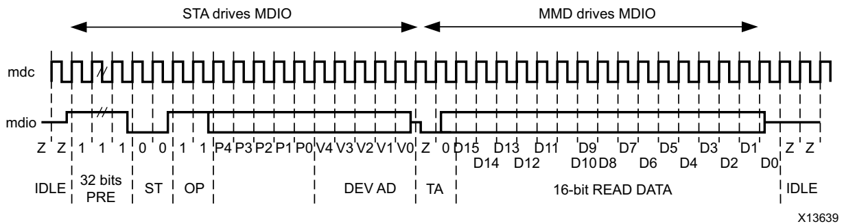
Figure 3-12: MDIO Read Transaction
