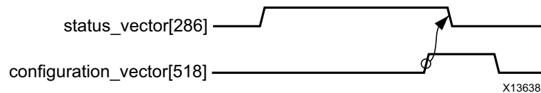
Figure 3-14: Clearing the Latching-High Bits
