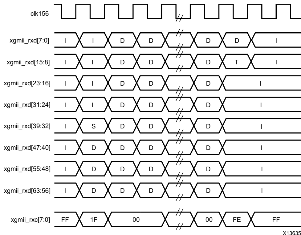
Figure 3-5: Normal Frame Transmission Across the Internal 64-bit Client-Side I/F
