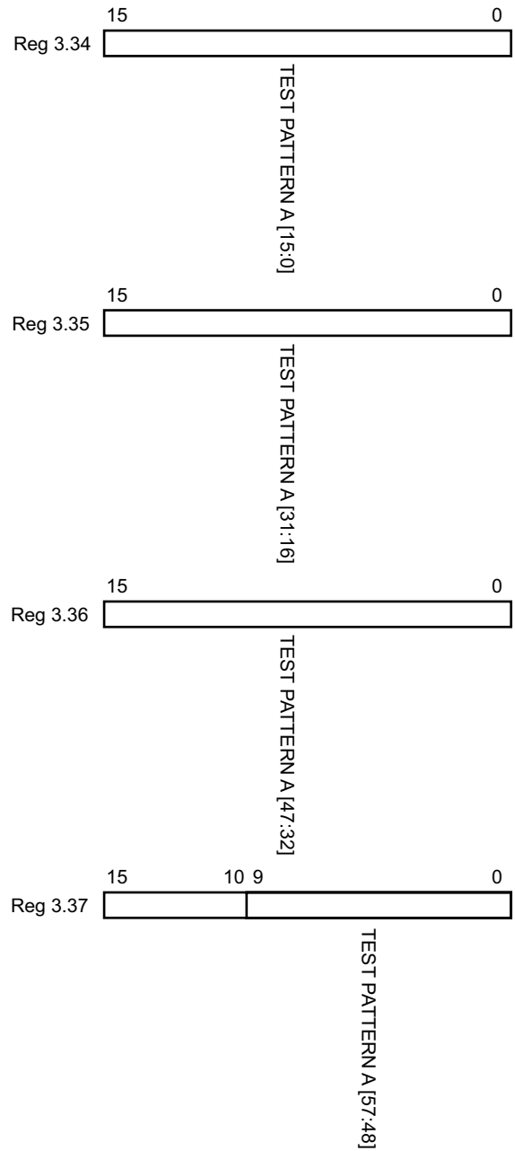
Figure 2-35: 10GBASE-R Test Pattern Seed A0-3 Registers
