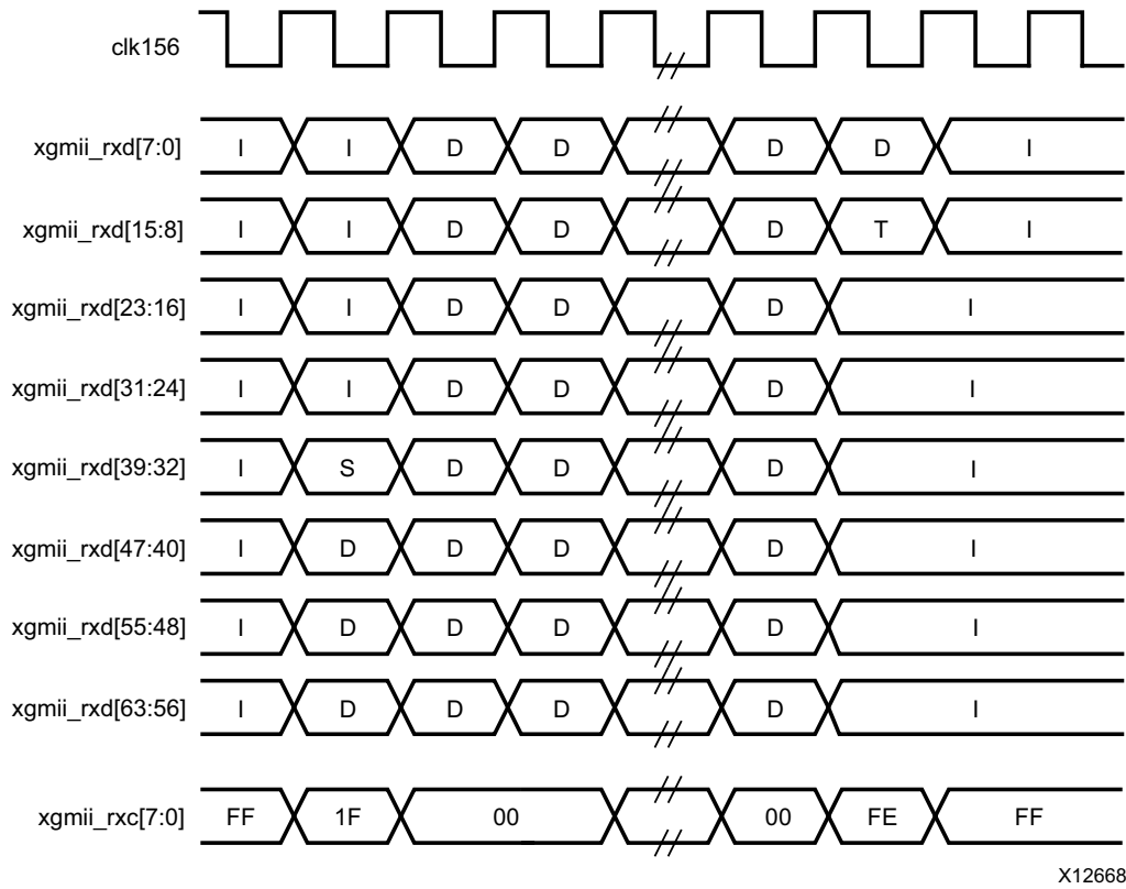
Figure 2-1: Transmitting a Frame Through the Client-Side Interface
