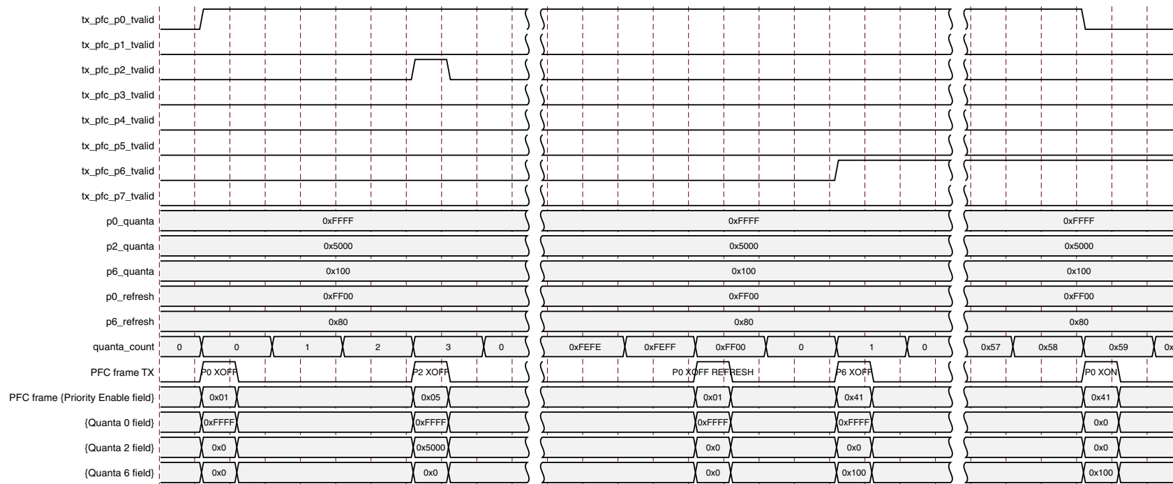
Figure 3-56: TX PFC Frame Transmission
