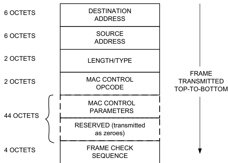
Figure 3-50: MAC Control Frame Format
