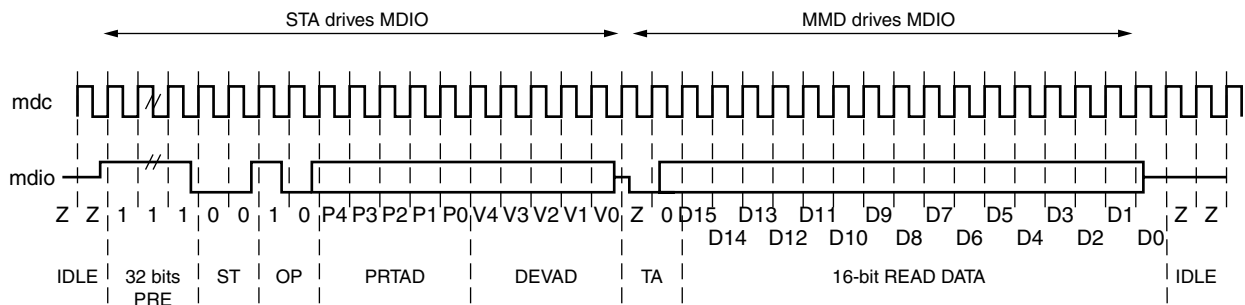
Figure 3-48: MDIO Read-and-Increment Transaction
