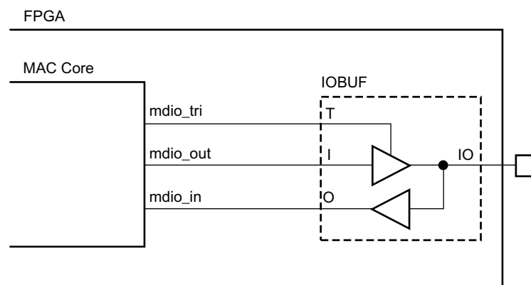
Figure 3-44: Using a SelectIO Interface 3-State Buffer to Drive MDIO
