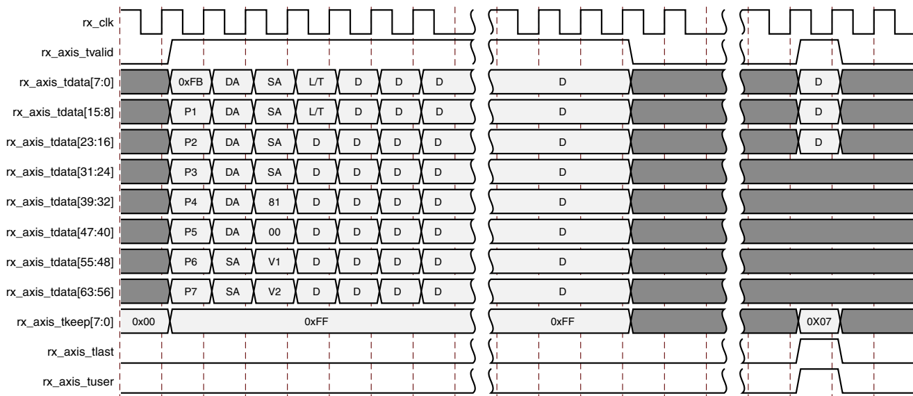
Figure 3-34: Frame Reception with Custom Preamble
