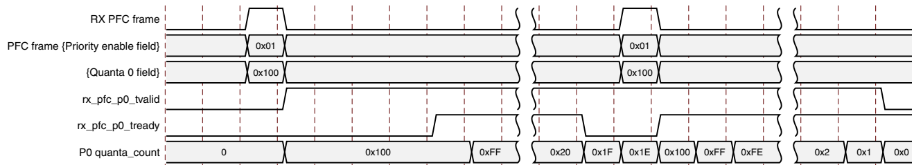
Figure 3-57: RX PFC Frame Reception
