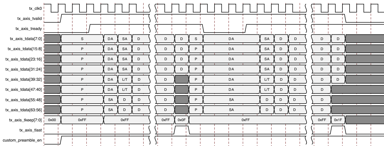
Figure 3-14: Transmission of Custom Preamble in the Continuous Case
