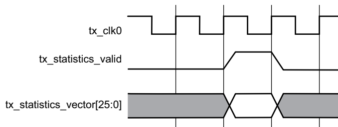
Figure 2-3: Transmitter Statistics Output Timing
