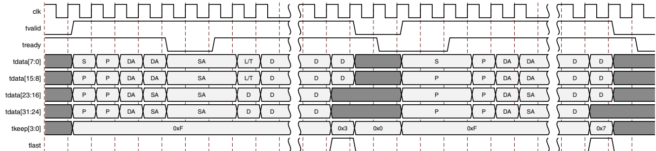
Figure 3-24: Transmission of Custom Preamble in the Non-Continuous Case
