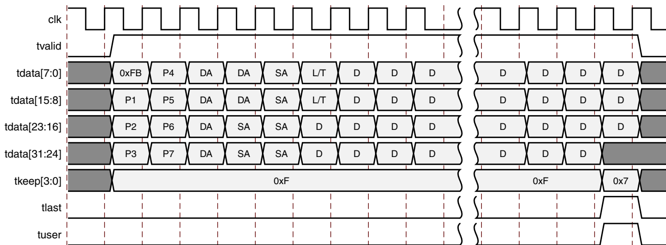
Figure 3-39: Frame Reception with Custom Preamble
