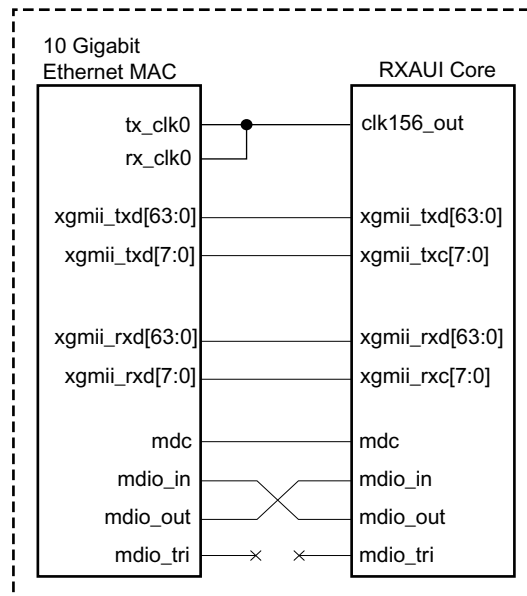
Figure 3-61: 10 Gigabit Ethernet MAC Core Integrated with RXAUI Core
