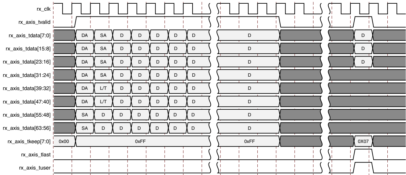
Figure 3-31: Reception of a Good Frame
