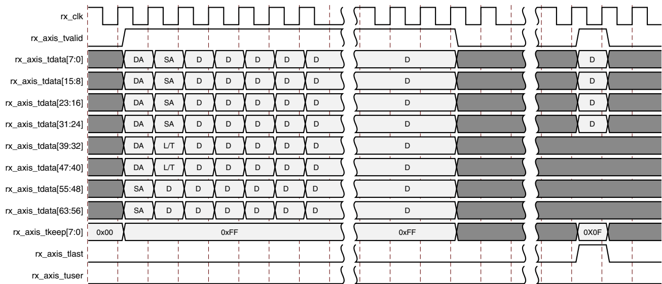
Figure 3-32: Frame Reception with Error
