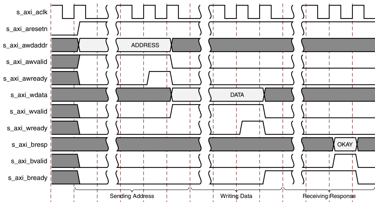
Figure 3-41: Management Register Write Timing
