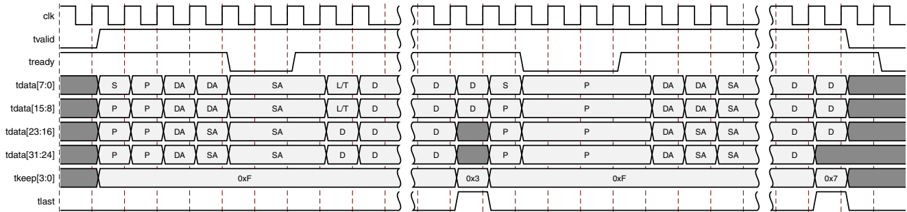
Figure 3-25: Transmission of Custom Preamble in the Continuous Case
