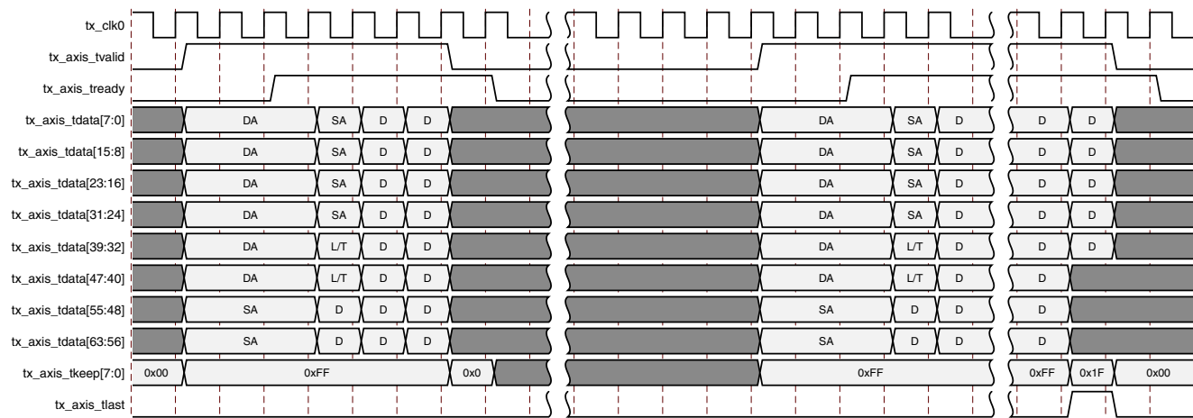
Figure 3-11: Frame Transfer Abort with tx_axis_tvalid Deasserted
