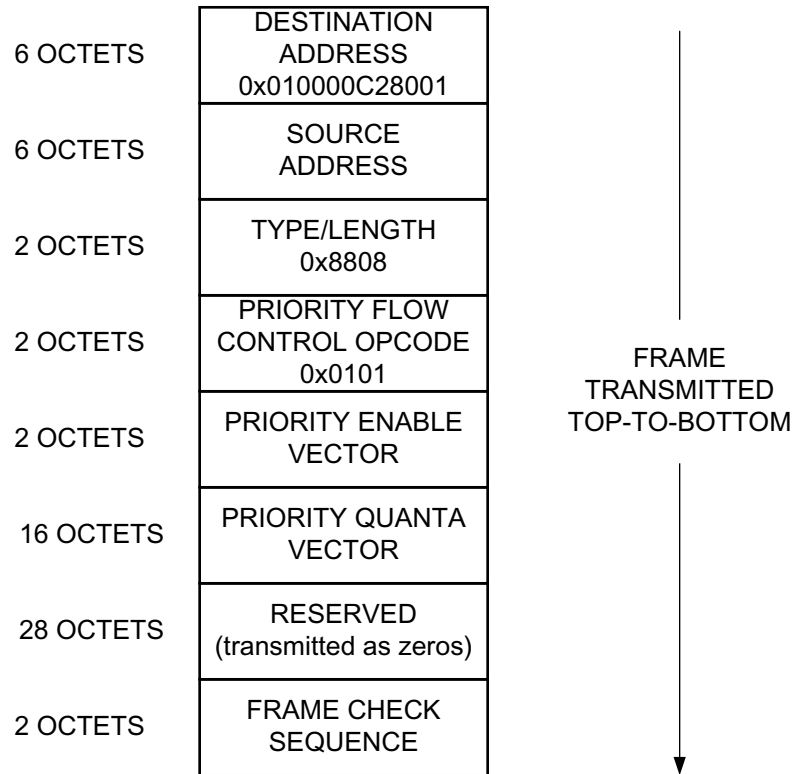
Figure 3-55: MAC Priority Control Flow Frame Format
