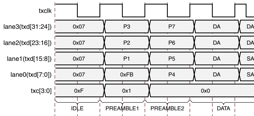
Figure 3-26: XGMII Frame Transmission of Custom Preamble
