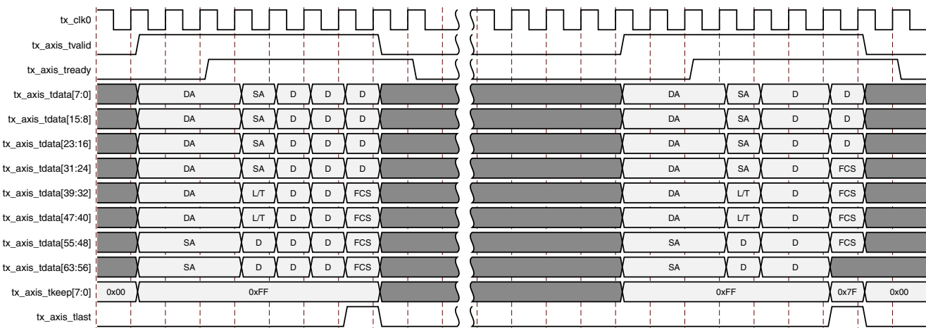
Figure 3-9: Transmission with In-Band FCS Passing
