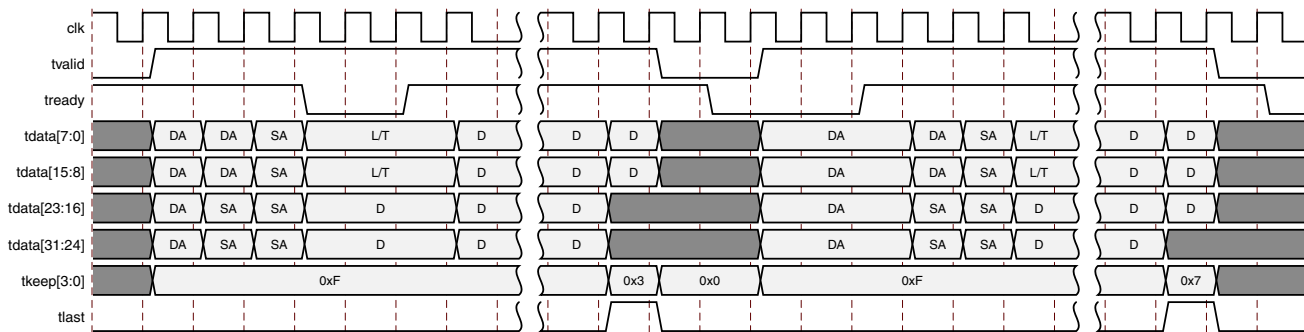
Figure 3-19: Frame Transmission
