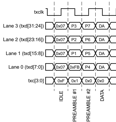
Figure 3-15: XGMII Frame Transmission of Custom Preamble
