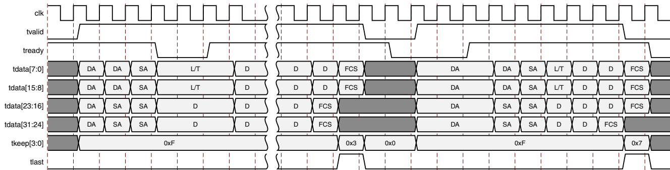
Figure 3-20: Transmission with In-Band FCS Passing
