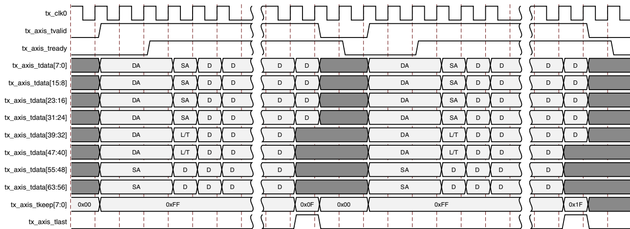
Figure 3-8: Frame Transmission
