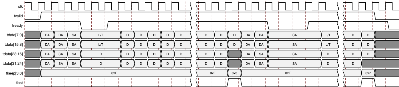
Figure 3-23: Back-to-Back Continuous Transfer on Transmit Client Interface
