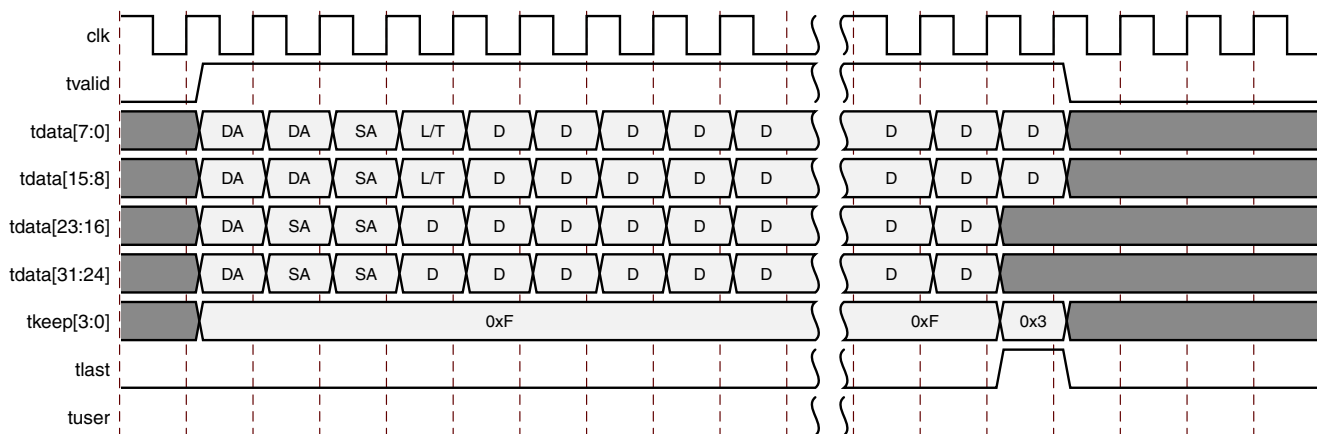
Figure 3-37: Frame Reception with Error
