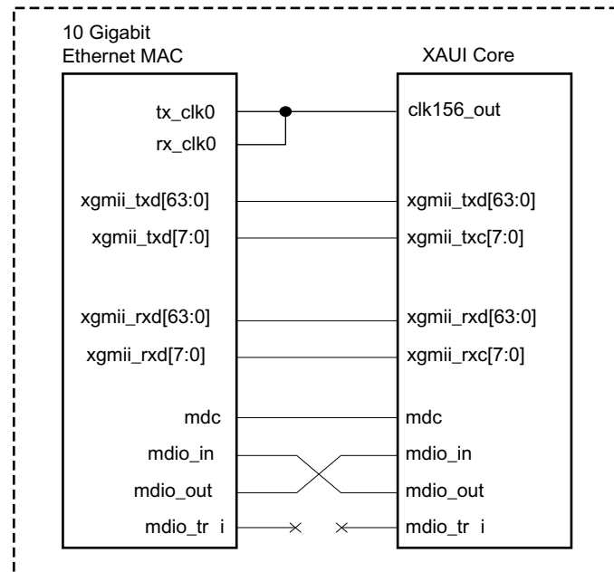
Figure 3-60: 10 Gigabit Ethernet MAC Core Integrated with XAUI Core
