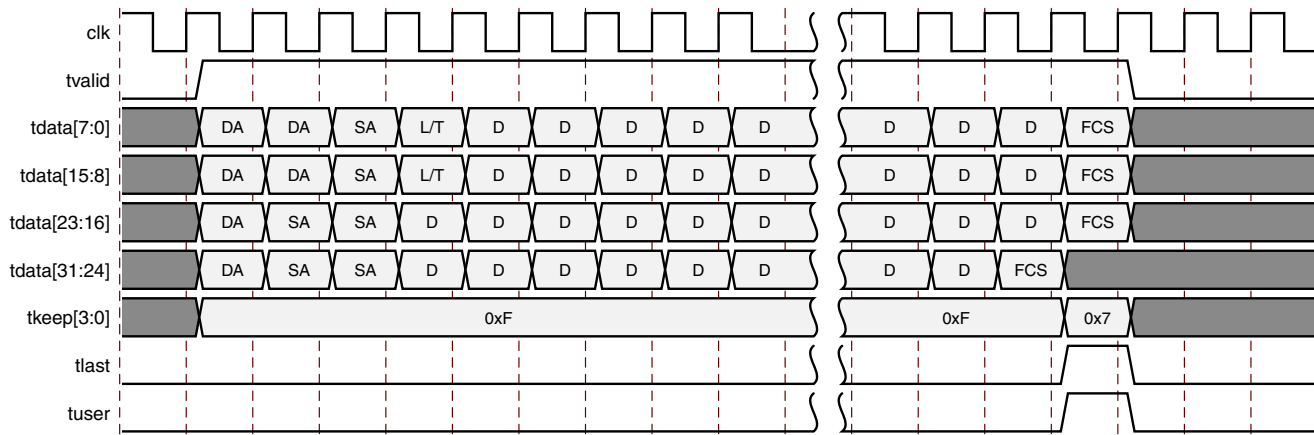
Figure 3-38: Frame Reception with In-Band FCS Passing
