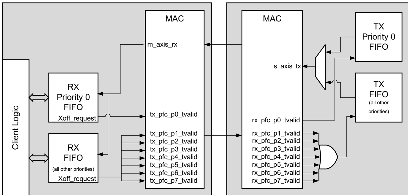
Figure 3-54: Priority Flow Control Requirement
