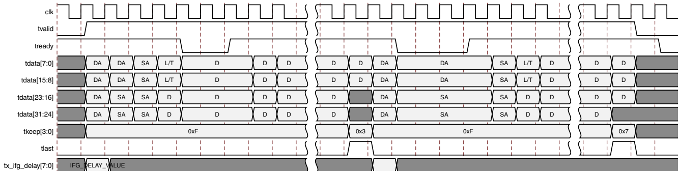
Figure 3-29: Interframe Gap Adjustment
