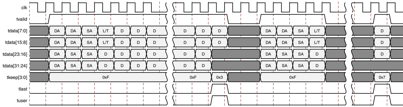
Figure 3-36: Reception of a Good Frame
