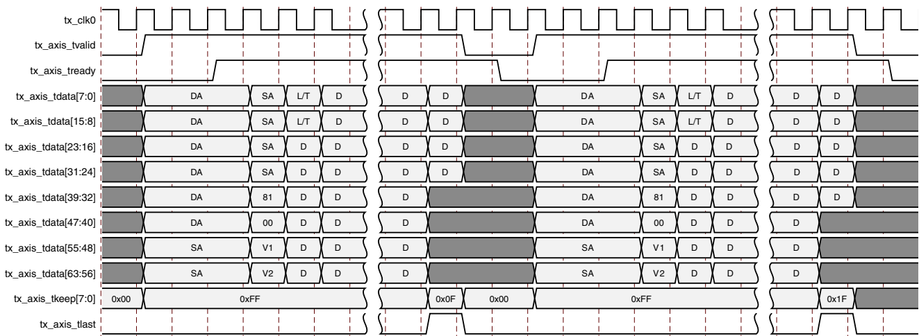
Figure 3-16: VLAN Tagged Frame Transmission
