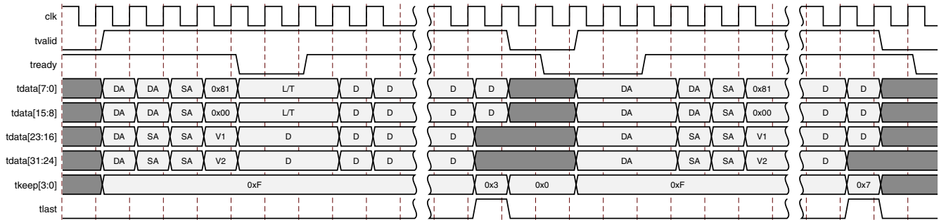
Figure 3-27: VLAN Tagged Frame Transmission
