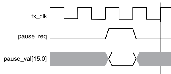
Figure 3-51: Pause Request Timing
