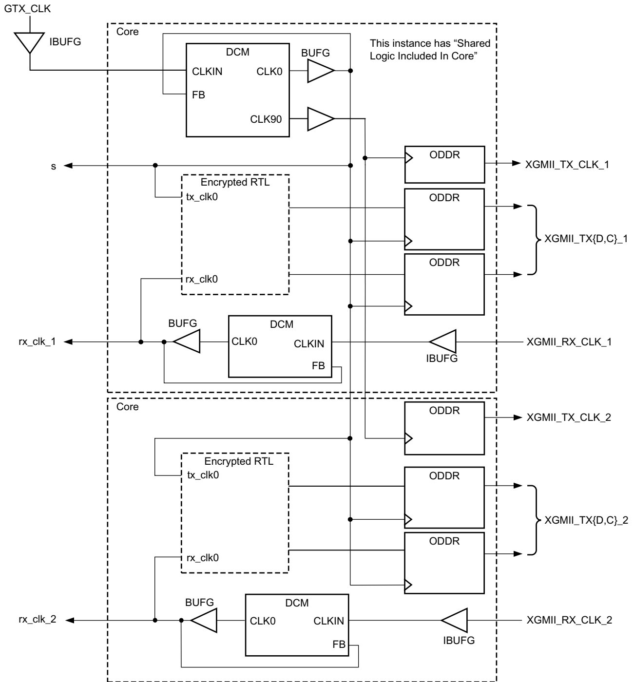
Figure 3-59: Clock Management, Multiple Core Instances with XGMII
