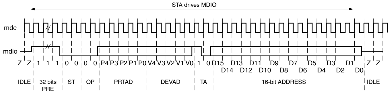
Figure 3-45: MDIO Set Address Transaction
