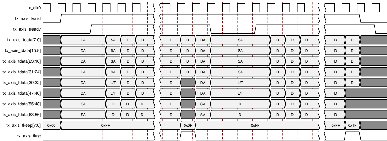
Figure 3-12: Back-to-Back Continuous Transfer on Transmit Client Interface
