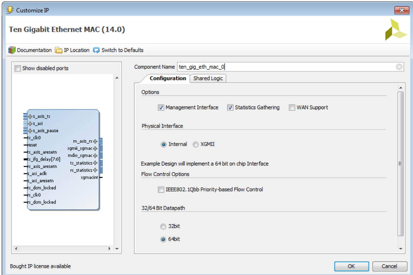
Figure 4-1: 10 Gigabit Ethernet MAC Customization Screen
