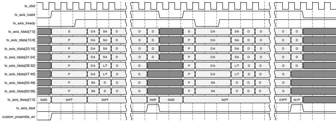
Figure 3-13: Transmission of Custom Preamble in the Non-Continuous Case
