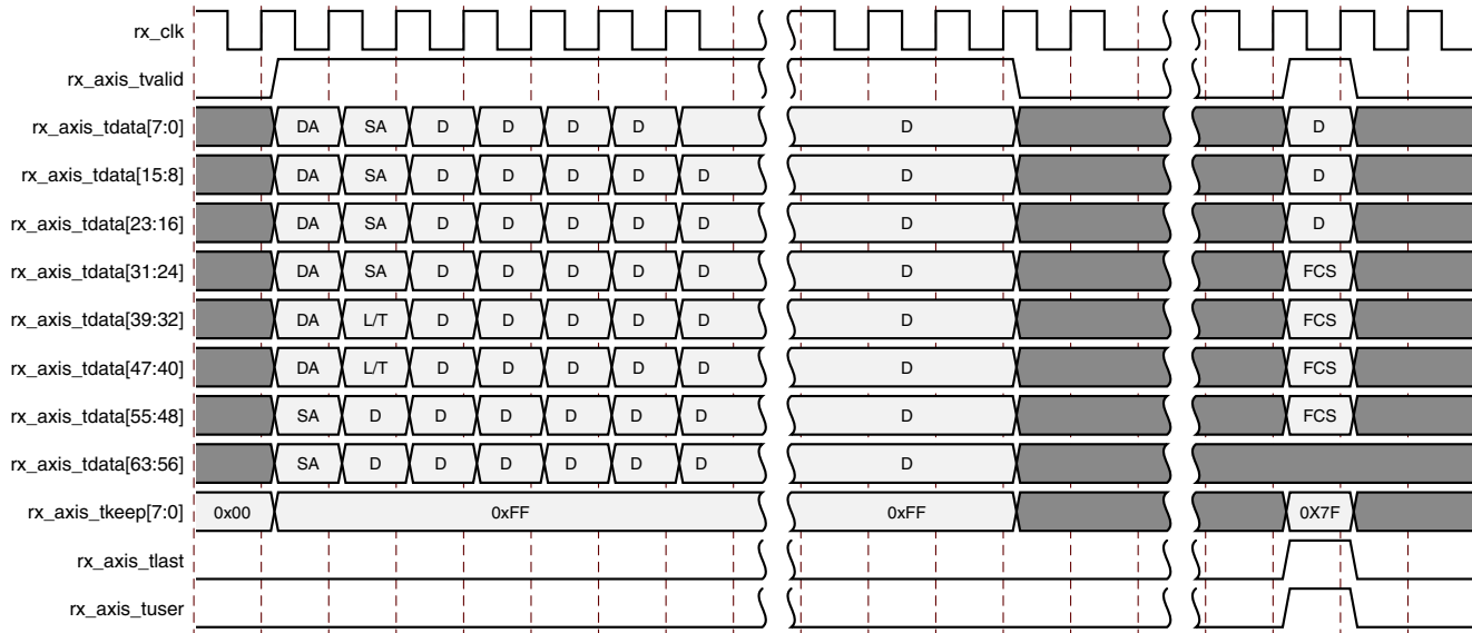
Figure 3-33: Frame Reception with In-Band FCS Passing
