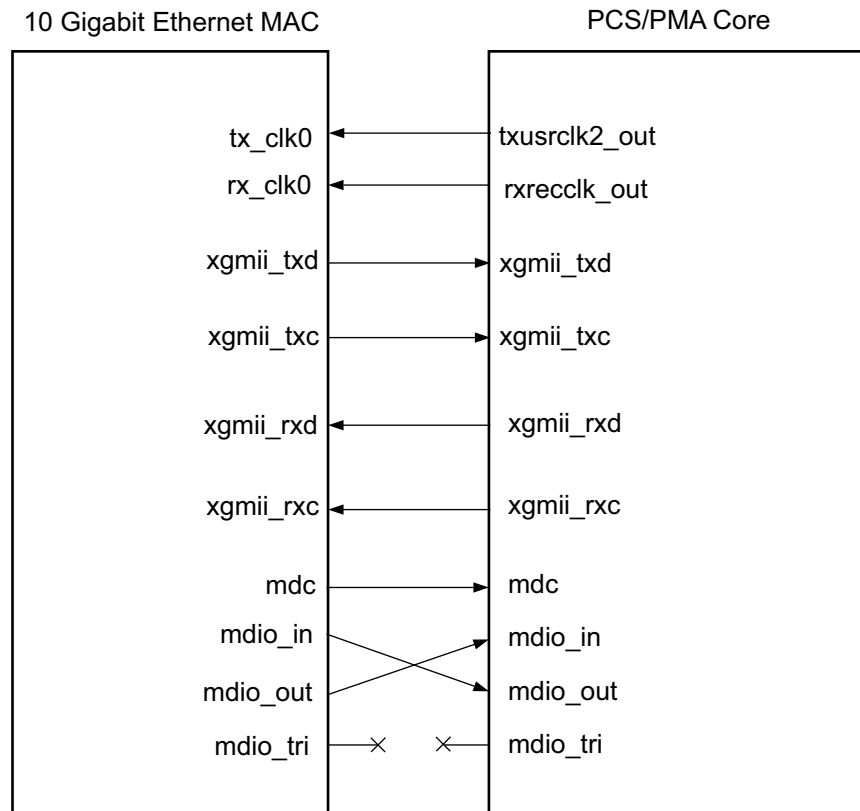
Figure 3-63: 10 Gigabit Ethernet MAC Core with PCS/PMA Core with No RX Elastic Buffer
