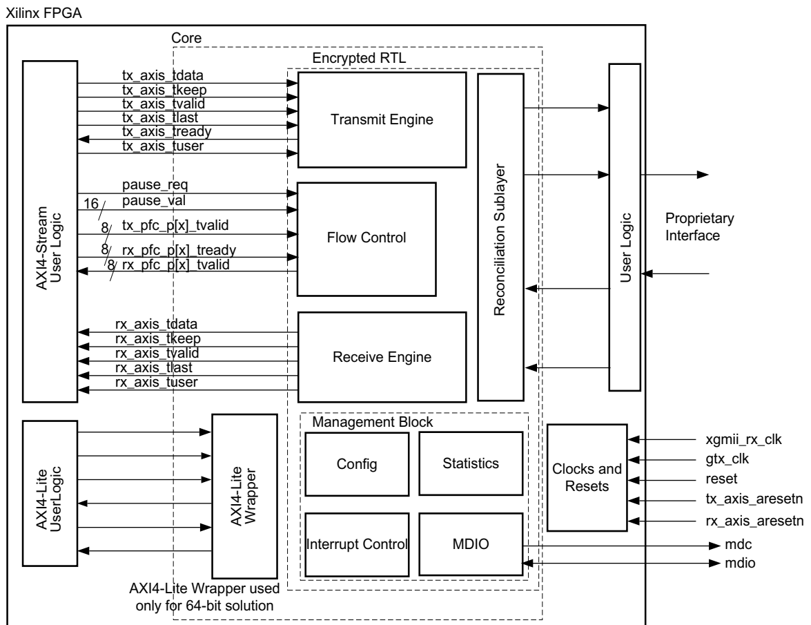
Figure 2-1: 10 Gigabit Ethernet MAC with User Logic on PHY Interface
