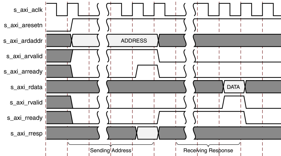
Figure 3-42: Management Register Read Timing
