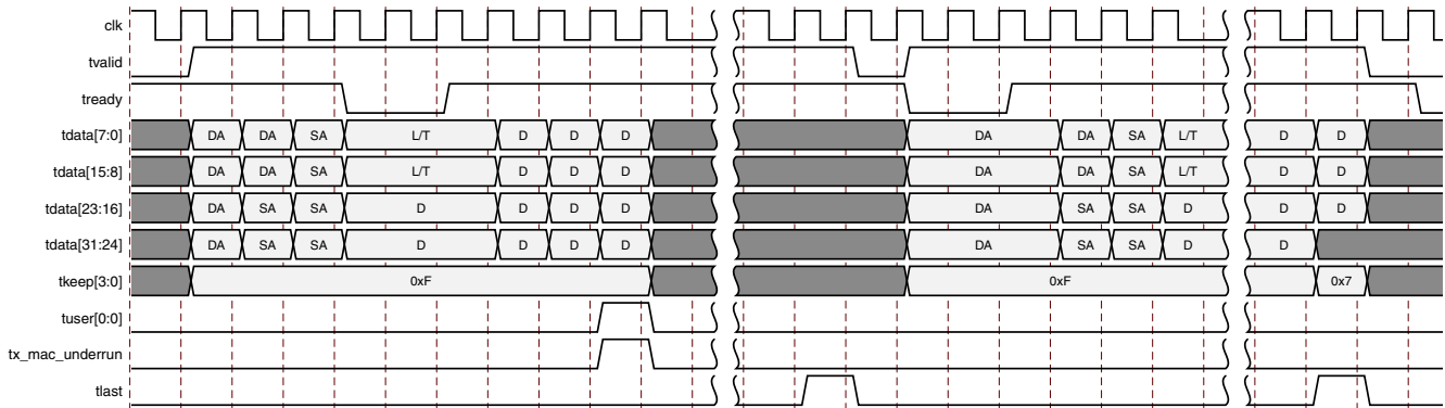
Figure 3-21: Frame Transfer Abort with tx_axis_tuser Asserted
