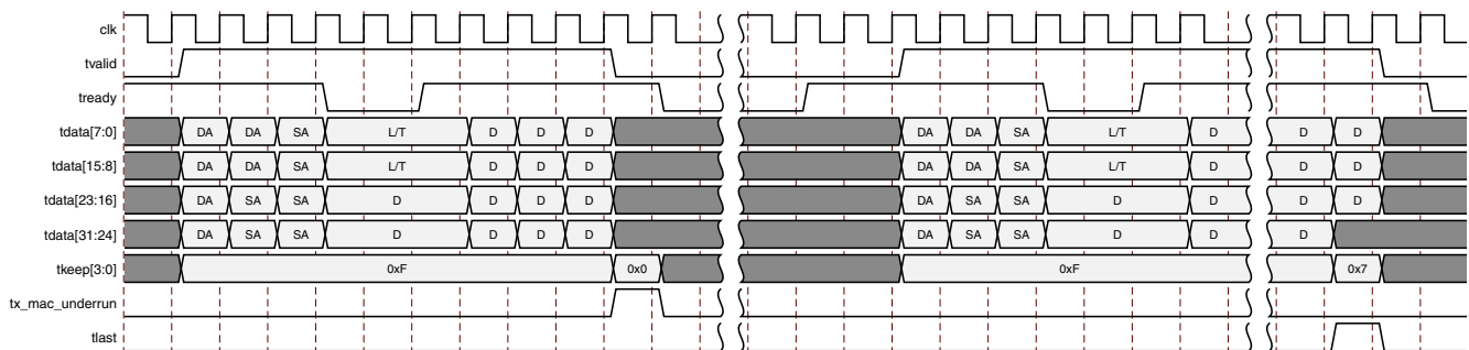
Figure 3-22: Frame Transfer Abort with tx_axis_tvalid Deasserted
