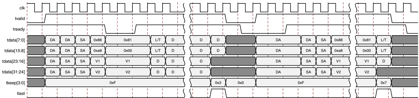
Figure 3-28: Q in Q VLAN Type Tag
