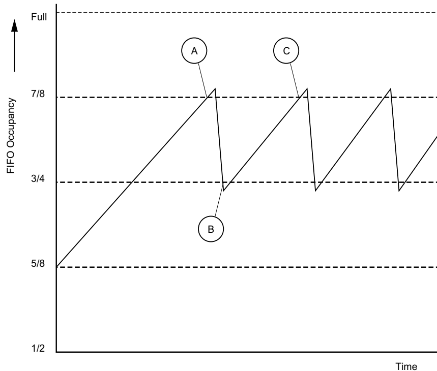
Figure 3-53: Flow Control Implementation Triggered from FIFO Occupancy
