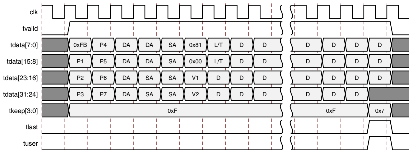
Figure 3-40: Frame Reception with VLAN Tagged Frames
