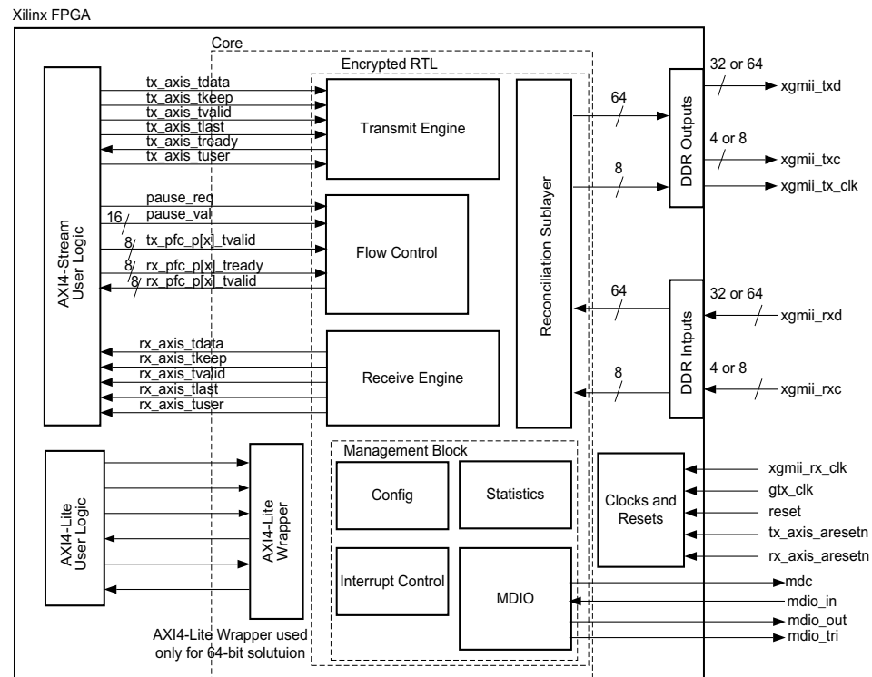
Figure 2-2: 10 Gigabit Ethernet MAC with External XGMII Interface
