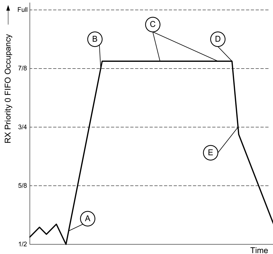
Figure 3-58: Priority Flow Control Implementation Triggered from FIFO Occupancy
