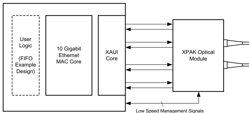
Figure 1-3: 10 Gigabit Ethernet MAC and XAUI Core Using XPAK
