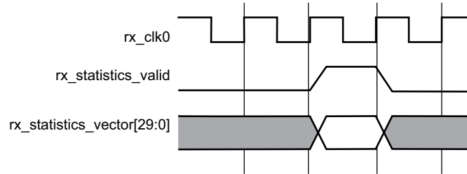
Figure 2-4: Receiver Statistics Output Timing
