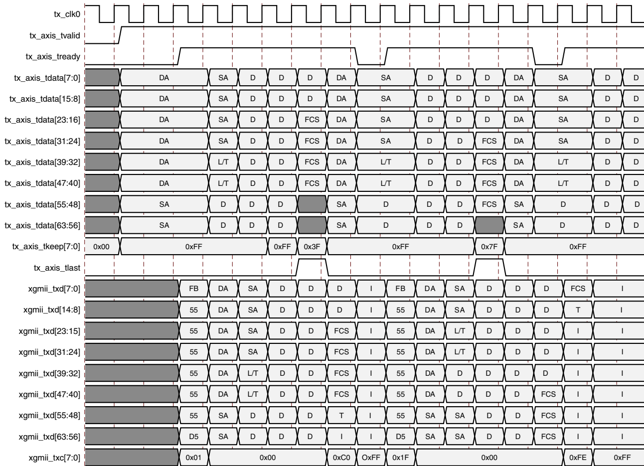
Figure 3-18: Back-to-Back Continuous Transfer on Transmit XGMII Interface
