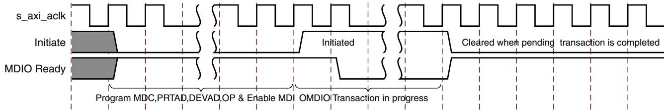
Figure 3-43: MDIO Initiate
