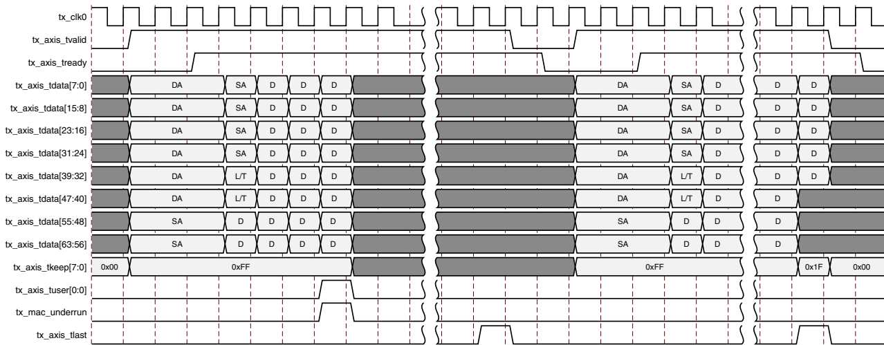
Figure 3-10: Frame Transfer Abort with tx_axis_tuser Asserted
