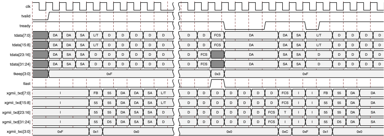
Figure 3-30: Back-to-Back Continuous Transfer on Transmit XGMII Interface
