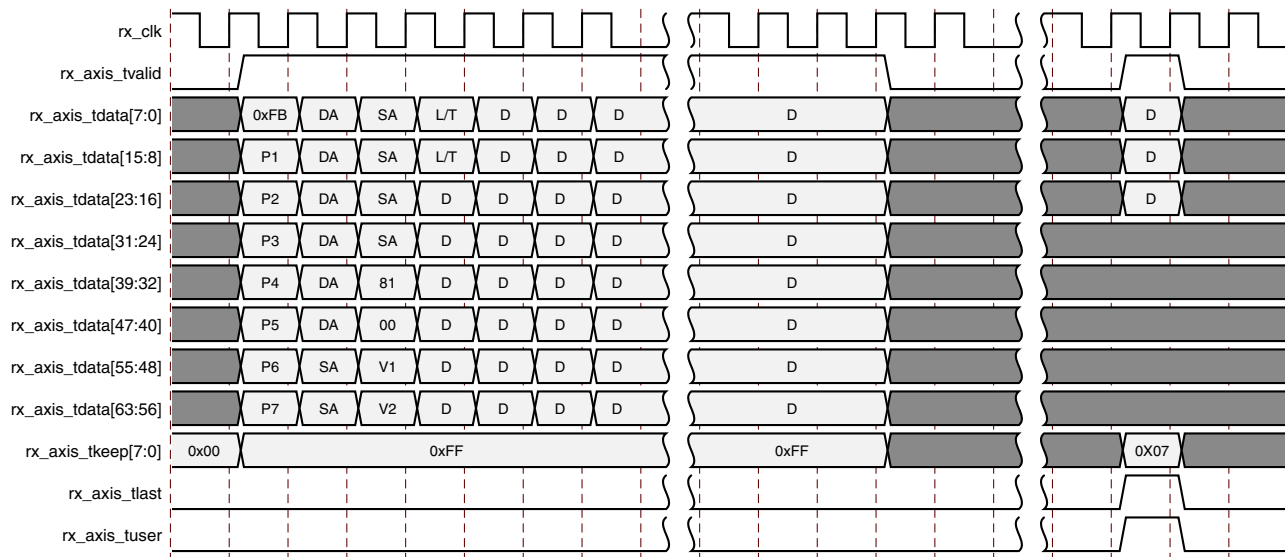
Figure 3-35: Frame Reception with VLAN Tagged Frames
