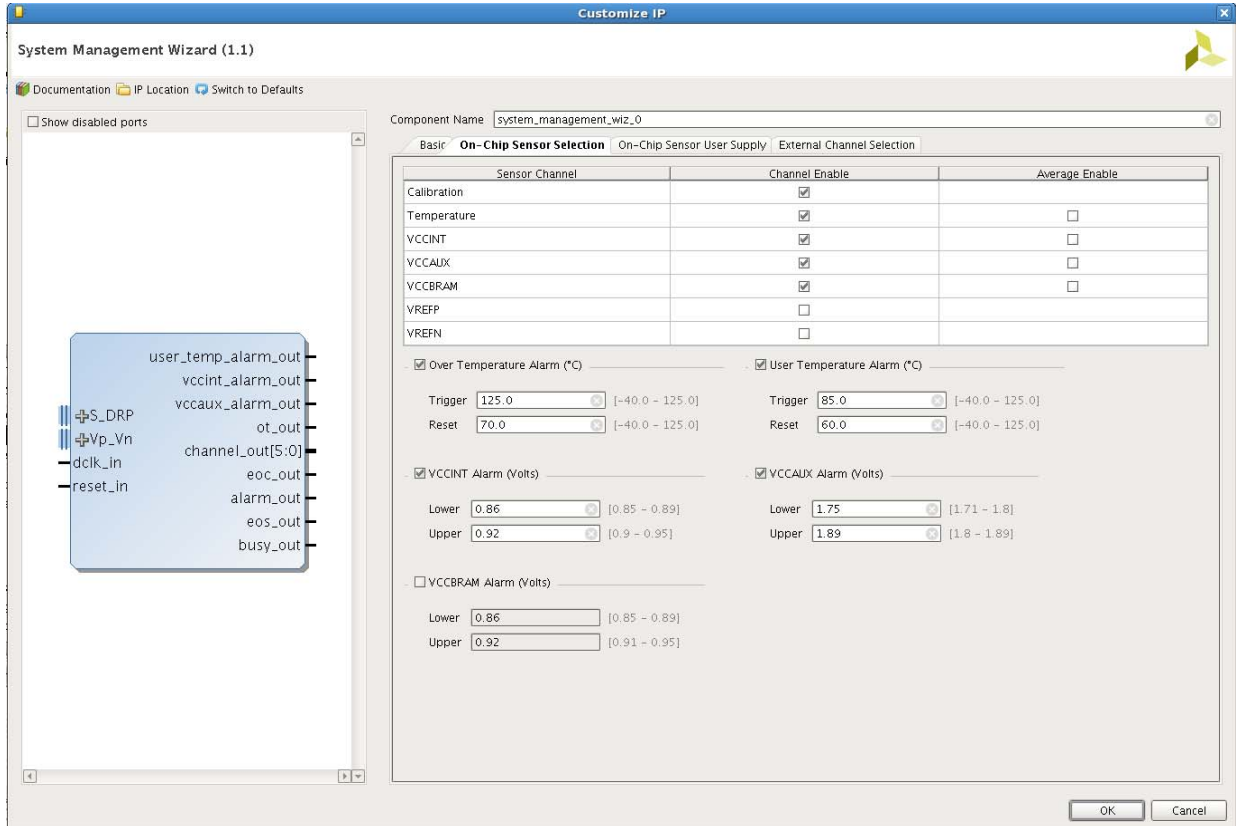
Figure 4-8: On-Chip Sensor Selection and Alarms for Channel Sequencer
