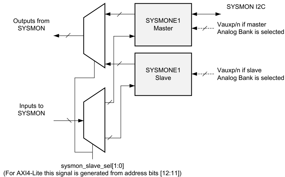
Figure 2-10: Switching Between Two SYSMONE1s
