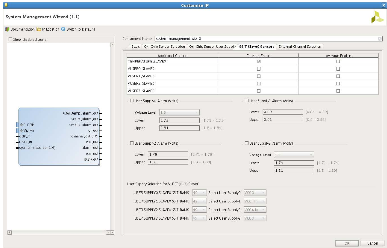
Figure 4-10: SSIT Slave0/Slave1 Sensors Tab
