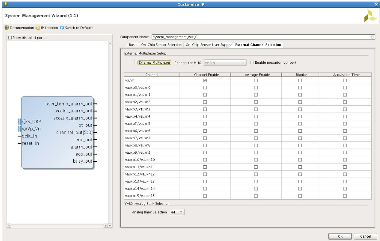
Figure 4-11: External Channel Selection Tab for Channel Sequencer
