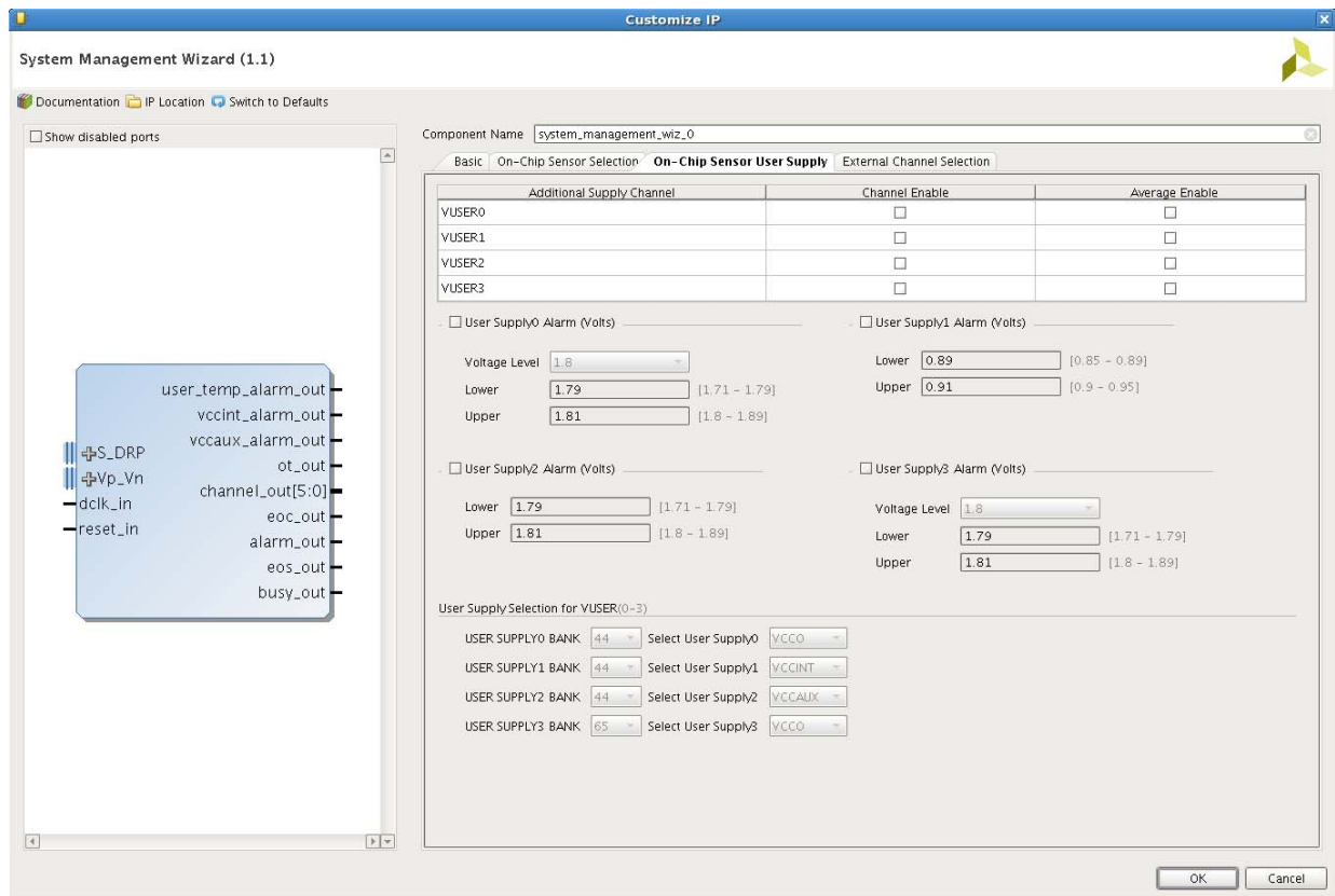
Figure 4-9: On-Chip Sensor User Supply and Alarms Tab for Channel Sequencer
