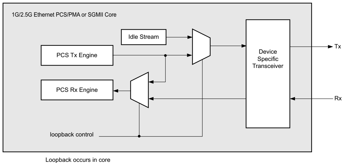
Figure 3-63: Loopback Implementation When Using the Core with Device-Specific Transceivers
