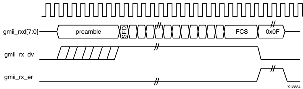
Figure 3-32: GMII Normal Frame Reception with Carrier Extension
