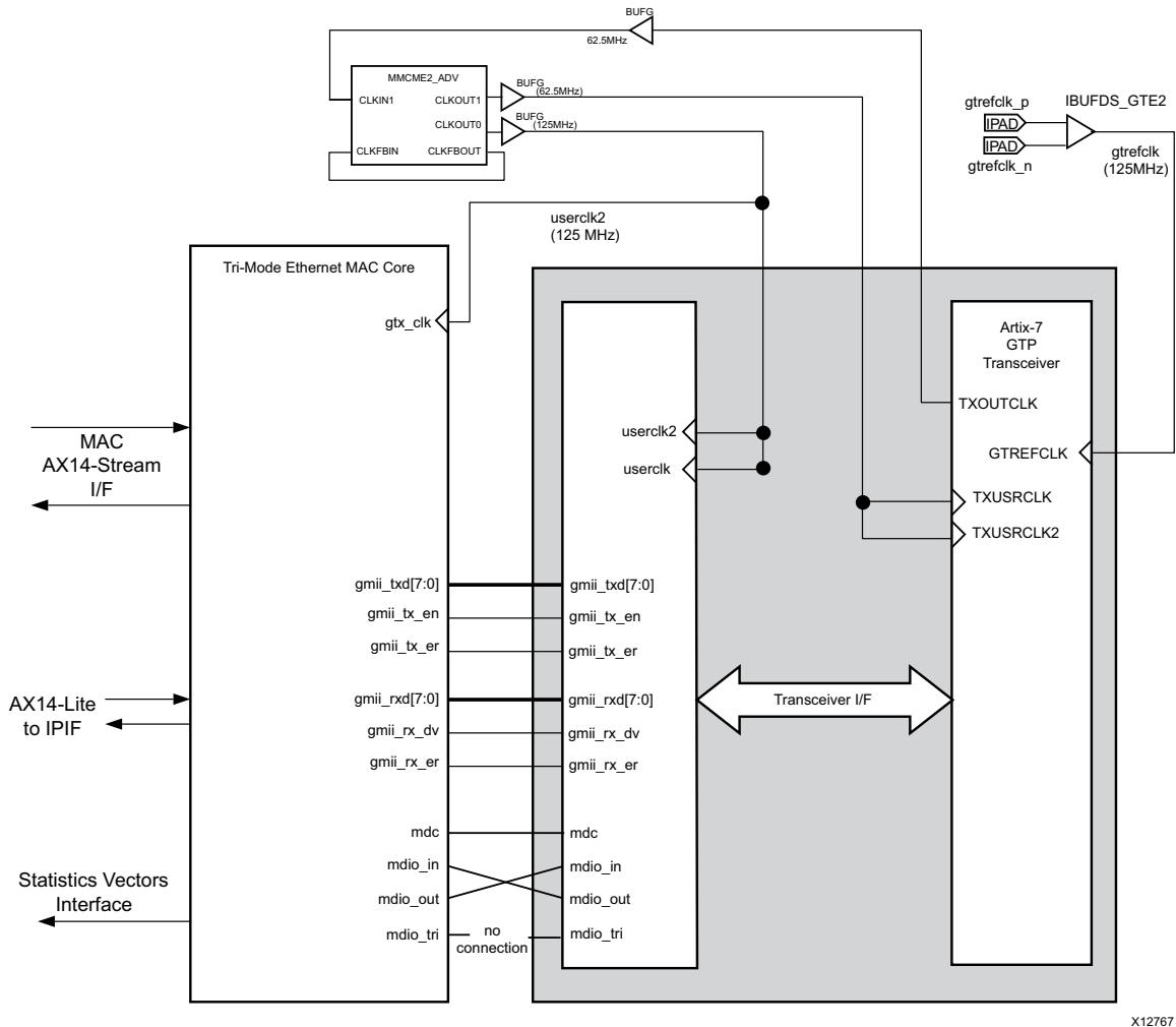
Figure 3-54: Core Using Artix-7 Transceiver Connected to the TEMAC Core
