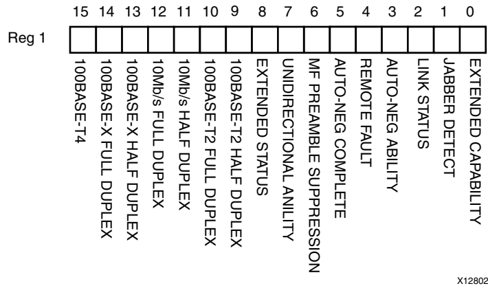
Figure 2-25: MDIO Register 1: SGMII Status
