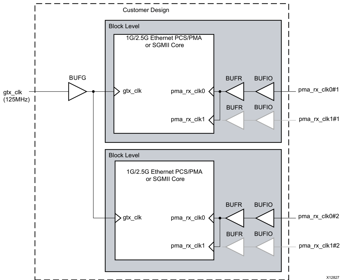
Figure 3-28: Clock Management, Multiple Core Instances with the TBI
