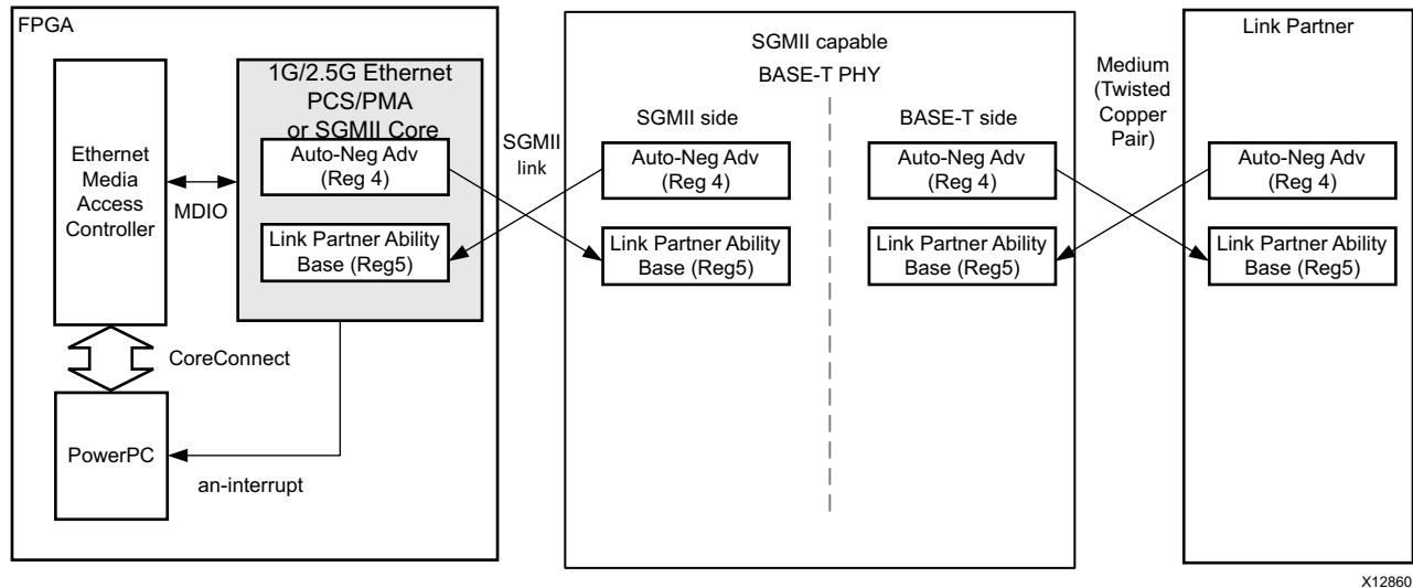
Figure 3-49: SGMII Auto-Negotiation in MAC Mode
