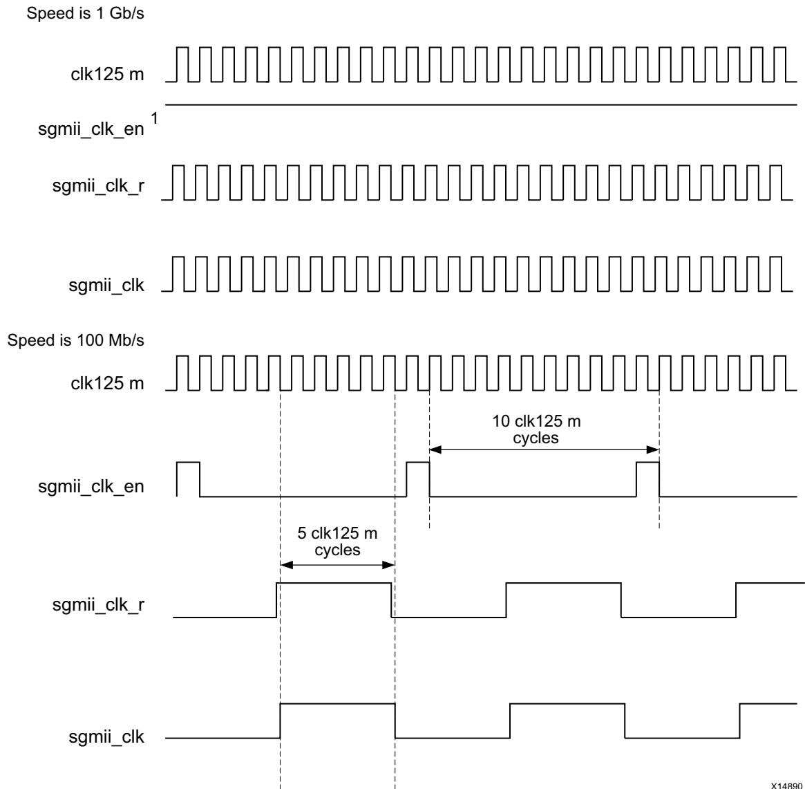
Figure 3-47: Clock Enable Signal for the Clock Generation Module
