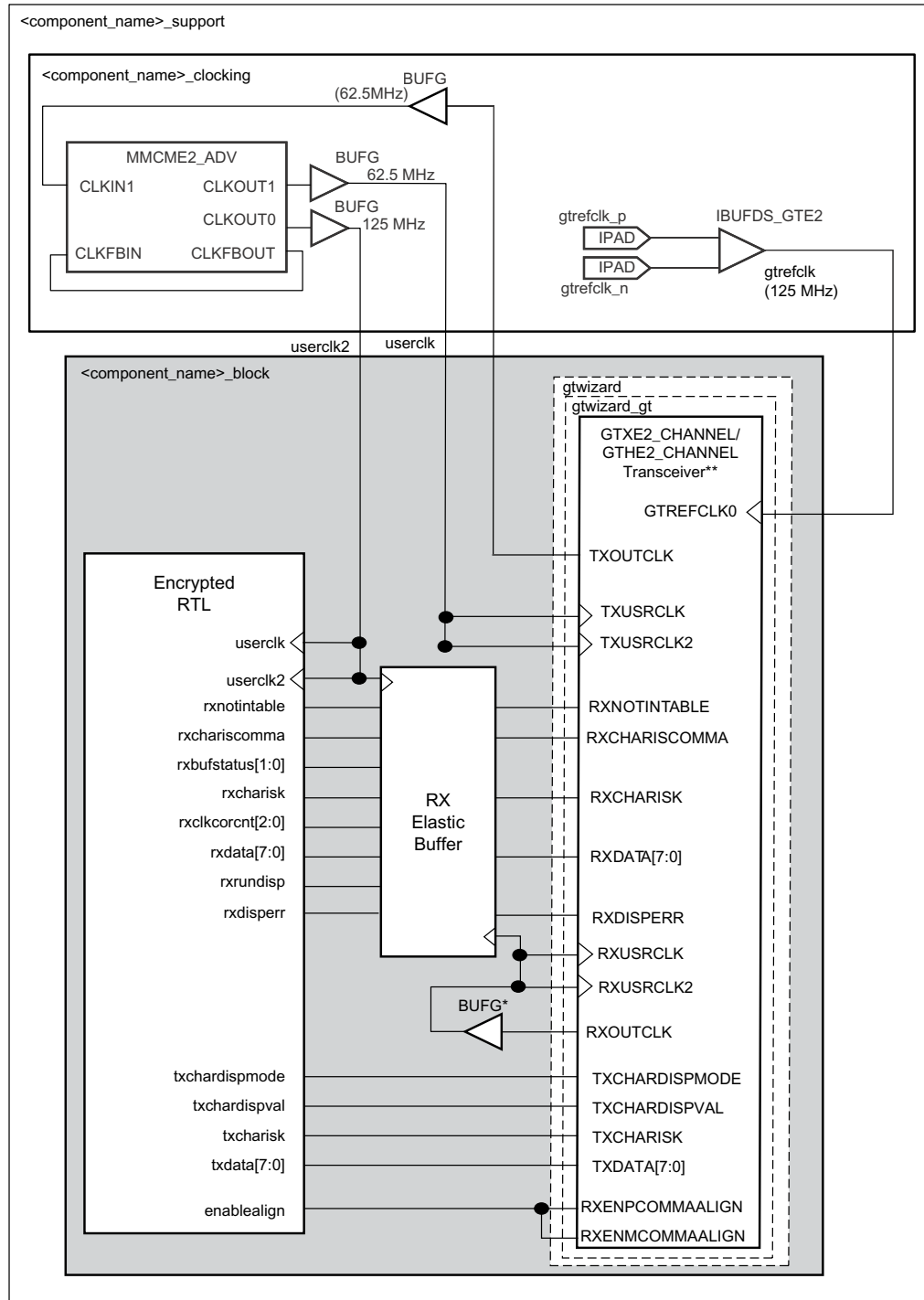
Figure 3-13: 1G SGMII Transceiver Connections (Virtex-7, Kintex-7, Zynq-7000)
