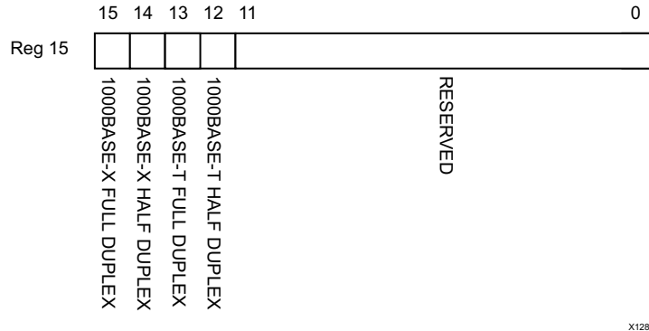
Figure 2-39: MDIO Register 15: SGMII Extended Status
