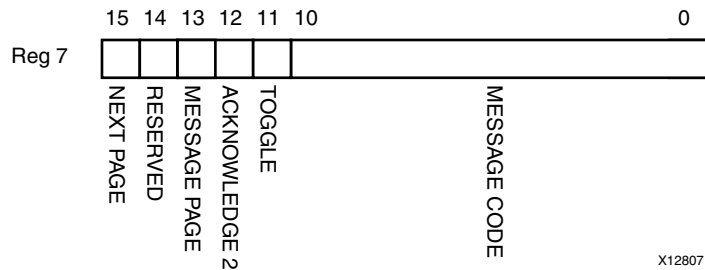
Figure 2-31: MDIO Register 7: SGMII Auto-Negotiation Next Page Transmit
