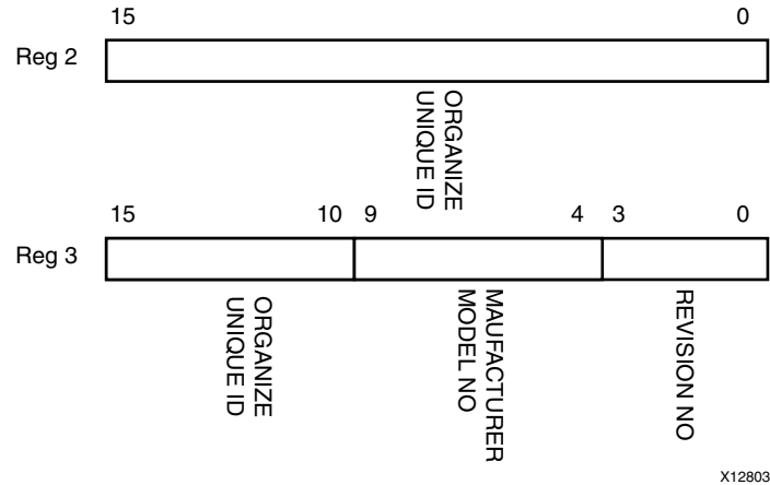
Figure 2-22: MDIO Registers 2 and 3: PHY Identifier
