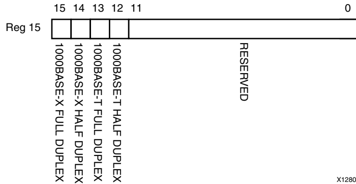
Figure 2-33: MDIO Register 15: SGMII Extended Status
