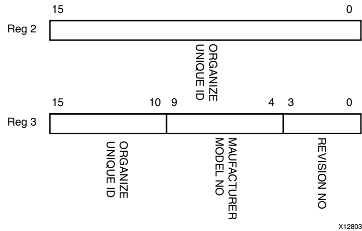
Figure 2-37: MDIO Registers 2 and 3: PHY Identifier
