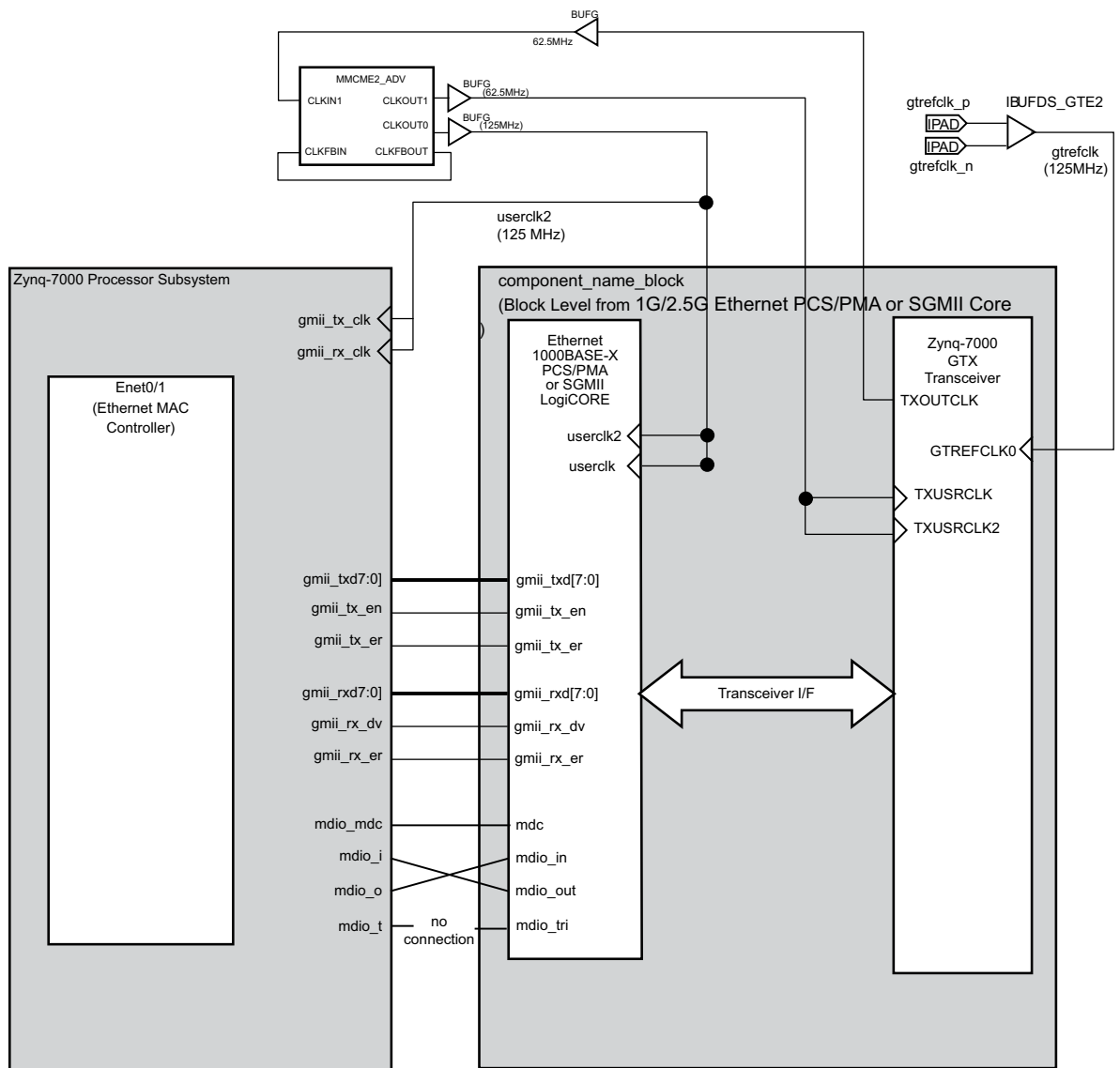
Figure 3-59: ENET0/1 Extended to Include 1000BASE-X PCS/PMA Using Device Transceiver
