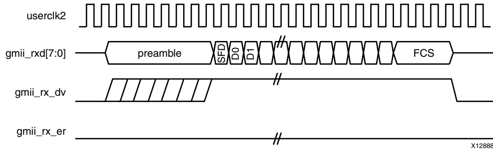
Figure 3-36: GMII Frame Transmission at 1/2.5 Gb/s
