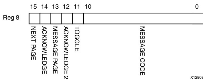
Figure 2-32: MDIO Register 8: SGMII Next Page Receive
