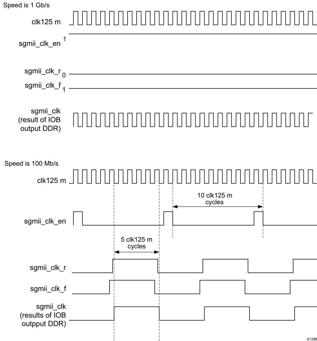
Figure 3-46: Clock Generator Output Clocks and Clock Enable
