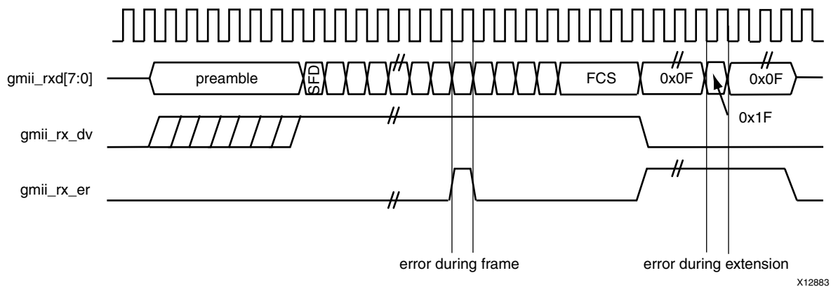
Figure 3-33: GMII Frame Reception with Errors
