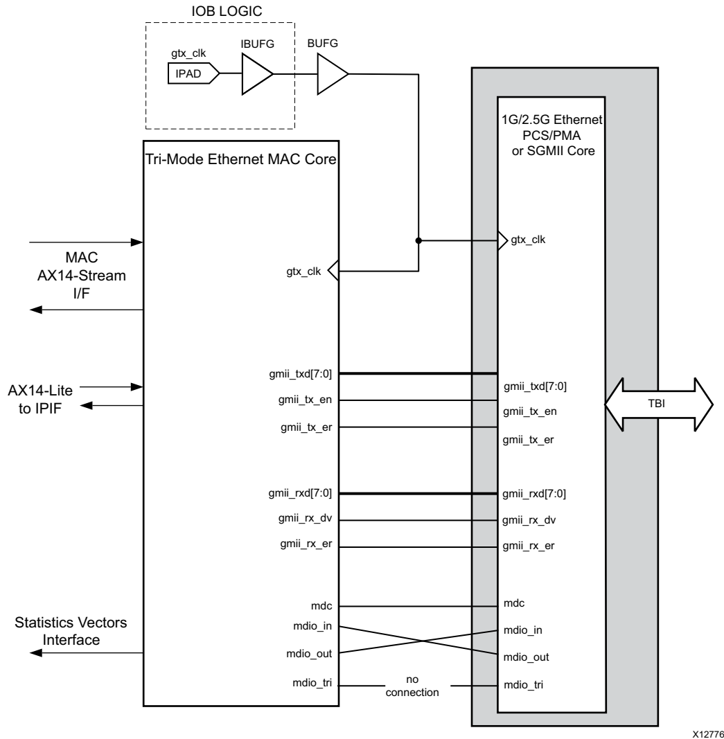
Figure 3-52: Core with TBI Connected to TEMAC Core
