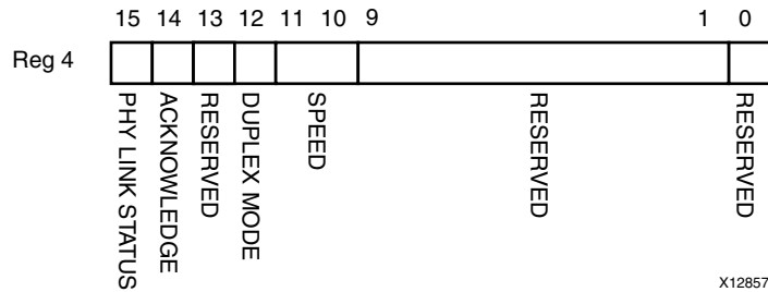
Figure 2-28: MDIO Register 4: SGMII Auto-Negotiation Advertisement
