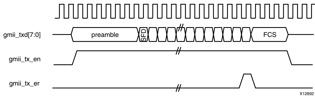
Figure 3-30: GMII Error Propagation Within a Frame
