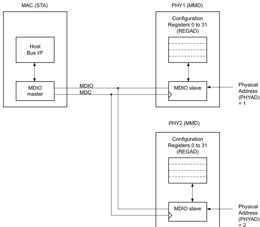
Figure 2-6: A Typical MDIO-Managed System
