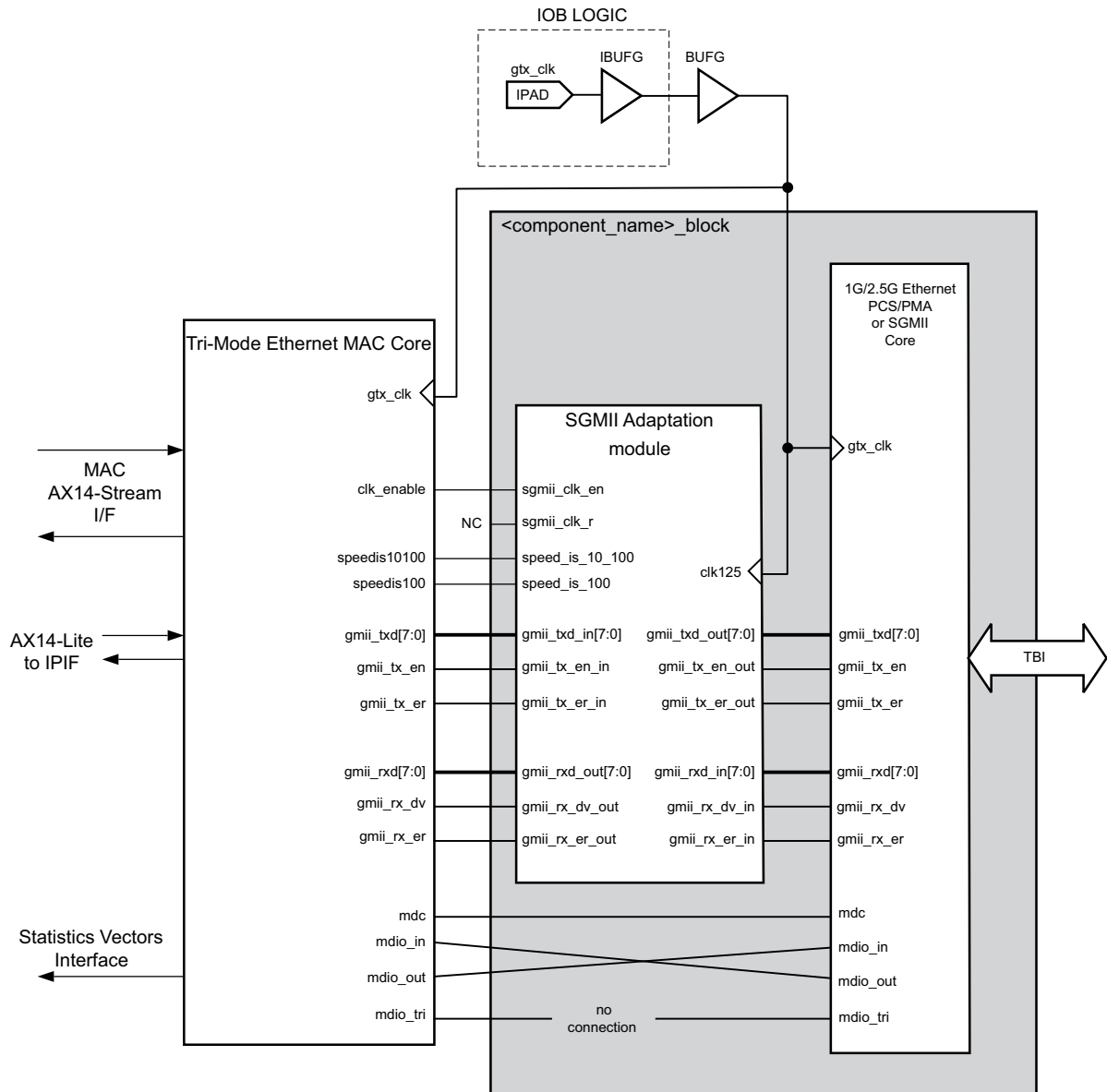
Figure 3-55: Core Using TBI Connected to the TEMAC Core
