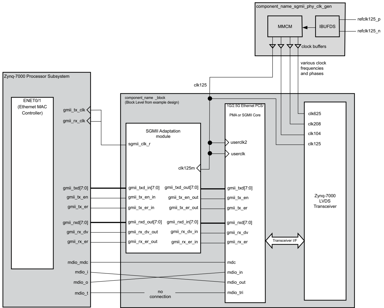
Figure 3-61: Zynq-7000 Device ENET0/1 Extended to Include SGMII Using Zynq-7000 Device Synchronous LVDS
