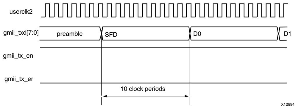
Figure 3-37: GMII Data Transmission at 100 Mb/s
