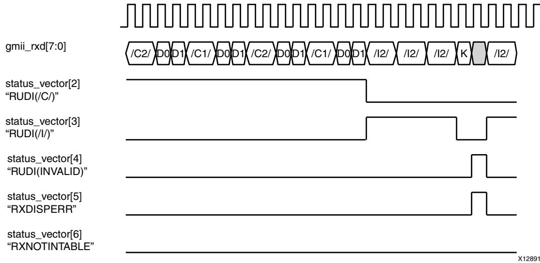
Figure 3-35: status_vector[4:2] timing
