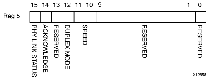
Figure 2-29: MDIO Register 5: SGMII Auto-Negotiation Link Partner Ability
