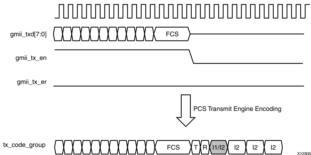
Figure C-5: 100BASE-X Transmit State Machine Operation (Even Case)
