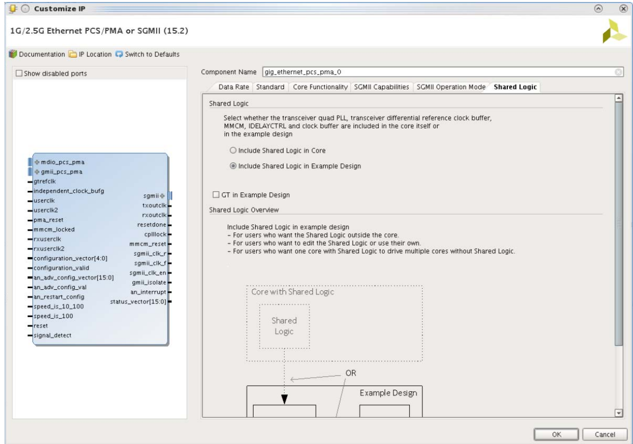
Figure 4-8: Shared Logic Placement Options
