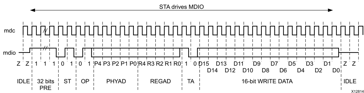
Figure 2-7: MDIO Write Transaction
