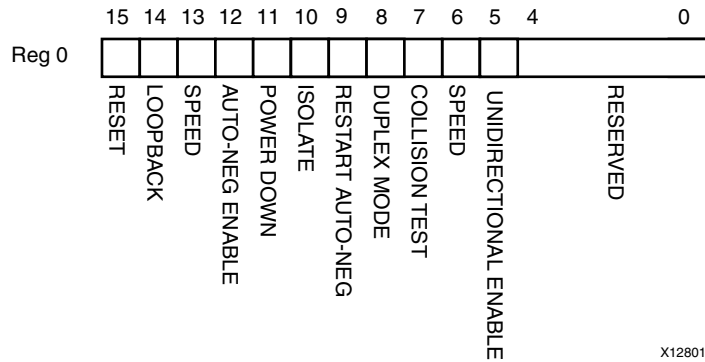
Figure 2-20: MDIO Register 0: Control Register
