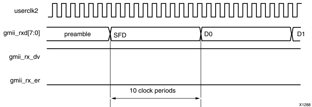
Figure 3-39: GMII Data Reception at 100 Mb/s
