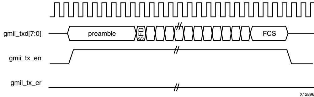
Figure 3-29: GMII Normal Frame Transmission
