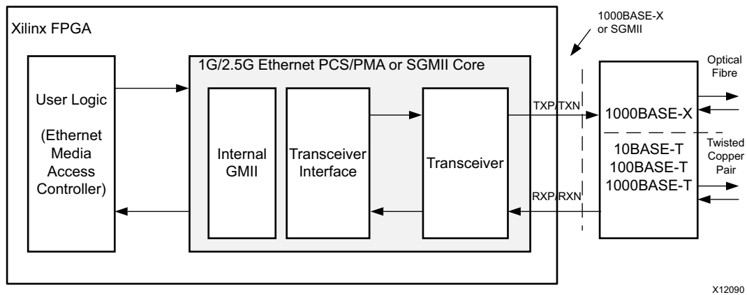
Figure 3-51: Typical Application for Dynamic Switching
