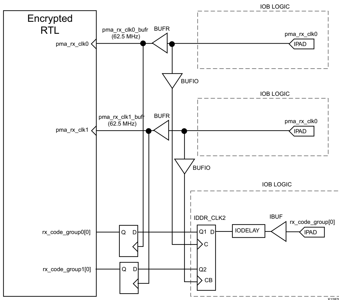
Figure 3-27: Alternate TBI Receiver Logic - Kintex-7 Devices
