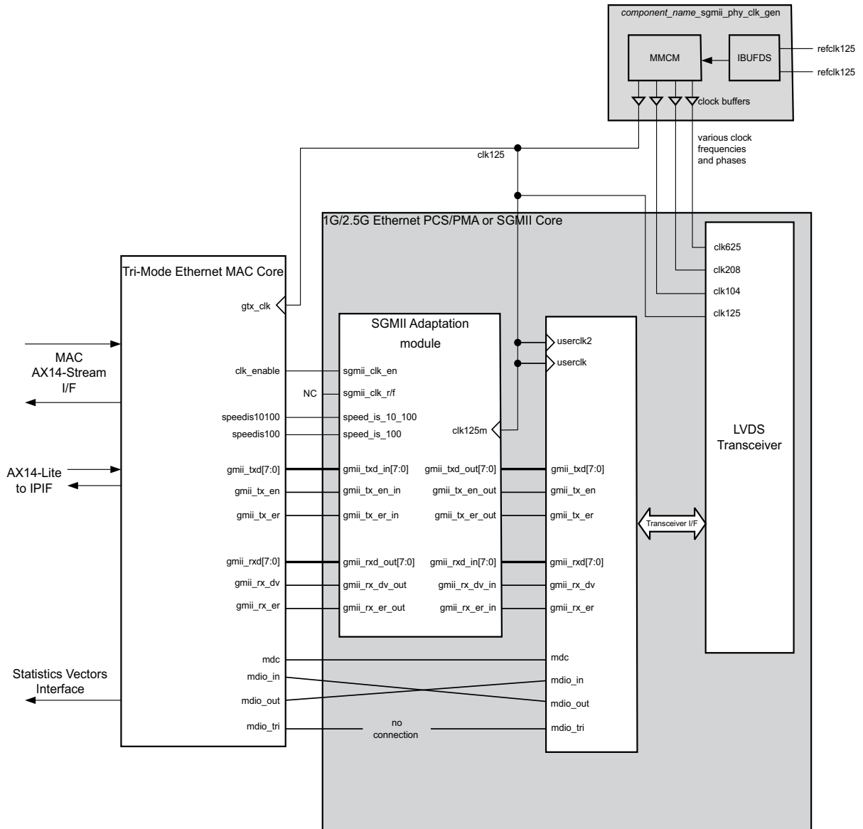
Figure 3-58: Core Using SGMII over LVDS Connected to the TEMAC Core
