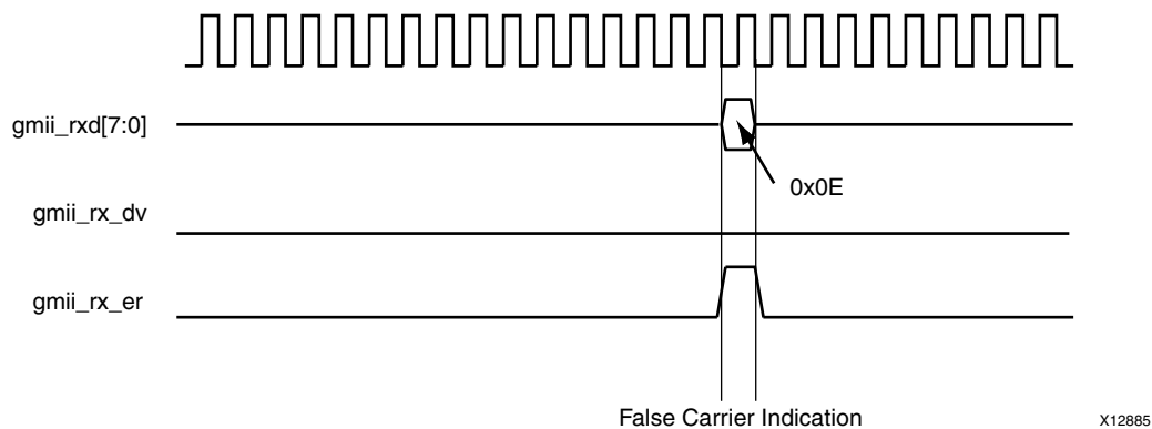
Figure 3-34: False Carrier Indication
