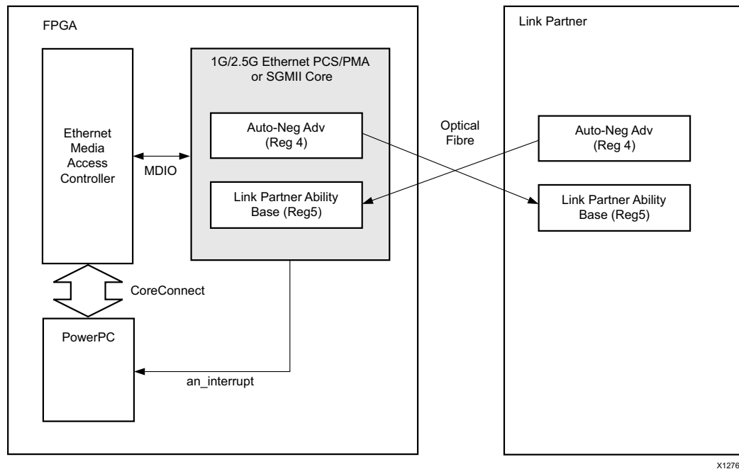
Figure 3-48: 1000BASE-X Auto-Negotiation Overview
