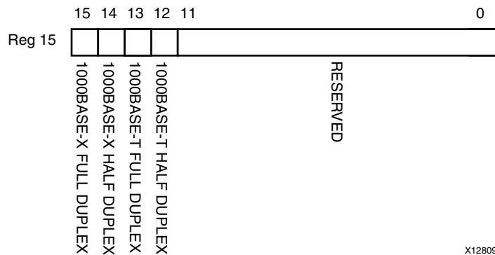
Figure 2-23: MDIO Register 15: Extended Status
