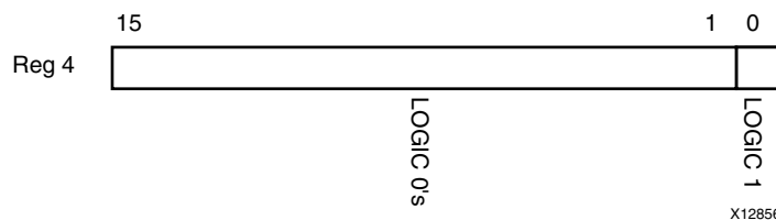
Figure 2-38: MDIO Register 4: SGMII Auto-Negotiation Advertisement
