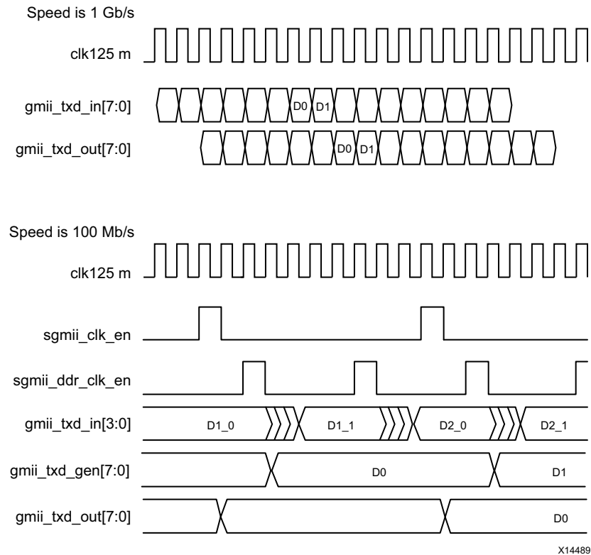
Figure 3-43: Transmitter Rate Adaptation Module Data Sampling
