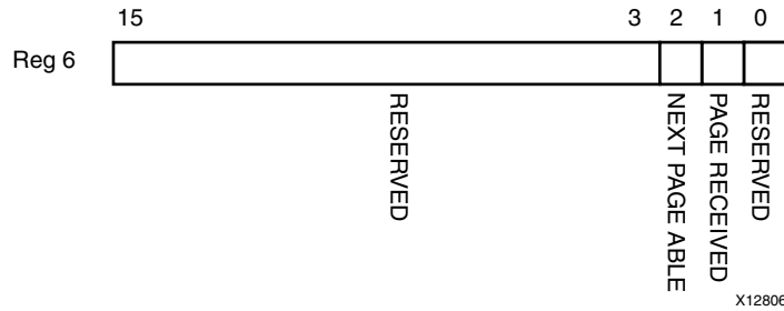
Figure 2-30: MDIO Register 6: SGMII Auto-Negotiation Expansion
