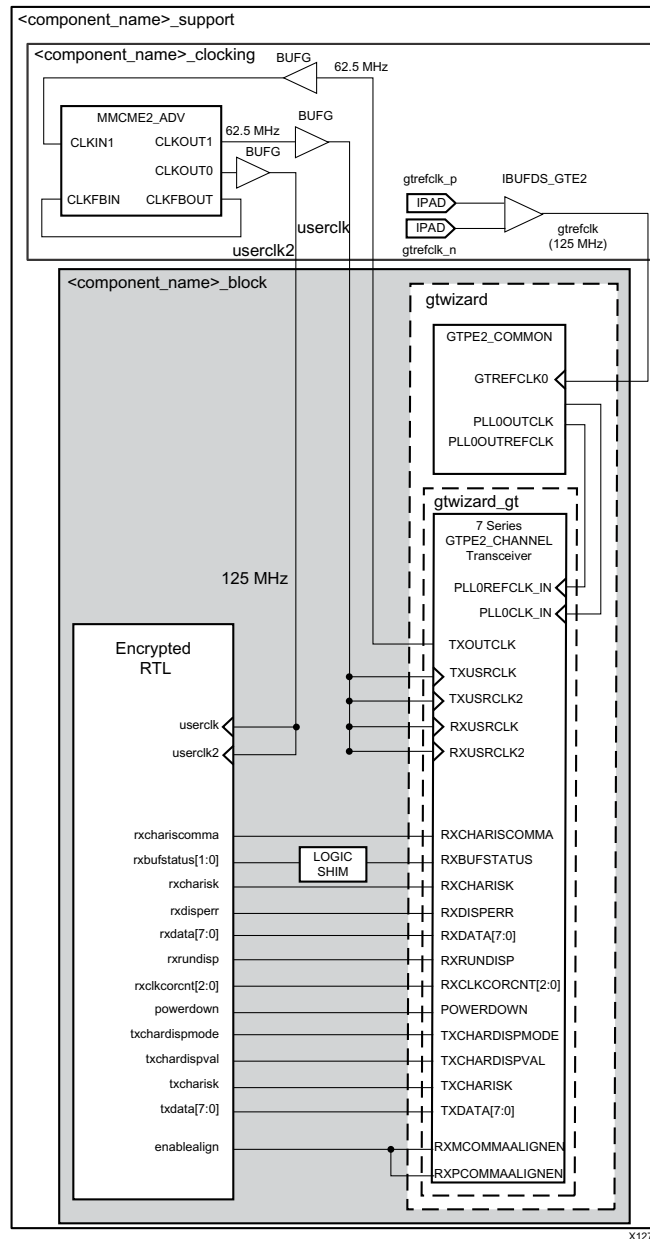
Figure 3-7: 100BASE-X Transceiver Connections (Artix-7)
