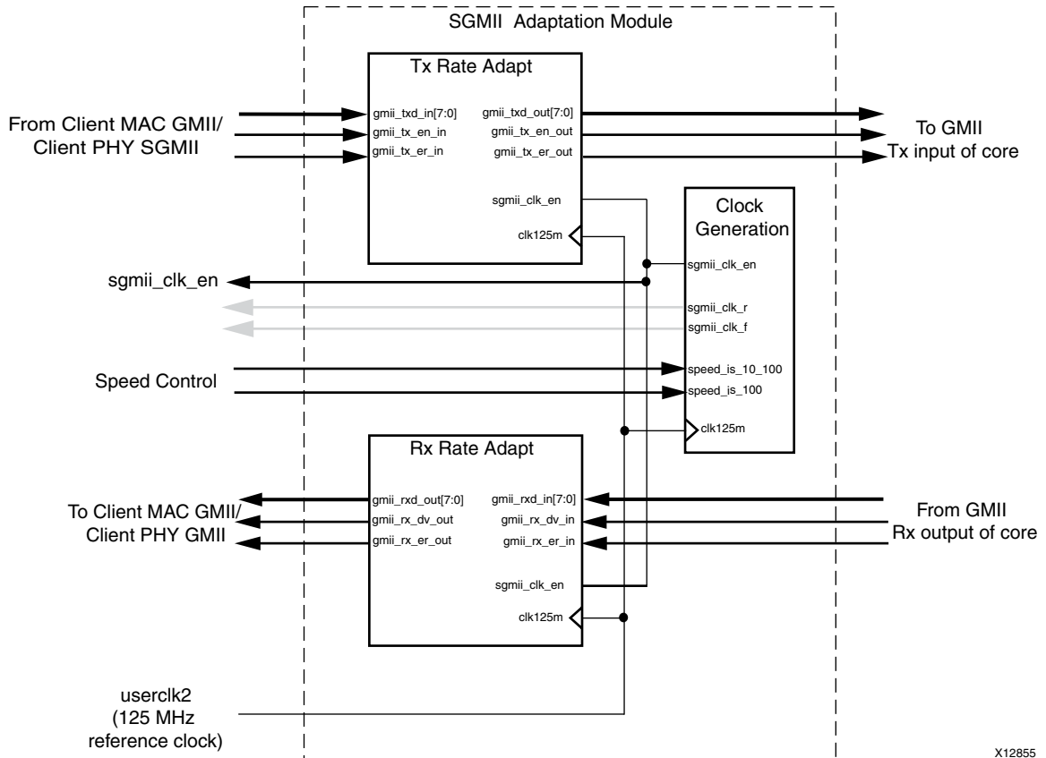
Figure 3-41: SGMII Adaptation Module
