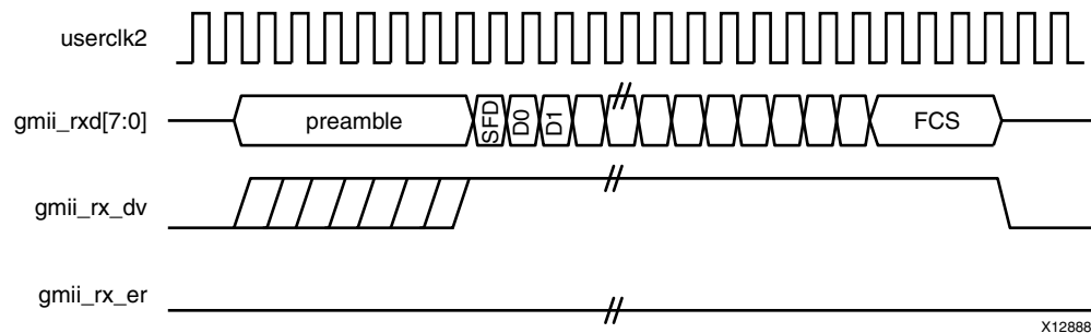
Figure 3-38: GMII Frame Reception at 1/2.5 Gb/s
