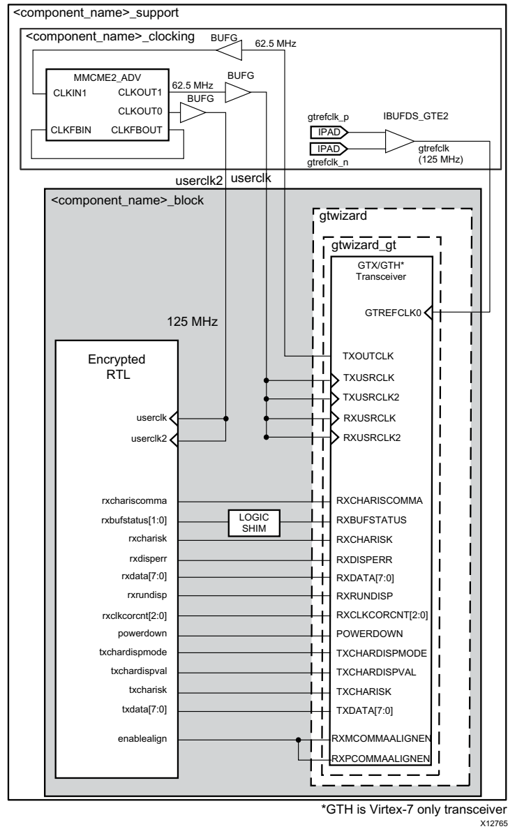
Figure 3-6: 100BASE-X Transceiver Connections (Virtex-7, Kintex-7, Zynq-7000)
