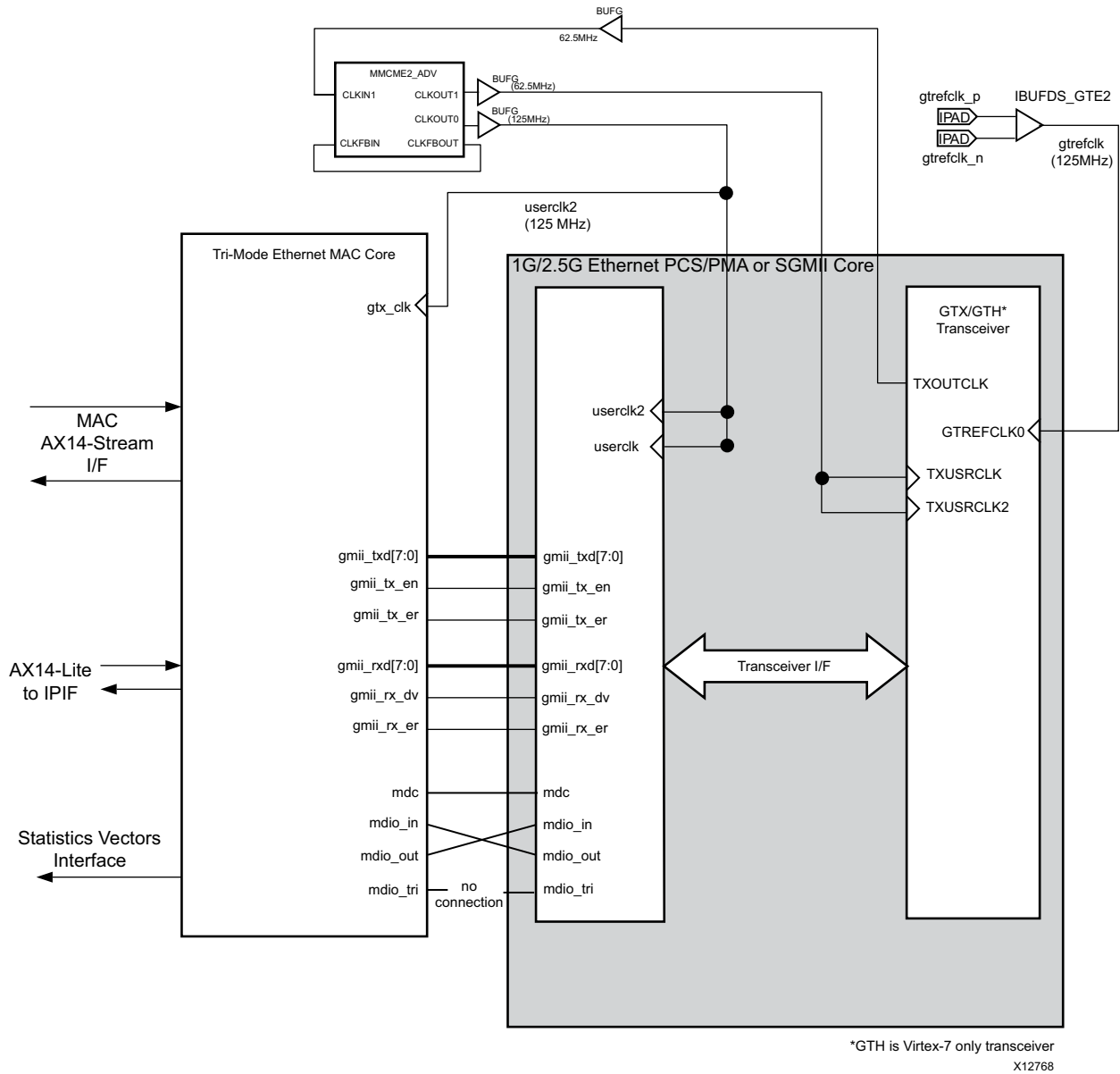
Figure 3-53: Core Using GTX/GTH Transceivers Connected to the TEMAC Core
