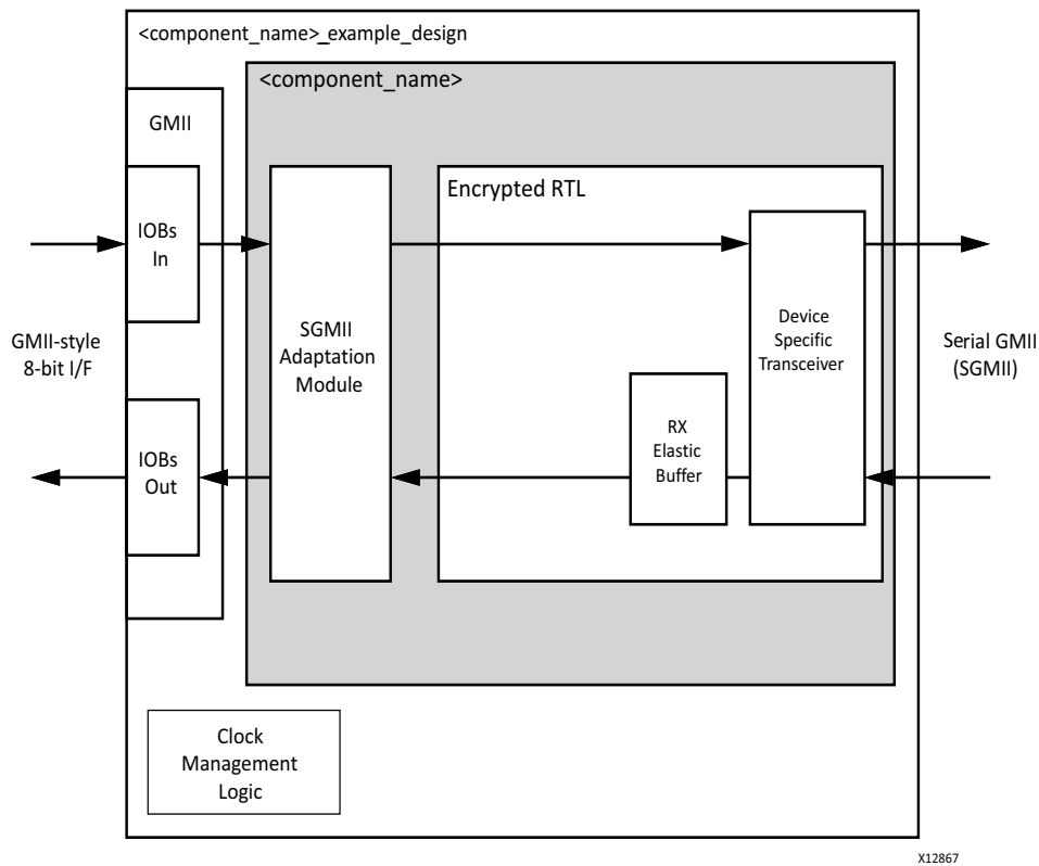
Figure 3-40: Block Level Diagram of an SGMII Example Design
