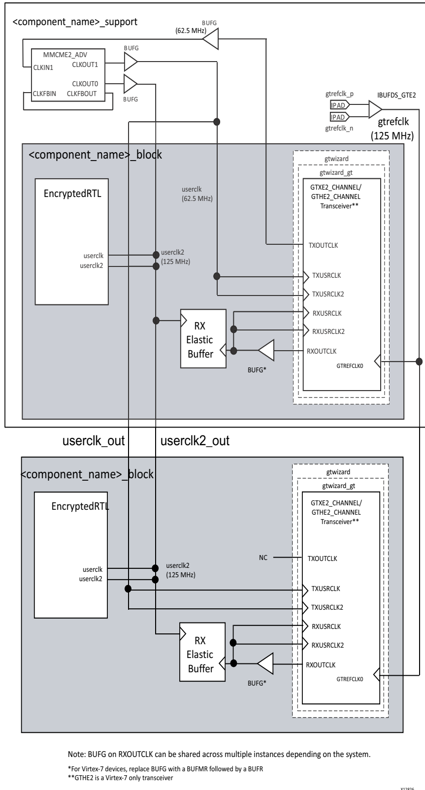
Figure 3-16: Clock Management with Multiple Core Instances for SGMII (Virtex-7, Kintex-7, Zynq-7000)
