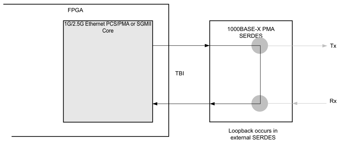
Figure 3-62: Loopback Implementation Using the TBI
