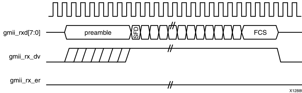
Figure 3-31: GMII Normal Frame Reception
