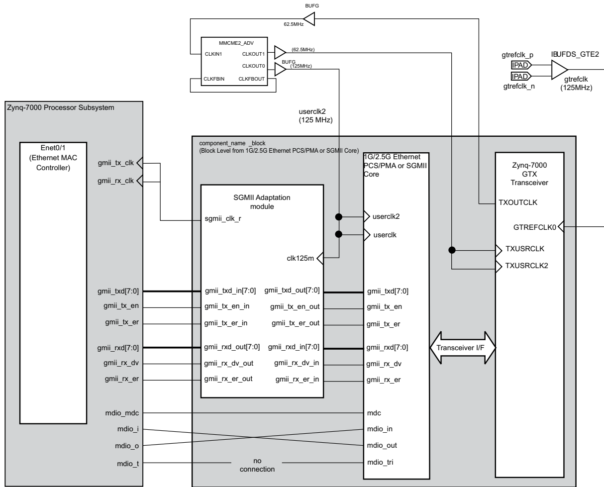
Figure 3-60: Zynq-7000 Device ENET0/1 Extended to Include SGMII Using GTX Transceiver
