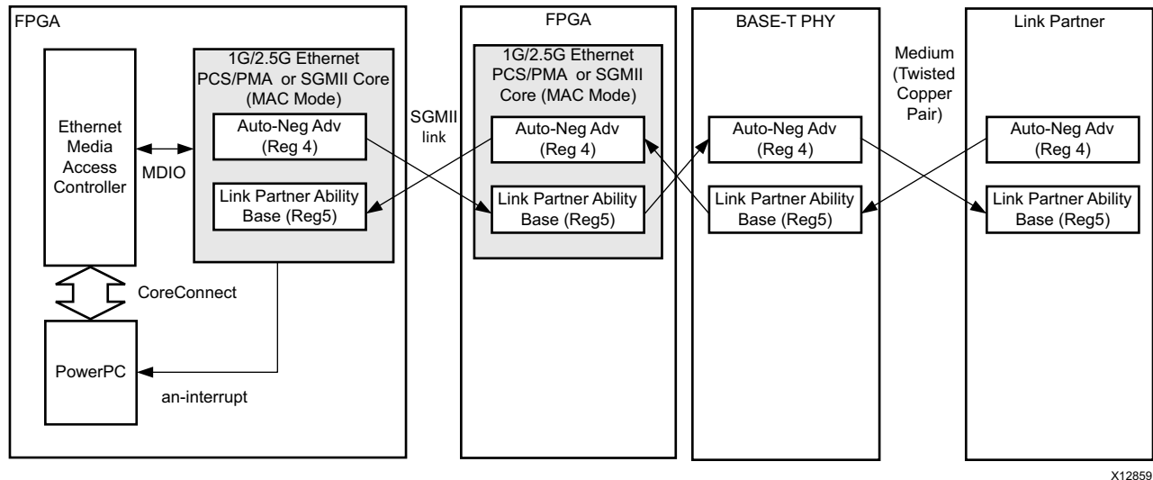
Figure 3-50: SGMII Auto-Negotiation
