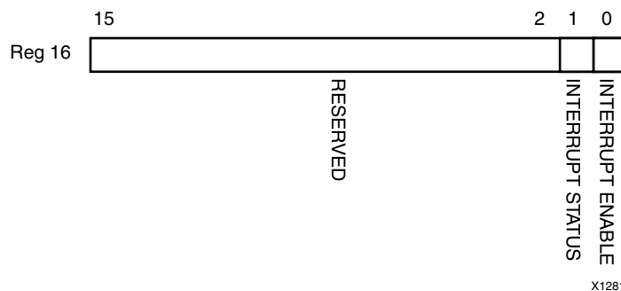
Figure 2-34: MDIO Register 16: SGMII Auto-Negotiation Interrupt Control
