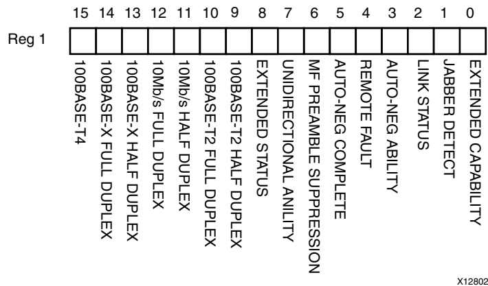
Figure 2-36: MDIO Register 1: SGMII Status
