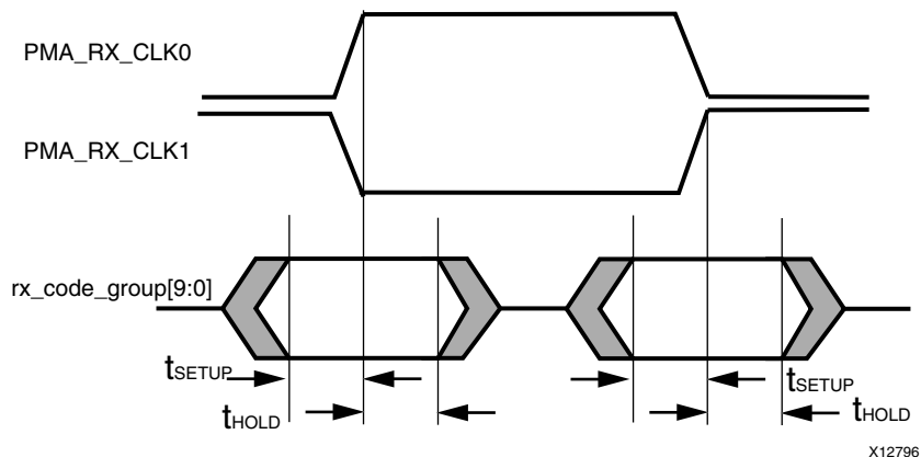
Figure 3-25: Input TBI timing
