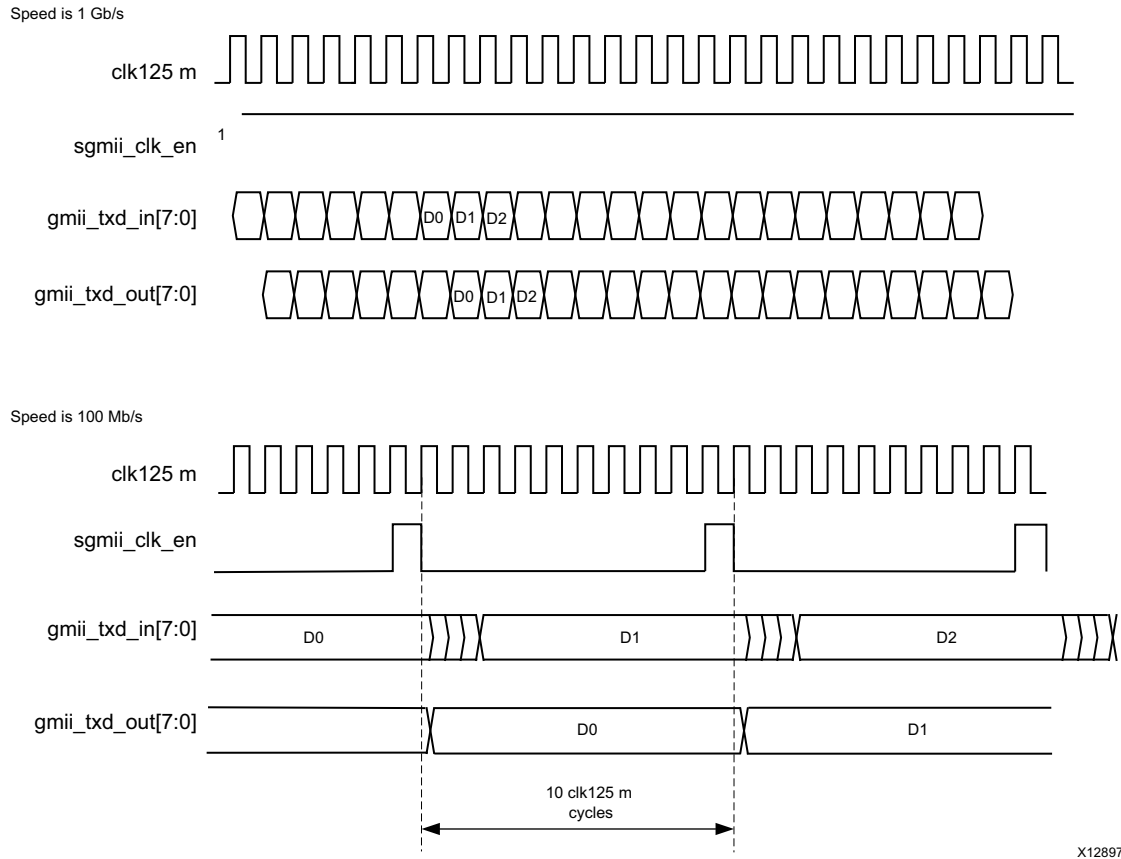
Figure 3-42: Transmitter Rate Adaptation Module Data Sampling
