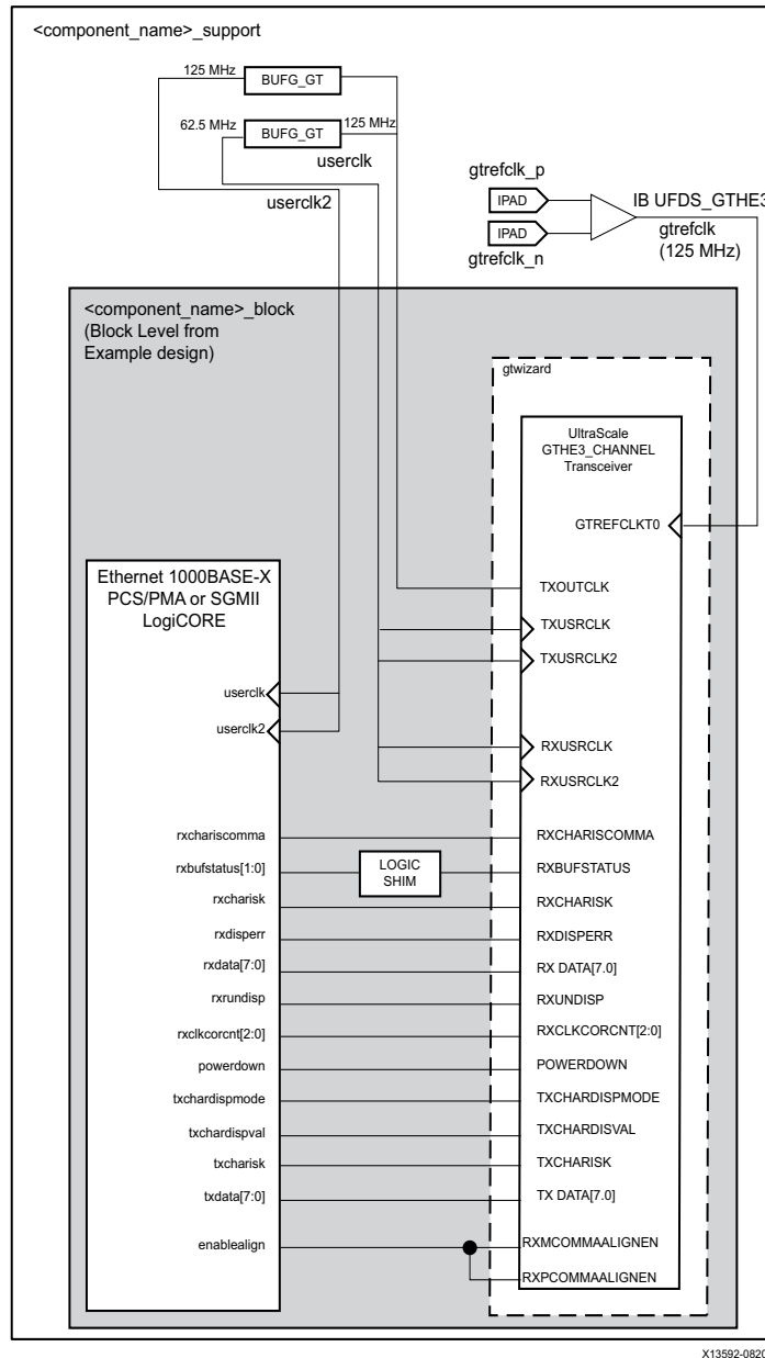
Figure 3-8: 1000BASE-X Transceiver Connections (UltraScale Architecture)
