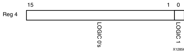
Figure 2-27: MDIO Register 4: SGMII Auto-Negotiation Advertisement
