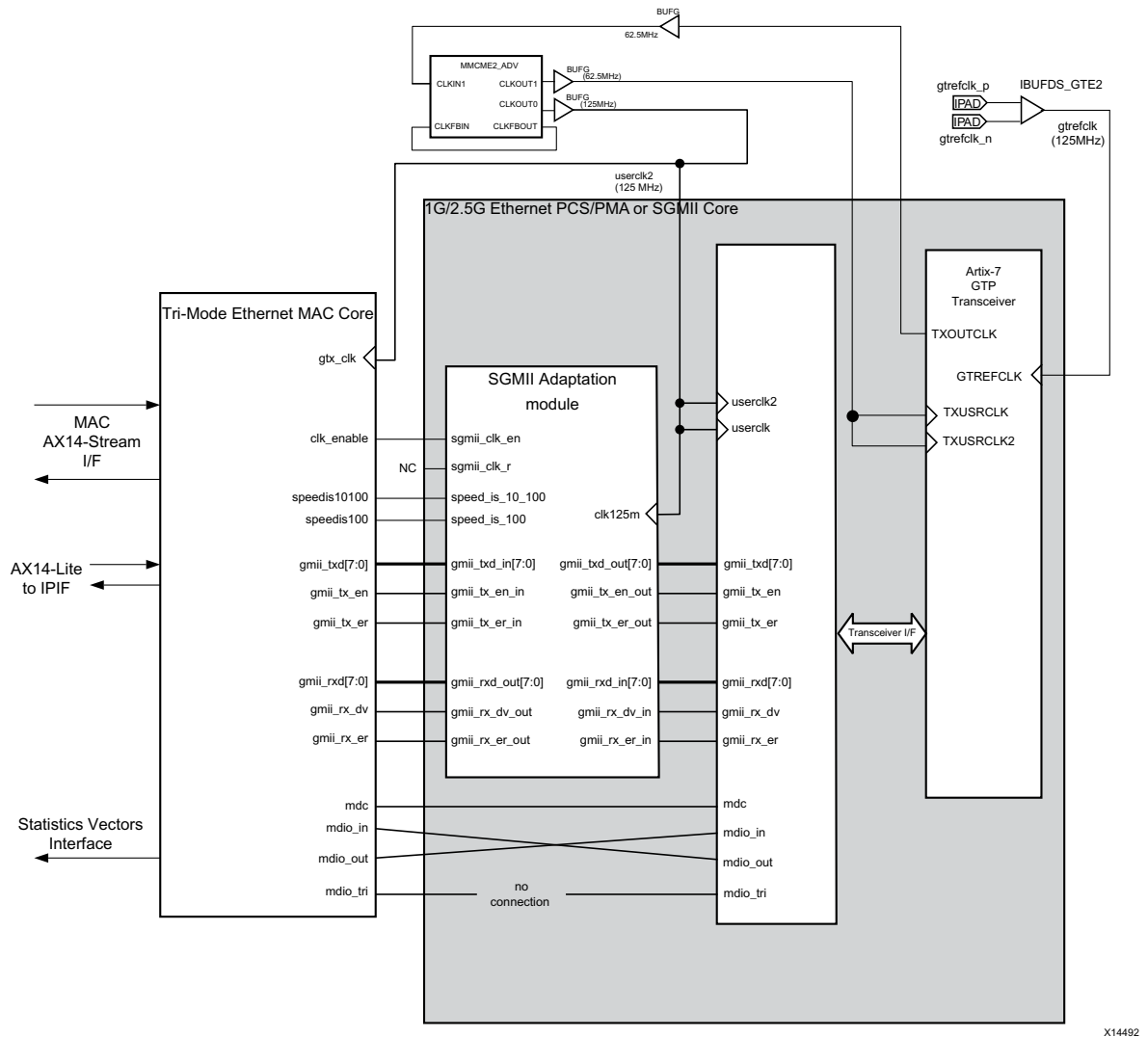
Figure 3-57: Core Using SGMII with Artix-7 Transceiver Connected to the TEMAC Core
