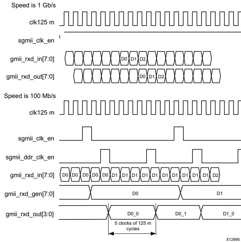
Figure 3-45: Receiver Rate Adaptation Module Data Sampling
