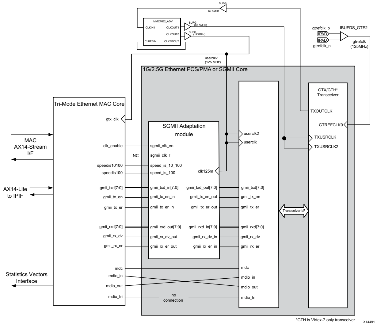
Figure 3-56: Core Using SGMII with the GTX/GTH Transceiver Connected to the TEMAC Core
