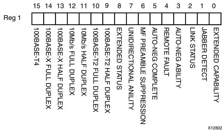
Figure 2-21: MDIO Register 1: Status Register
