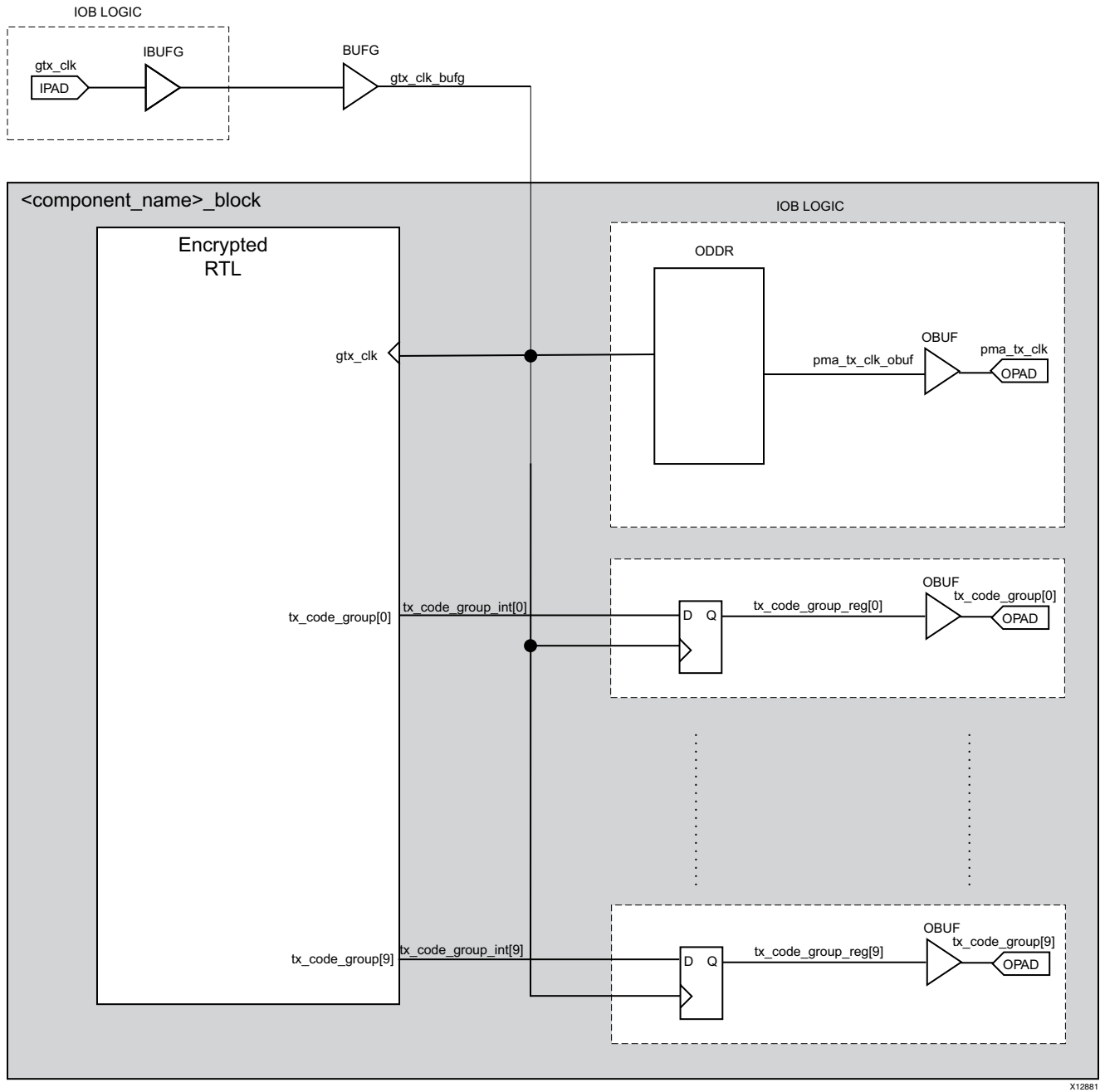
Figure 3-24: Ten-Bit Interface Transmitter Logic
