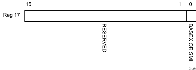
Figure 2-39: Dynamic Switching (Register 17)
