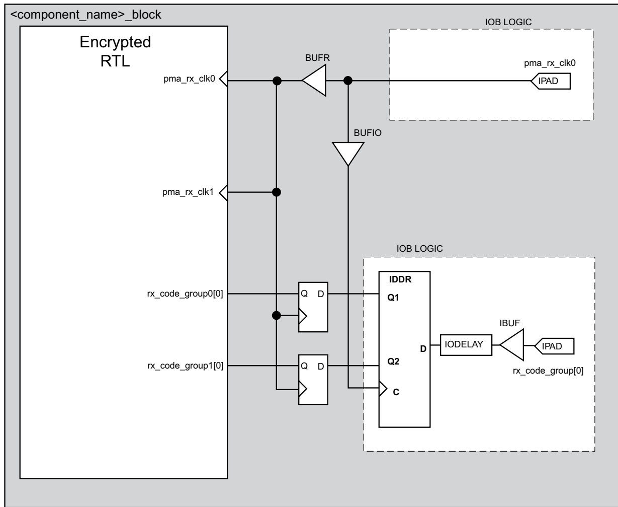
Figure 3-26: Ten-Bit Interface Receiver Logic - Kintex-7 Devices (Example Design)
