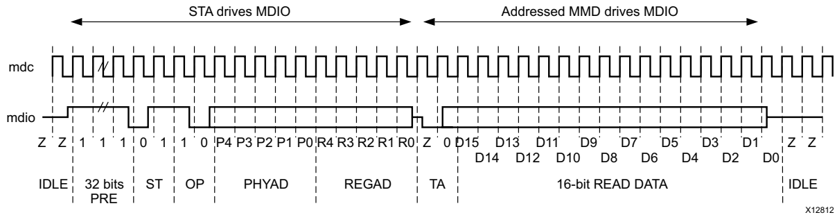
Figure 2-8: MDIO Read Transaction
