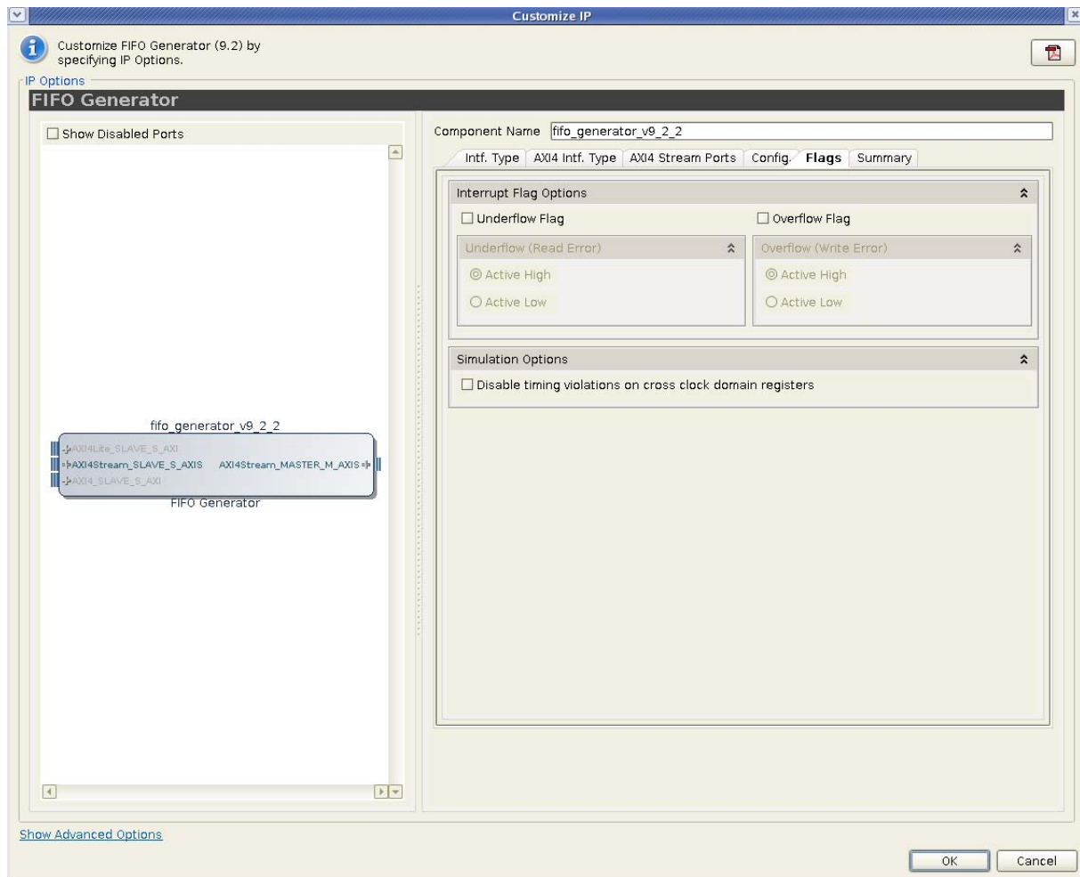
Figure 6-6: AXI4 FIFO Common Configurations Screen
