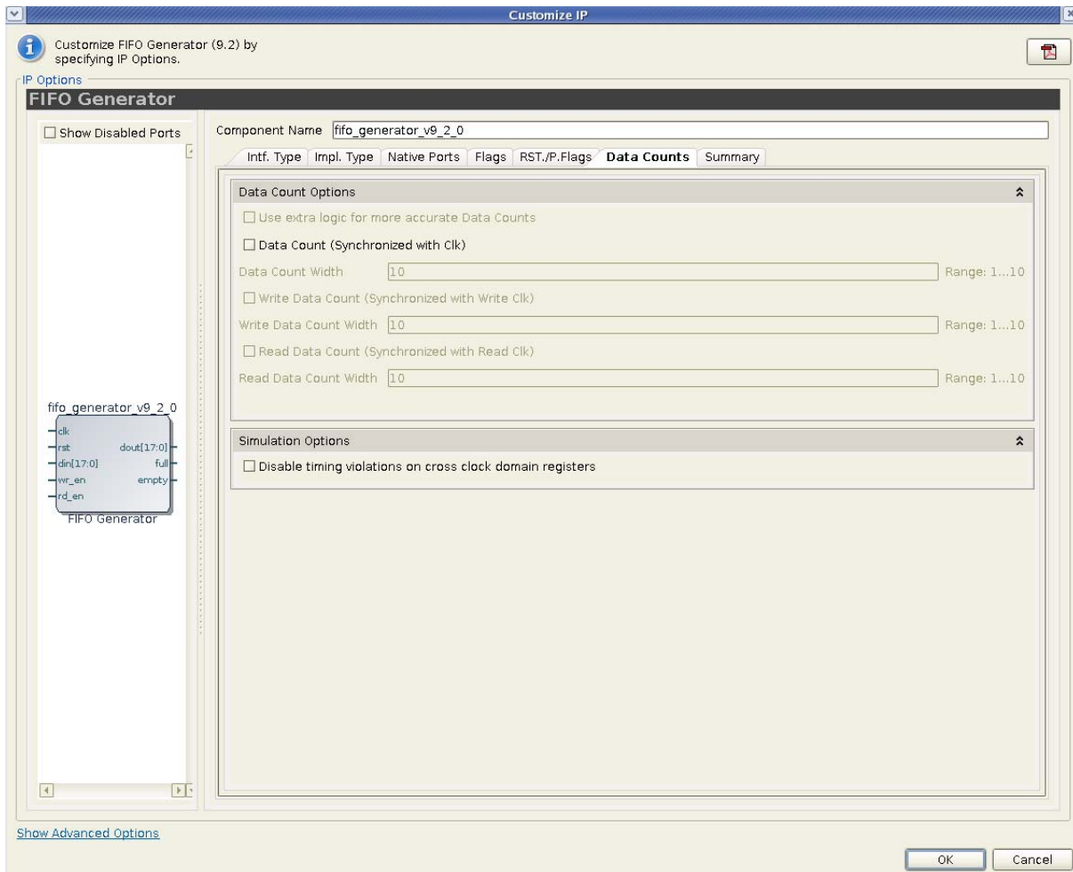
Figure 5-6: Data Count Screen
