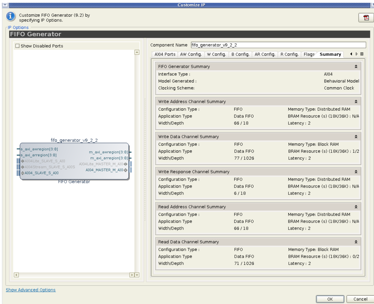
Figure 6-8: AXI4 / AXI4-Lite Summary Screen
