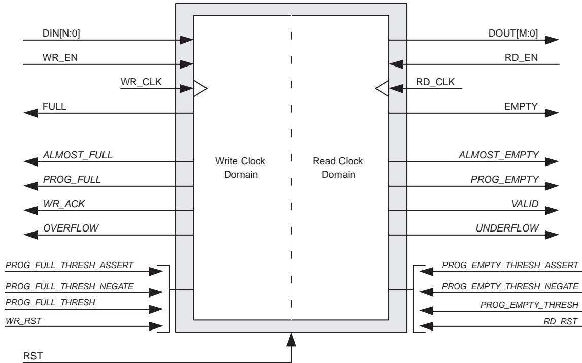
Figure 1-4: FIFO with Independent Clocks: Interface Signals
