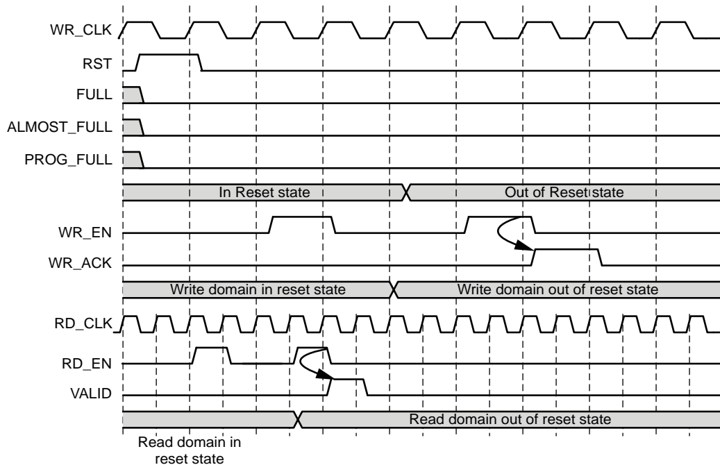
Figure 3-28: Block RAM, Distributed RAM, Shift RAM with Full Flags Reset Value of 0
