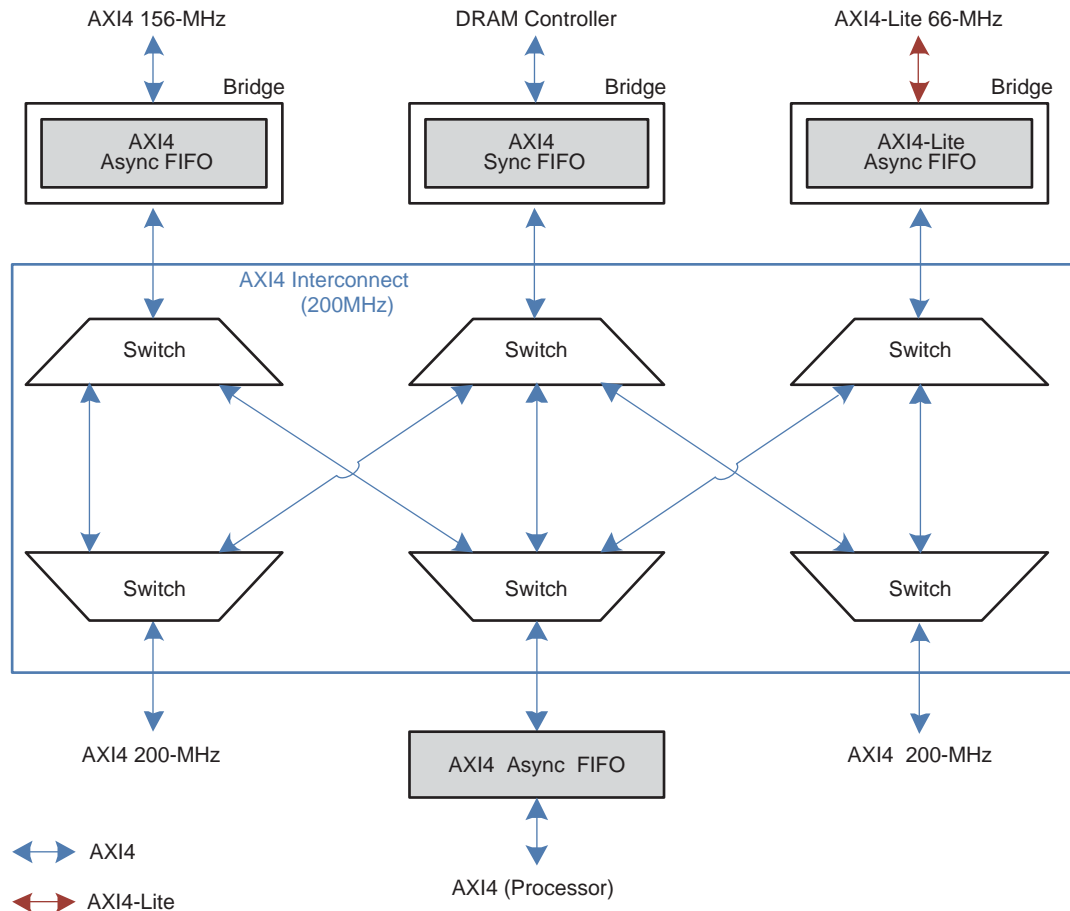
Figure 1-8: AXI4 Application Diagram
