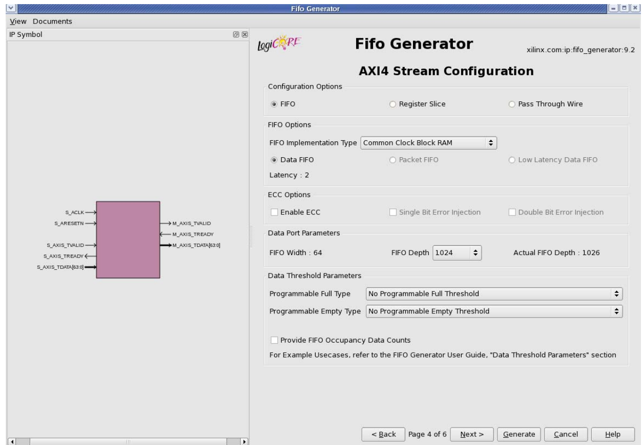
Figure 10-5: AXI4 FIFO Configurations Screen
