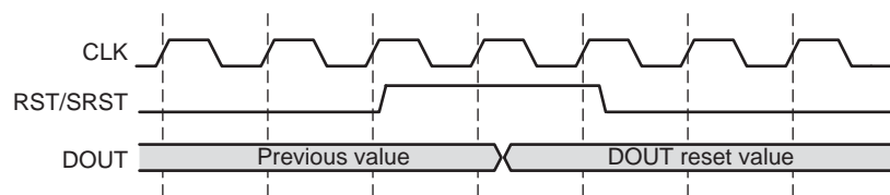
Figure F-1: DOUT Reset Value for Synchronous Reset (SRST) and for Asynchronous Reset (RST) for Common Clock Block RAM Based FIFO
