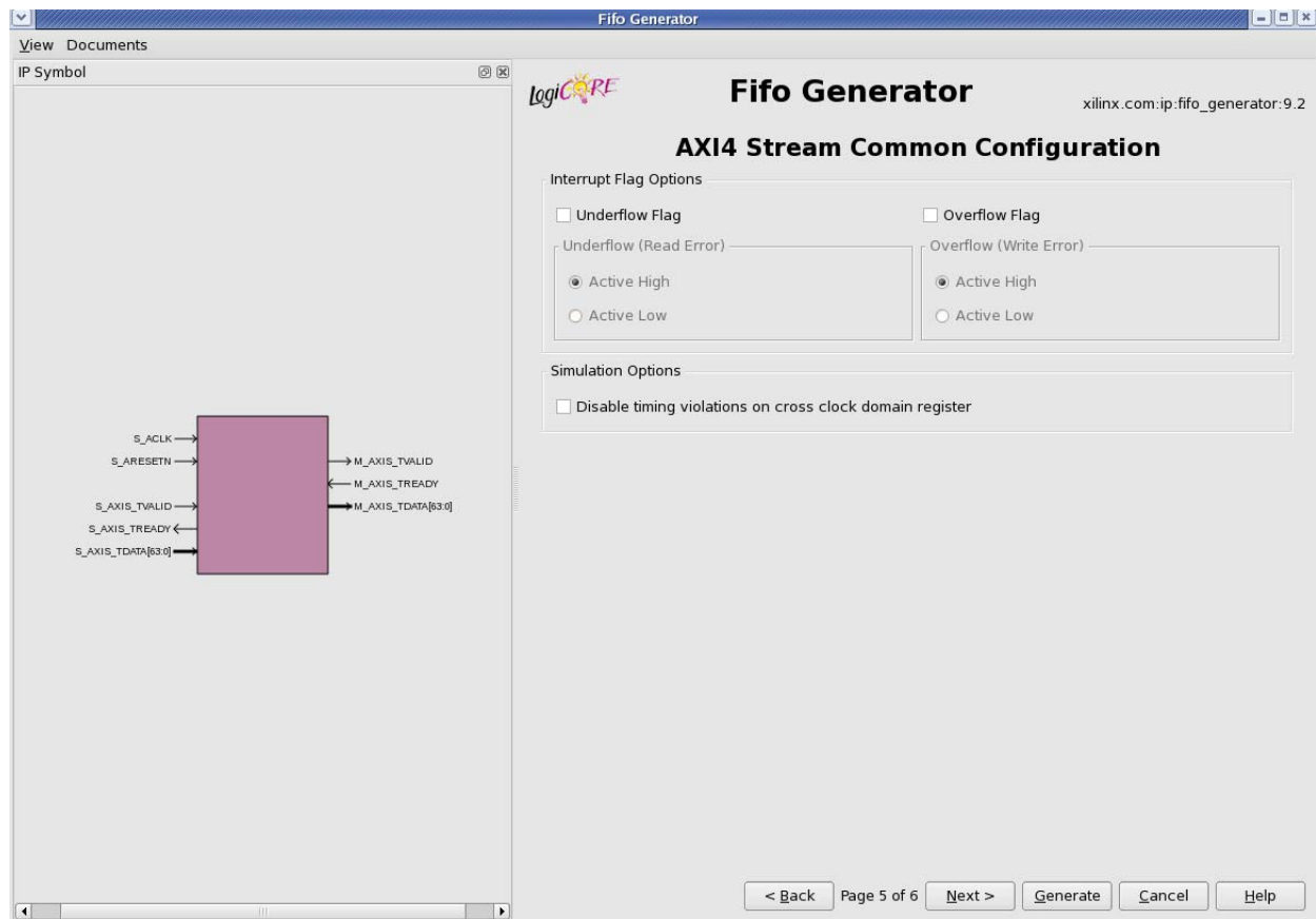
Figure 10-6: AXI4 FIFO Common Configurations Screen
