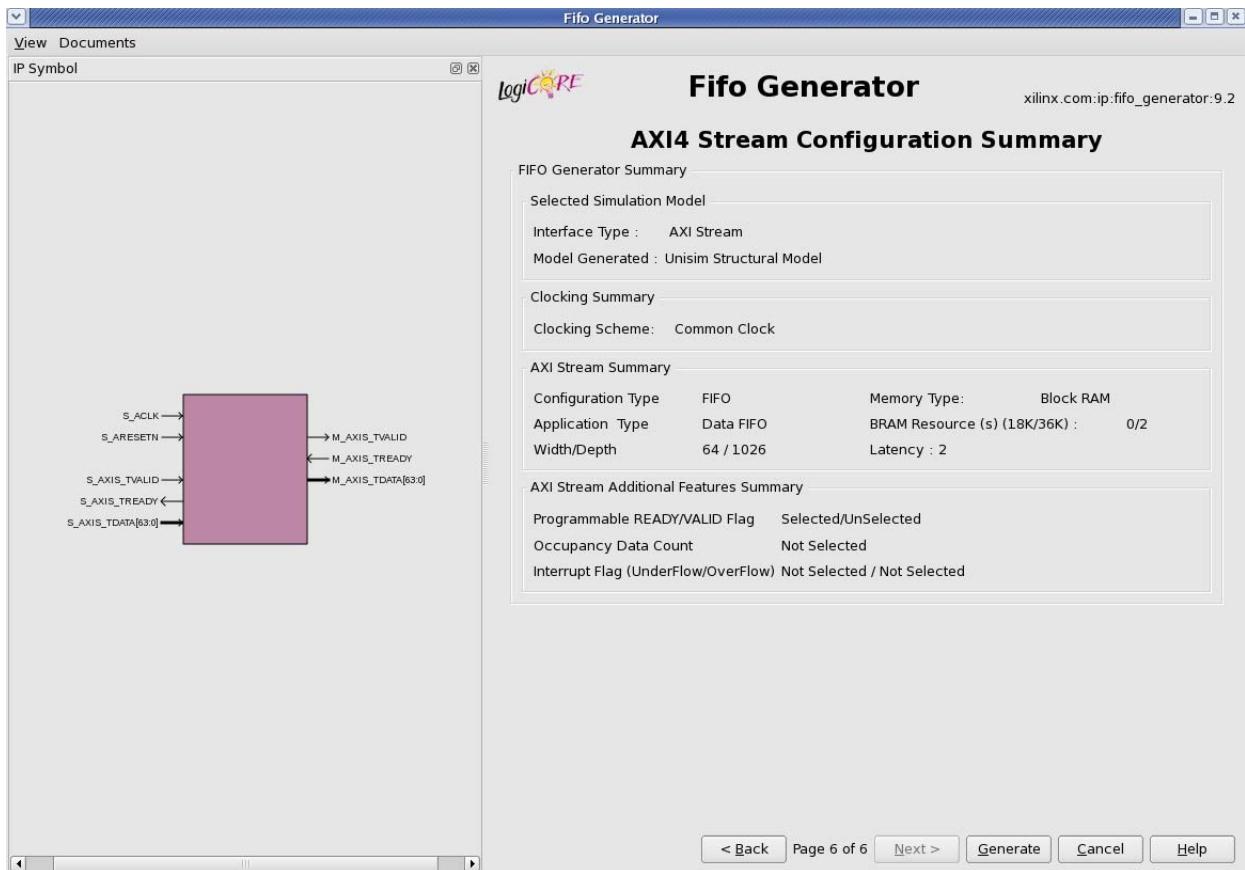
Figure 10-7: AXI4-Stream Summary Screen
