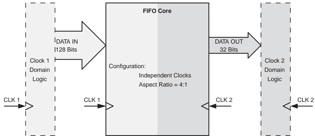
Figure 1-6: FIFO Generator Application Example
