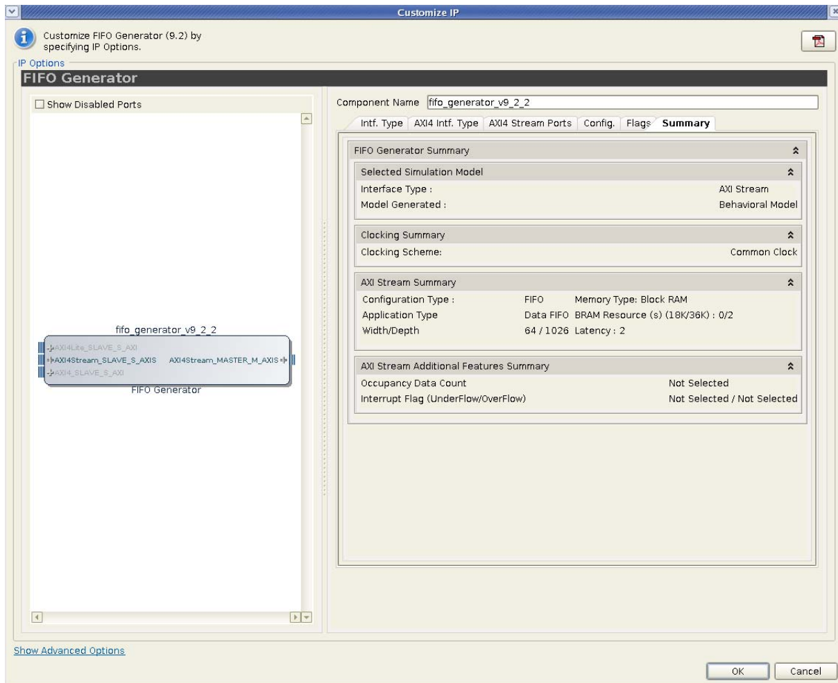
Figure 6-7: AXI4-Stream Summary Screen
