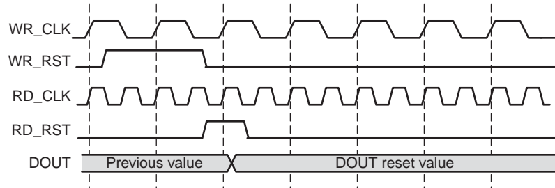
Figure F-4: DOUT Reset Value for Independent Clock Block RAM Based FIFO
