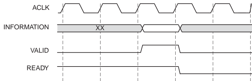
Figure 1-3: AXI4-FIFO Timing Diagram
