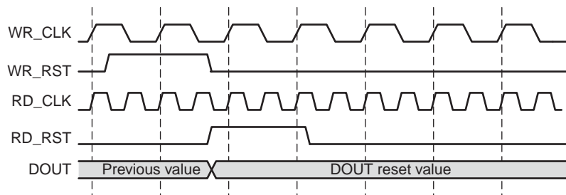
Figure F-5: DOUT Reset Value for Independent Clock Distributed RAM Based FIFO
