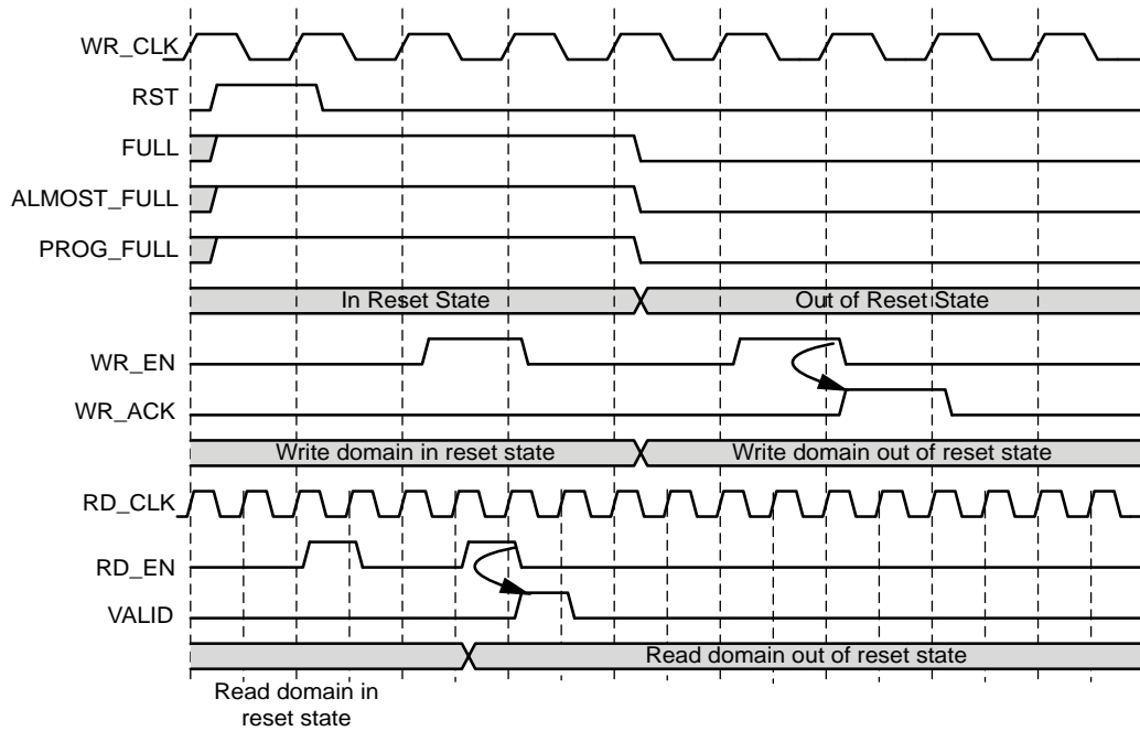
Figure 3-26: Block RAM, Distributed RAM, Shift RAM with Full Flags Reset Value of 1 for the Reset Pulse of One Clock
