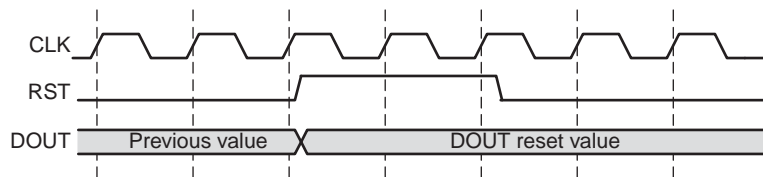
Figure F-2: DOUT Reset Value for Asynchronous Reset (RST) for Common Clock Distributed/Shift RAM Based FIFO
