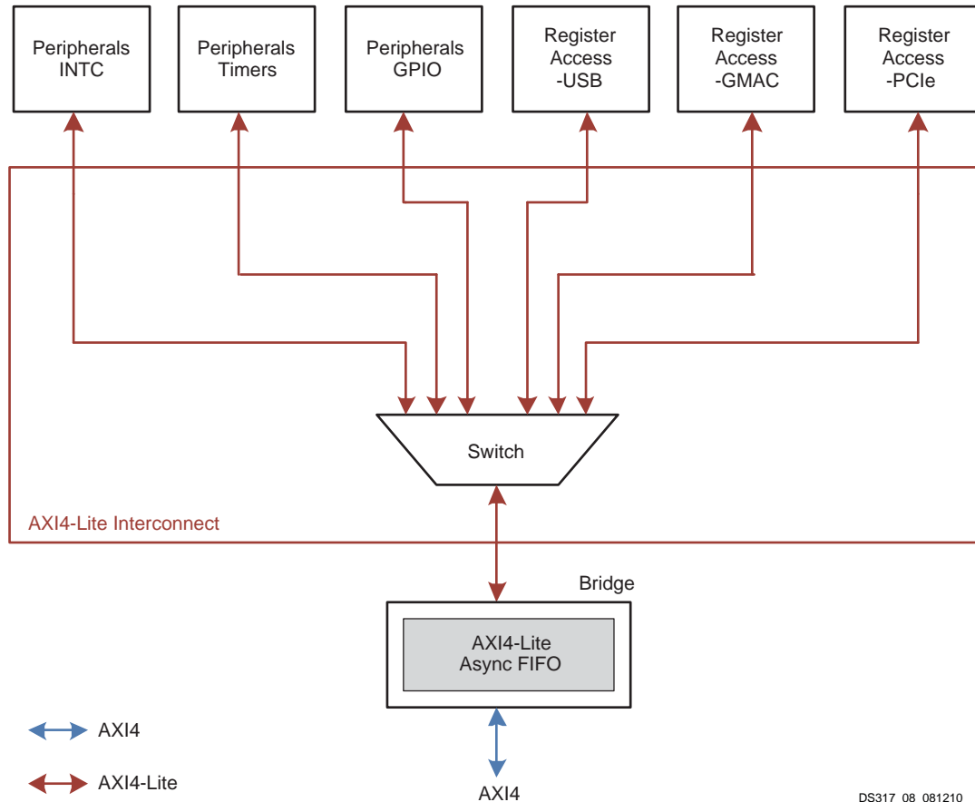
Figure 1-9: AXI4-Lite Application Diagram
