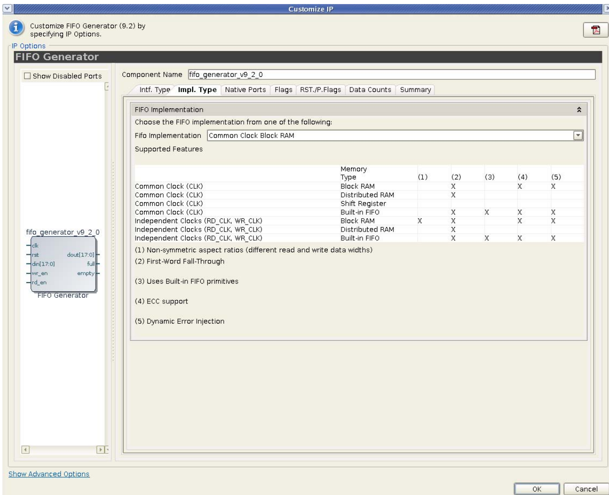
Figure 5-2: FIFO Implementation Screen
