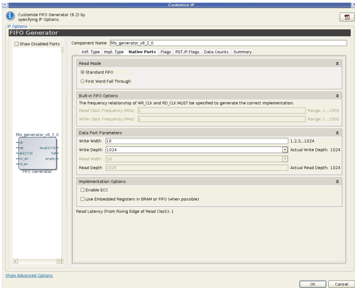
Figure 5-3: Performance Options and Data Port Parameters Screen
