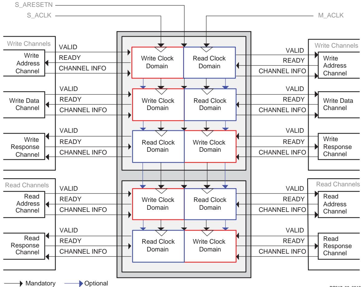
Figure 1-5: AXI4 Block Diagram
