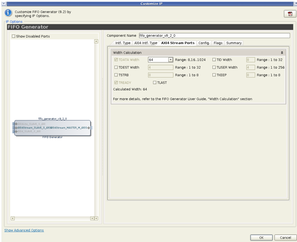
Figure 6-2: AXI4-Stream Width Calculation Screen
