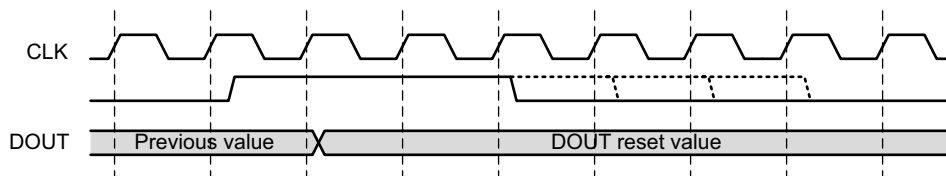
Figure F-3: DOUT Reset Value for Common Clock Built-in FIFO
