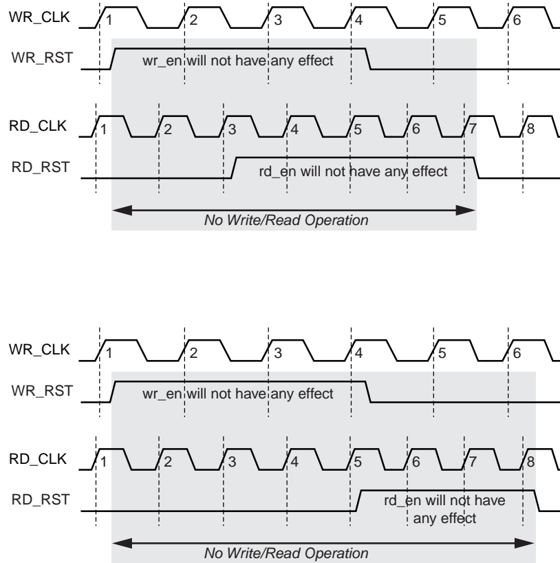
Figure 3-33: Synchronous Reset: FIFO with Independent Clock - WR_RST then RD_RST
