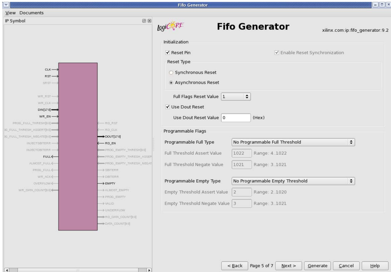
Figure 9-5: Programmable Flags and Reset Screen
