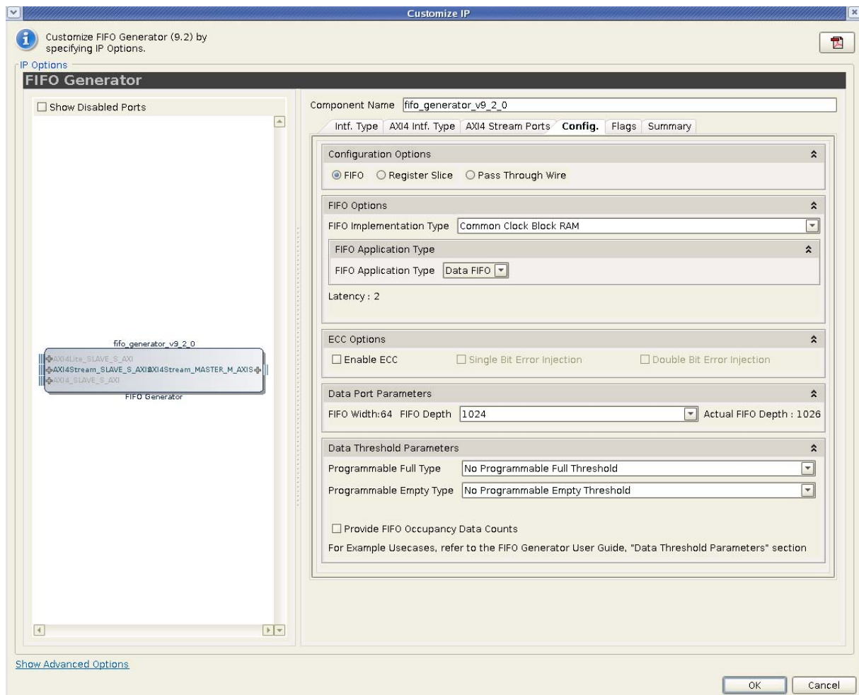
Figure 6-5: AXI4 FIFO Configurations Screen
