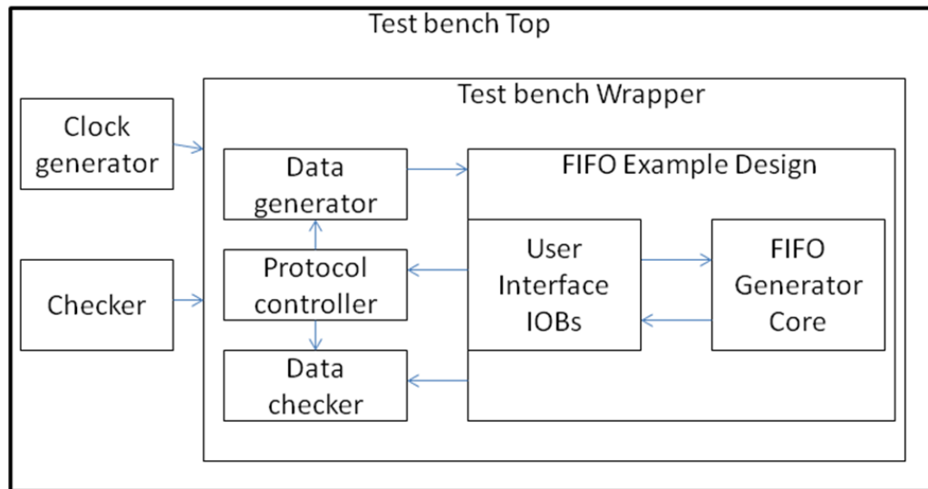
Figure 12-2: Demonstration Test Bench
