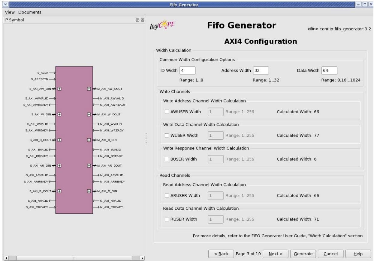
Figure 10-3: AXI4 Width Calculation Screen
