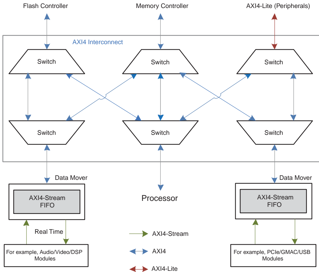
Figure 1-7: AXI4-Stream Application Diagram
