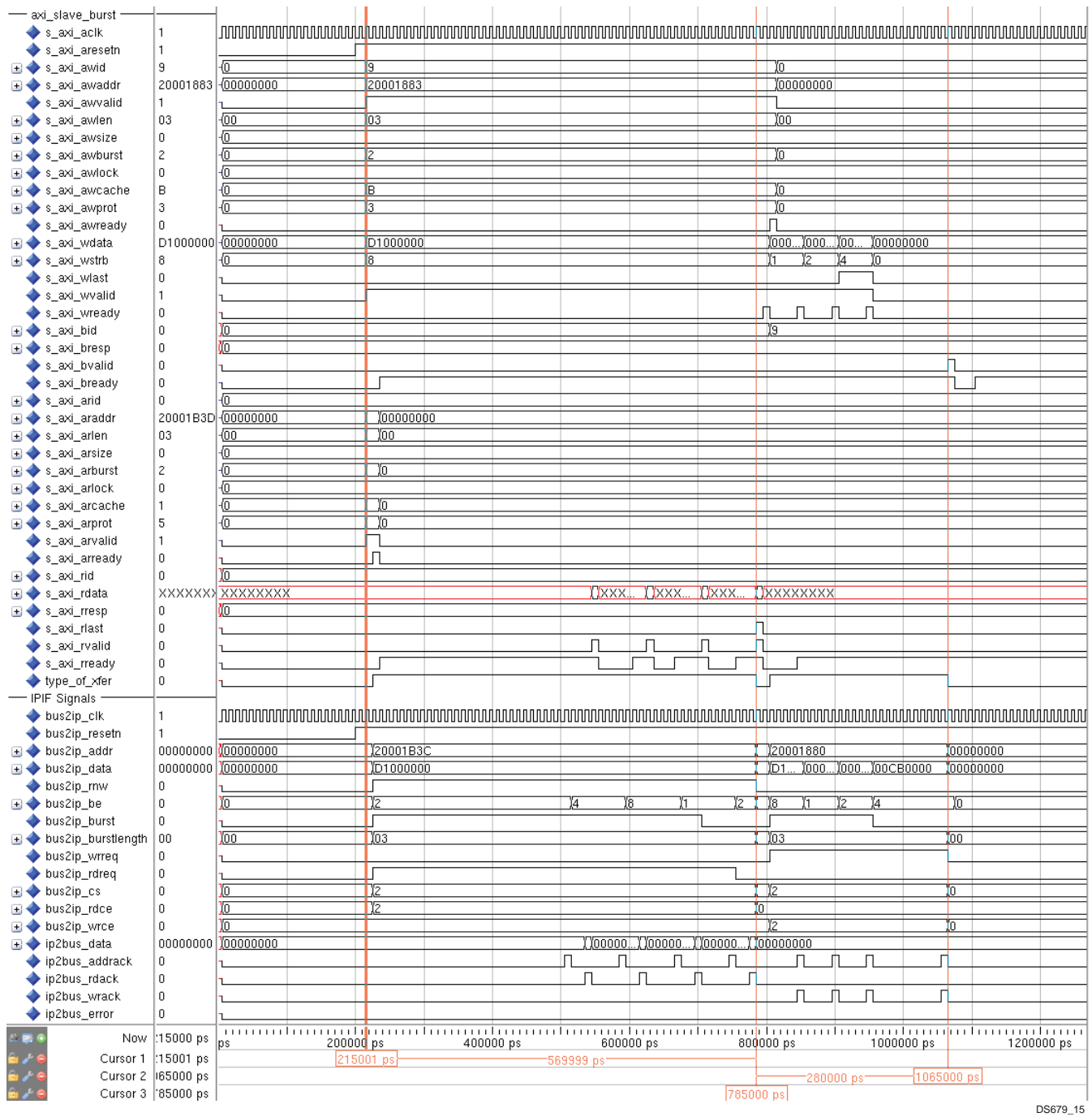
Figure 15: AXI Slave Burst Response For AXI4 FIXED Read-Write Transactions (FIFO is Included)
