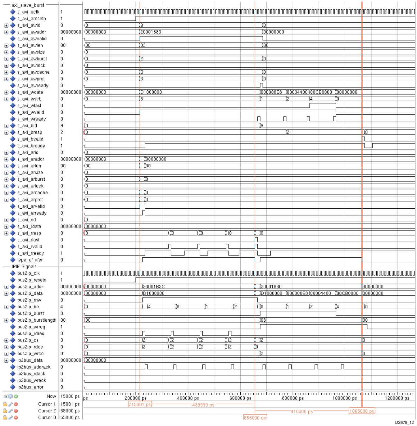
Figure 12: AXI Slave Burst Response For AXI4 WRAP Mode Transactions When Slave IP Does Not Respond the Read and Write Data Phase (FIFO Not Included)
