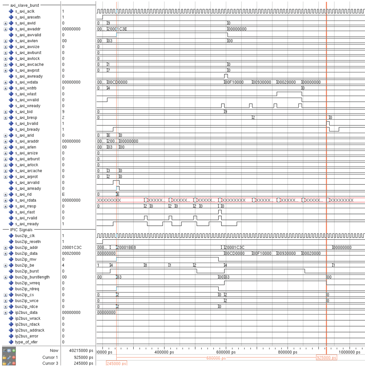
Figure 18: AXI Slave Burst Response For AXI4 FIXED Mode Transactions When Slave IP Does Not Respond the Address Available on Bus2IP_Addr (FIFO is Included)
