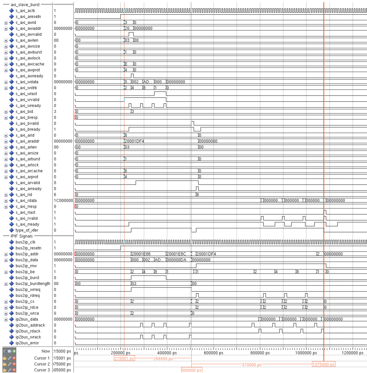
Figure 7: AXI Slave Burst Response For AXI4 INCR Mode Transactions When Slave IP Does Not Respond the Address Available on Bus2IP_Addr (FIFO Not Included)
