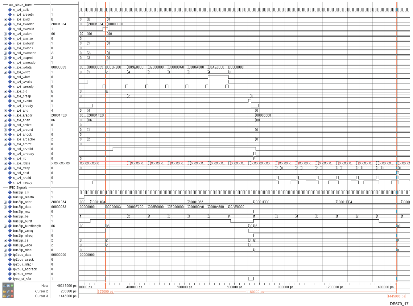
Figure 17: AXI Slave Burst Response For AXI4 INCR Mode Transactions When Slave IP Does Not Respond the Address Available on Bus2IP_Addr (FIFO is Included)
