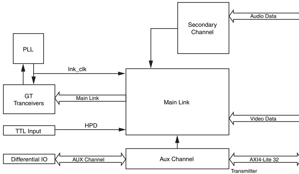
Figure 1-1: Source Core Top Level
