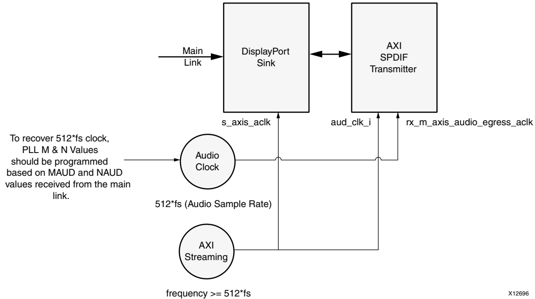
Figure 3-15: Sink: Audio Clocking
