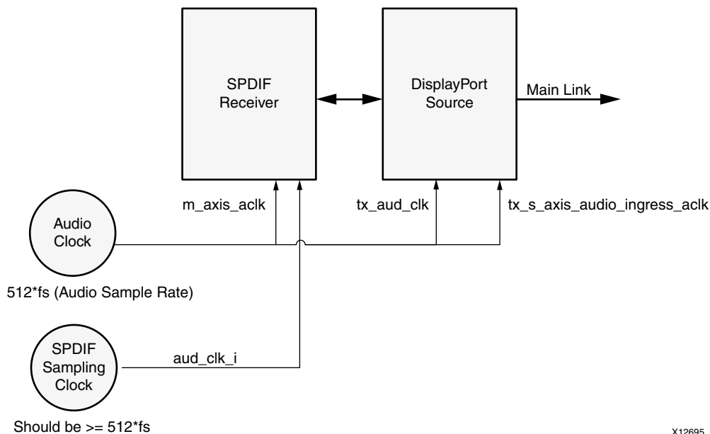
Figure 3-9: Source: Audio Clocking
