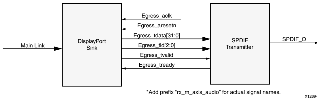
Figure 3-14: Audio Data Interface of DisplayPort Sink System
