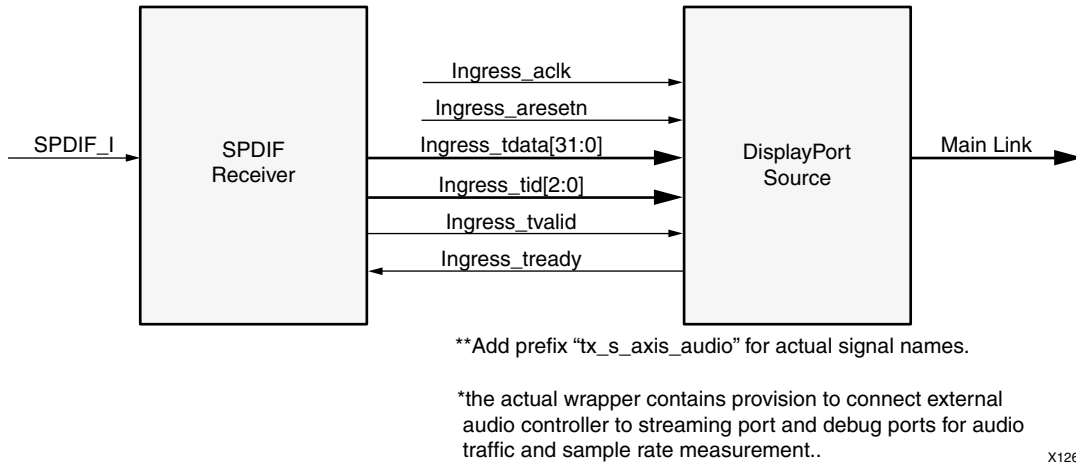
Figure 3-8: Audio Data Interface of DisplayPort Source System
