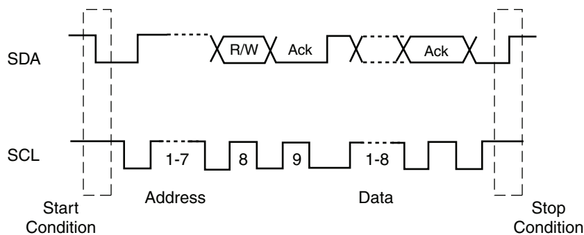
Figure 3-28: I2C Transaction
