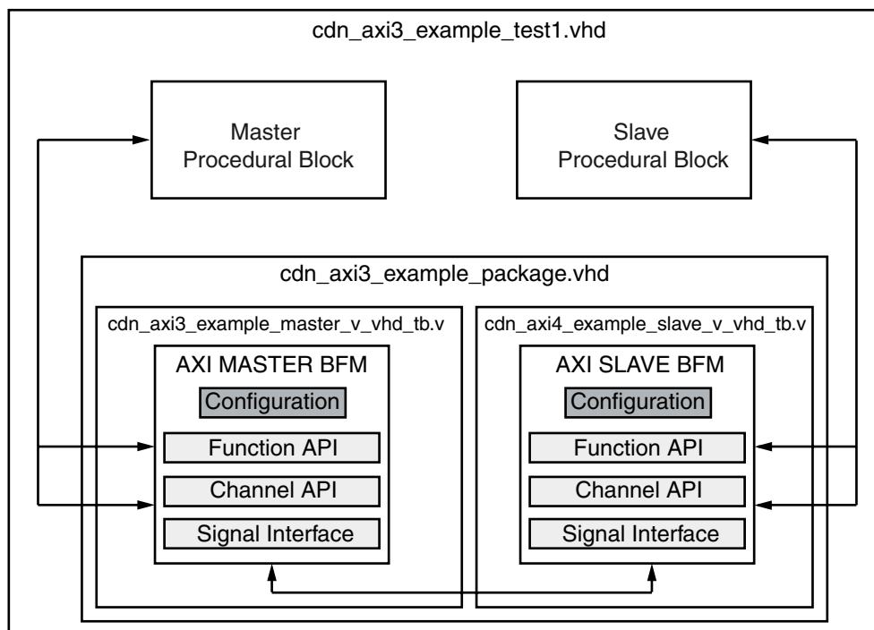
Figure 4: AXI3 BFM VHDL Example Test Bench and Example Test
