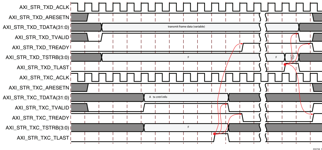
Figure 3-2: Normal Transmit AXI4-Stream Waveform
