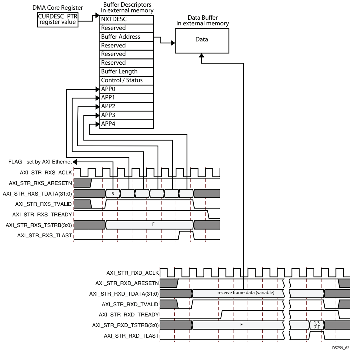
Figure 3-7: Receive AXI DMA Buffer Descriptor AXI4-Stream Field Mapping
