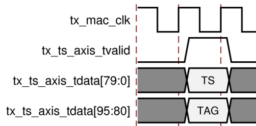
Figure 2-21: Transmit 2-step Timestamp
