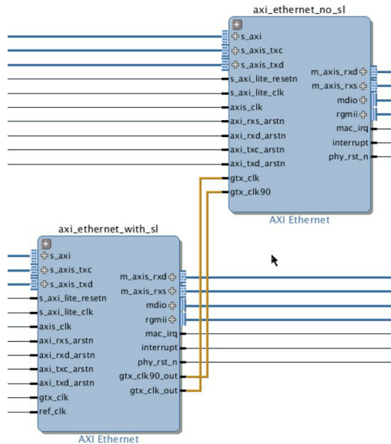
Figure 4-7: Connections to Enable Sharing Logic among Two Instances
