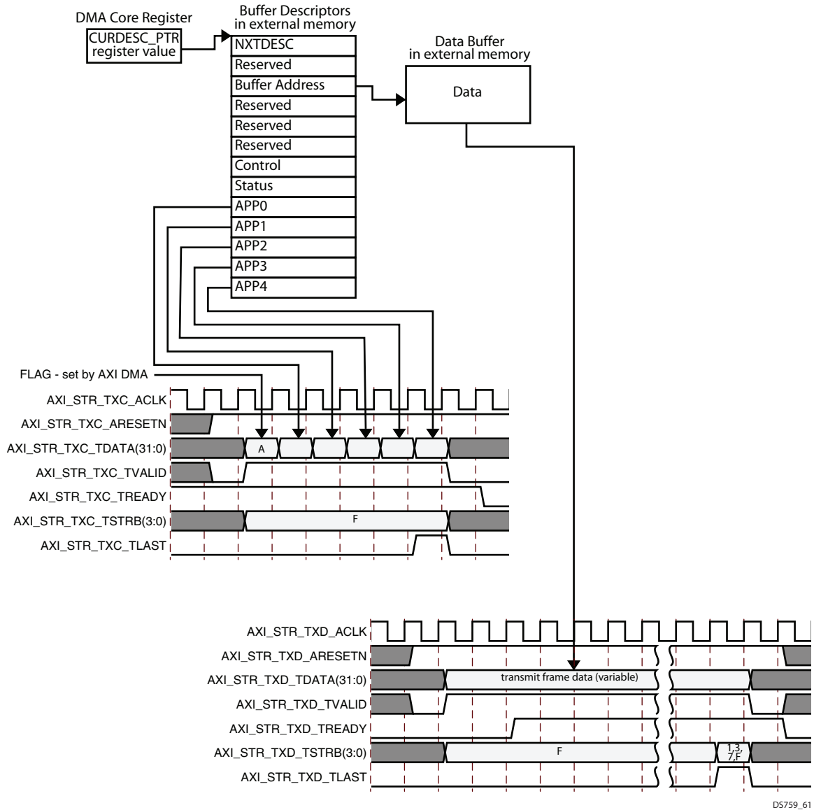
Figure 3-6: Transmit AXI DMA Buffer Descriptor AXI4-Stream Field Mapping
