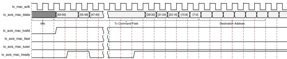
Figure A-5: Timing Diagram of the In-line Command Field and Frame Data for Transmission
