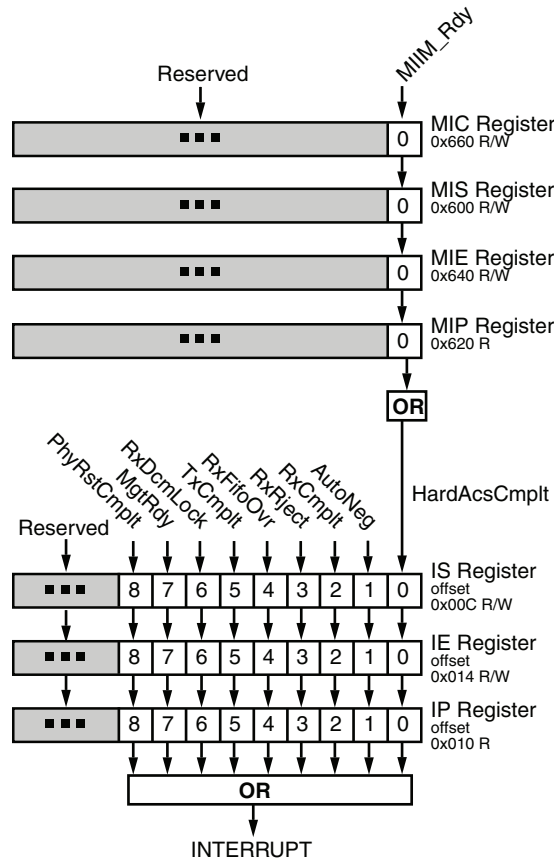
Figure 2-25: Subsystem Interrupt Structure
