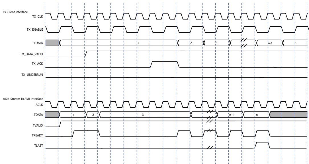
Figure 3-9: 100 Mb/s Transmit AVB AXI4-Stream
