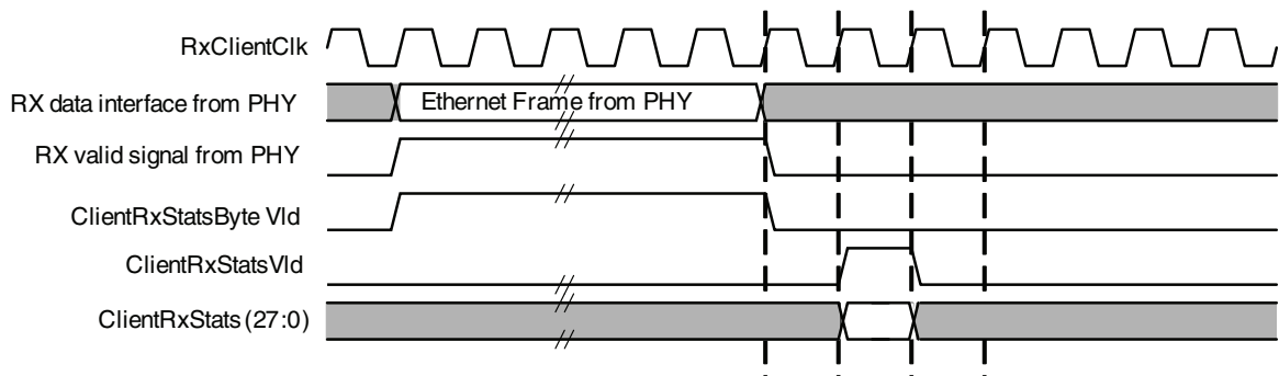
Figure 2-24: Receive Statistics Waveforms
