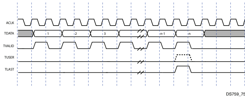
Figure 3-10: 100 Mb/s Receive AVB AXI4-Stream
