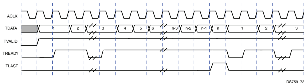
Figure 3-8: 1000 Mb/s Transmit AVB AXI4-Stream (back-to back)
