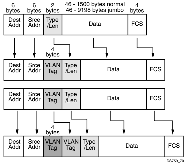
Figure 2-16: VLAN Tagging
