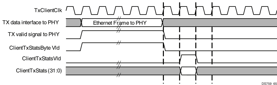
Figure 2-23: TEMAC Transmit Statistics Waveforms
