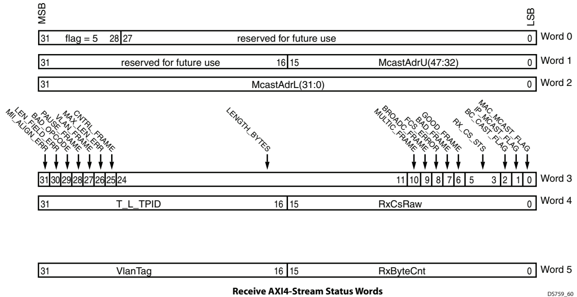
Figure 3-5: Receive AXI4-Stream Status Words
