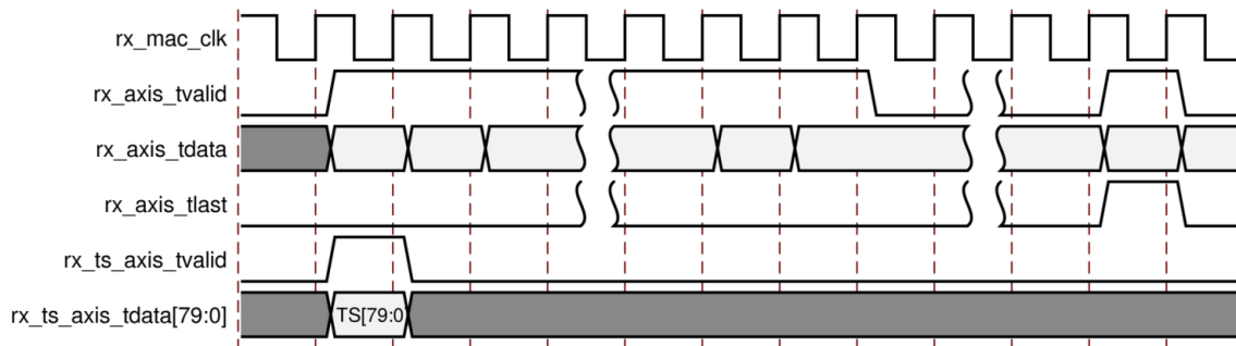
Figure A-3: Timing Diagram of the In-line Timestamp and Received Frame
