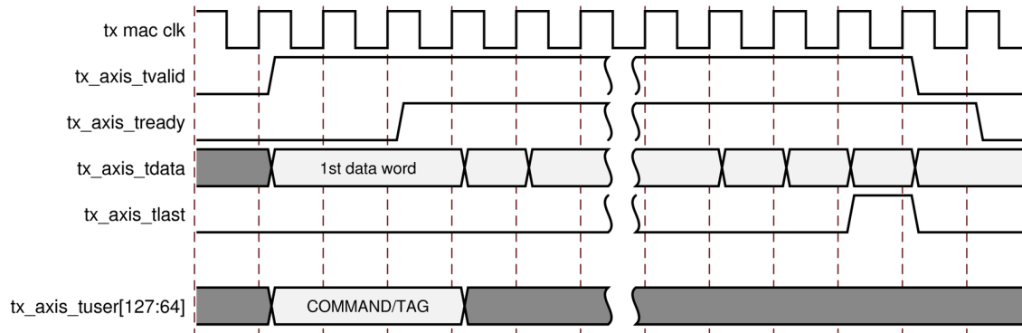
Figure A-4: AXI4-Stream Interface Timing – Out-of-band Command Field
