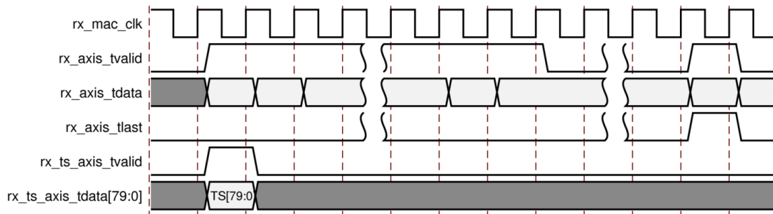
Figure 2-22: AXI4-Stream Interface Timing – Receive Timestamp
