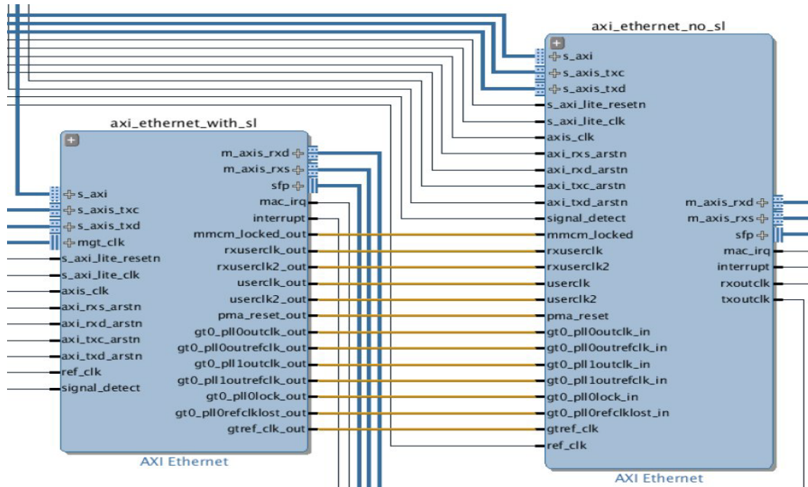
Figure 4-8: Connections to Enable Sharing of GTCOMMON among Two Instances
