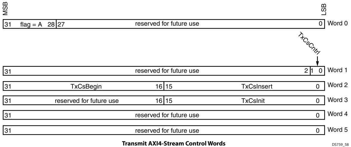
Figure 3-3: Transmit AXI4-Stream Control Words
