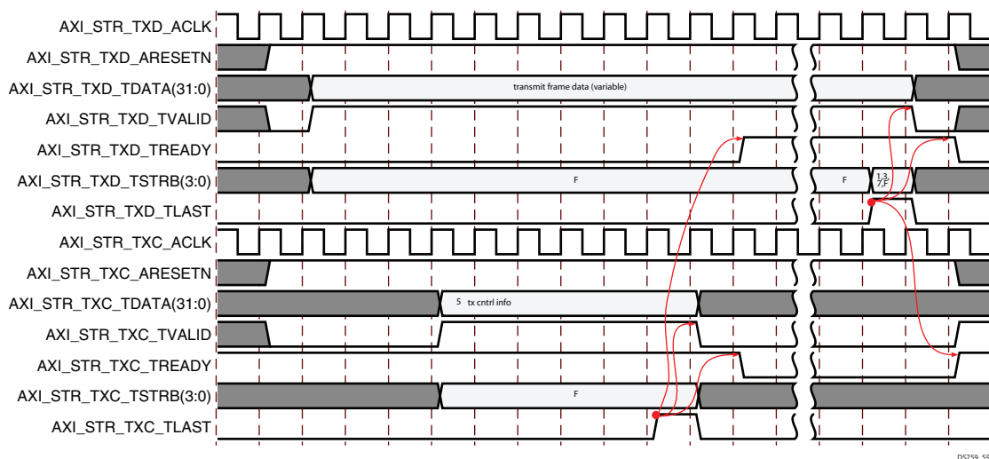
Figure 3-4: Receive Status Transmit AXI4-Stream Waveform
