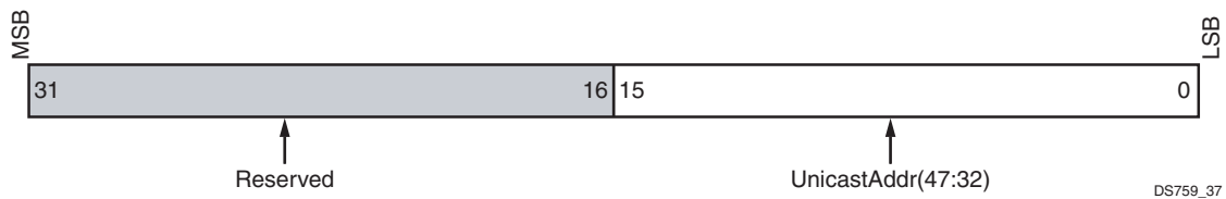
Figure 2-65: TEMAC Unicast Address Word 1 Register (offset 0x0000704)
