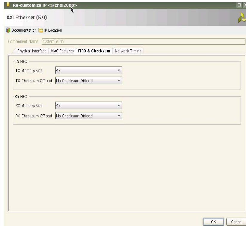
Figure 4-3: FIFO and Checksum
