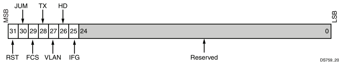
Figure 2-49: TEMAC Transmit Configuration Register (offset 0x408)
