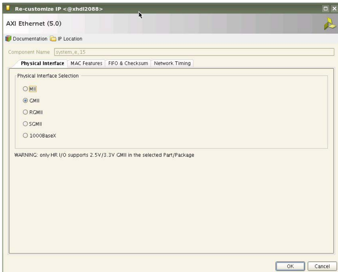
Figure 4-1: Physical Interface
