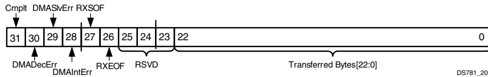
Figure 3-10: S2MM_STATUS
