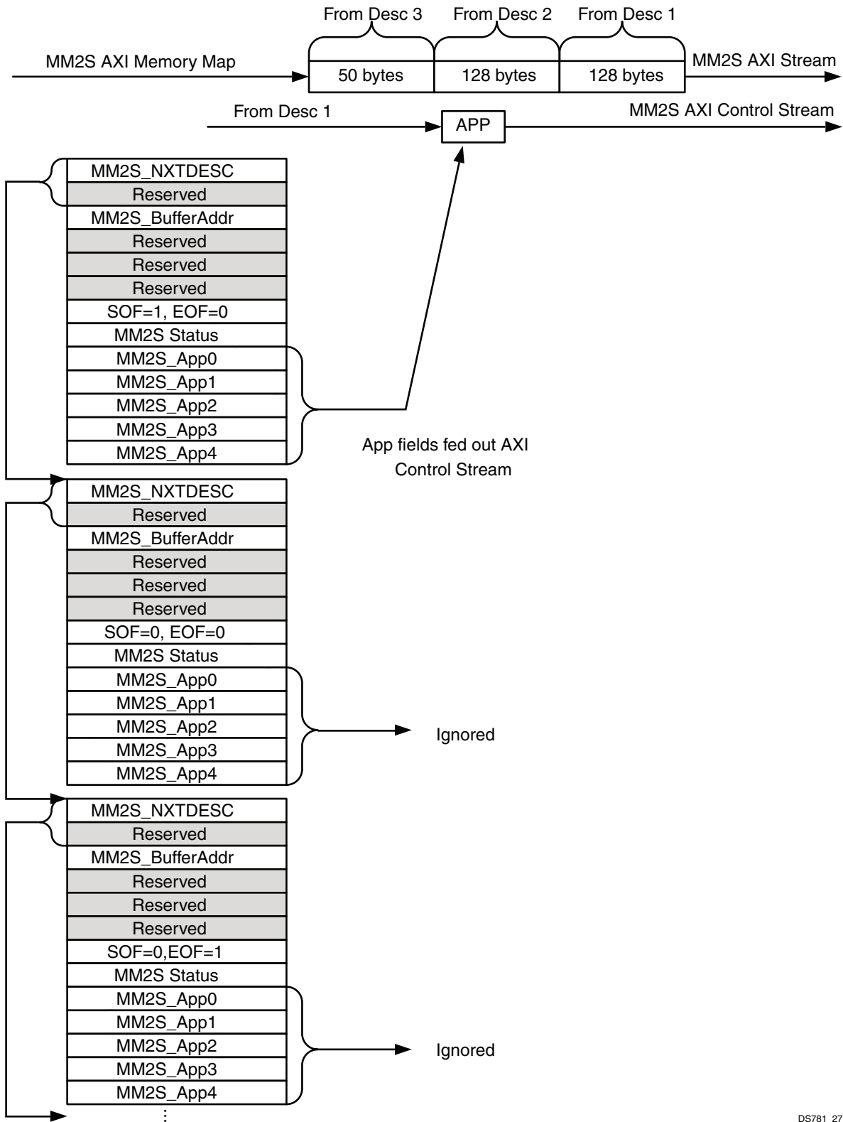
Figure 4-17: Detail of Descriptor Relationship to MM2S Stream and Control Stream
