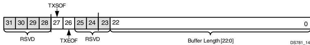
Figure 4-4: MM2S_CONTROL
