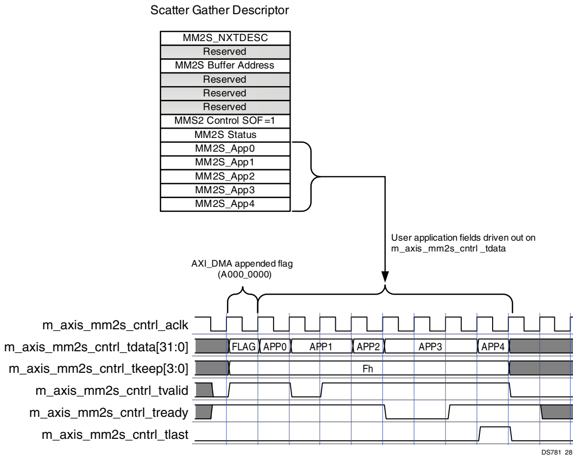
Figure 4-18: Example User Application Field / Timing for MM2S Control Stream
