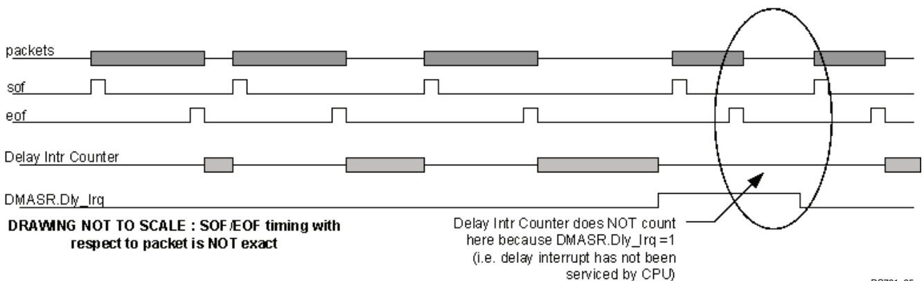
Figure 4-32: Example Delay Timer Timing
