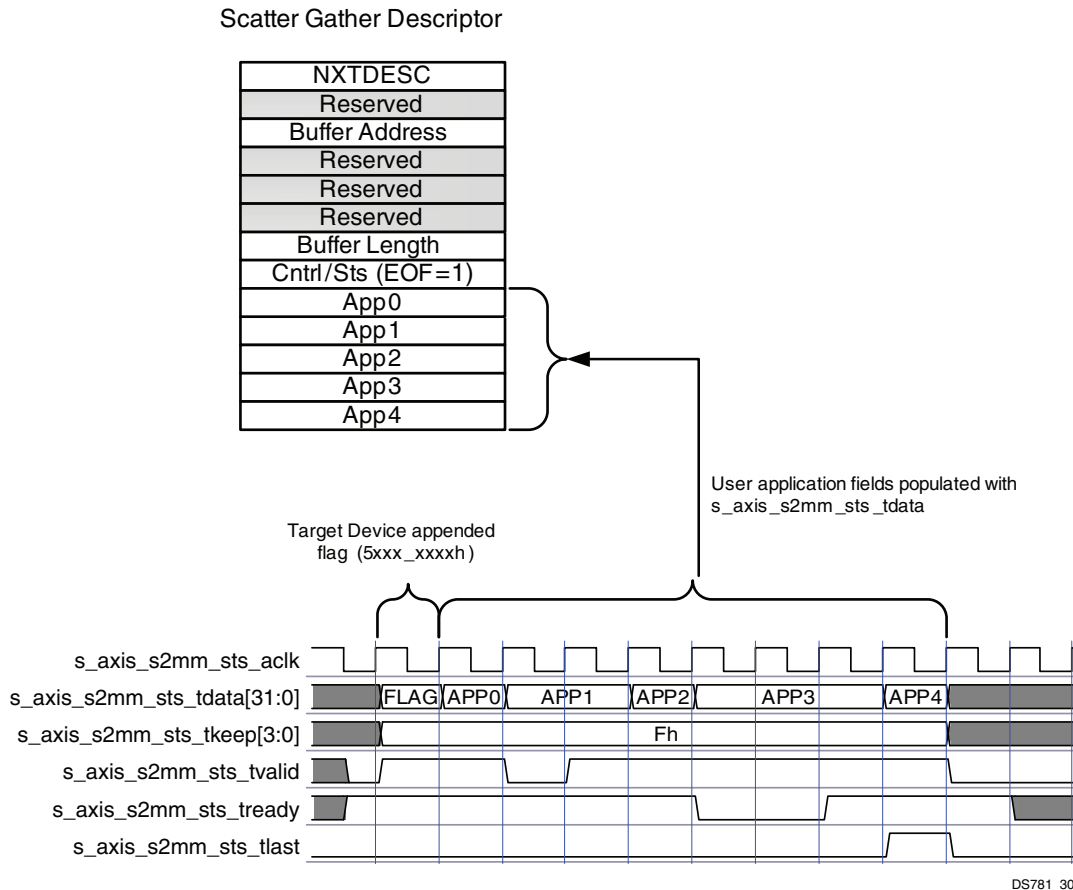
Figure 4-20: Example User Application Field / Timing for S2MM Status Stream
