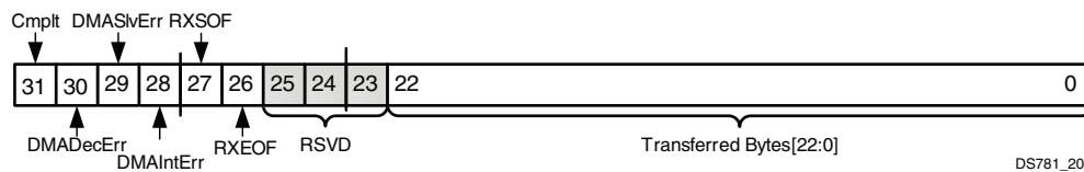
Figure 4-10: S2MM_STATUS
