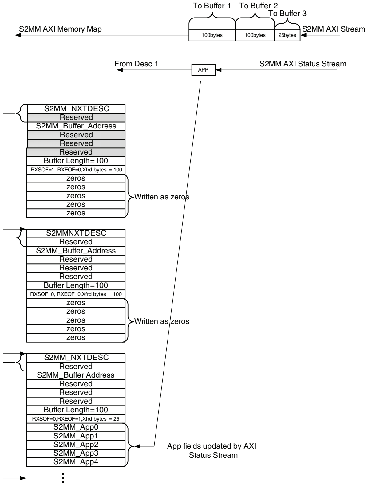
Figure 4-19: Detail of Descriptor Relationship to S2MM Stream and Status Stream
