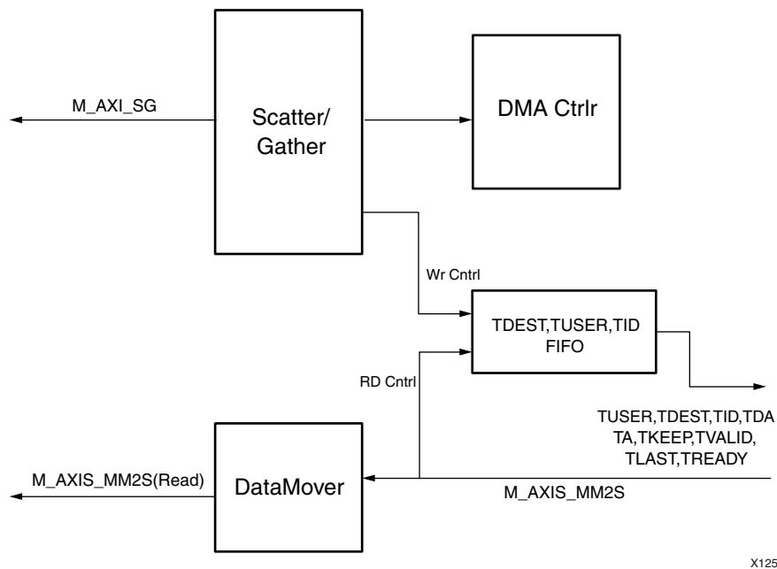
Figure 4-24: MM2S Control and Datapath Flow
