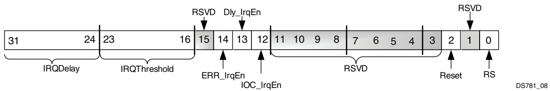
Figure 2-10: S2MM DMCCR Register
