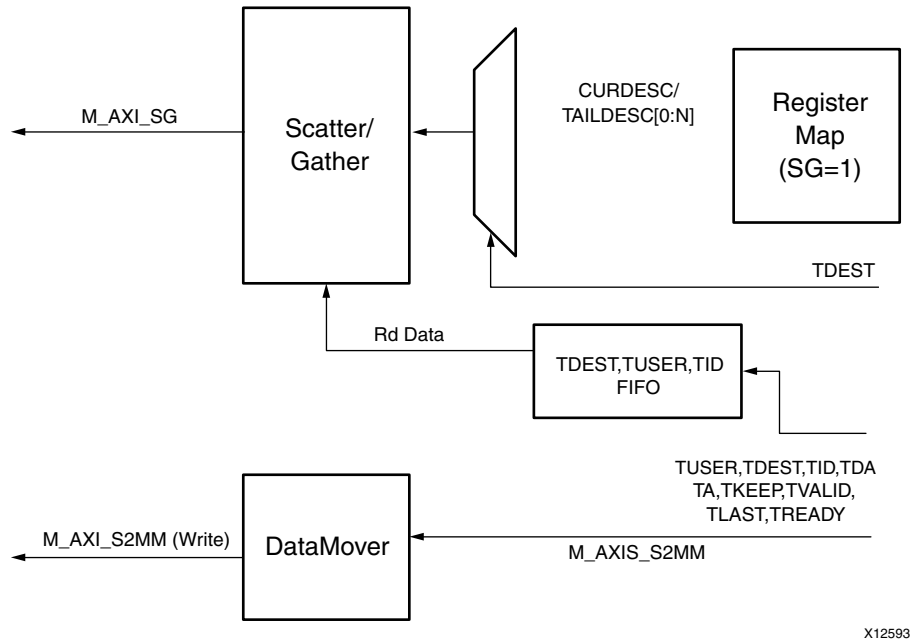
Figure 4-25: S2MM Control and Datapath Flow
