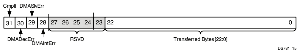
Figure 4-5: MM2S_STATUS
