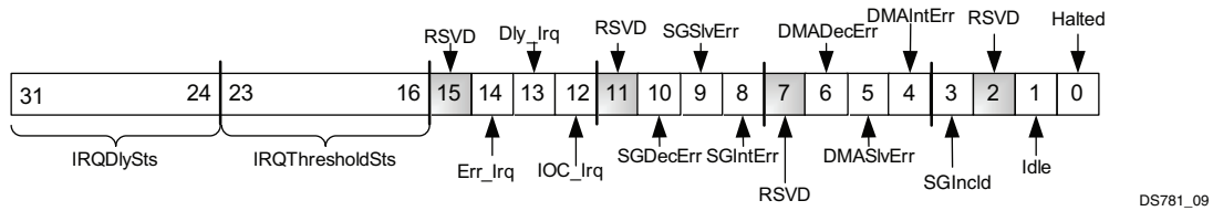
Figure 2-11: S2MM DMASR Register
