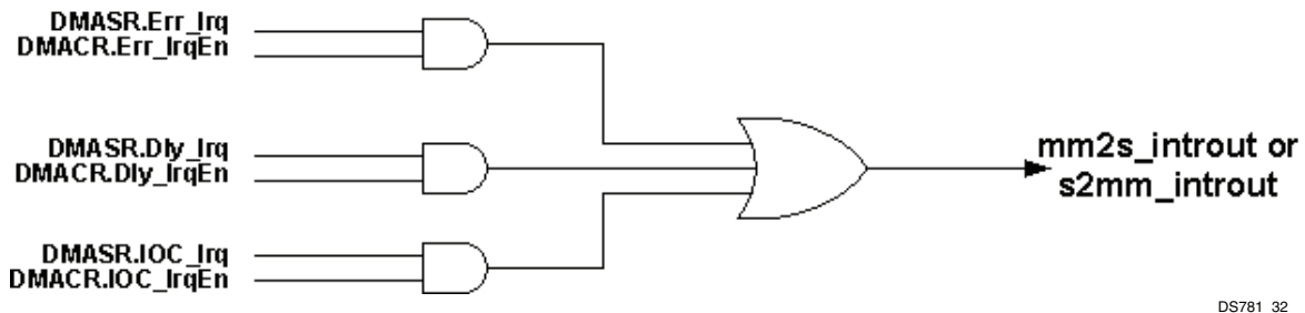
Figure 4-29: Interrupt Out Concept
