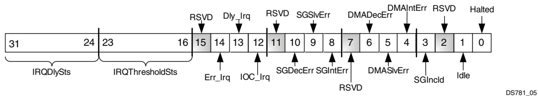
Figure 2-4: MM2S DMASR Register
