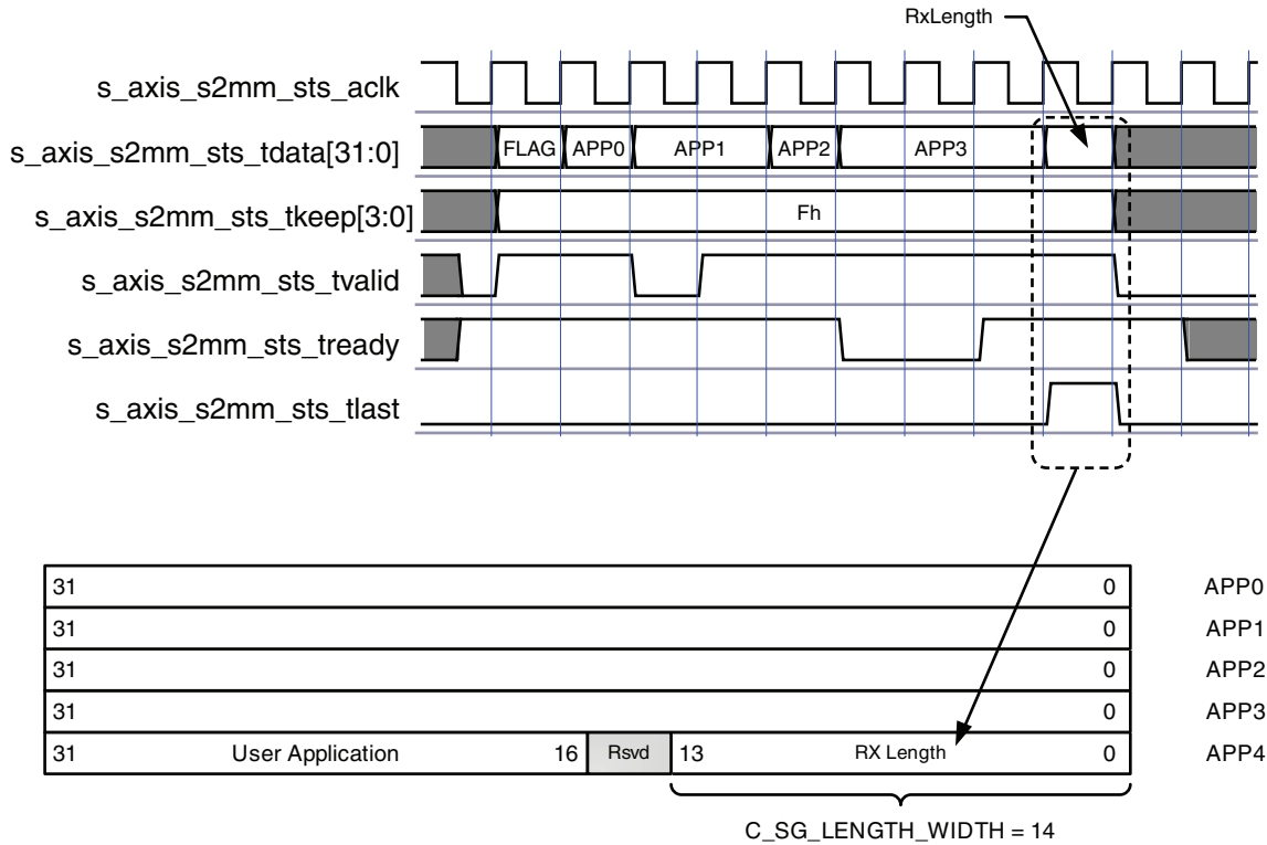
Figure 4-21: Receive Length Timing
