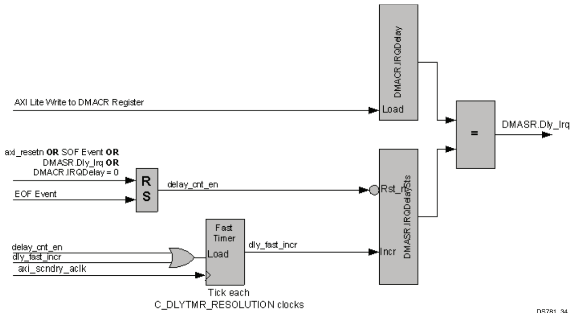
Figure 4-31: Delay Interrupt Logic Concept
