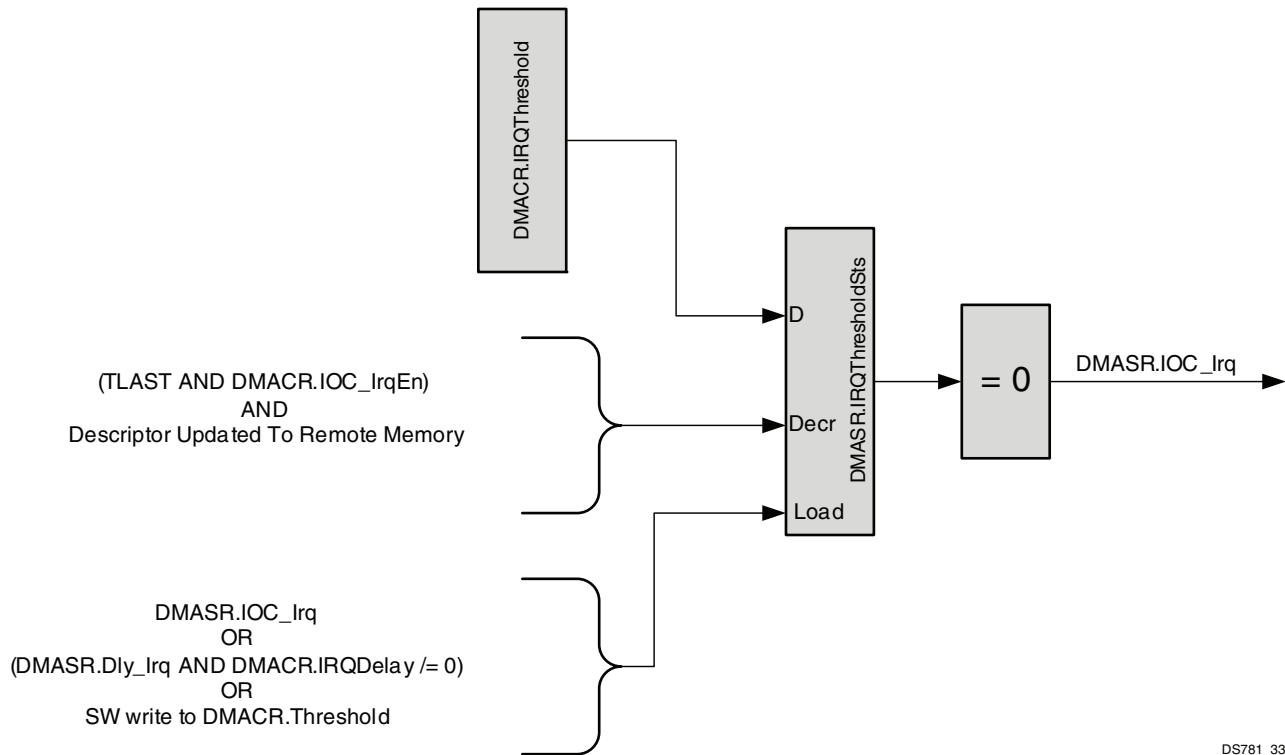
Figure 4-30: Interrupt On Complete Threshold Logic Concept
