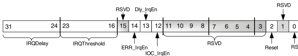
Figure 2-3: MM2S DMACR Register
