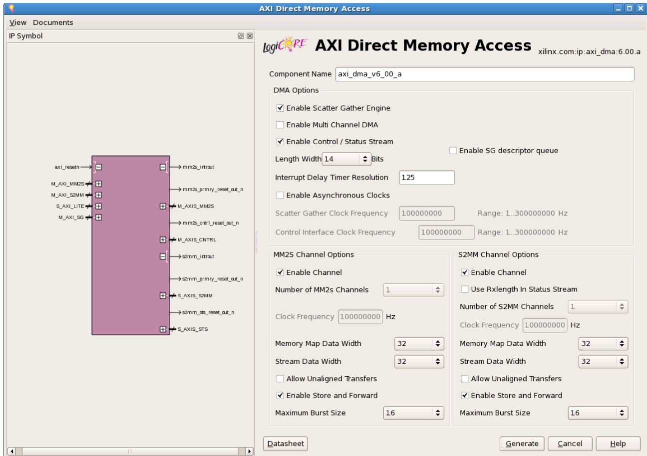
Figure 3-1: AXI DMA GUI
