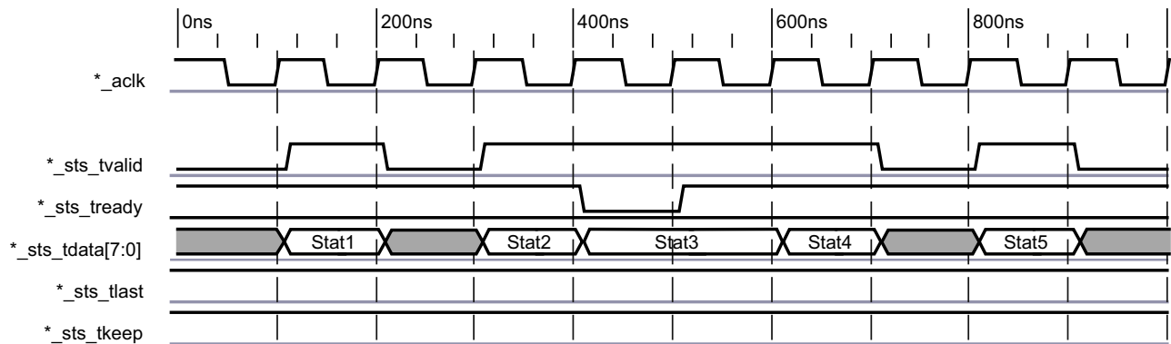
Figure 2-5: Reading Status over the Status Interface
