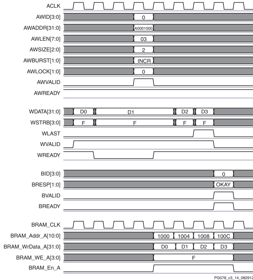
Figure 3-14: AXI Delayed Write Address
