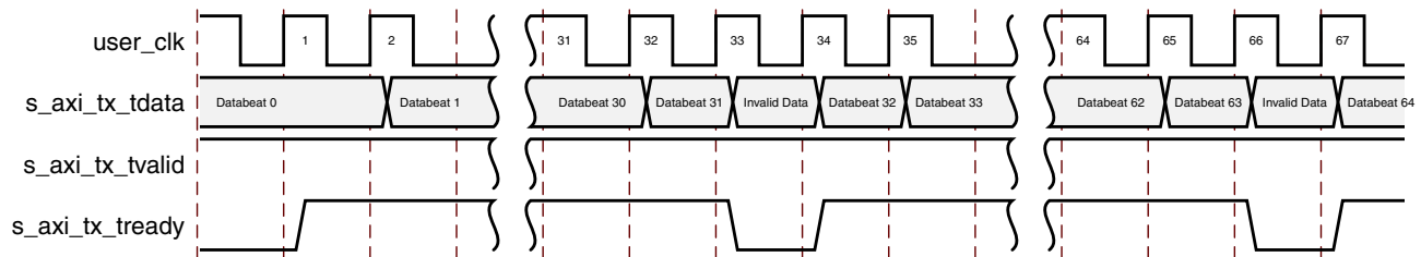
Figure 2-12: Framing Efficiency
