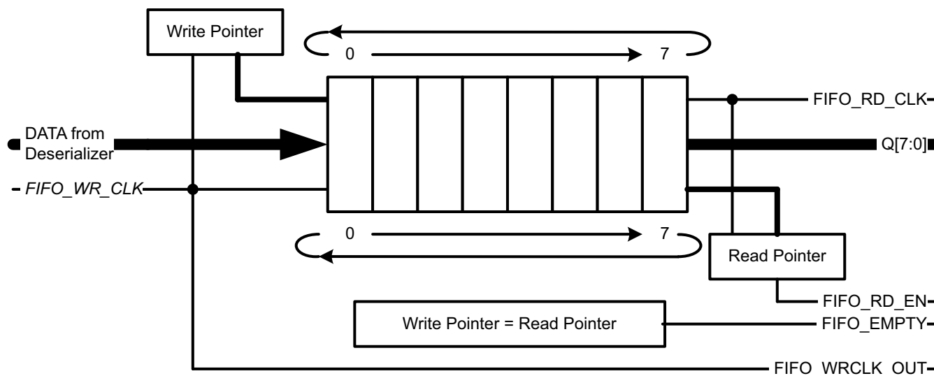
Figure 2-36: Schematic View of a Receiver FIFO
