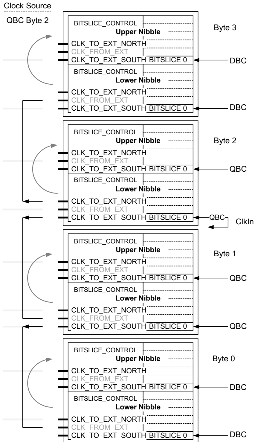
Figure 2-70: Combination of Inter-Nibble and Inter-Byte Clocking
