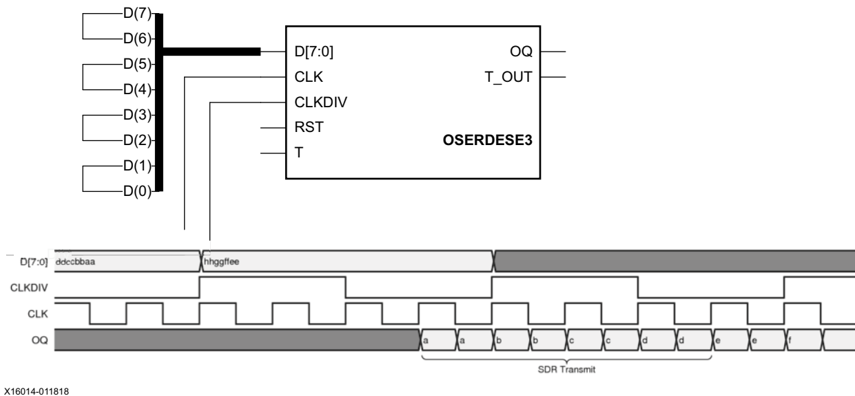
Figure 2-15: OSERDES Used in x4 SDR Mode (DATA_WIDTH = 8)
