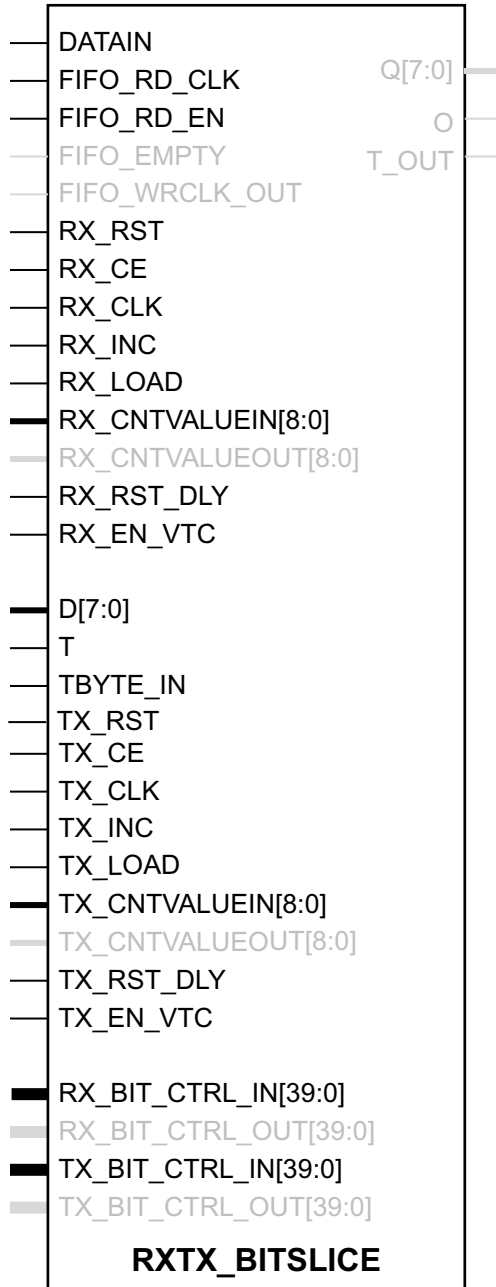
Figure 2-45: RXTX_BITSLICE Primitive
