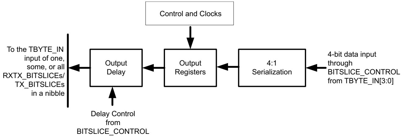
Figure 2-52: TX_BITSLICE_TRI Block Diagram
