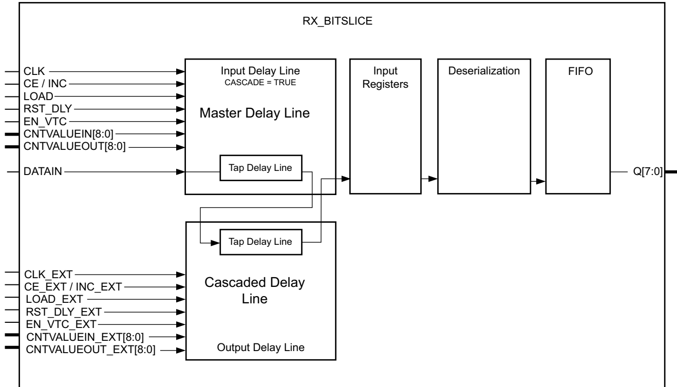
Figure 2-49: Extended Delay Control Signals
