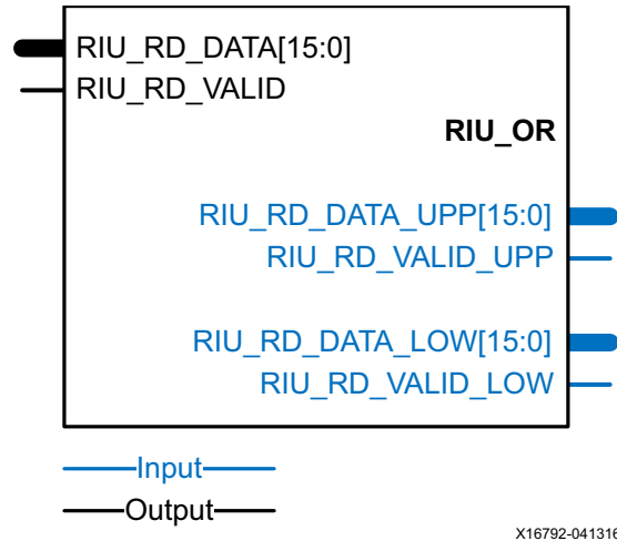
Figure 2-75: RIU Primitive
