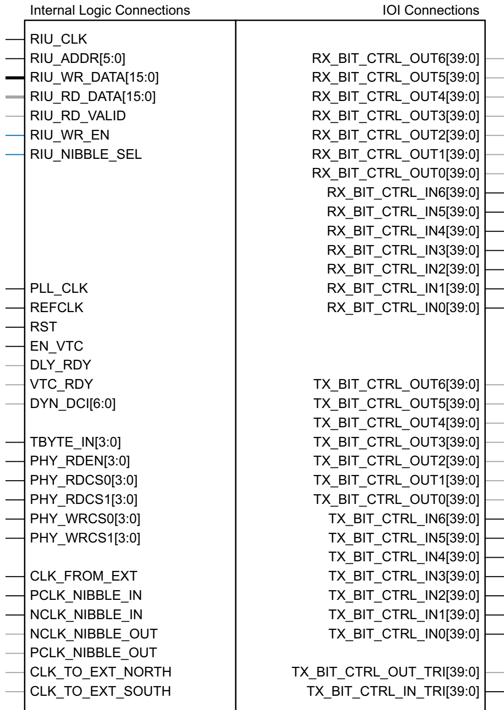
Figure 2-60: BITSlice_CONTROL Primitive
