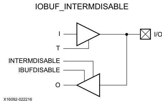
Figure 1-32: Bidirectional Buffer with Input Path Disable and On-Die Input Termination Disable (IOBUF_INTERMDISABLE)
