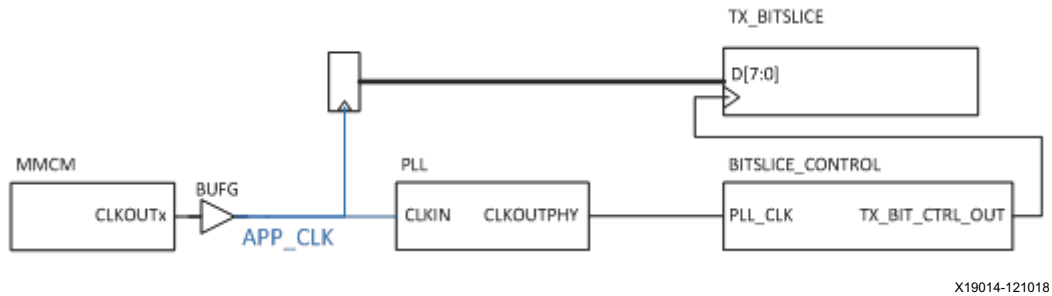
Figure 2-62: TX_BITSLICE Application Clock
