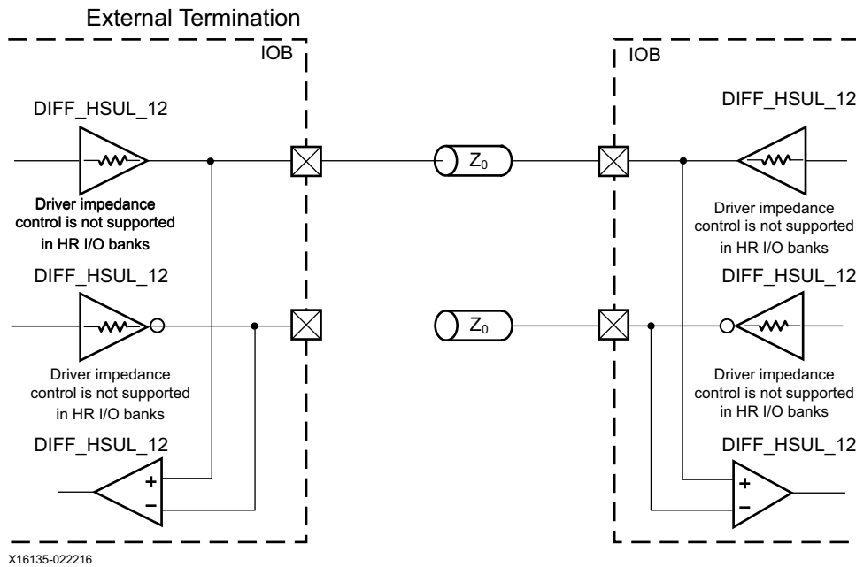
Figure 1-75: Differential HSUL_12 with Bidirectional Signaling
