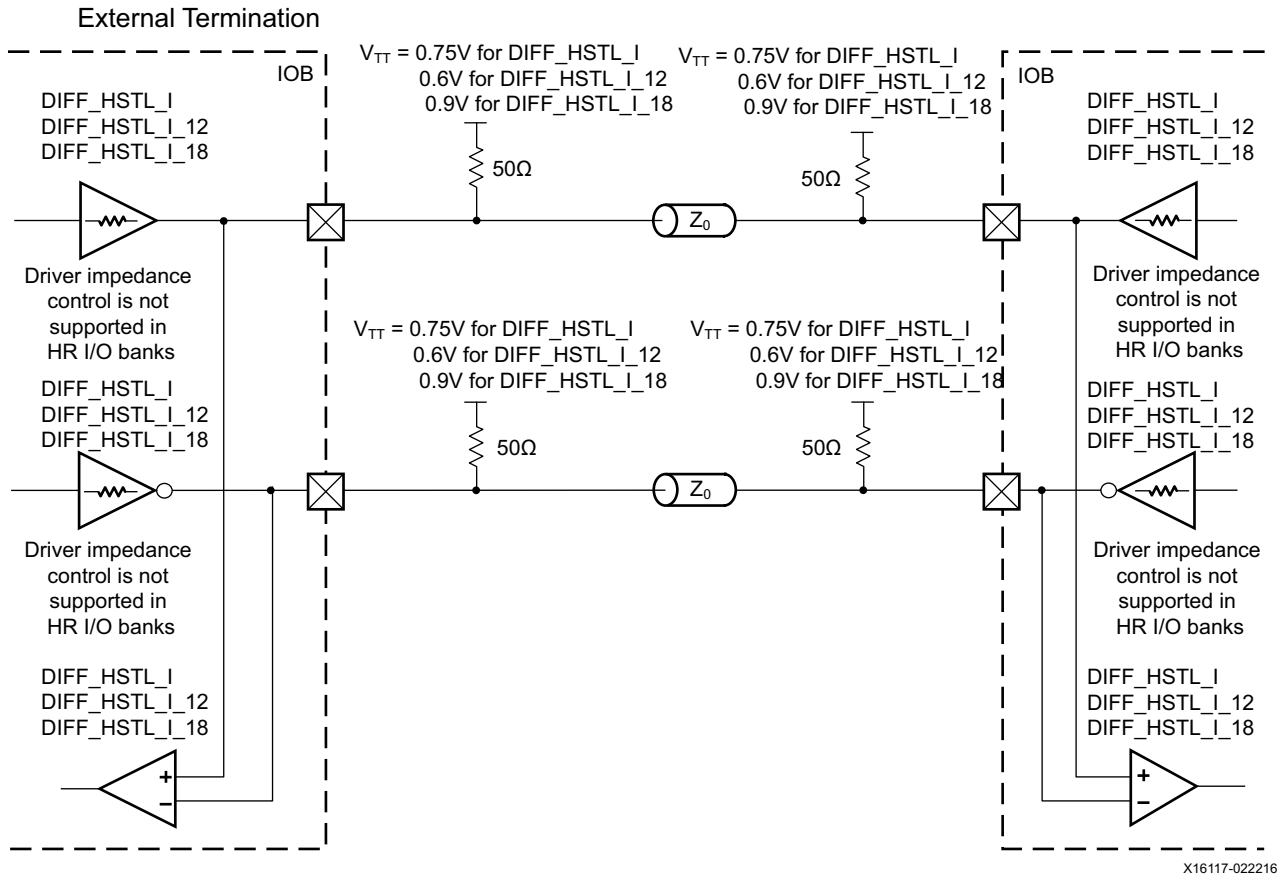
Figure 1-57: Differential HSTL Class I (1.2V, 1.5V, or 1.8V) Bidirectional Termination
