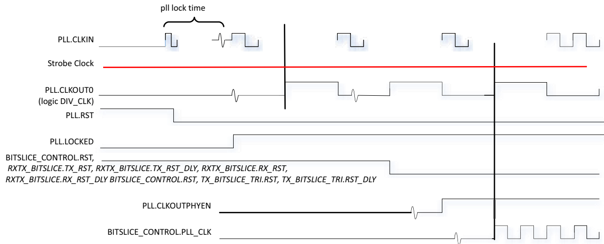
Figure 2-61: PLL and Reset Bring-up Sequence
