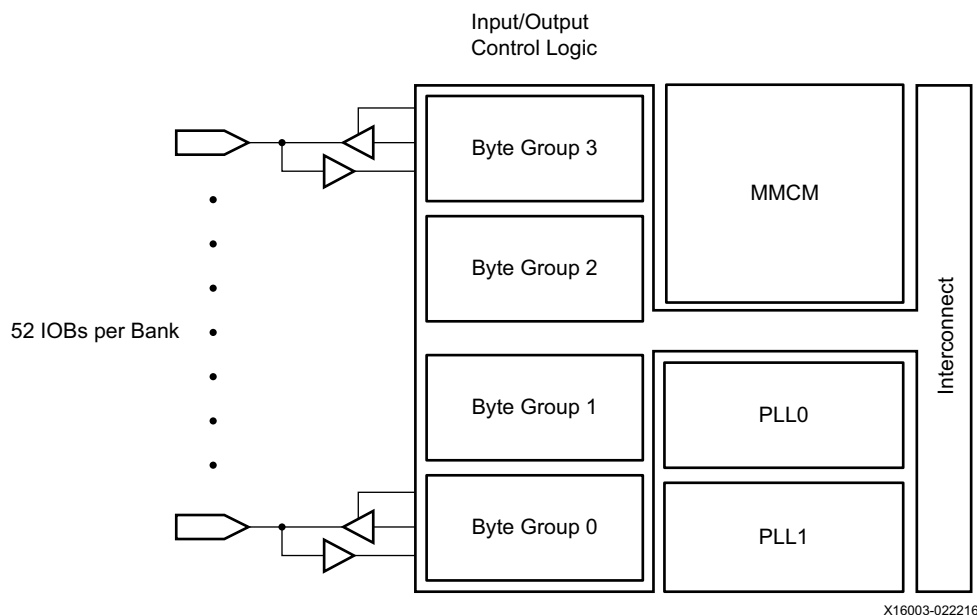
Figure 2-1: Bank Overview
