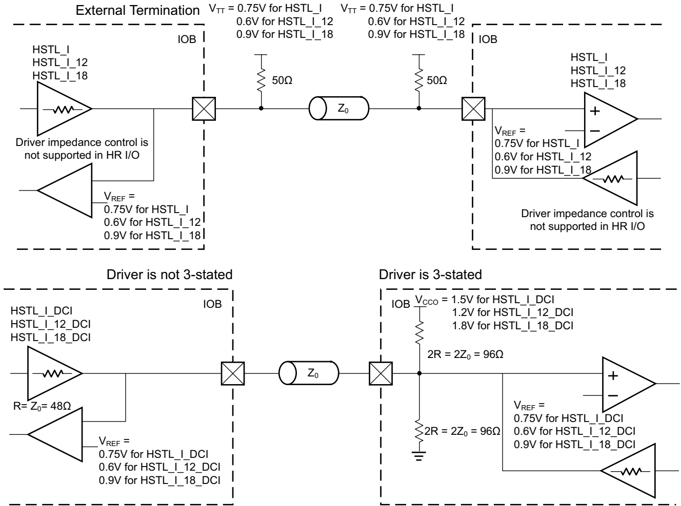
Figure 1-55: HSTL Class I (1.2V, 1.5V, or 1.8V) Bidirectional Termination
