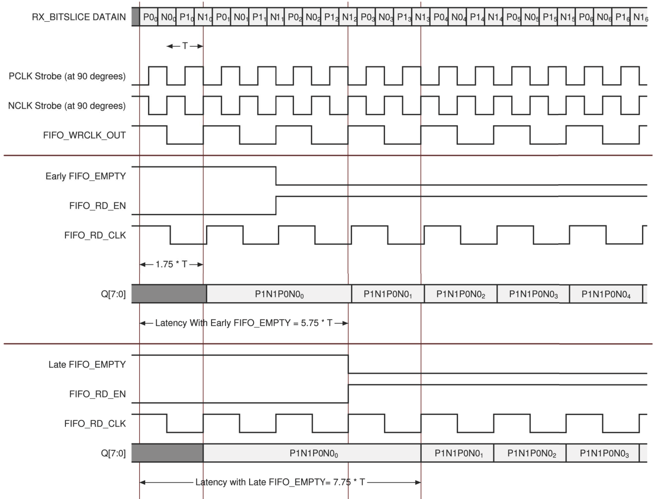
Figure 2-39: RX_BITSLICE FIFO, DATA_WIDTH = 4
