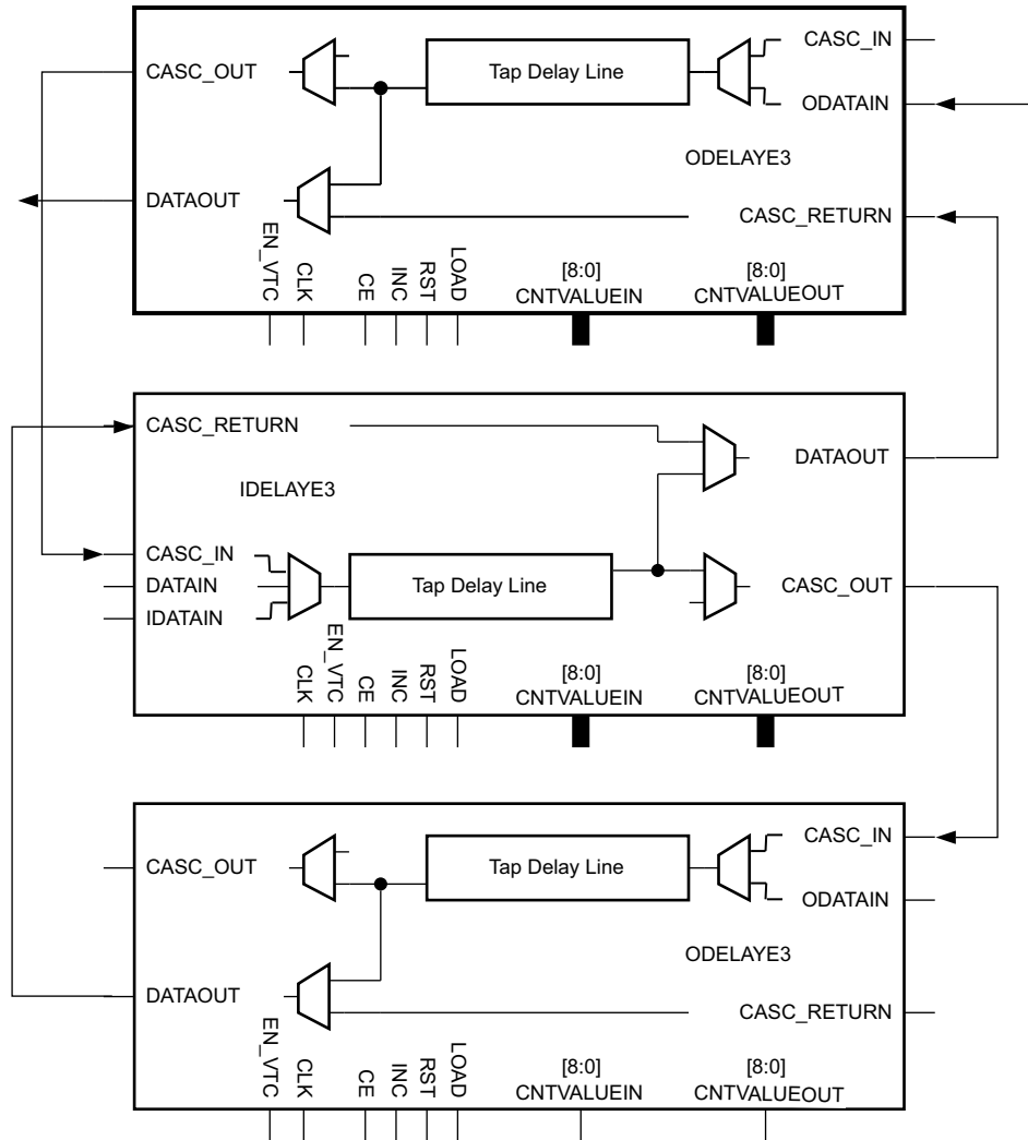
Figure 2-24: ODELAYE3 Cascading to Three Delays
