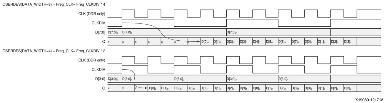
Figure 2-14: OSERDES Latency
