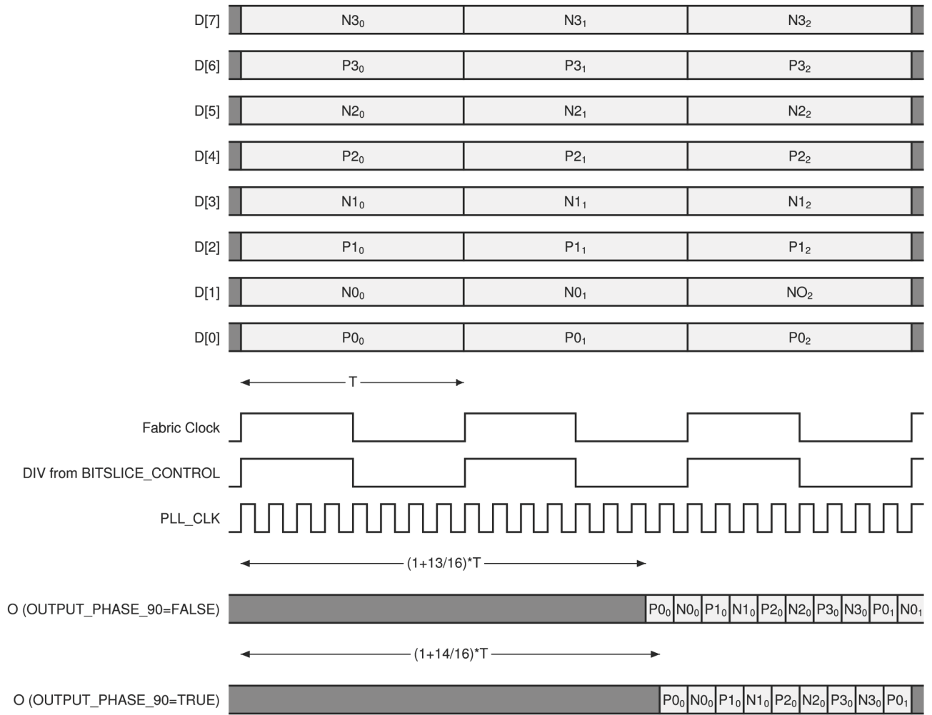
Figure 2-41: TX_BITSLICE Latency, DATA_WIDTH = 8
