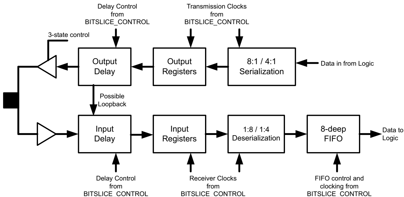
Figure 2-32: RXTX_BITSLICE Block Diagram
