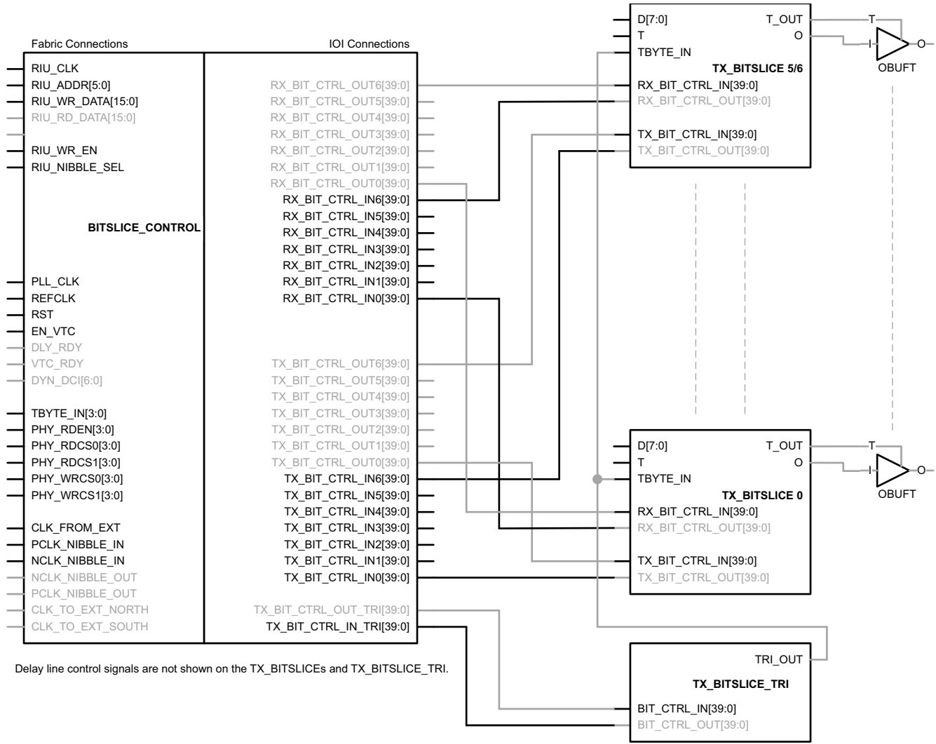
Figure 2-54: Connections for a 3-State Path when Using the TBYTE Port
