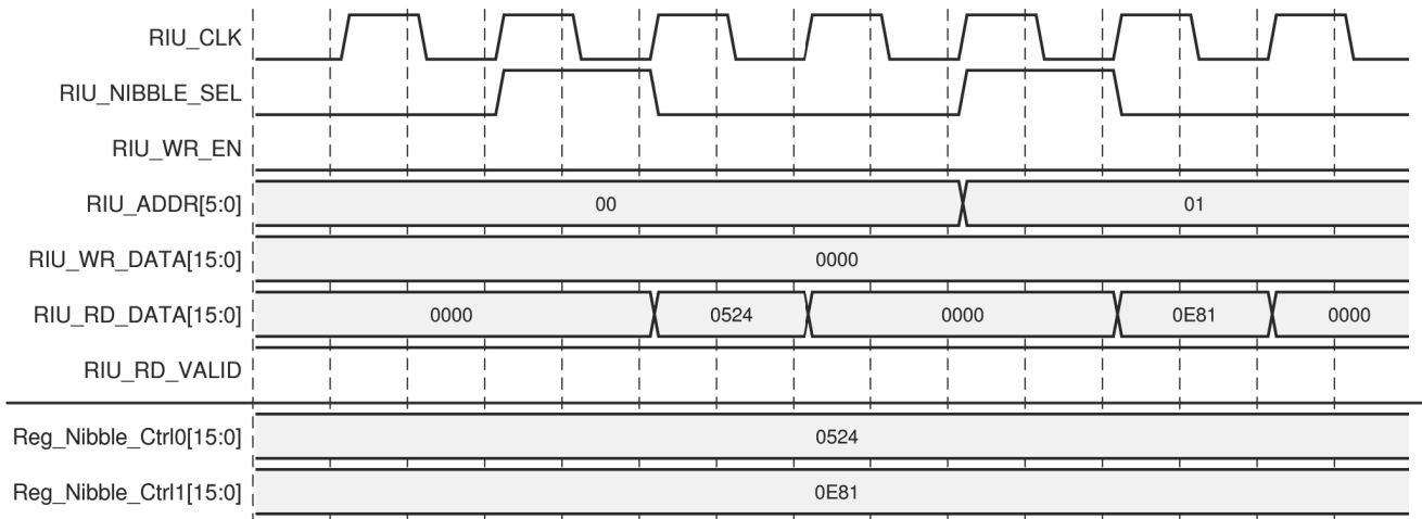
Figure 2-78: RIU Read
