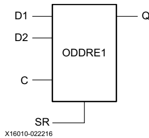
Figure 2-9: ODDRE1 Primitive Block Diagram
