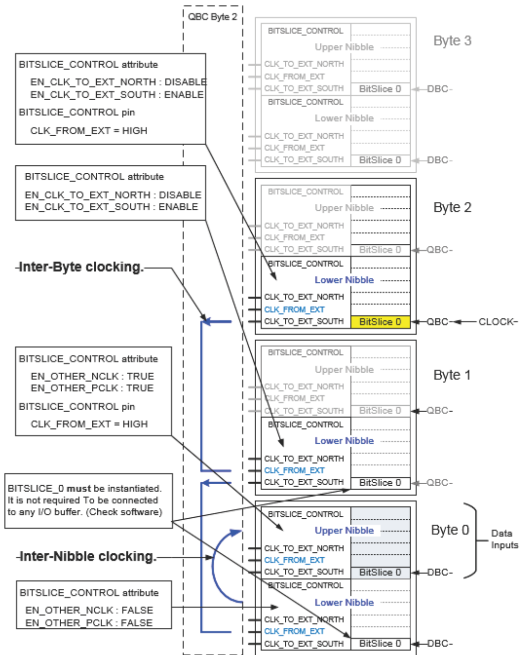
Figure 2-71: Inter-byte Clocking with BITSlice_0 Bypass
