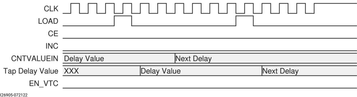
Figure 2-20: VAR_LOAD Mode Using COUNT as DELAY_FORMAT
