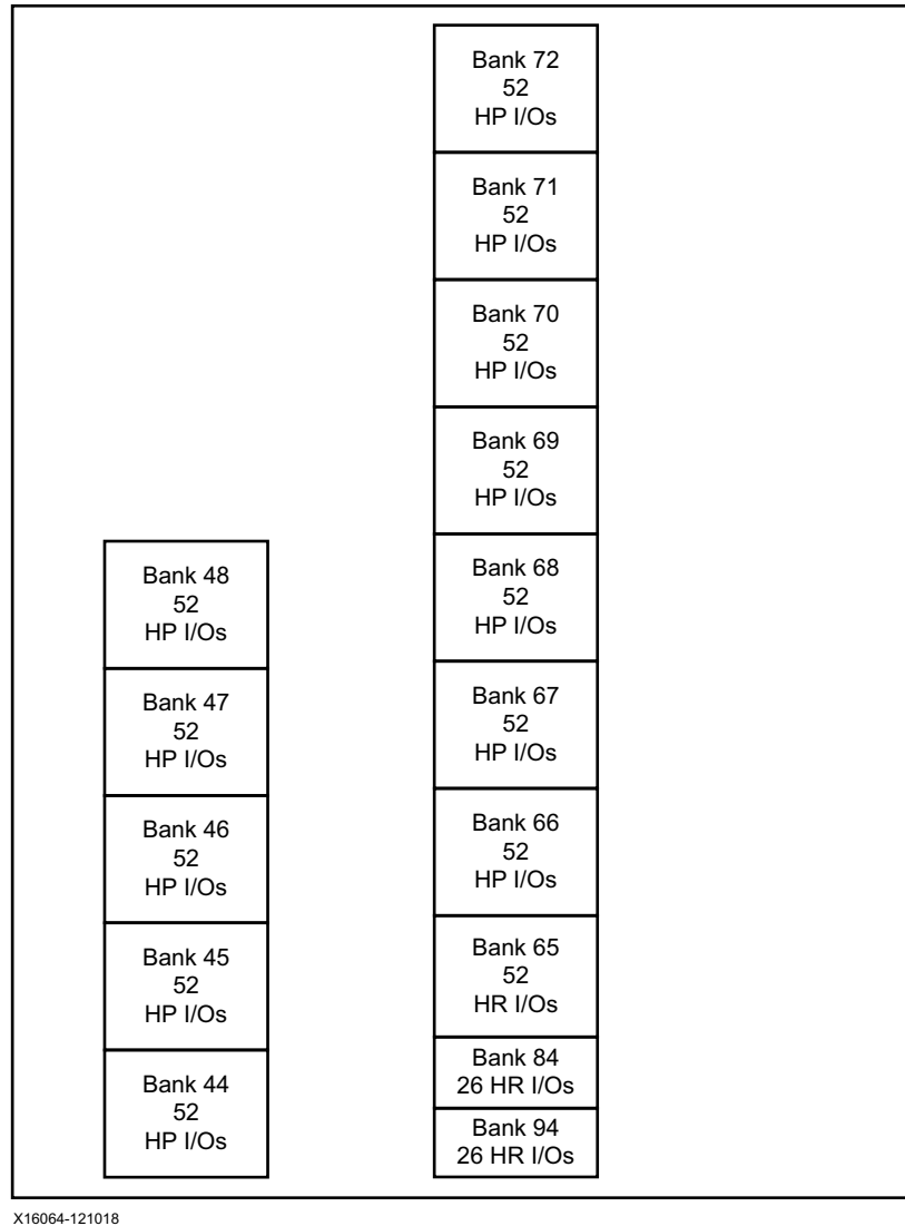
Figure 1-6: Example I/O Banks
