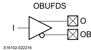
Figure 1-42: Differential Output Buffer Primitive (OBUFDS)
