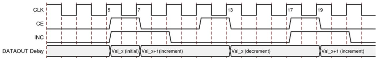
Figure 2-34: Variable Mode, UPDATE_MODE = ASYNC
