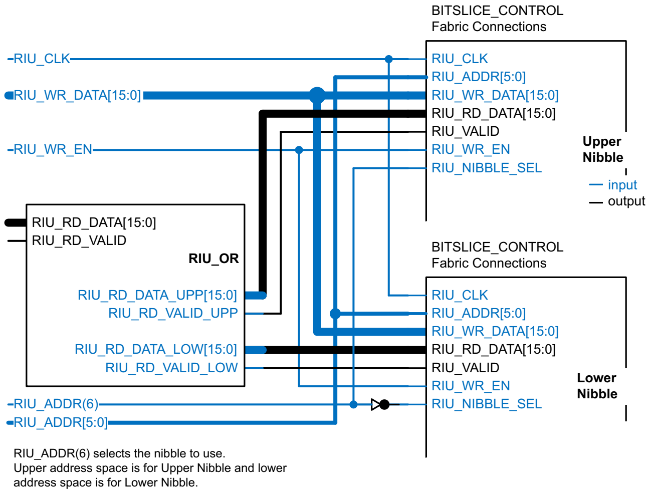
Figure 2-76: RIU_OR Combining Two RIU Ports
