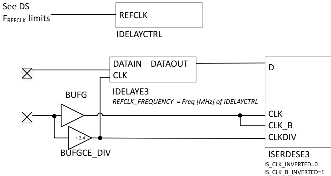
Figure 2-29: Clocking Connections for ISERDES with IDELAY (TIME Mode)
