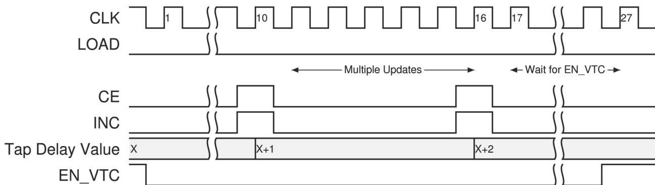
Figure 2-25: Variable Mode, UPDATE_MODE = ASYNC
