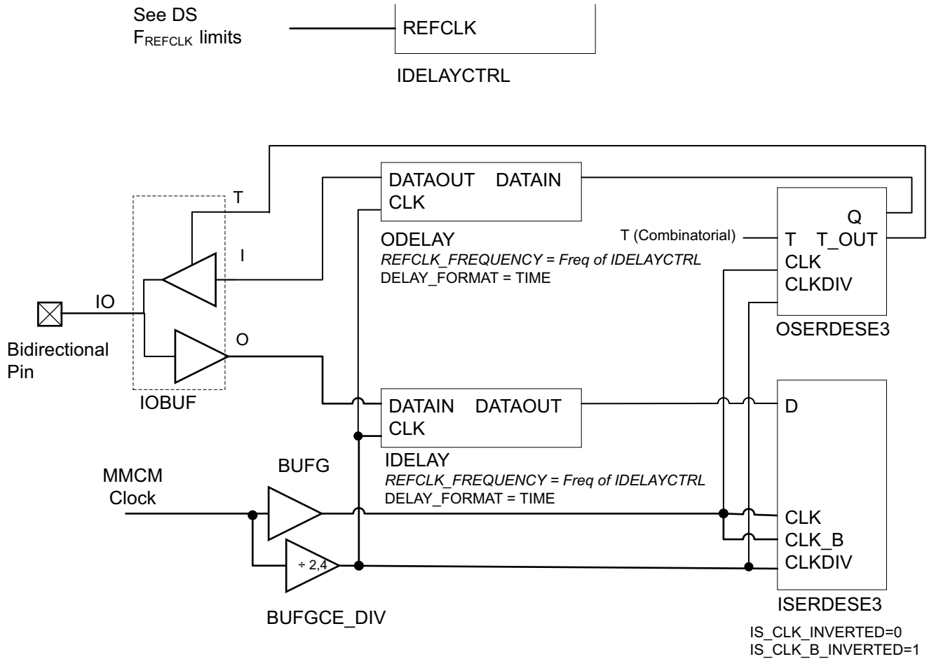
Figure 2-30: Bidirectional Signaling Using IDELAY/ODELAY with ISERDES and OSERDES
