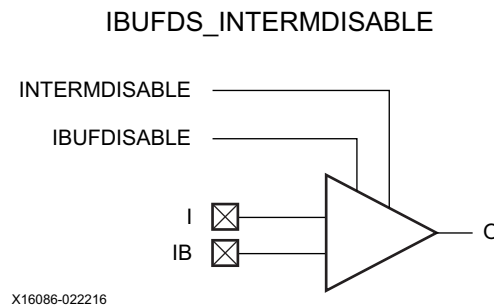
Figure 1-27: Differential Input Buffer with Input Buffer Disable and On-Die Input Termination Disable (IBUFDS_INTERMDISABLE)
