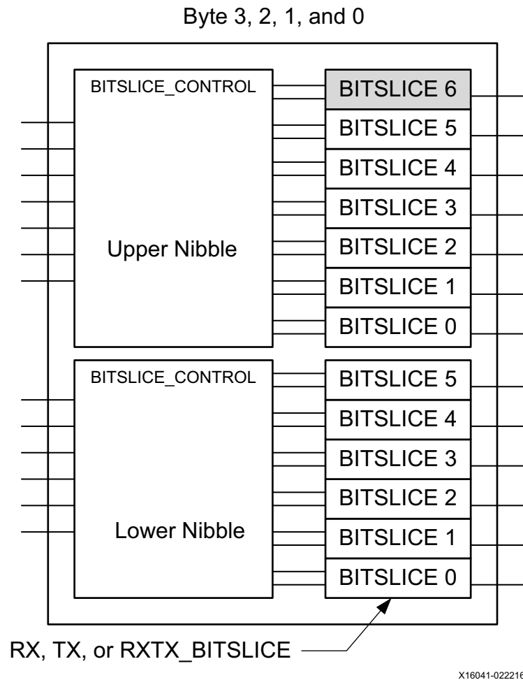
Figure 2-59: BITSLICE_CONTROL with Respect to Bit Slices
