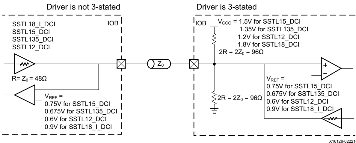
Figure 1-66: SSTL18_DCI, SSTL15_DCI, SSTL135_DCI, or SSTL12_DCI Bidirectional Termination
