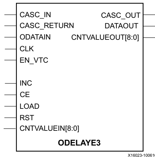
Figure 2-23: ODELAYE3 Primitive
