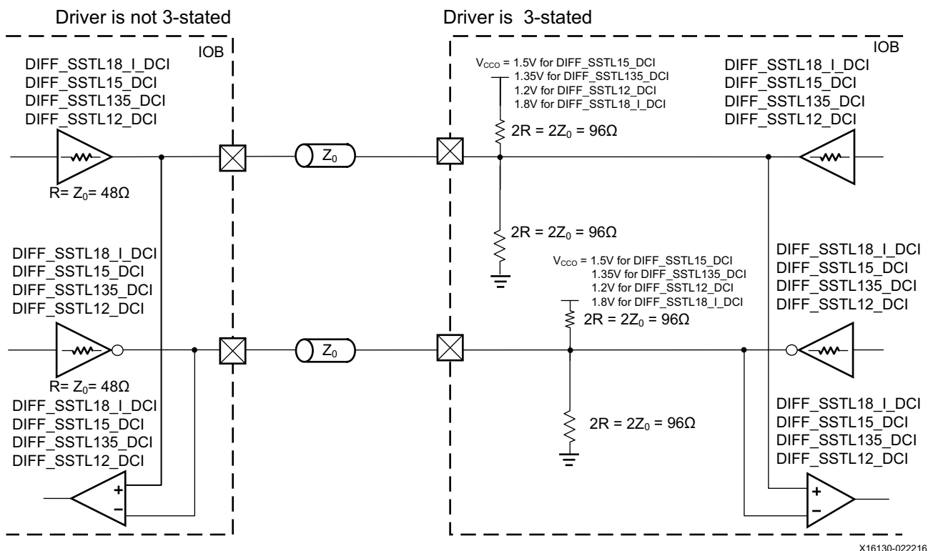
Figure 1-70: Differential SSTL18, SSTL15, SSTL135, or SSTL12 with Bidirectional DCI Termination
