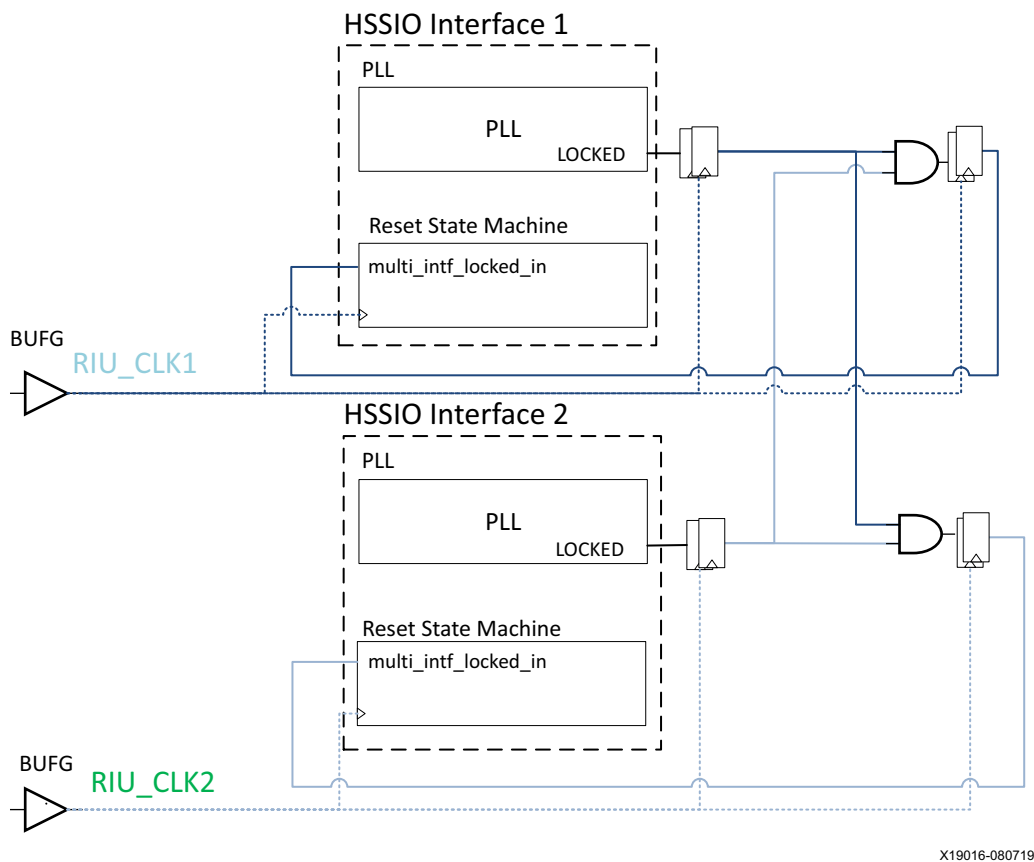
Figure 2-64: Multiple Interfaces in a Shared Bank
