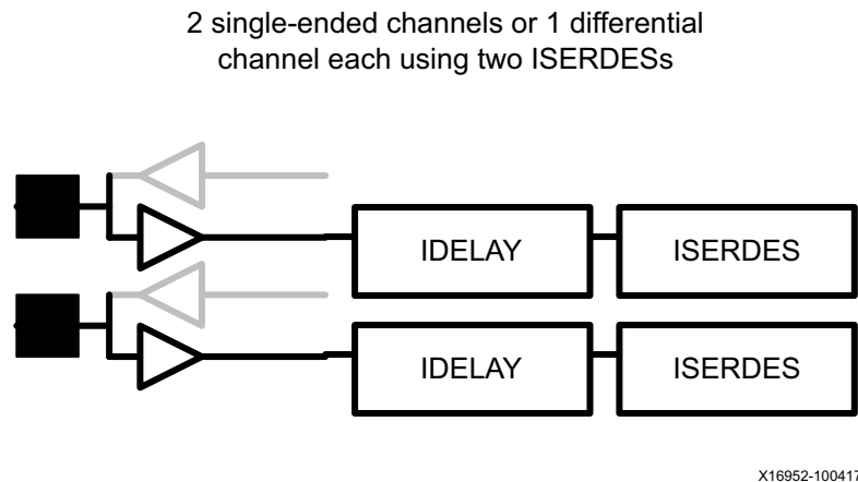
Figure 2-21: Two Single-ended or One Differential RX Channel
