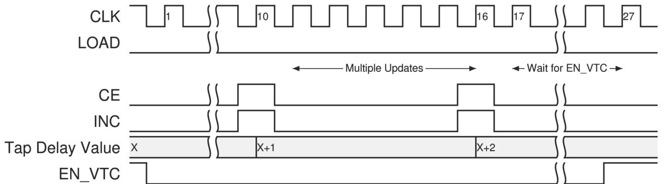
Figure 2-43: Variable Mode, UPDATE_MODE = ASYNC
