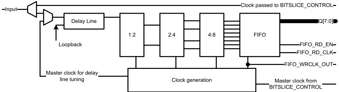
Figure 2-33: Receiver Block Diagram
