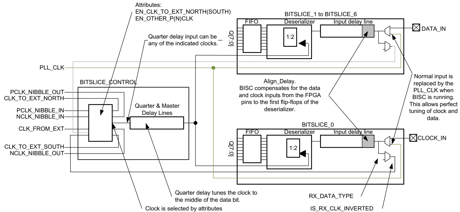
Figure 2-73: Delay Calibration by BISC
