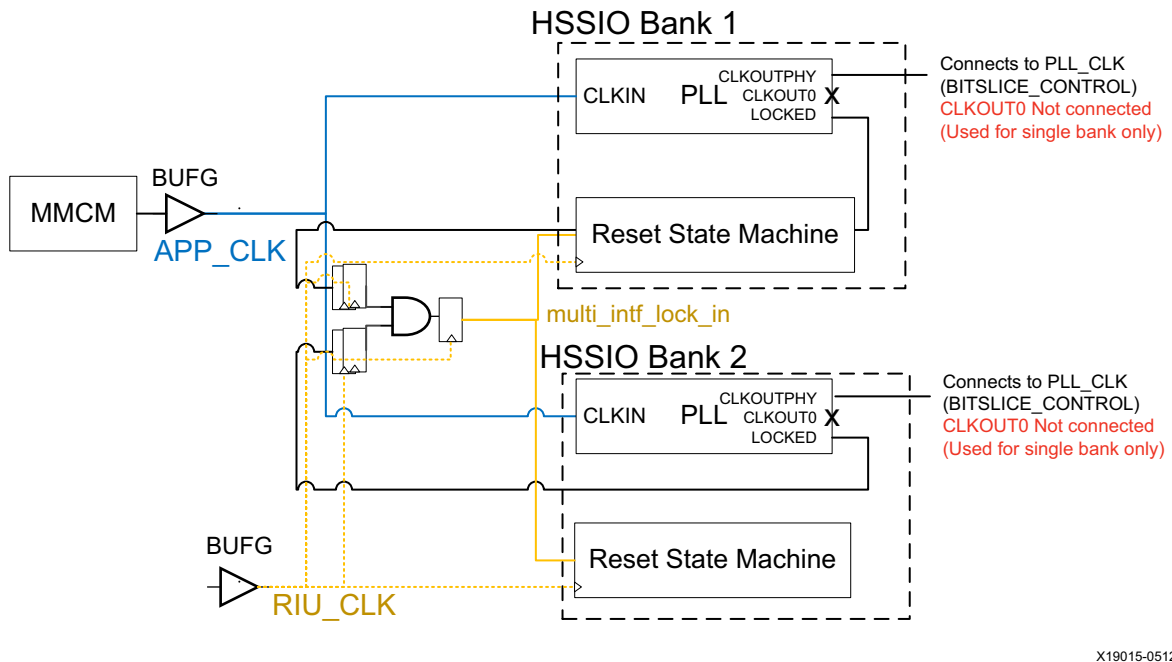
Figure 2-63: Multi-bank Clocking
