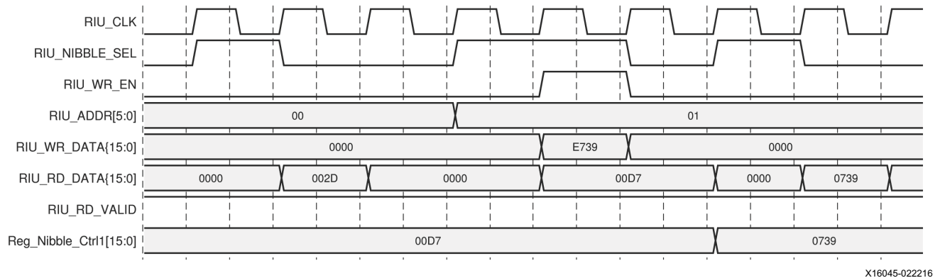
Figure 2-79: RIU Read Modify Write
