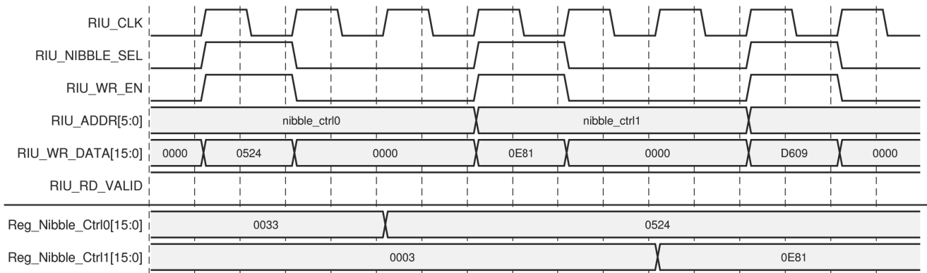
Figure 2-77: RIU Write
