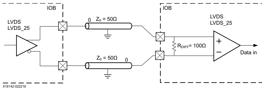
Figure 1-82: LVDS or LVDS_25 with DIFF_TERM Receiver Termination
