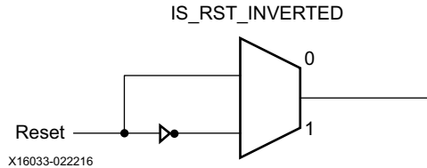
Figure 2-46: IS_RST_INVERTED Attribute
