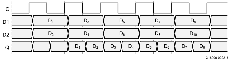
Figure 2-8: Output DDR Timing
