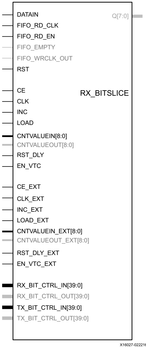
Figure 2-48: RX_BITSLICE Primitive
