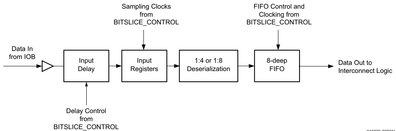
Figure 2-47: RX_BITSLICE Block Diagram
