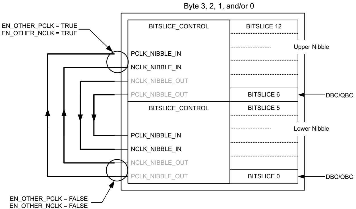
Figure 2-68: Inter-Nibble Clocking
