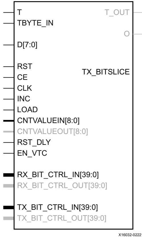
Figure 2-51: TX_BITSLICE Primitive
