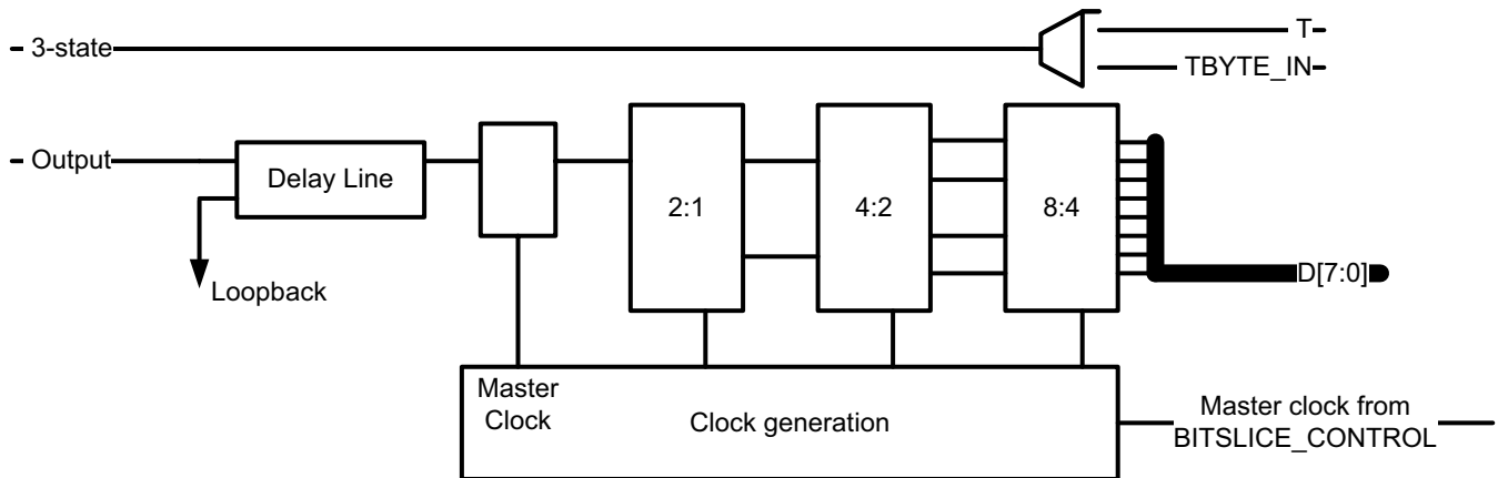
Figure 2-40: RXTX_BITSLICE Transmitter Block Diagram
