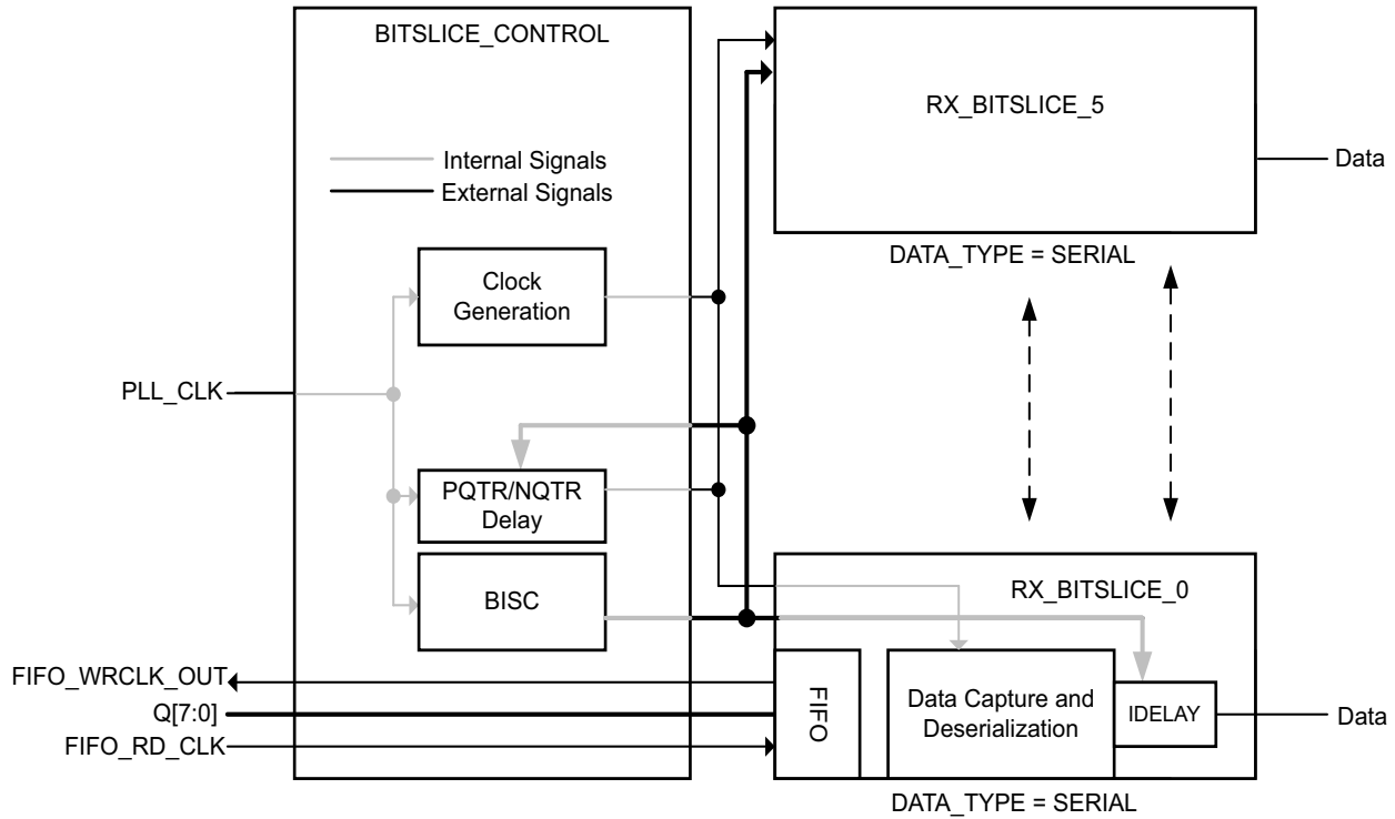
Figure 2-65: Data Capture in Serial Mode
