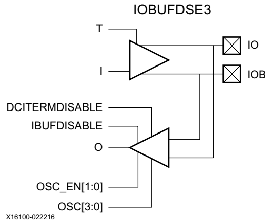
Figure 1-40: IOBUFDSE3 Primitive—Differential Bidirectional I/O Buffer with Offset Calibration (HP I/O Banks Only)
