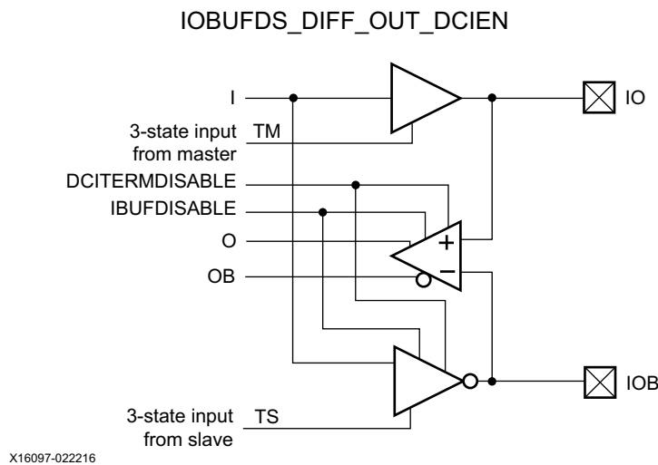
Figure 1-37: Differential Bidirectional Buffer with Complementary Outputs, Input Path Disable, and On-Die Input Termination Disable (IOBUFDS_DIFF_OUT_DCIEEN)
