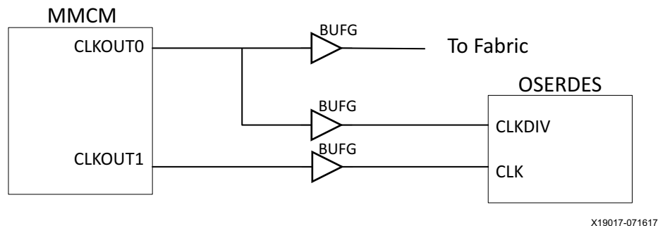
Figure 2-28: MMCM with Separate Clock Outputs
