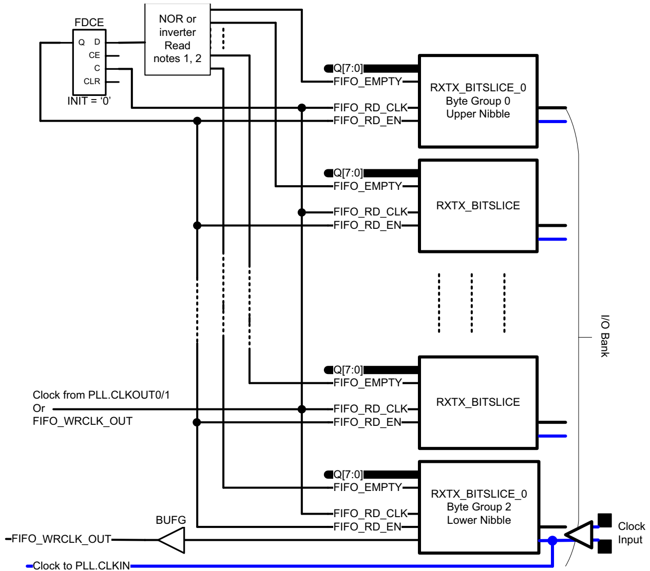
Figure 2-37: FIFO as Bit Slice Output Synchronizer (Multiple Clocks or Strokes)
