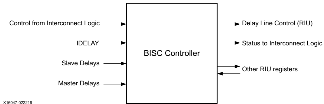
Figure 2-72: Block Diagram of the BISC Controller and Connections
