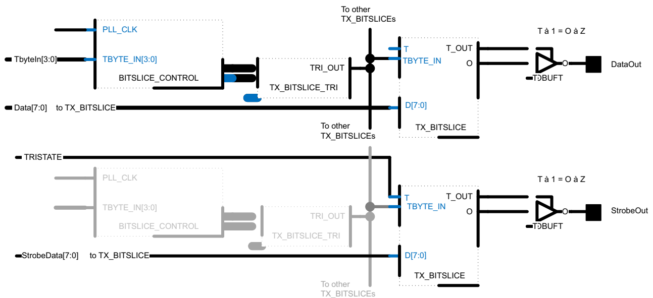
Figure 2-56: Using the TBYTE_CTL Attribute Settings TBYTE_IN or T
