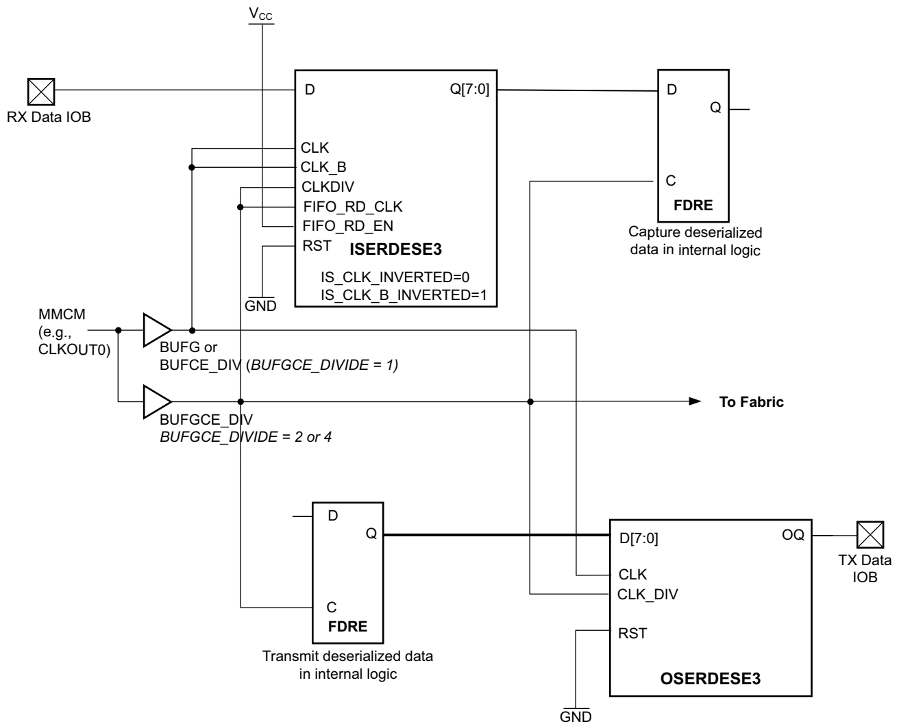
Figure 2-27: Component Mode Clocking Circuit
