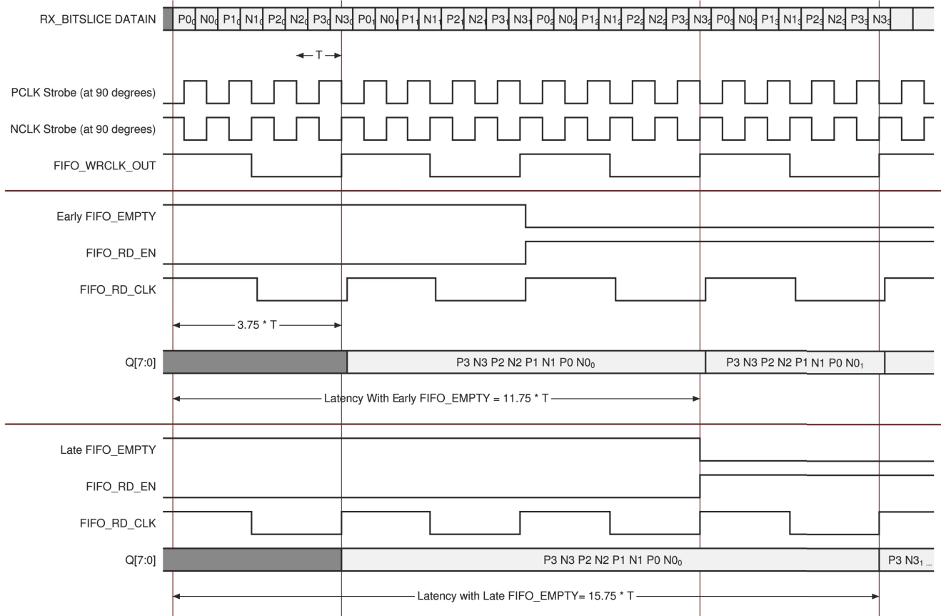
Figure 2-38: RX_BITSLICE FIFO, DATA_WIDTH = 8
