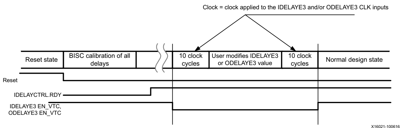
Figure 2-22: Changing Delay when DELAY_TYPE = VAR_LOAD
