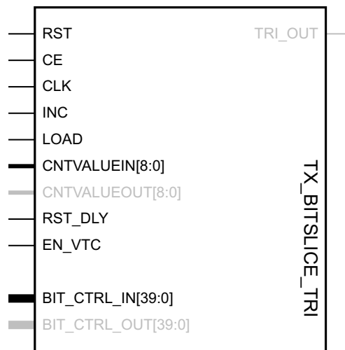
Figure 2-53: TX_BITSLICE_TRI Primitive
