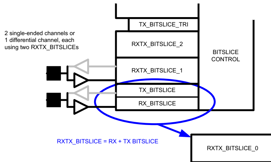
Figure 2-35: Two Single-Ended or One Differential RX Channel
