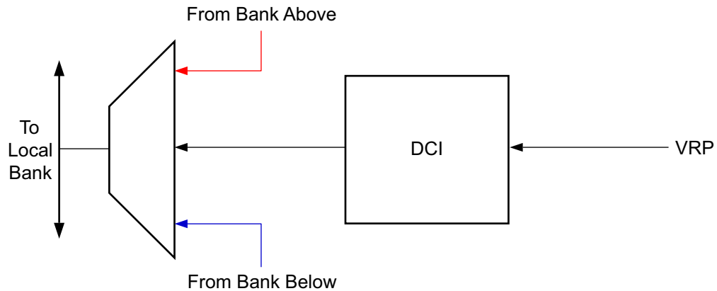
Figure 1-7: DCI Use within a Bank
