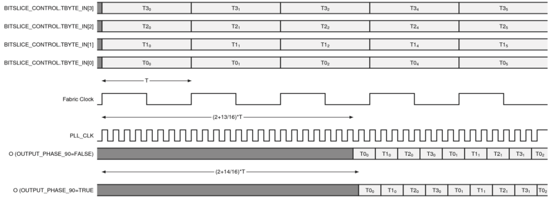
Figure 2-57: 3-State Latency, DATA_WIDTH = 8
