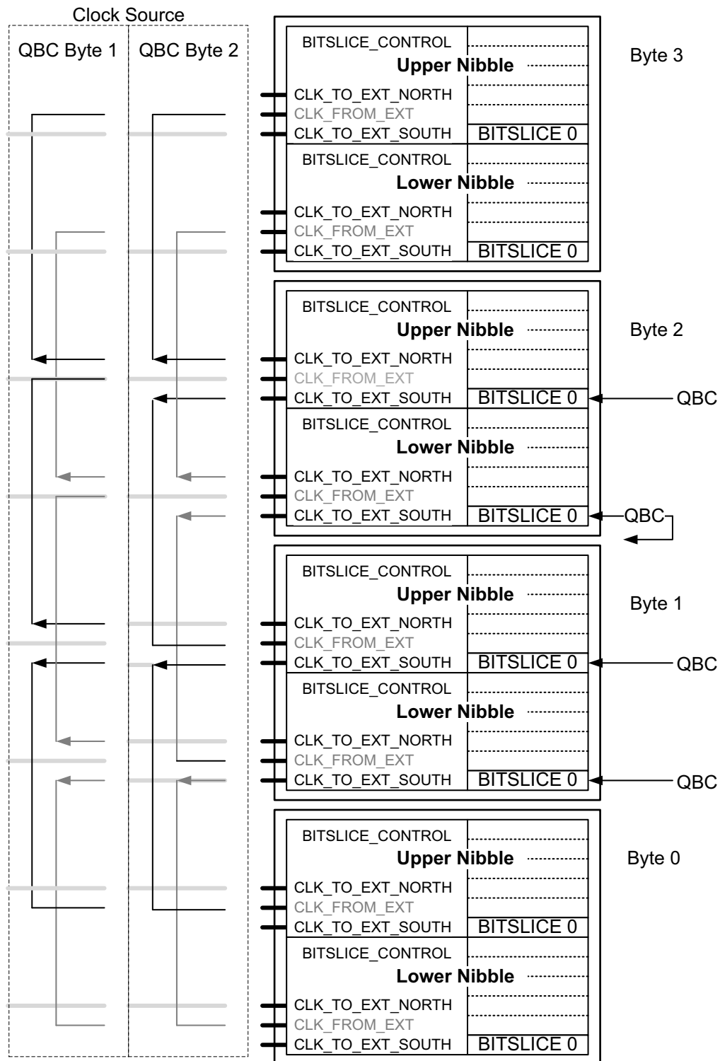
Figure 2-69: Inter-Byte Clocking
