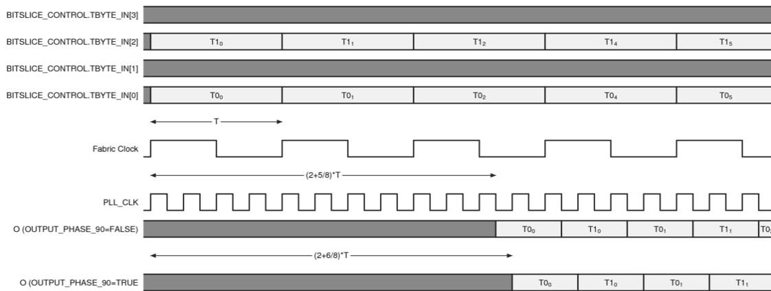
Figure 2-58: 3-State Latency, DATA_WIDTH = 4
