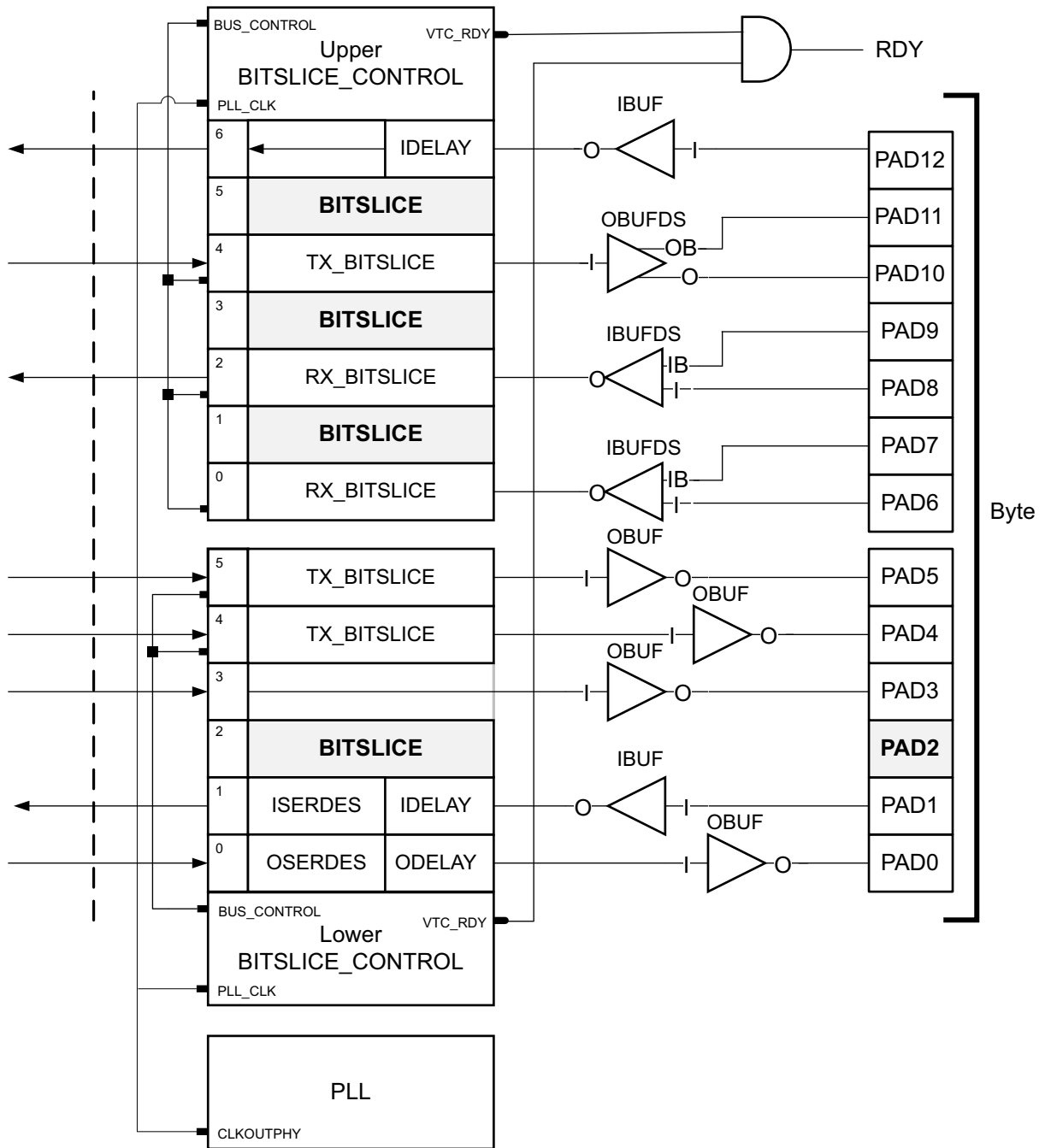
Figure 2-31: Example Mixed-Mode Byte
