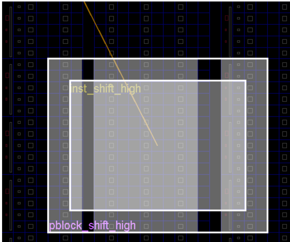
Figure 7-2: PU Aligned Pblock
