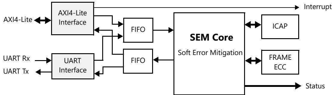
Figure 2-14: TMR SEM Block Diagram
