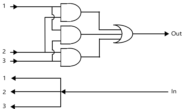
Figure 2-8: TMR Voter Logic in TMR Configuration
