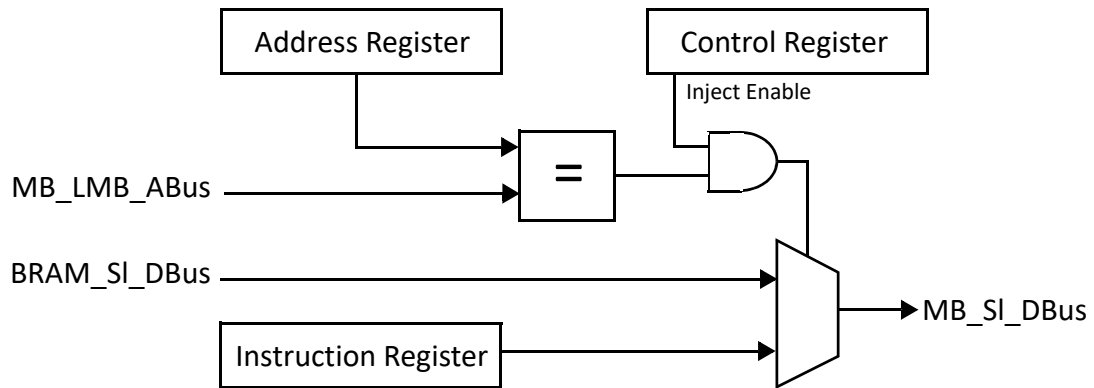
Figure 2-13: TMR Inject Block Diagram
