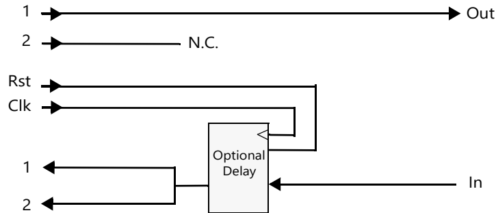
Figure 2-9: TMR Voter Logic in Lockstep Fail Safe Configuration
