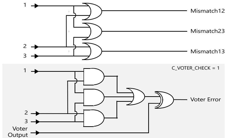
Figure 2-10: TMR Comparator Logic in TMR Configuration
