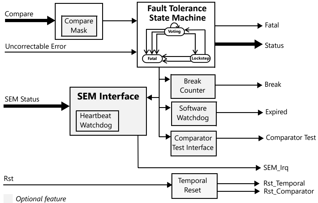
Figure 2-12: TMR Manager Block Diagram
