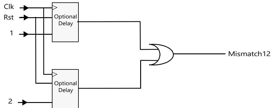
Figure 2-11: TMR Comparator Logic in Lockstep Fail Safe Configuration
