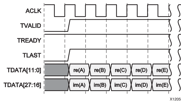
Figure 4-4: Complex Scalar Example with 32-Bit TDATA Signal
