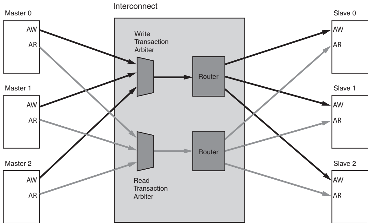
Figure 3-4: Shared Write and Read Address Arbitrations
