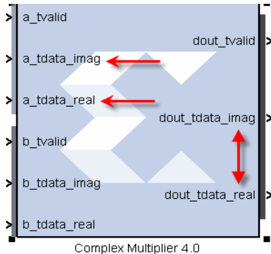
Figure 2-12: Multi-Channel TDATA
