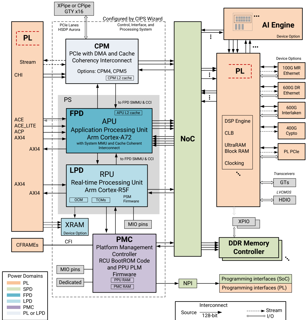
Figure 1: System-level Interconnect Architecture
