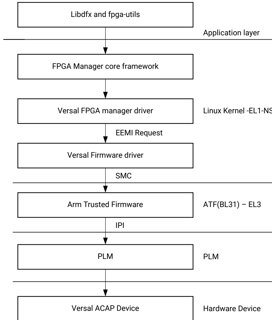
Figure 31: FPGA Programming Flow from Linux
