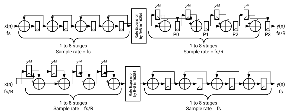
Figure 92: CIC Filter
