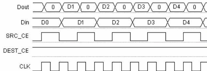
Figure 90: Up Sample Output
