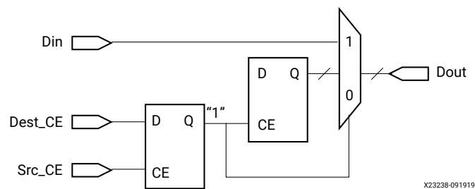
Figure 85: Zero Latency Vector Down Sample
