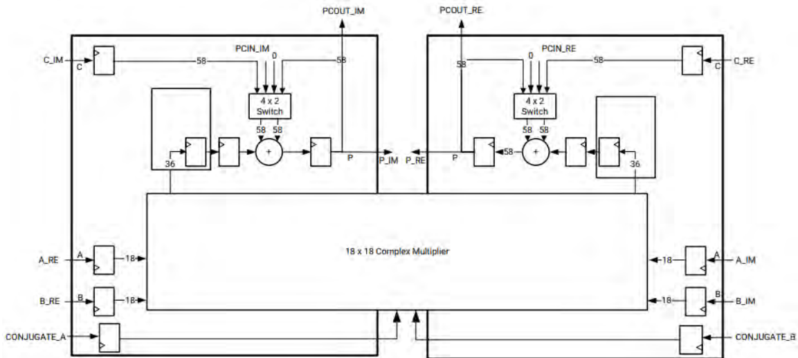
Figure 29: Unisim DSPCPLX Primitive
