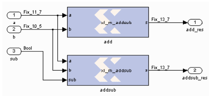
Figure 54: Two Blocks Using Same xl_m_addsub Function
