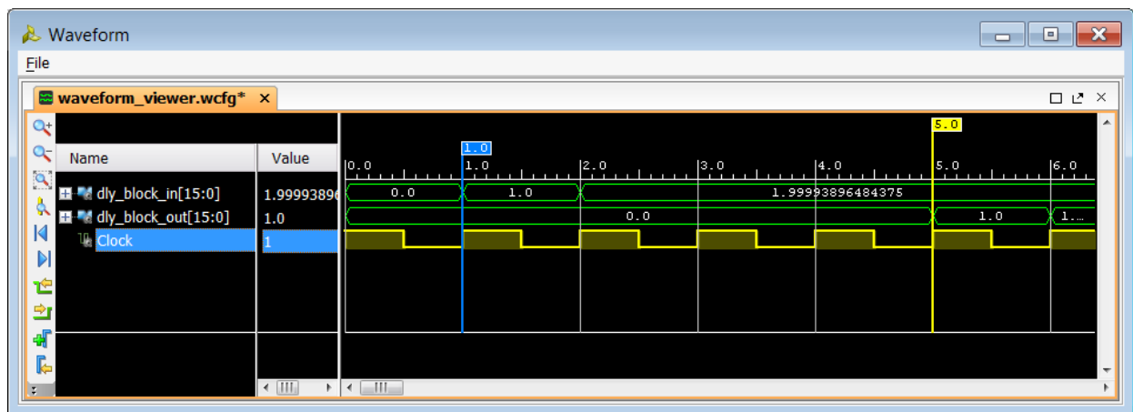
Figure 83: Vector Delay block behavior when L=4 and \text{Period}=1\text{s}
