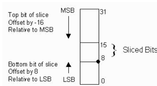
Figure 72: Extracting Top 16 and Bottom 8 Bits
