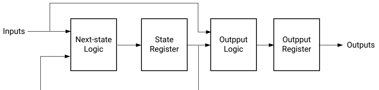
Figure 101: Mealy State Machine Block Diagram
