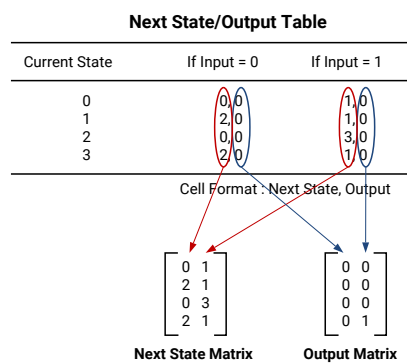
Figure 97: Next State Output Table
