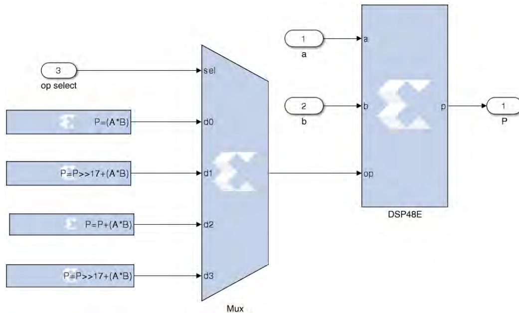
Figure 60: DSP48E Block
