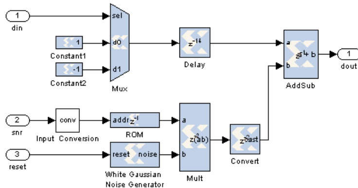
Figure 91: BPSK AWGN Channel Diagram
