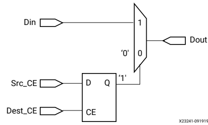
Figure 89: Zero Padding Up Sample Circuit
