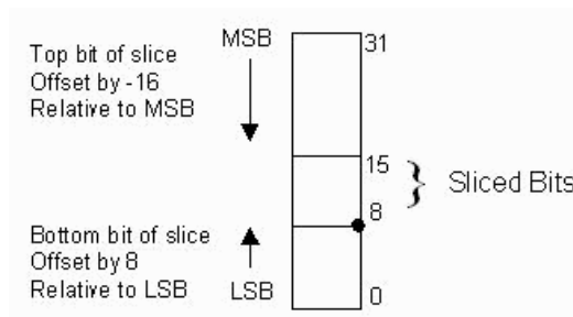
Figure 88: Extracting Top 16 and Bottom 8 Bits
