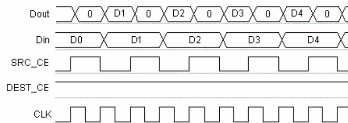
Figure 81: Up Sample Output
