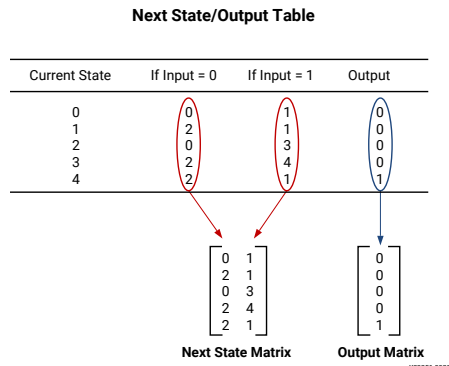
Figure 100: Next State Output Table
