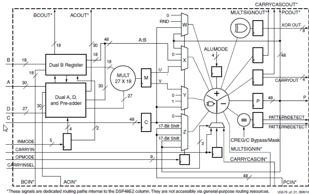
Figure 27: DSP48E2
