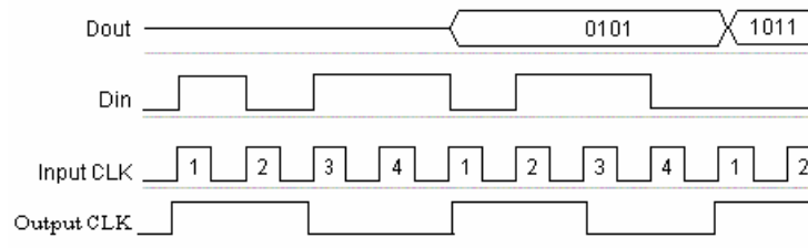
Figure 66: Serial to Parallel Behavior
