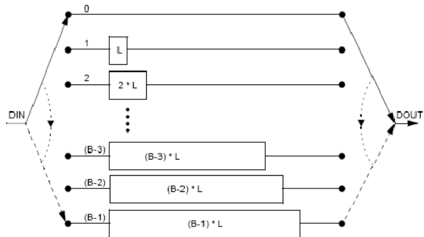
Figure 35: Interleaver
