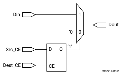
Figure 80: Zero Padding Up Sample Circuit
