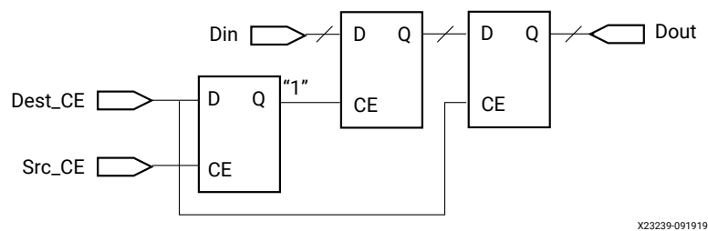
Figure 86: Two Register Example
