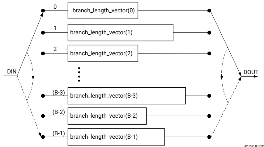
Figure 37: Interleaver/De-Interleaver
