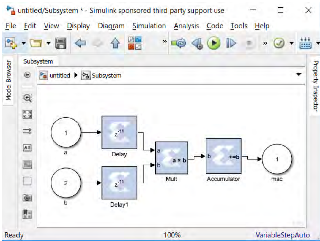
Figure 171: Generated Diagram
