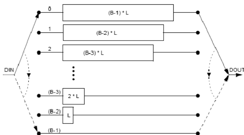
Figure 36: De-interleaver
