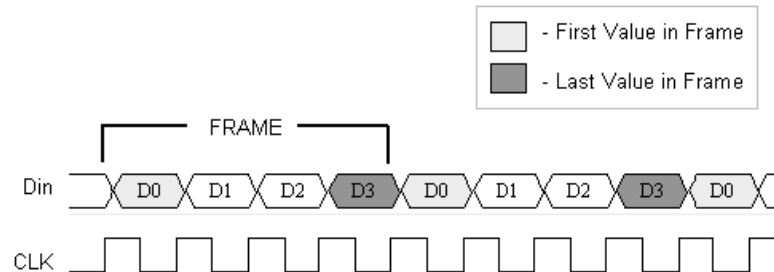
Figure 84: Vector Down Sample with Sampling Rate of 4
