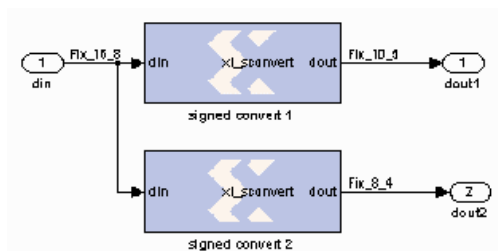
Figure 53: Block Diagram
