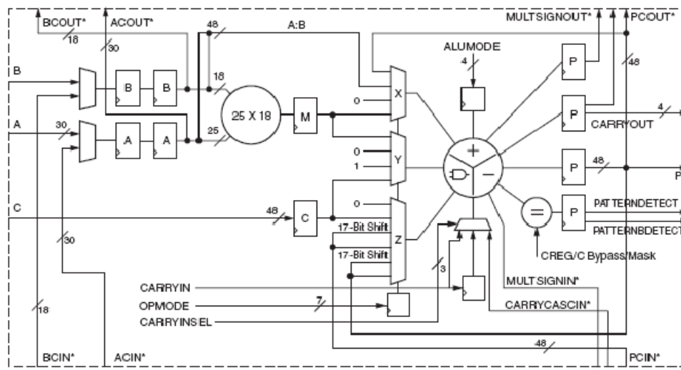
Figure 25: DSP48E
