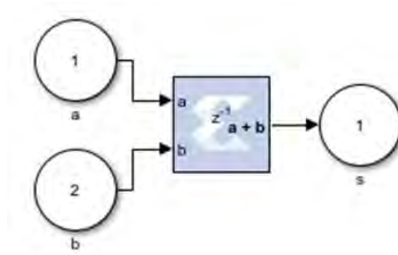
Figure 164: Subsystem Example
