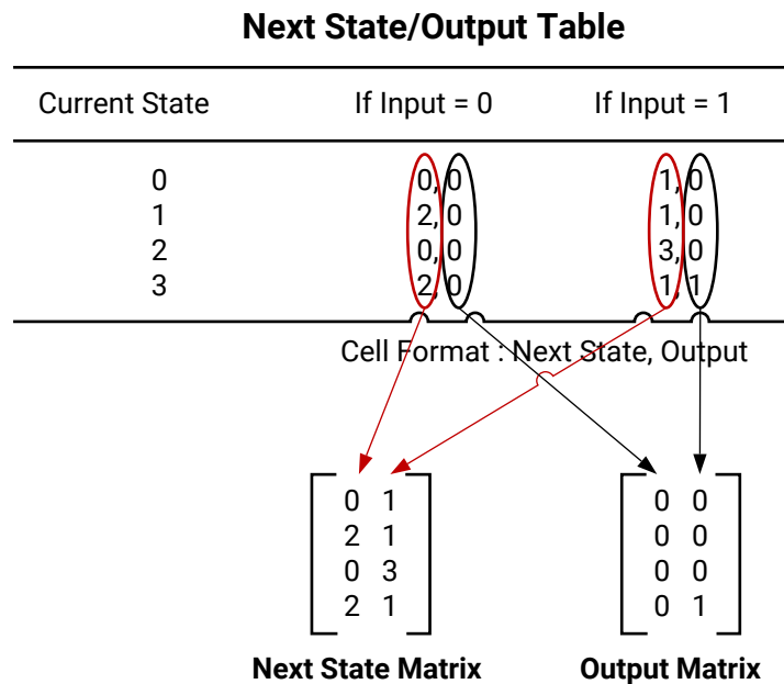
Figure 103: Next State Output Table
