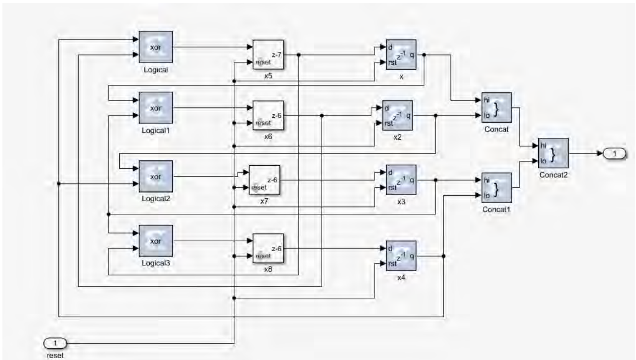
Figure 107: 4-bit Leap-Forward LFSR Diagram
