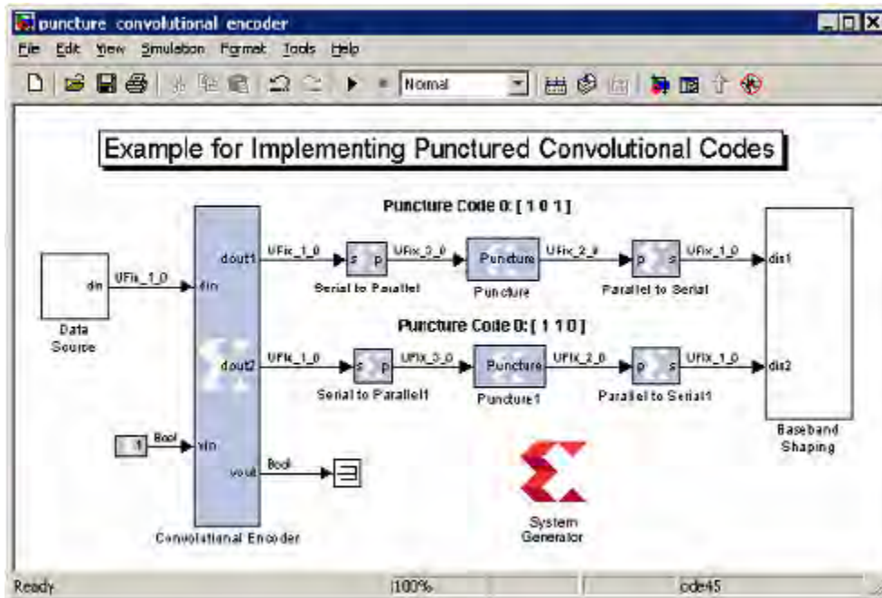
Figure 62: Implementing Punctured Convolutional Codes
