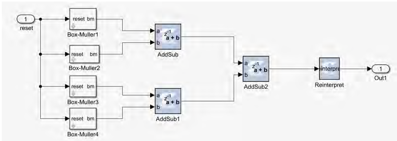
Figure 108: Box-Muller Method Diagram
