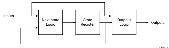
Figure 95: Mealy Machine Block Diagram
