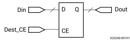
Figure 87: One Register Example
