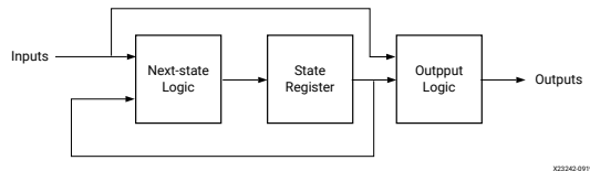
Figure 98: Moore State Machine Block Diagram
