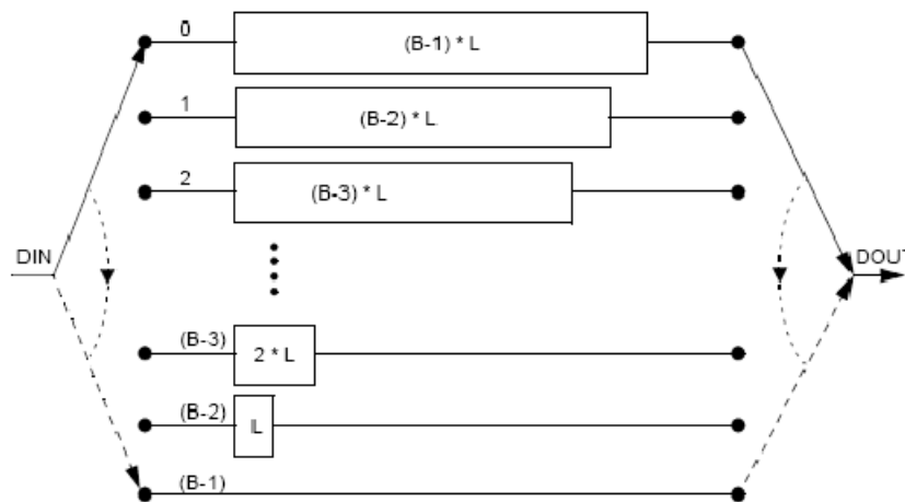
Figure 34: De-interleaver
