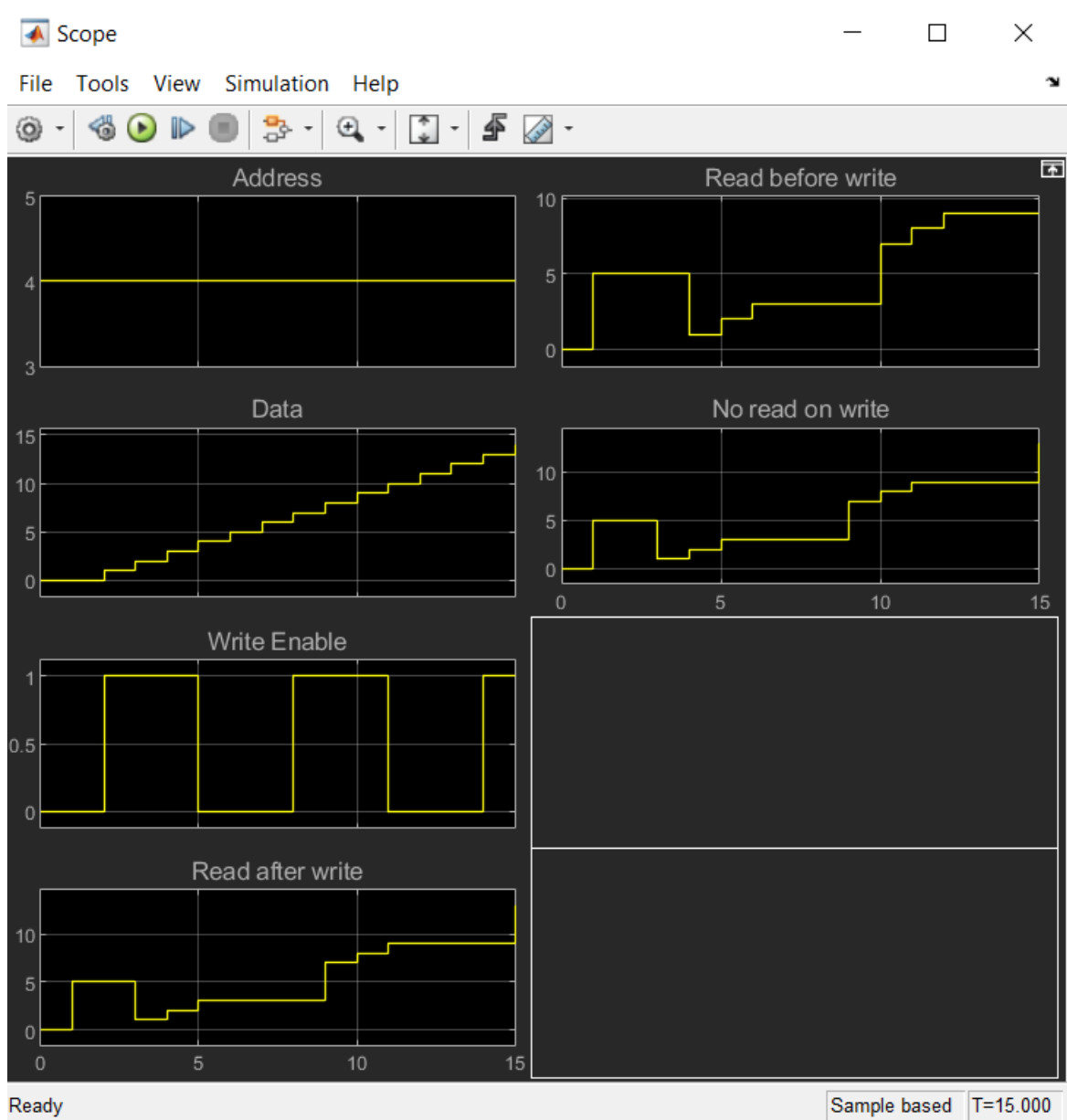
Figure 69: Write Output
