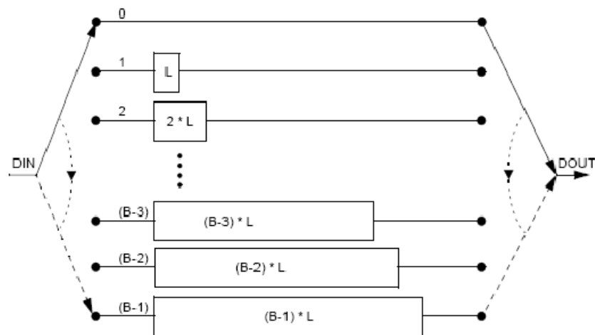
Figure 33: Interleaver
