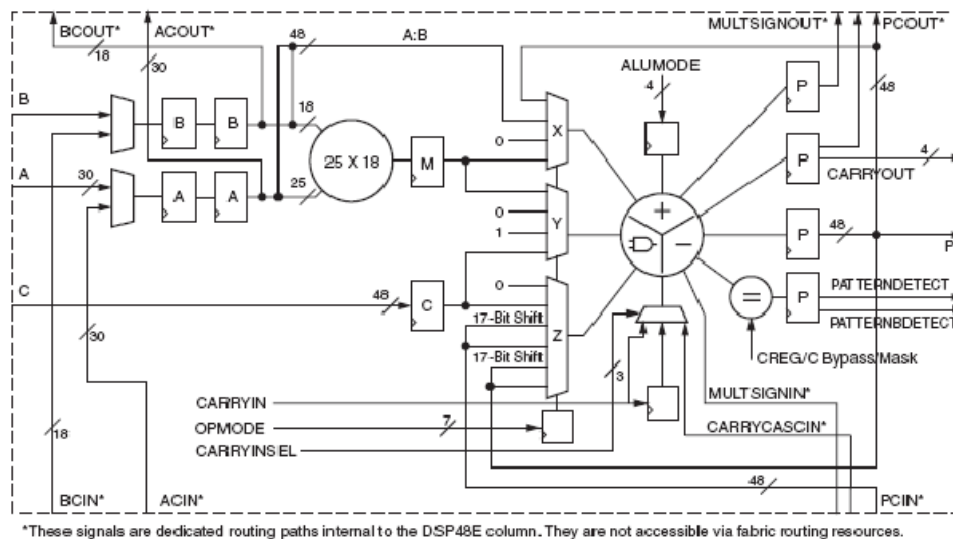
Figure 25: DSP48E
