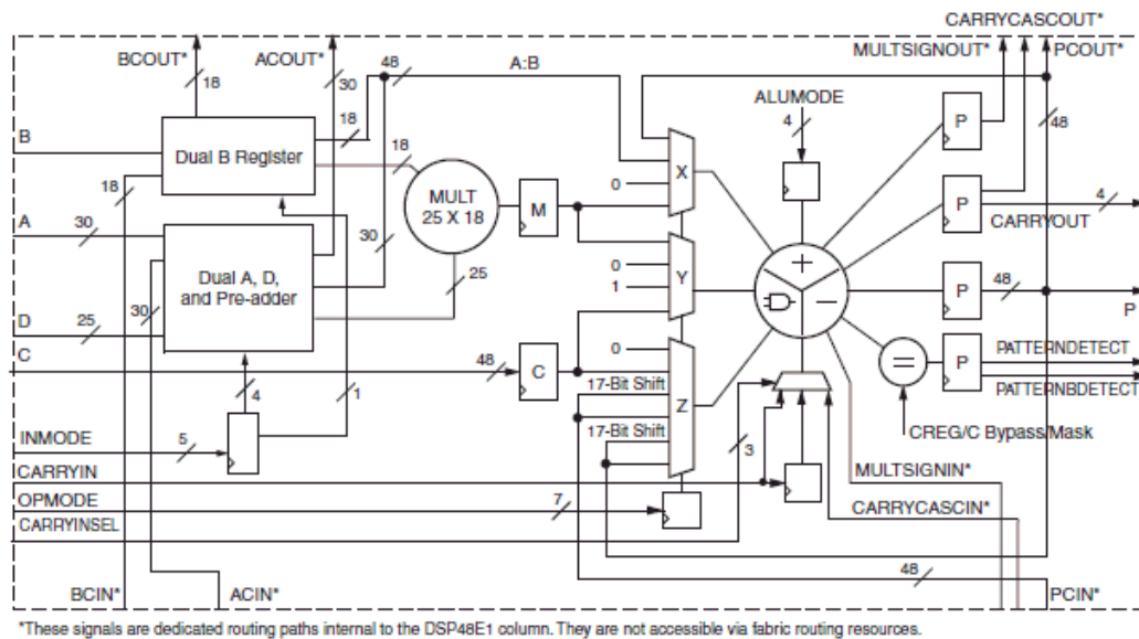
Figure 26: DSP48E1
