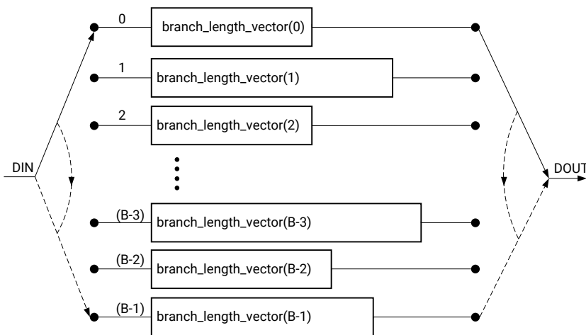
Figure 35: Interleaver/De-Interleaver
