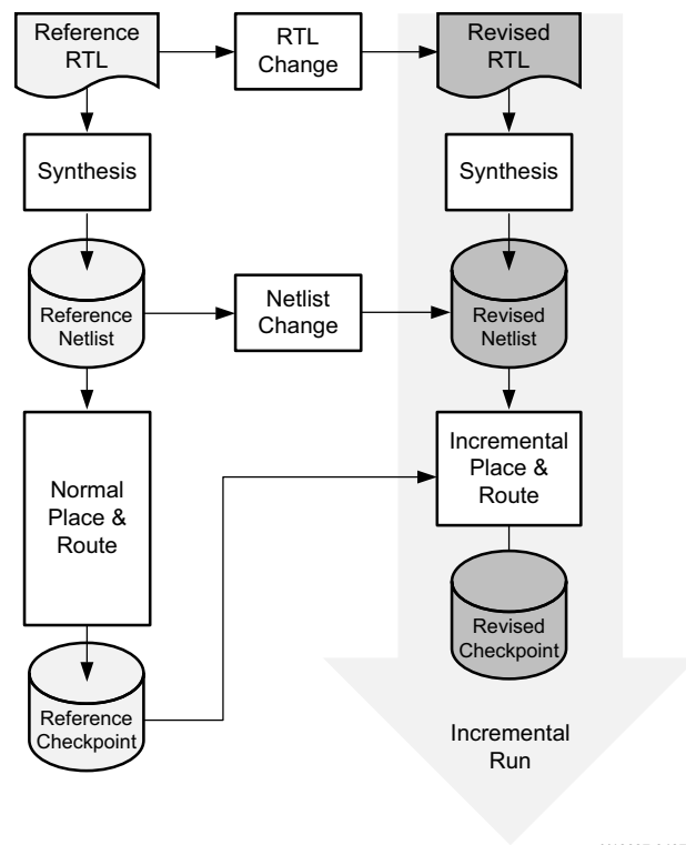
Figure 2-22: Incremental Compile Design Flow
