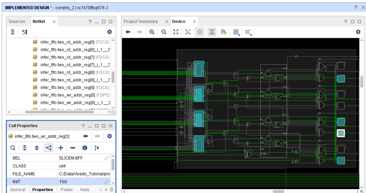
Figure 3-24: Property Modify
