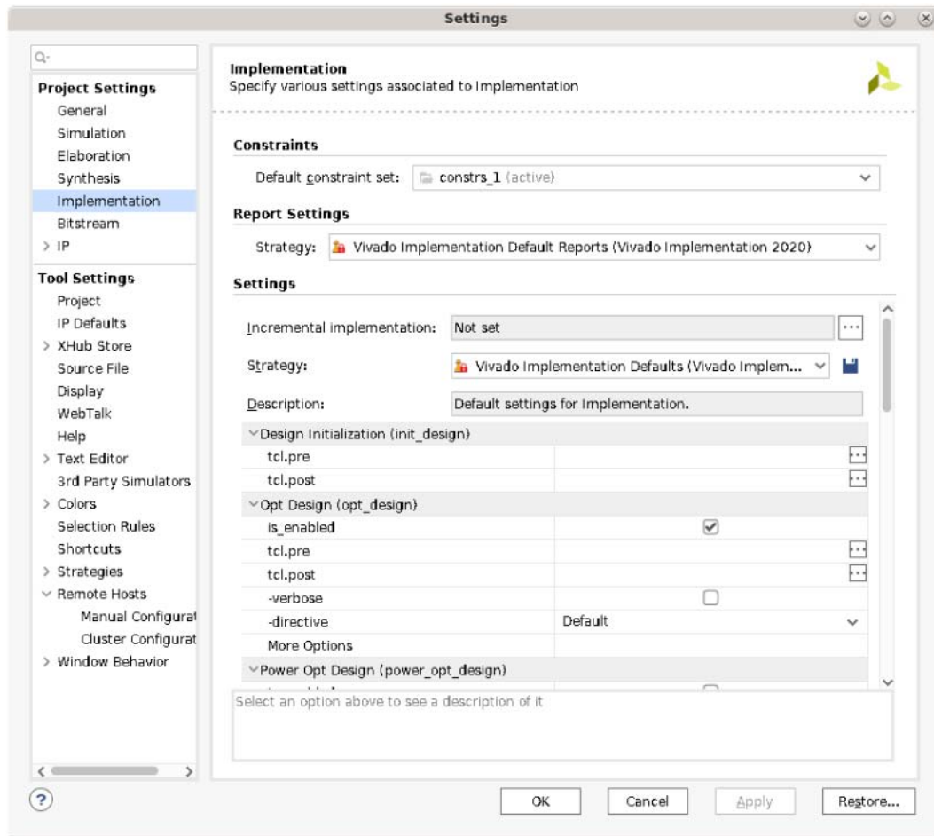
Figure 2-8: Implementation Settings
