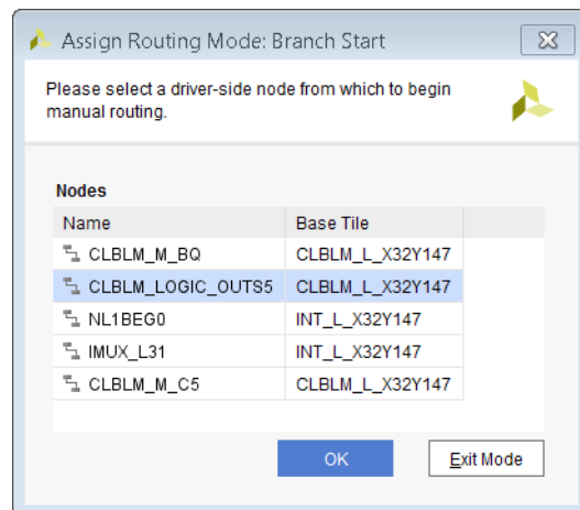
Figure 3-22: Branch Start
