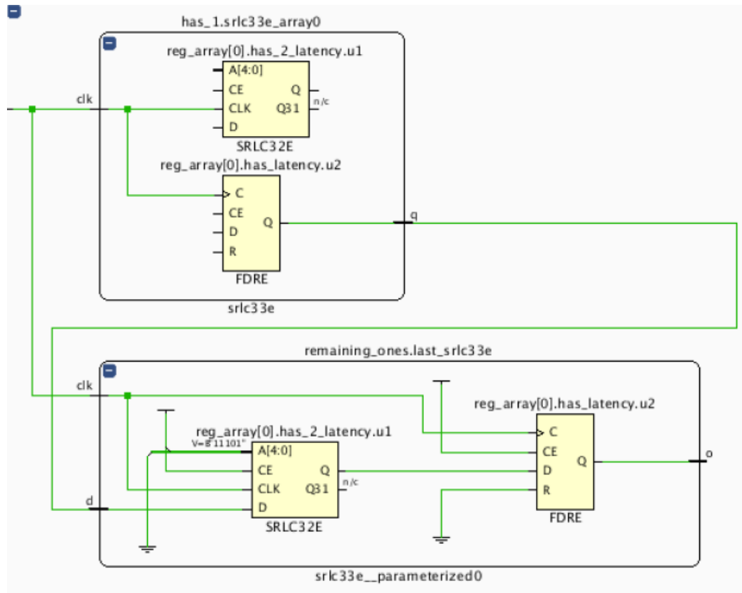
Figure 13: 1-Bit Wide Delay Block with a Latency of L=64
