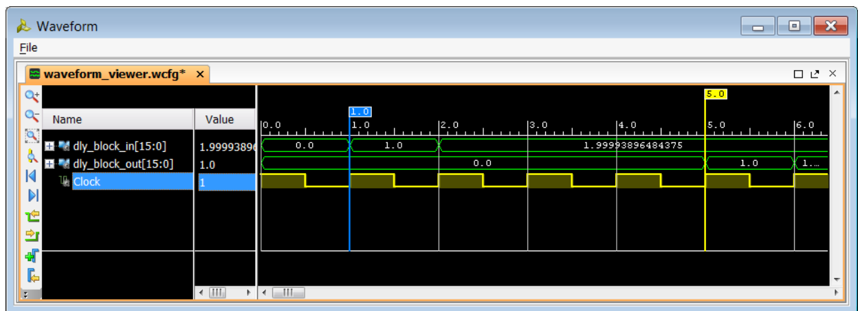
Figure 82: Vector Delay block behavior when L=4 and \text{Period}=1\text{s}
