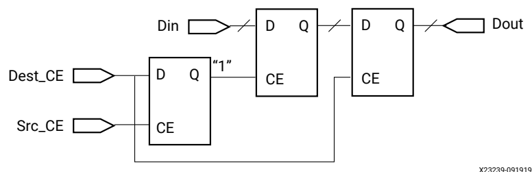
Figure 22: Down Sample with Latency Example
