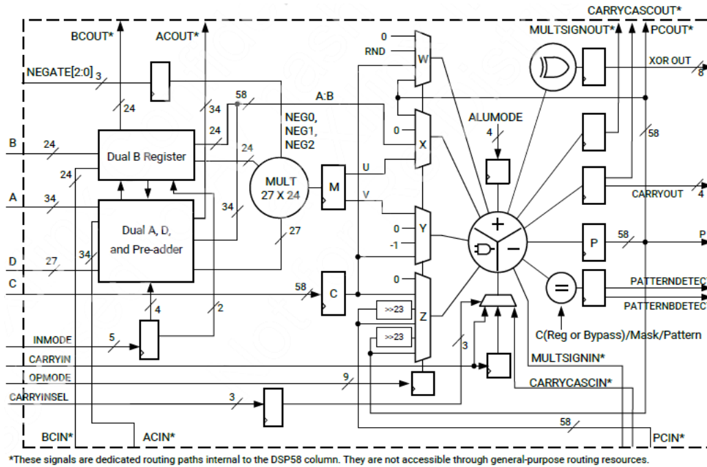
Figure 27: DSP58
