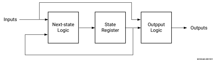
Figure 94: Mealy Machine Block Diagram
