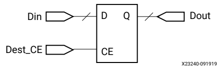
Figure 23: Sampling Last Value
