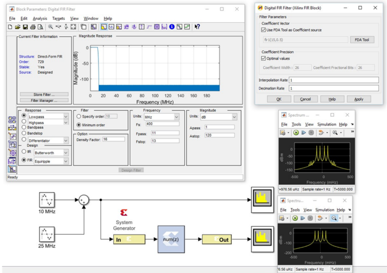
Figure 19: Digital FIR Filter Example
