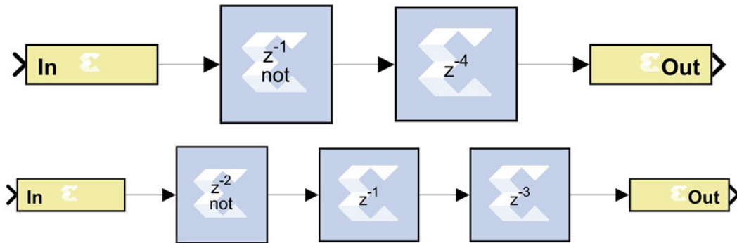
Figure 14: Delay Block with an Additional Delay Block with a Latency
