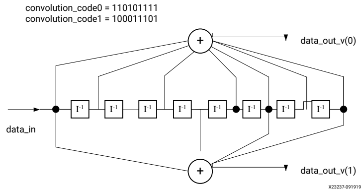
Figure 10: Linear Feed Forward Shift Register
