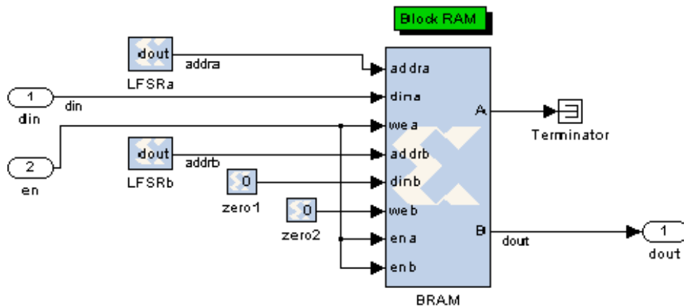
Figure 16: Novel Use of Long Delay LFSRs
