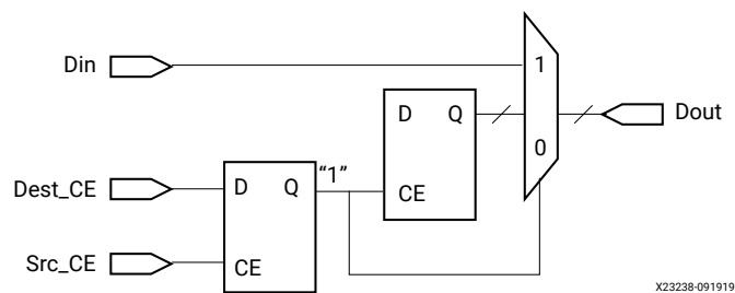
Figure 21: Down Sample with Zero Latency Example
