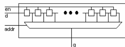
Figure 2: Output Data Port
