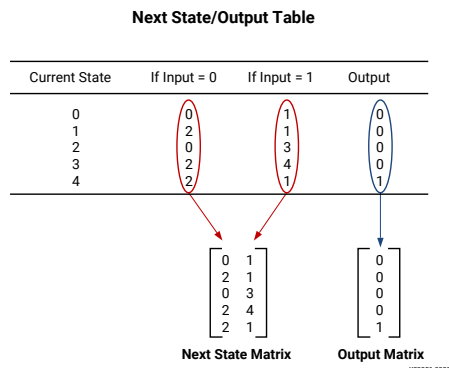
Figure 99: Next State Output Table
