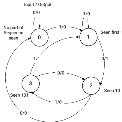
Figure 95: State Transition Diagram
