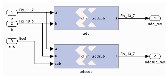
Figure 52: Two Blocks Using Same xl_m_addsub Function
