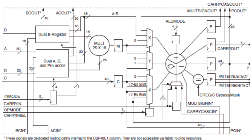
Figure 25: DSP48E1
