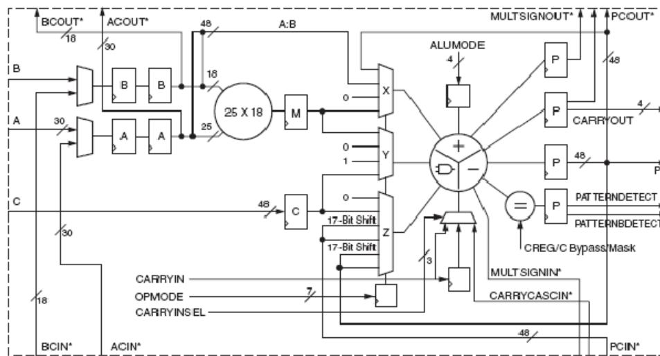
Figure 24: DSP48E
