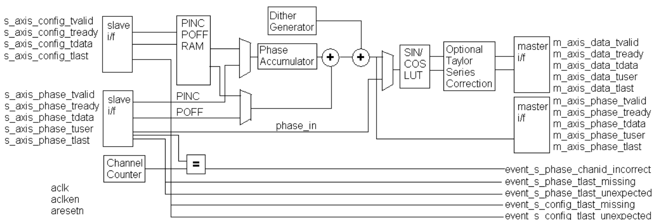
Figure 11: DDS Compiler Block Diagram
