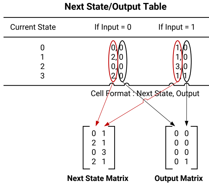
Figure 102: Next State Output Table
