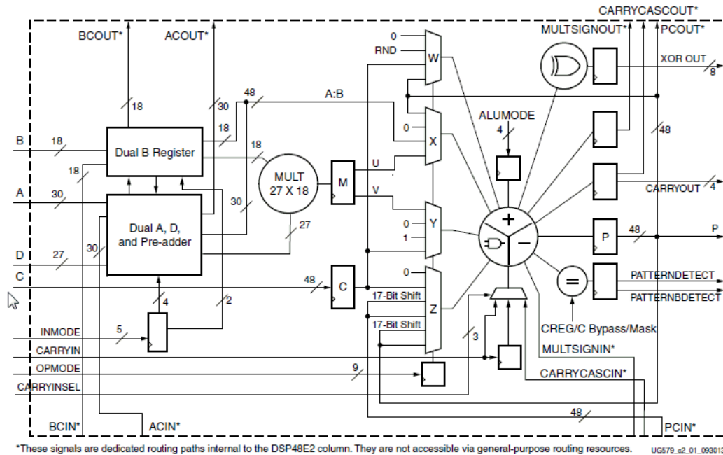
Figure 26: DSP48E2
