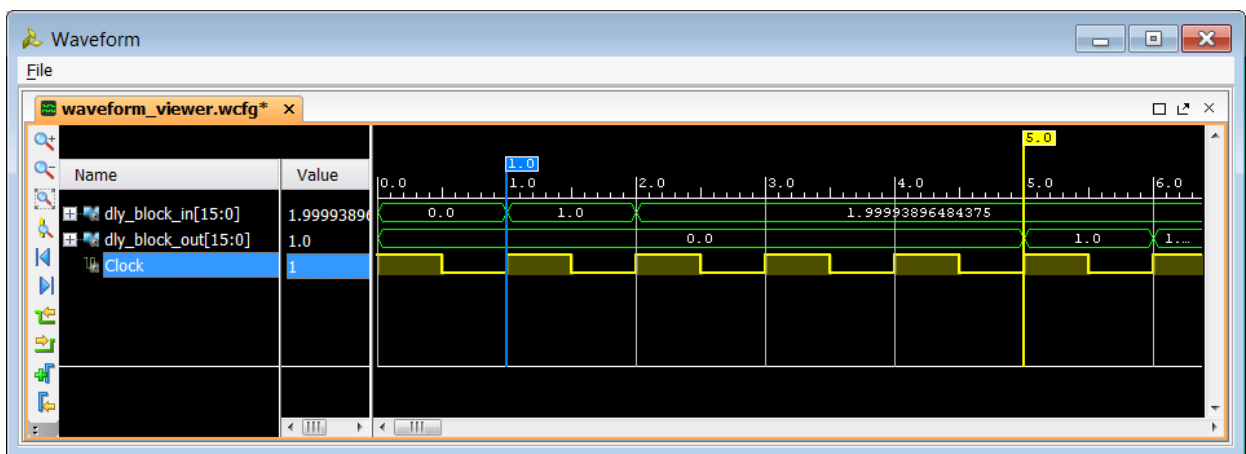
Figure 12: Delay Block Behavior
