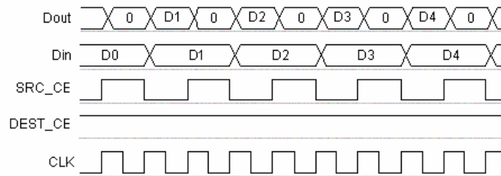
Figure 89: Up Sample Output
