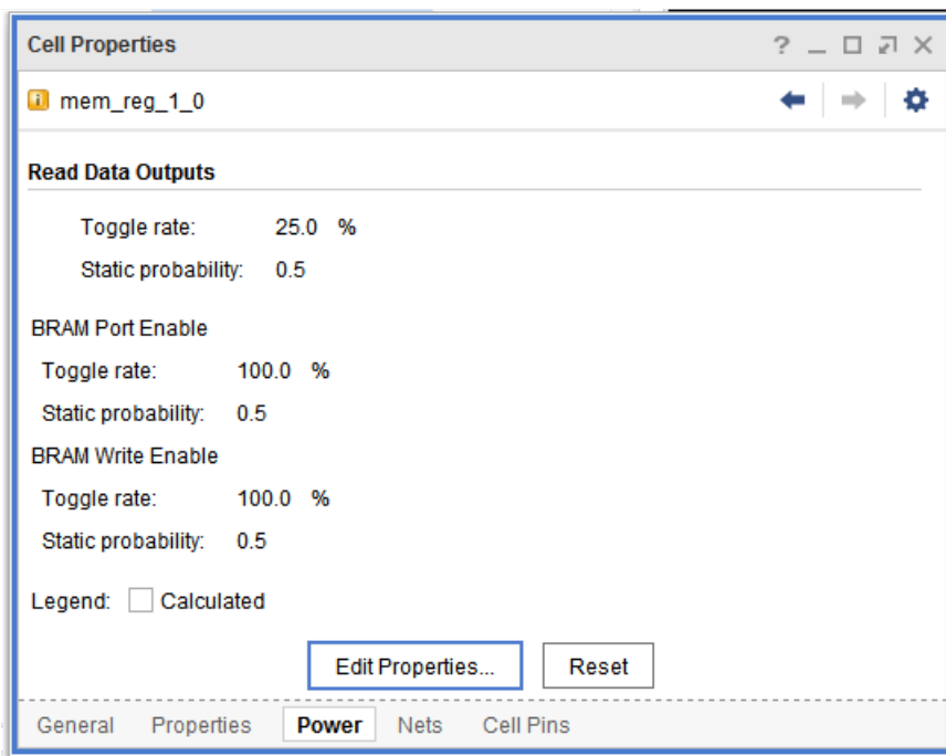
Figure 5-16: Power Properties View for BRAM Cell
