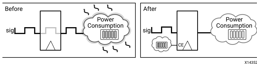
Figure 4-11: Intelligent Clock Gating
