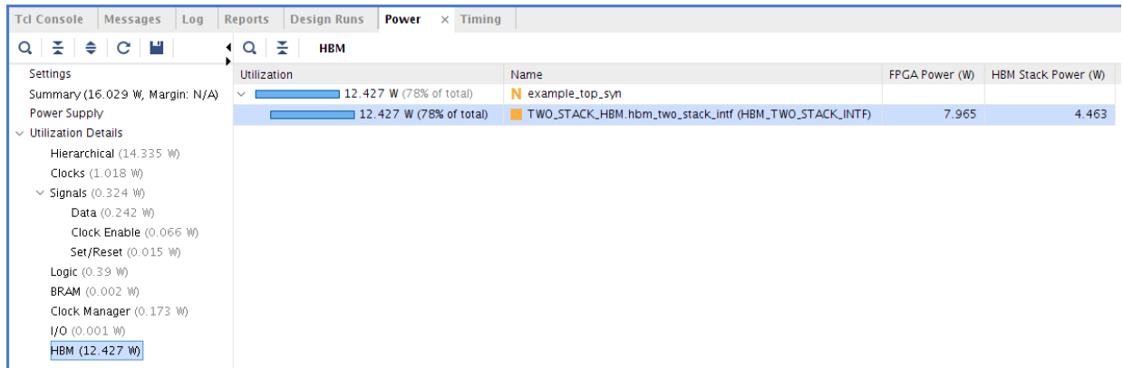
Figure 3-10: Report Power for HBM
