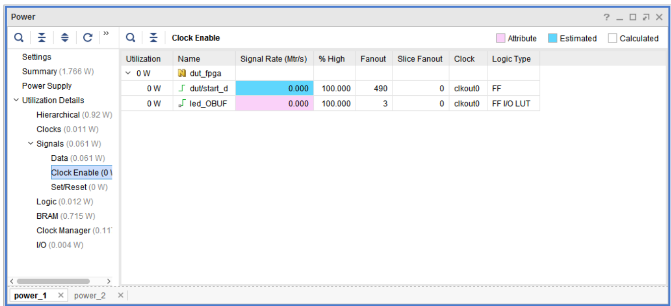
Figure 5-12: Clock Enable Net in the Power Report
