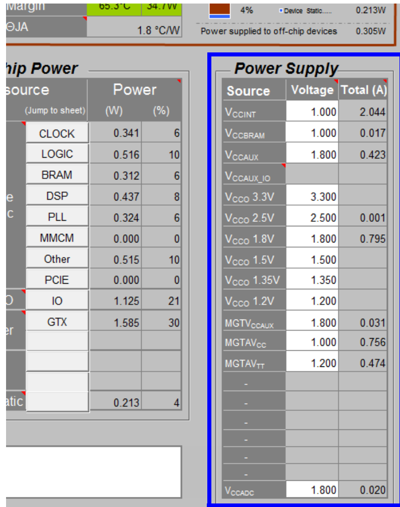
Figure 2-4: Power Supply Voltage Source Information - Summary Sheet for 7 Series Devices
