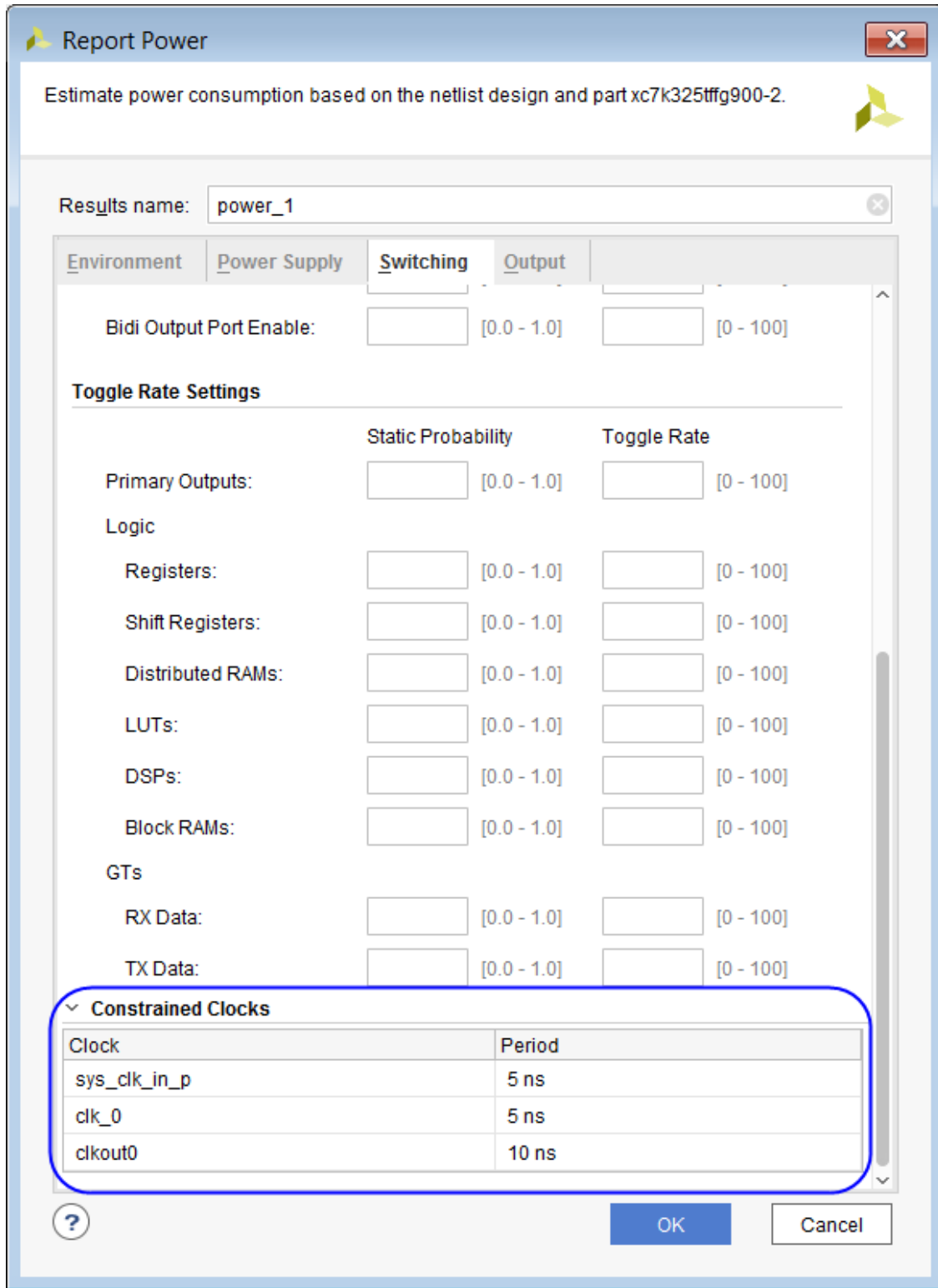
Figure 5-4: Constrained Clocks for Report Power
