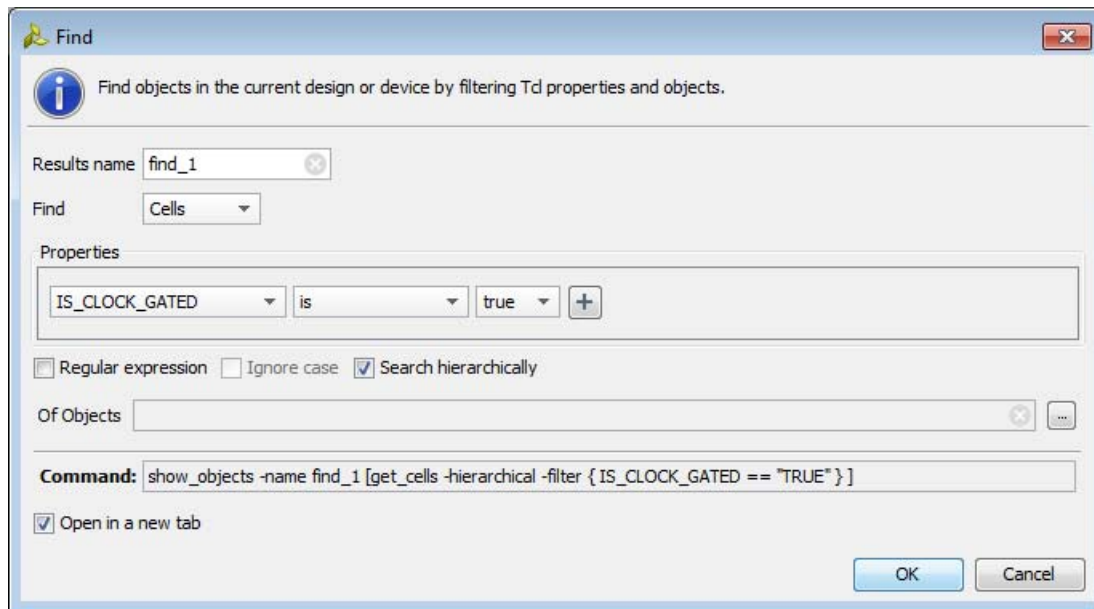
Figure 4-17: Finding Power Optimized Cells
