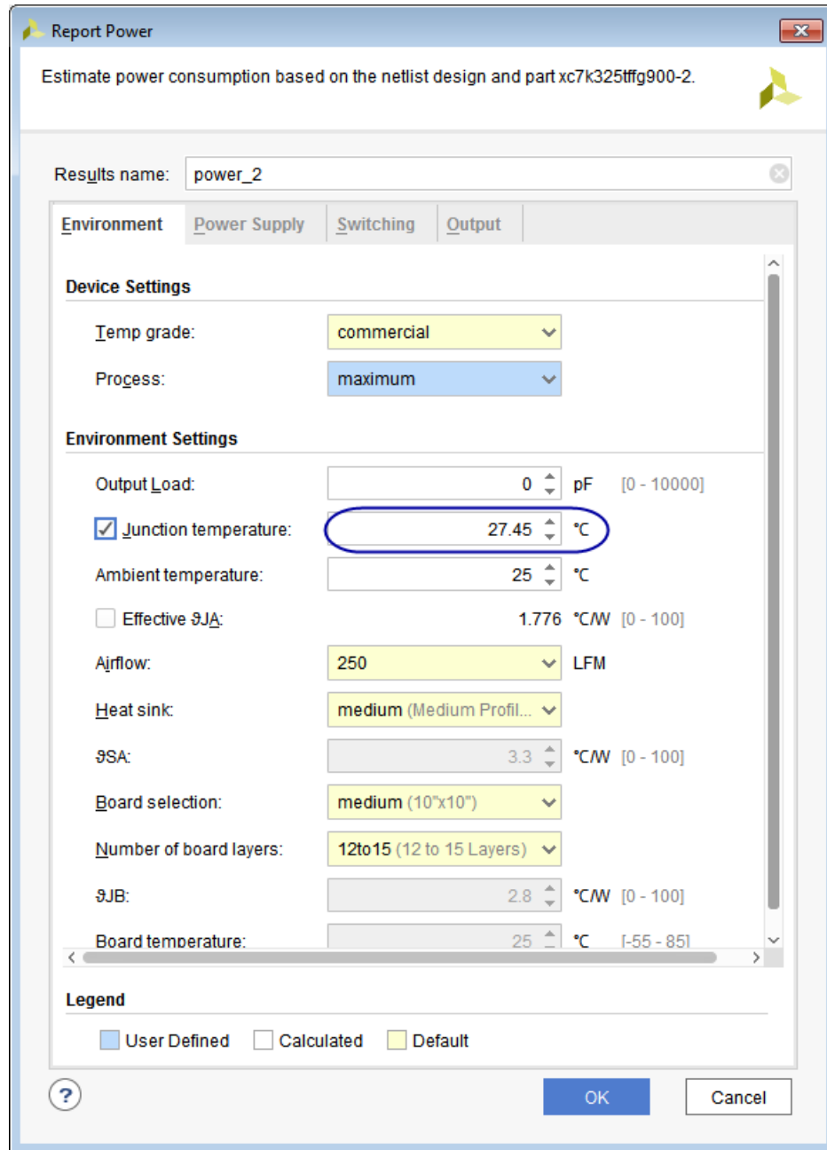
Figure 5-2: Setting Junction Temperature for Report Power
