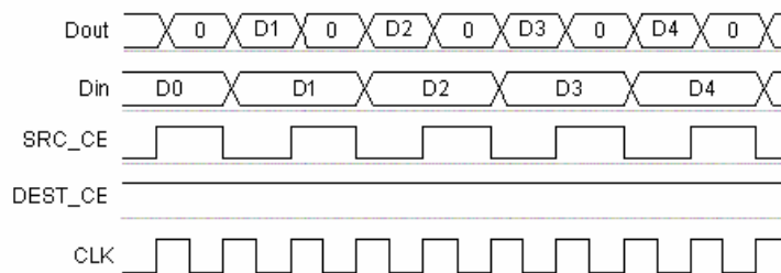
Figure 99: Up Sample Output
