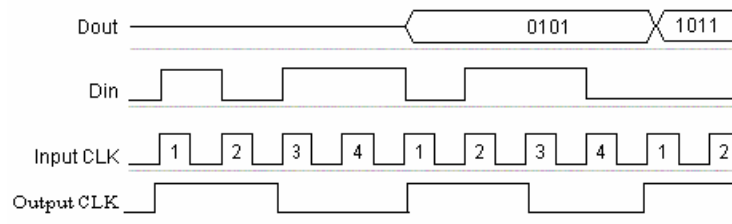
Figure 75: Serial to Parallel Behavior
