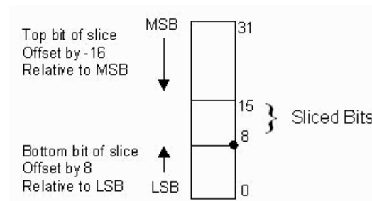
Figure 97: Extracting Top 16 and Bottom 8 Bits
