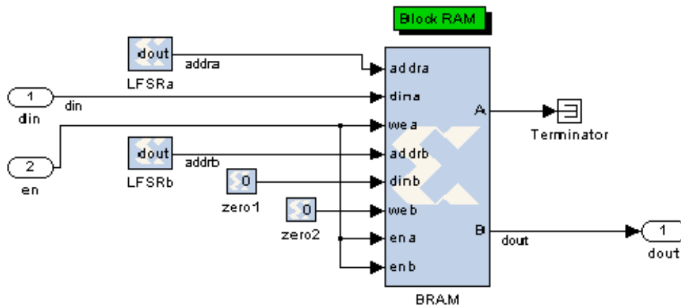
Figure 21: Novel Use of Long Delay LFSRs
