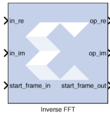
Figure 47: Adding Start Frame Ports
