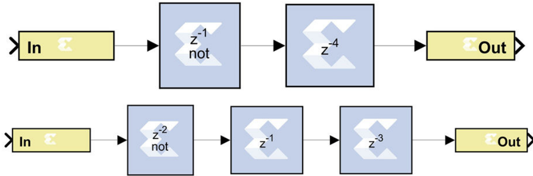
Figure 19: Delay Block with an Additional Delay Block with a Latency
