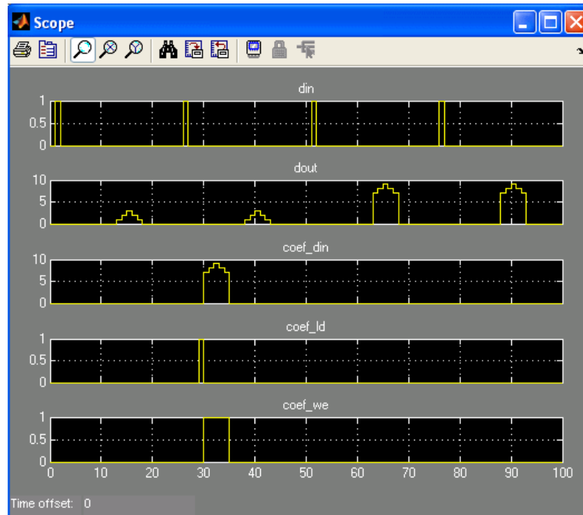
Figure 42: Non-AXI Output Example
