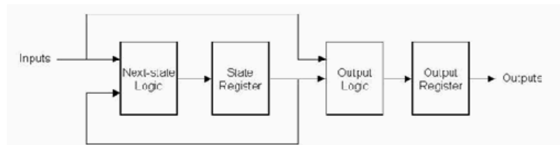
Figure 110: Mealy State Machine Block Diagram
