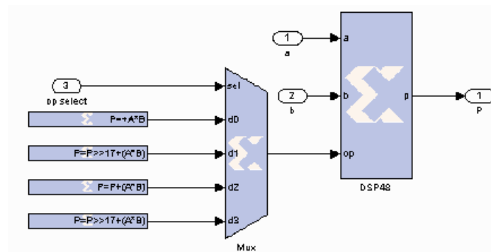
Figure 12: Example of Constant Block Creating a DSP48 Instruction
