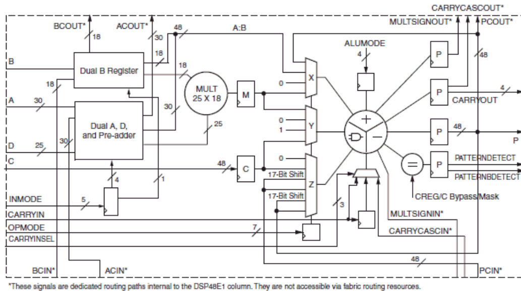
Figure 32: DSP48E2
