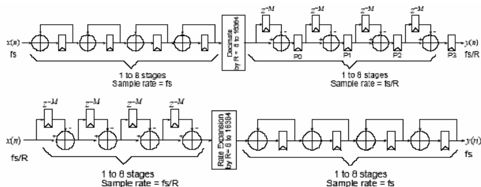
Figure 101: CIC Filter
