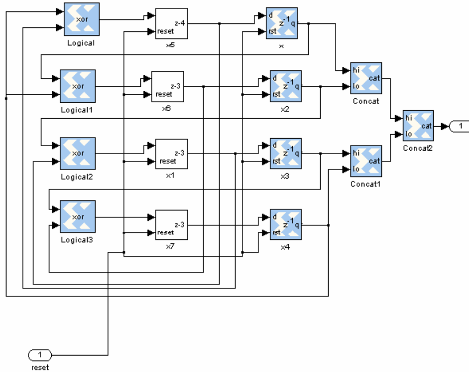
Figure 116: 4-bit Leap-Forward LFSR Diagram
