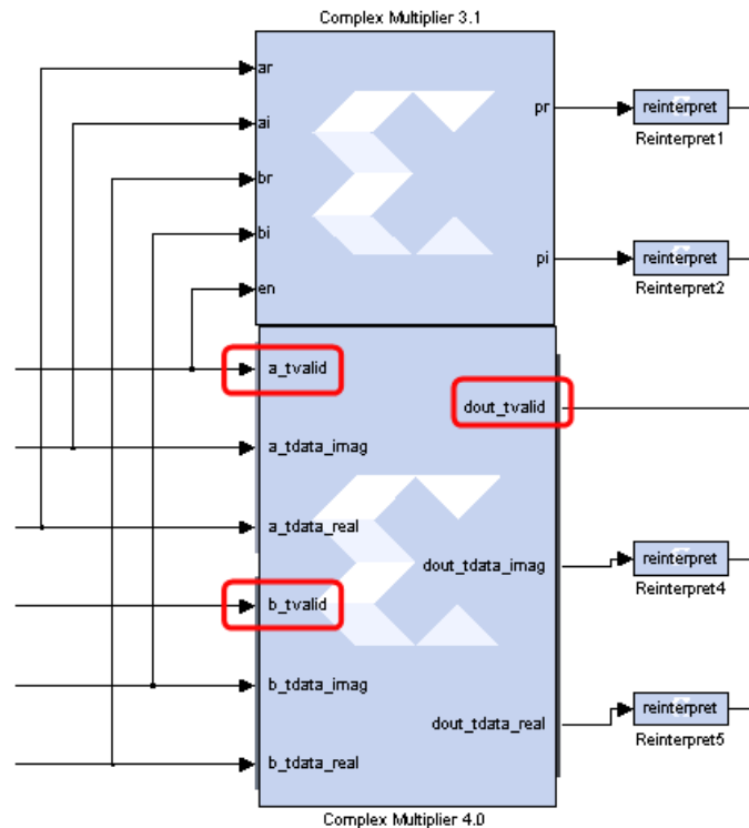
Figure 11: AXI4 Complex Multiplier IP Block
