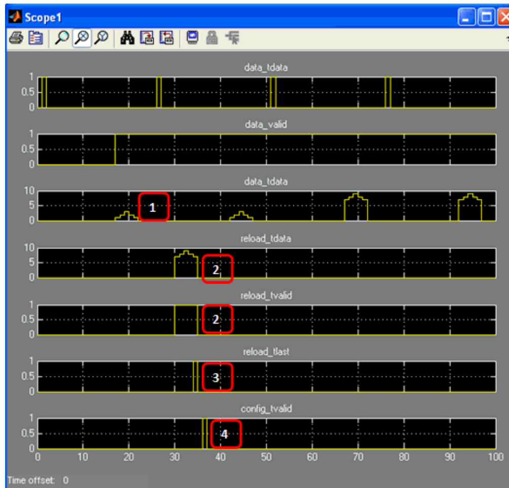
Figure 43: AXI4 Output Example
