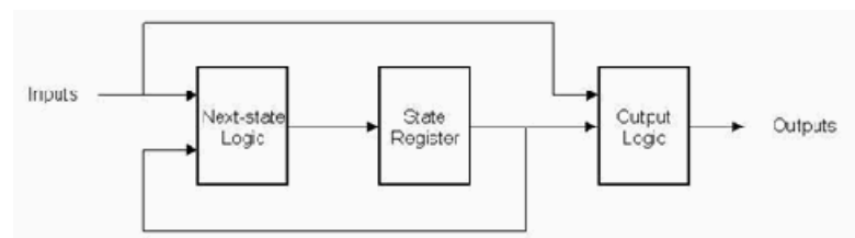
Figure 104: Mealy Machine Block Diagram
