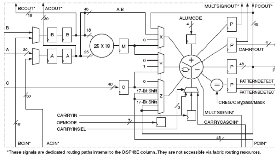
Figure 29: DSP48
