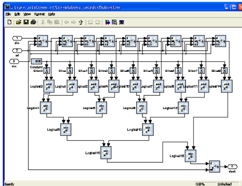
Figure 103: Implementation
