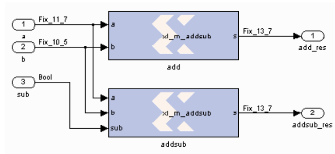
Figure 63: Two Blocks Using Same xl_m_addsub Function
