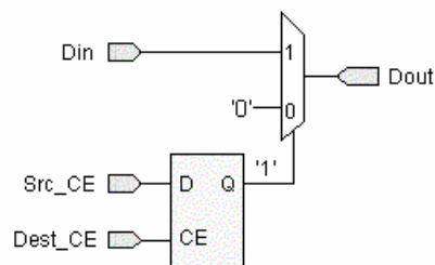
Figure 88: Zero Padding Up Sample Circuit
