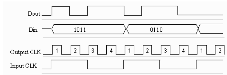
Figure 70: Block Behavior
