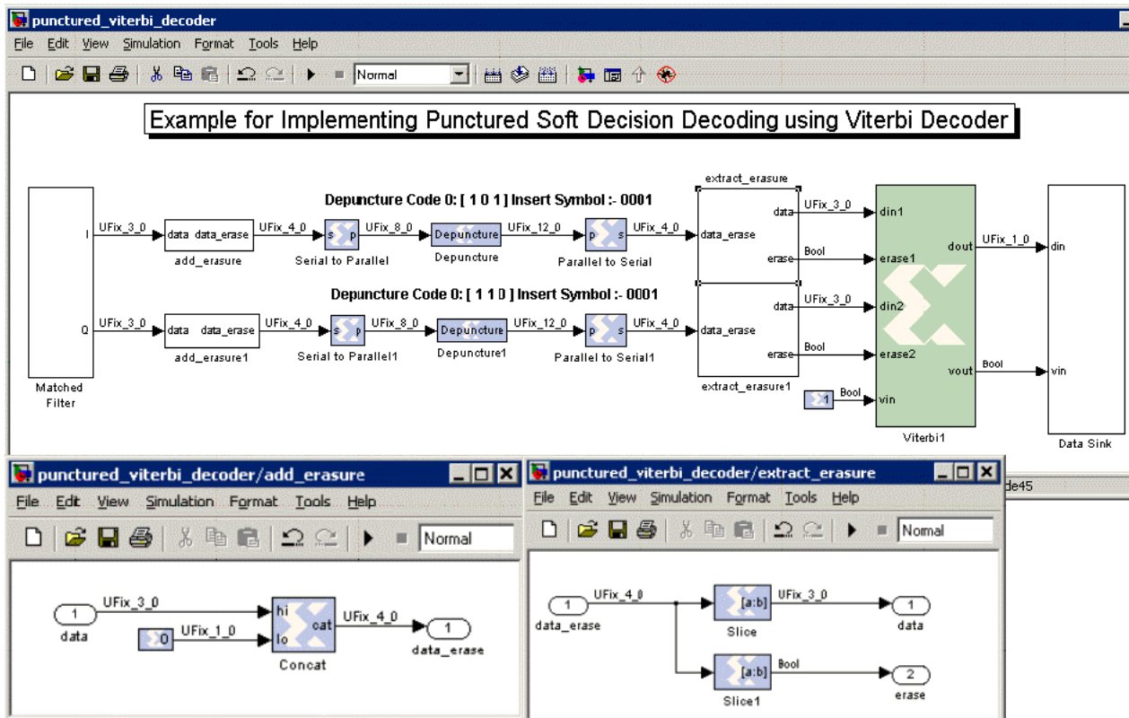
Figure 22: Soft Decision Viterbi Decoding
