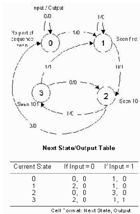
Figure 105: State Transmission Diagram
