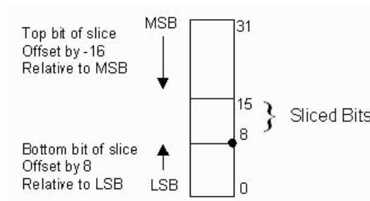
Figure 80: Extracting Top 16 and Bottom 8 Bits
