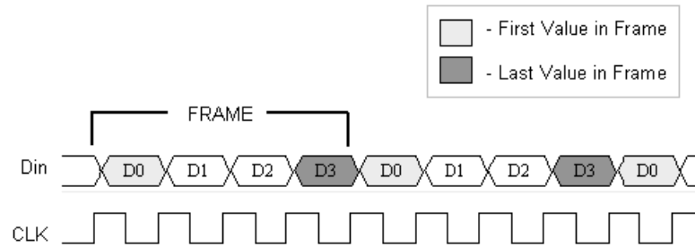
Figure 93: Vector Down Sample with Sampling Rate of 4
