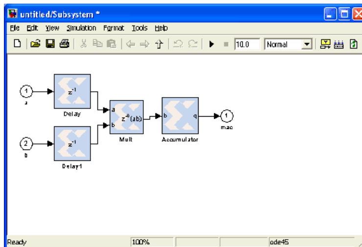
Figure 180: Generated Diagram
