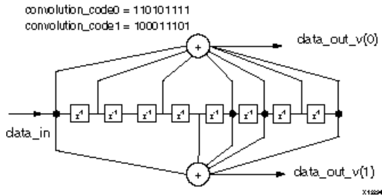
Figure 13: Linear Feed Forward Shift Register
