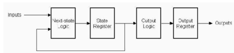
Figure 113: Moore State Machine Block Diagram
