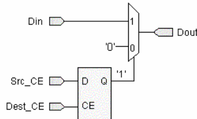
Figure 98: Zero Padding Up Sample Circuit
