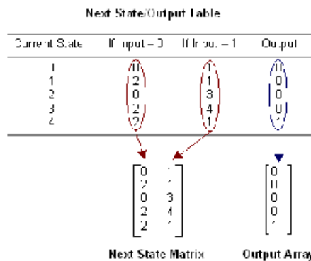
Figure 109: Next State Output Table
