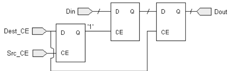
Figure 95: Two Register Example
