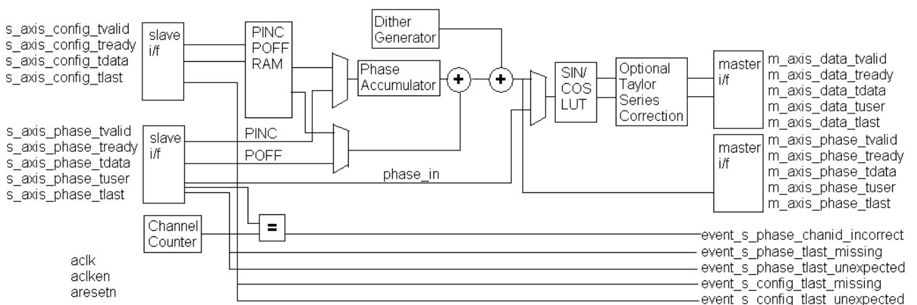
Figure 14: DDS Compiler Block Diagram
