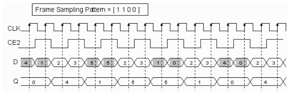
Figure 86: Single Channel Implementation
