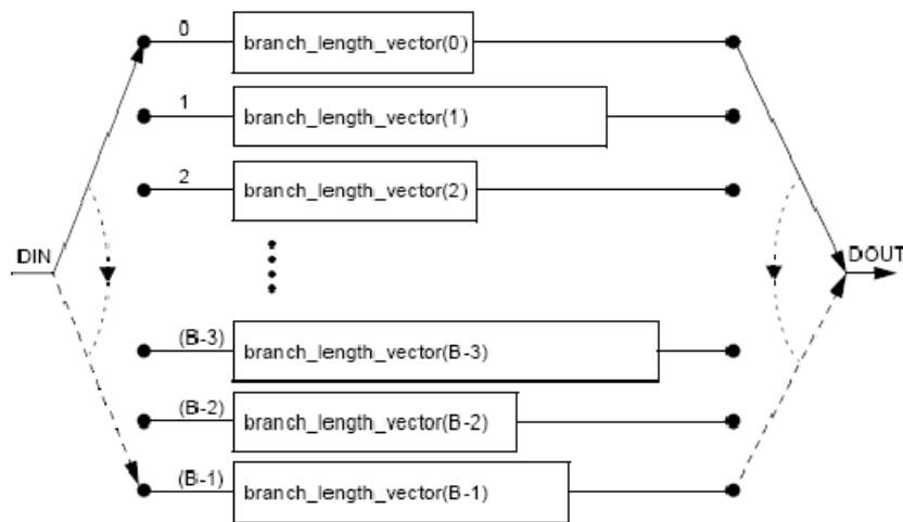
Figure 46: Interleaver/De-Interleaver
