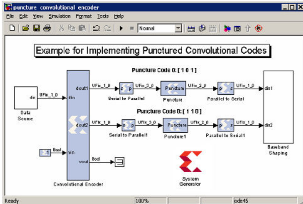
Figure 71: Implementing Punctured Convolution Codes
