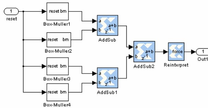
Figure 117: Box-Muller Method Diagram
