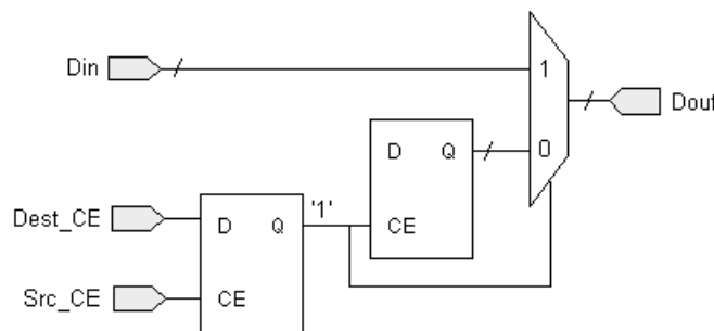
Figure 26: Down Sample with Zero Latency Example
