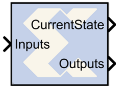
Figure 113: Moore State Machine Block Diagram
