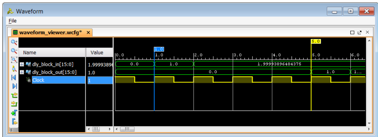
Figure 92: Vector Delay block behavior when L=4 and Period=1s
