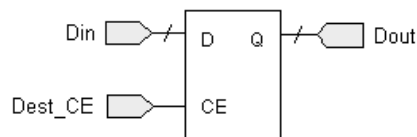
Figure 28: Sampling Last Value
