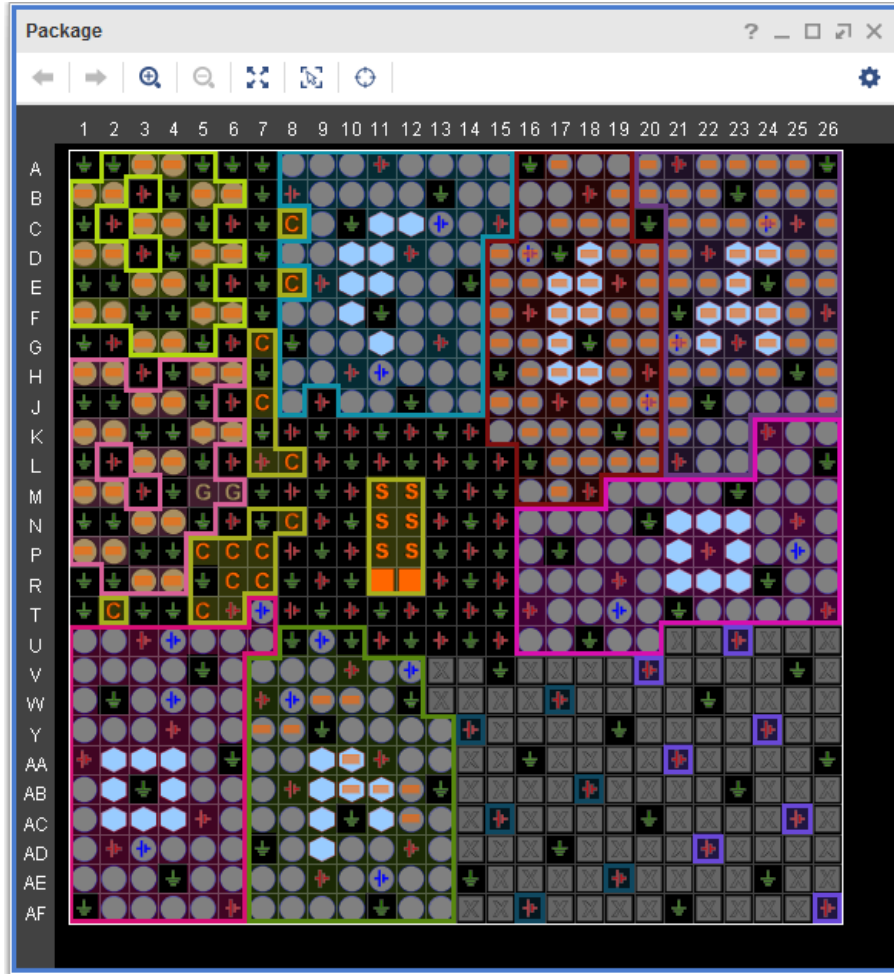
Figure 3-34: Package Window
