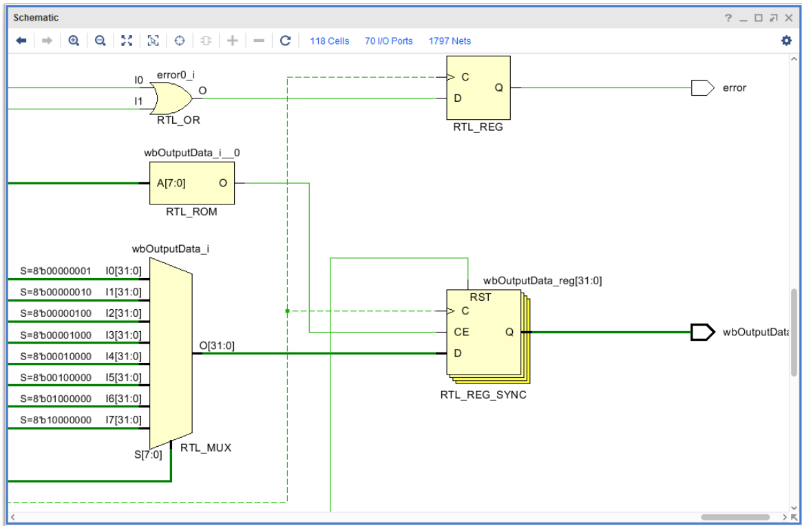
Figure 3-43: RTL Schematic with Bundled Logic
