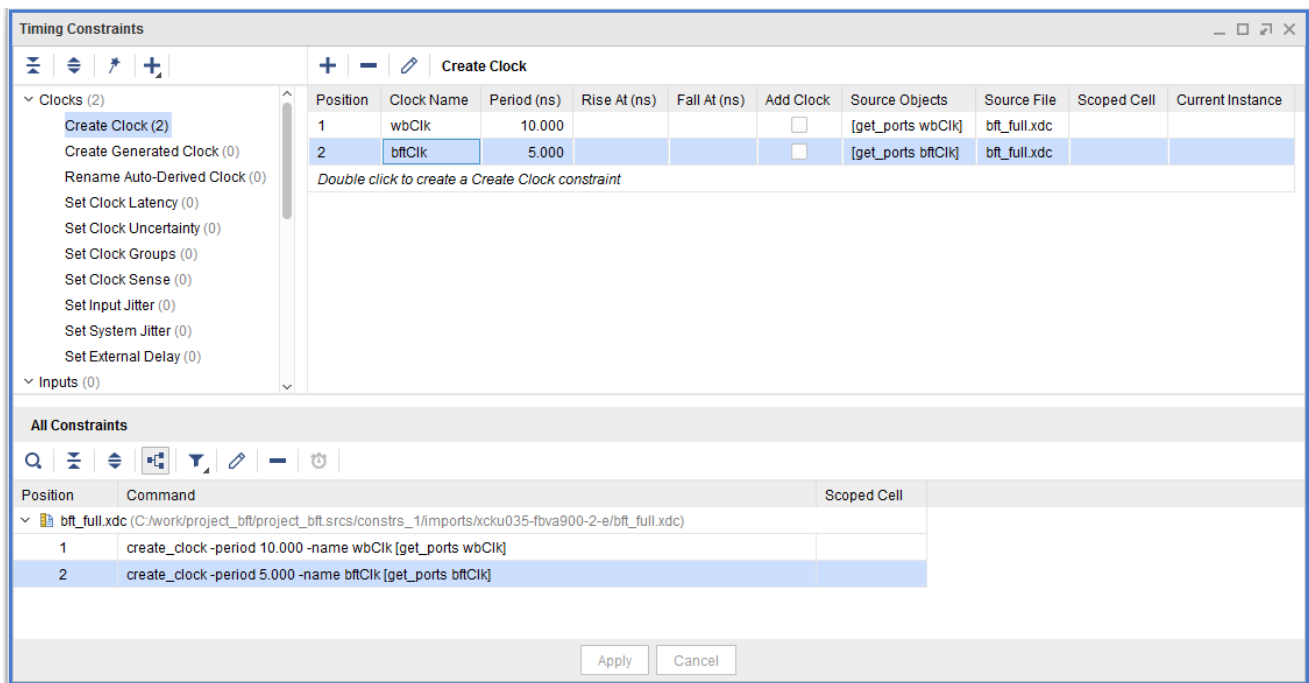
Figure 3-46: Timing Constraints Window
