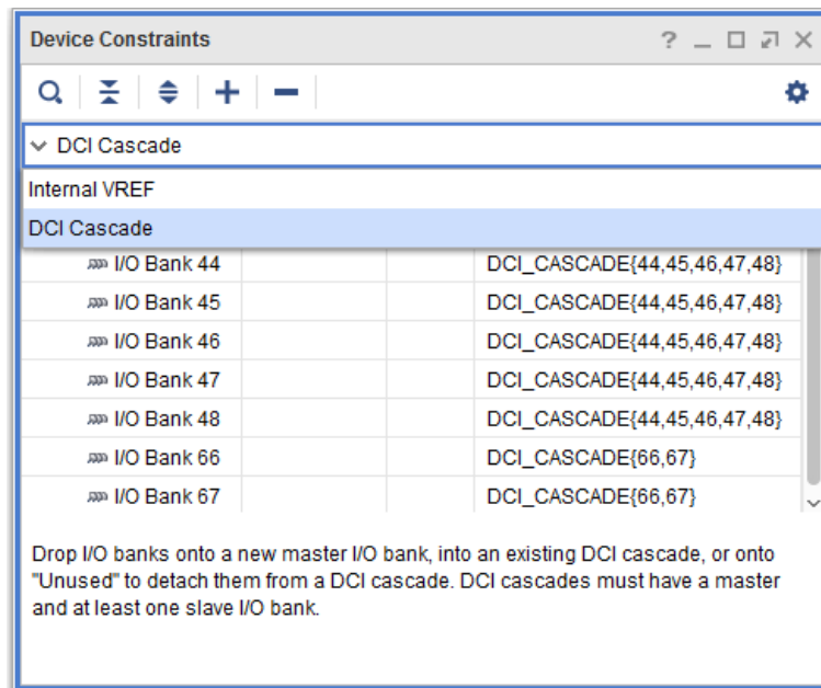
Figure 3-20: Device Constraints Window
