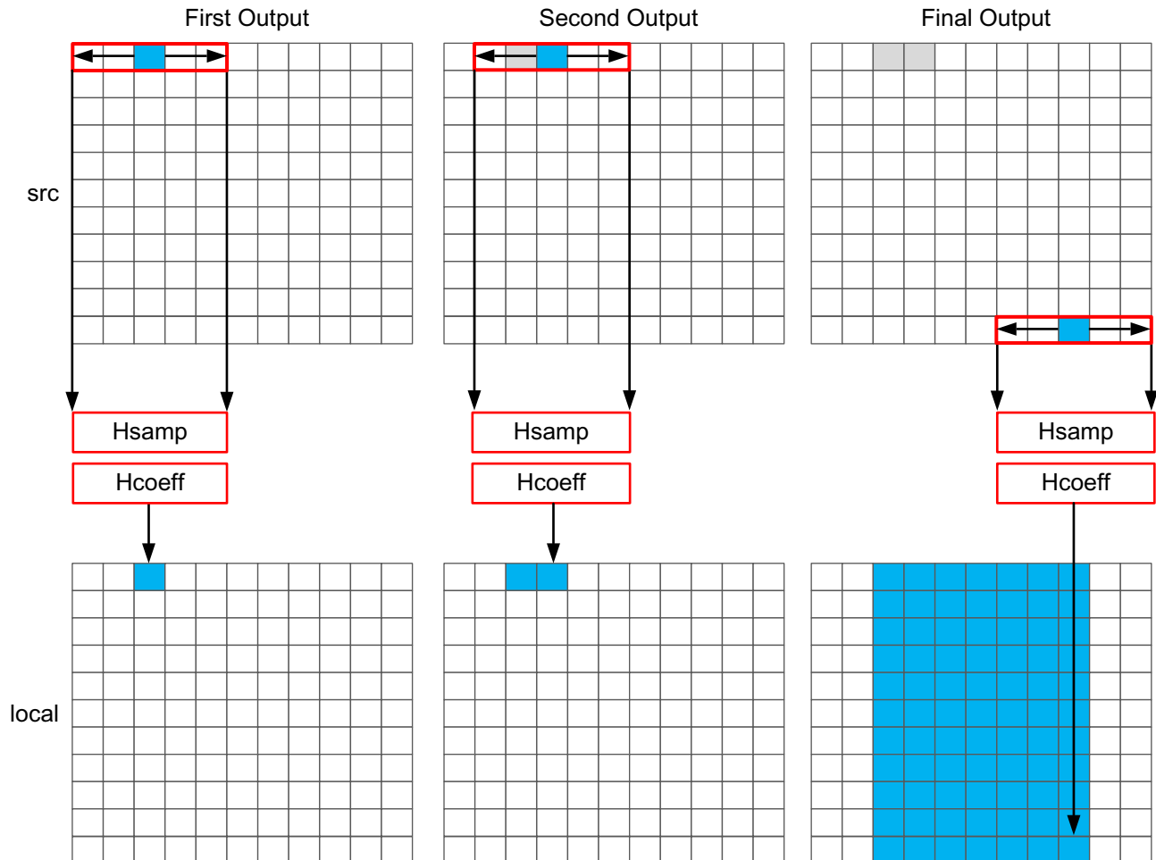
Figure 3-2: Horizontal Convolution
