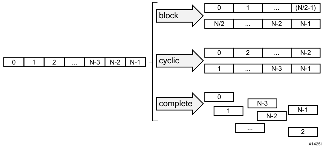
Figure 1-55: Array Partitioning
