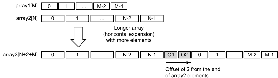
Figure 1-67: Horizontal Mapping with Offset
