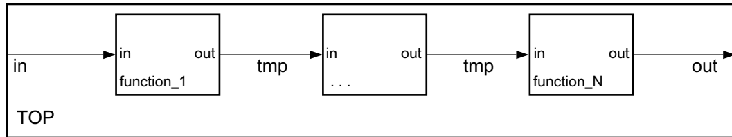
Figure 1-61: Sequential Functional Description
