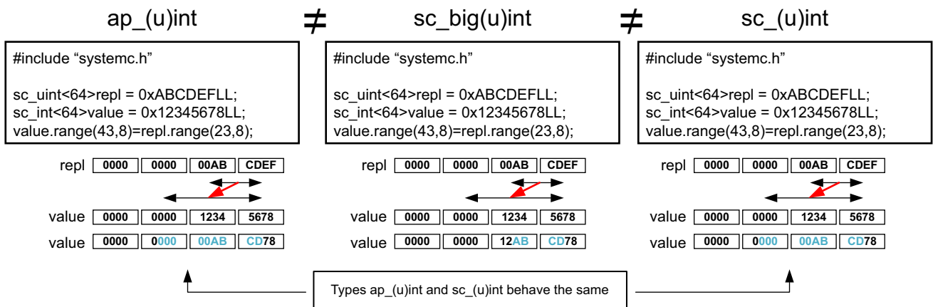
Figure 4-19: Range Operation Differences
