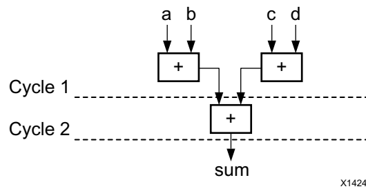
Figure 1-72: Adder Tree After Balancing
