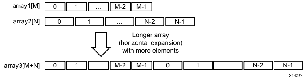
Figure 1-65: Horizontal Mapping
