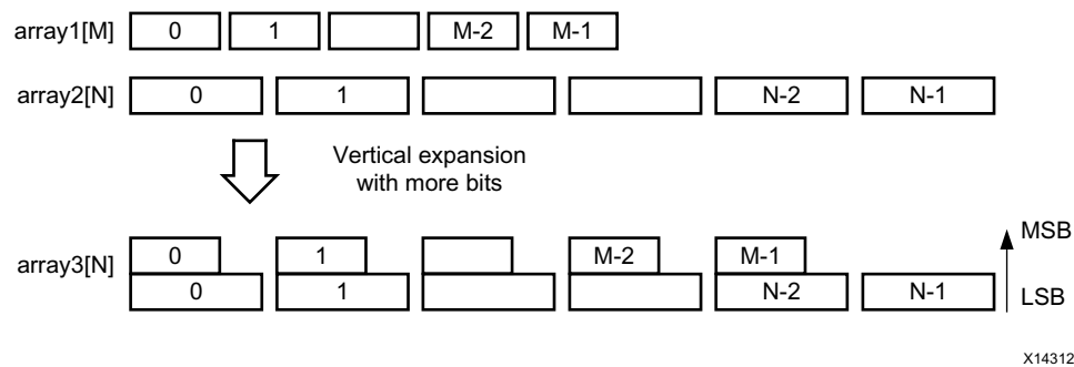
Figure 1-68: Vertical Mapping
