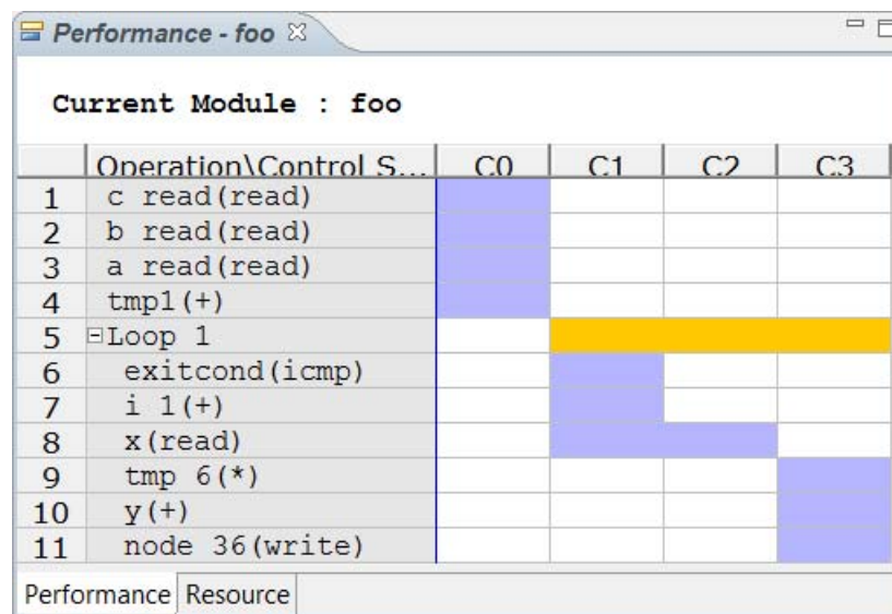
Figure 1-5: Vivado HLS Analysis Example
