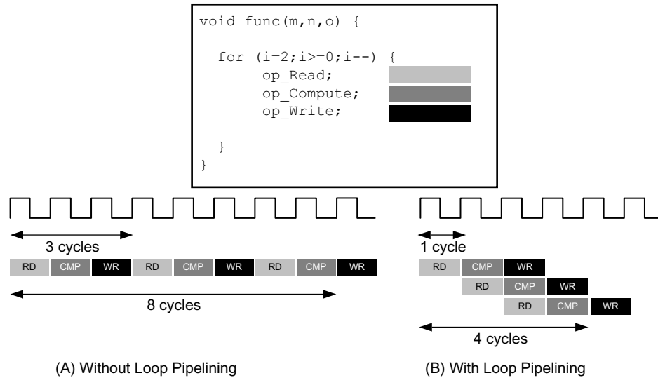
Figure 1-51: Loop Pipelining
