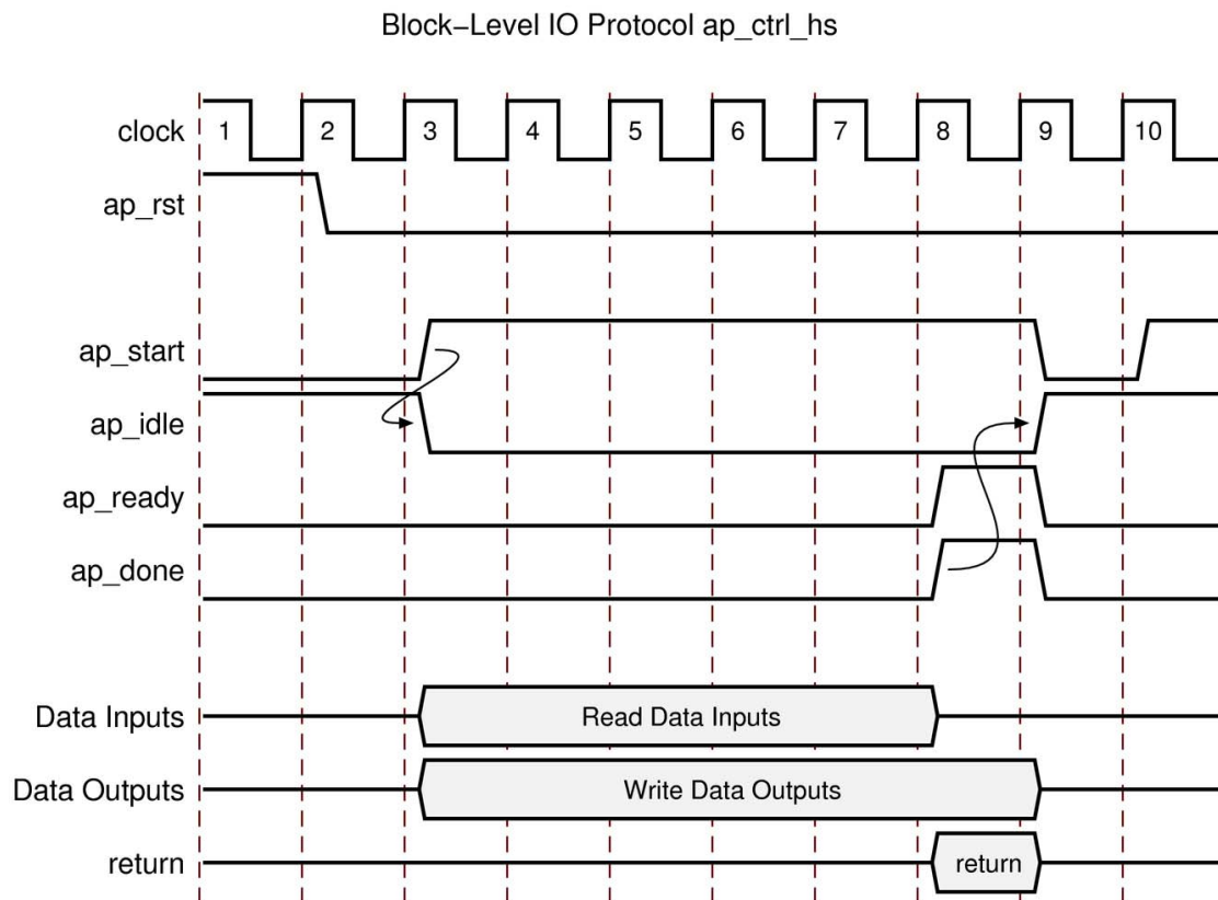
Figure 4-6: Behavior of ap_ctrl_hs Interface
