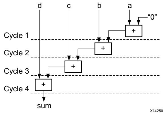
Figure 1-71: Adder Tree
