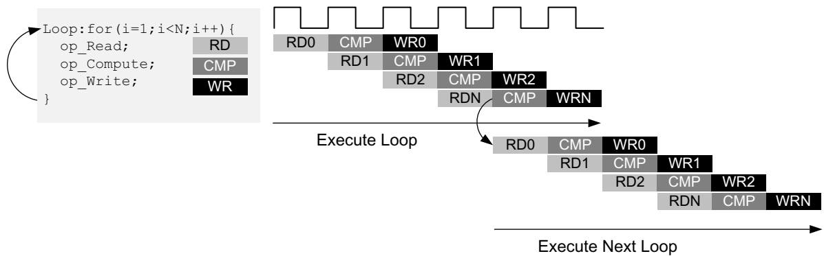
Figure 1-53: Loop Pipelining with Rewind Option
