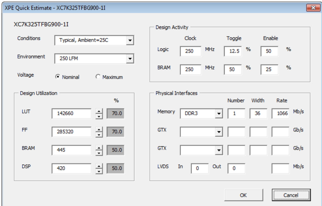
Figure 1-10: XPE Quick Estimate Dialog Box (Virtex-7 Devices)
