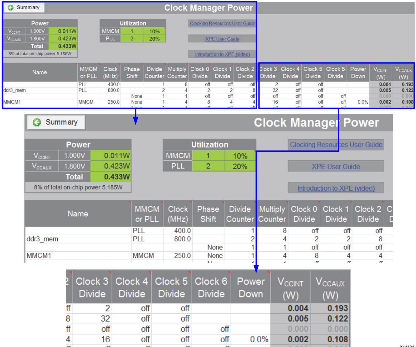
Figure 2-2: Clock Manager Power Sheet (7 Series Devices)
