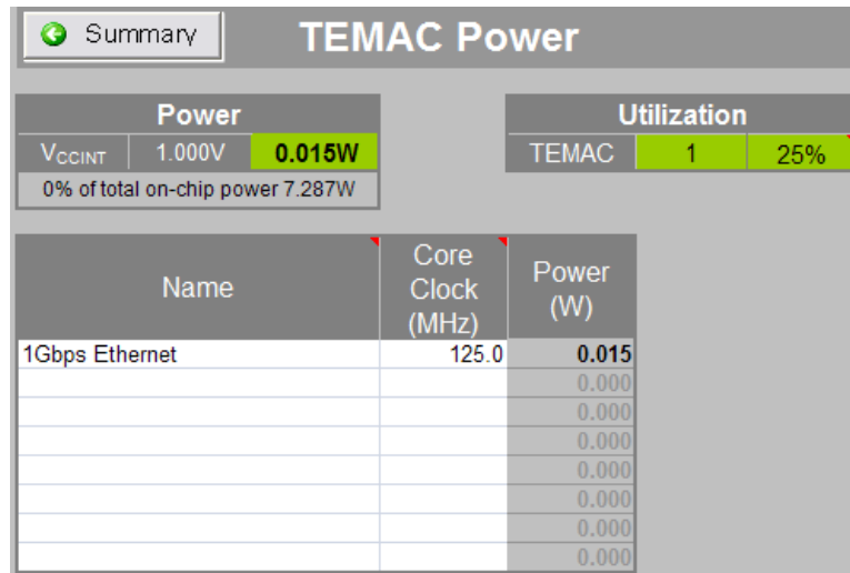
Figure 3-14: TEMAC Power Sheet (Virtex-6 Devices)
