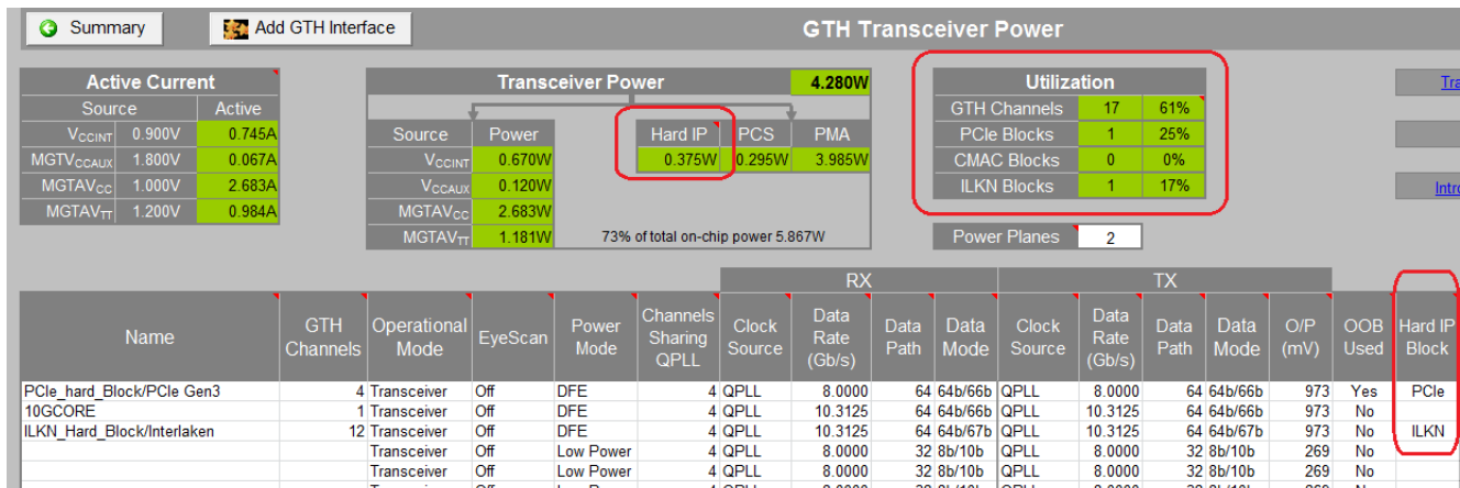
Figure 3-13: Hard IP Settings for UltraScale Devices
