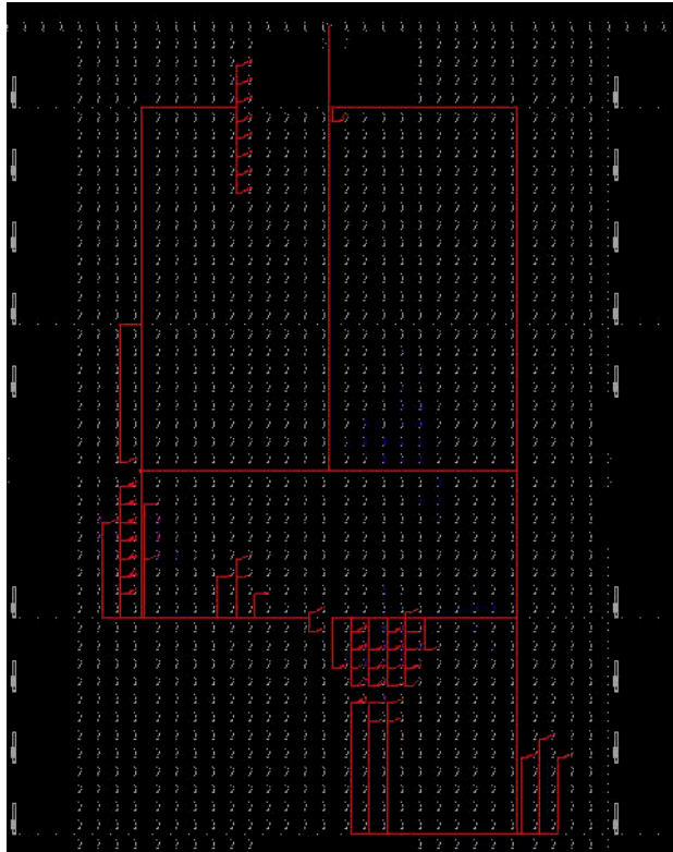
Figure 6-22: Clock Net
