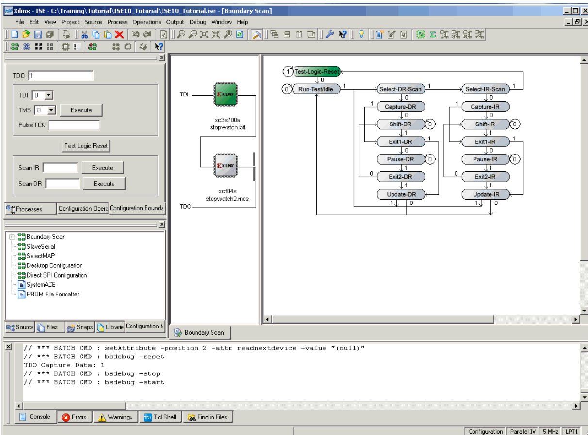
Figure 8-11: Debug Chain
