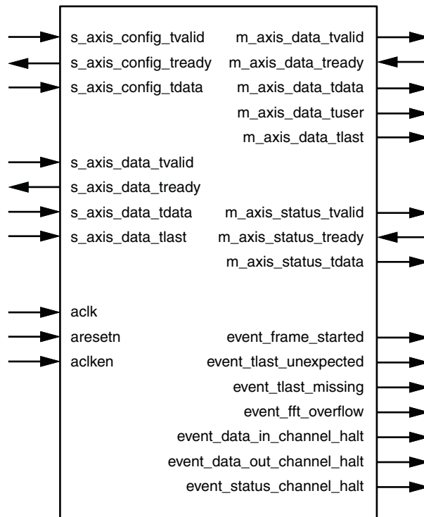
Figure 2-1: Core Schematic Symbol
