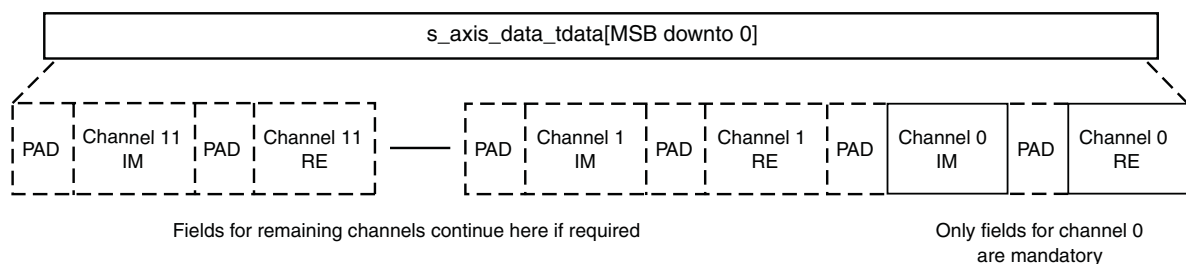
Figure 3-4: Data Input Channel TDATA ( s_axis_data_tdata ) Format
