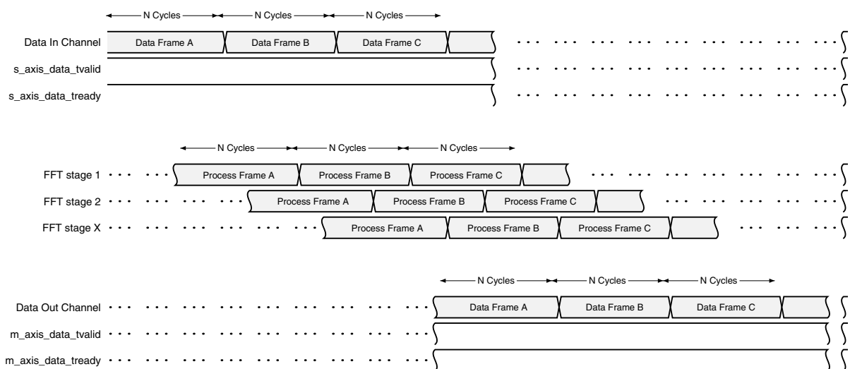
Figure 3-42: Transform Timing for Entire Frames in Pipelined Streaming I/O with no Cyclic Prefix Insertion
