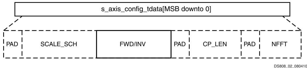
Figure 3-2: Configuration Channel TDATA ( s_axis_config_tdata ) Format
