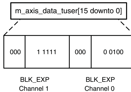
Figure 3-10: Data Output Channel TUSER Example 2
