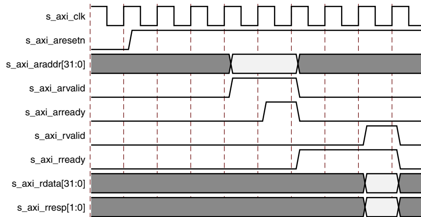
Figure 3-28: AXI4-Lite Read Timing Diagram
