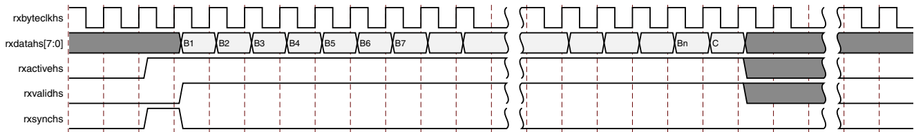
Figure 3-19: High-speed Mode Data Receive at the D-PHY RX (Slave)
