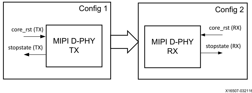
Figure 3-12: MIPI D-PHY TX and RX System
