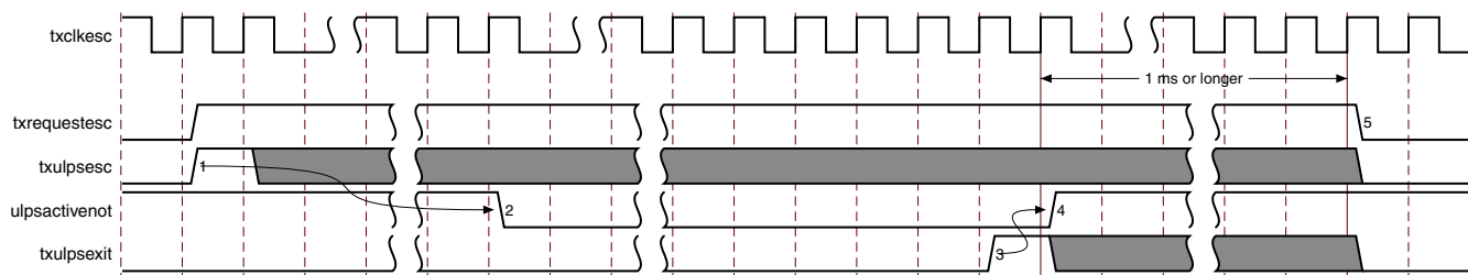
Figure 3-17: D-PHY TX (Master) ULPS Mode Operation for Data Lane
