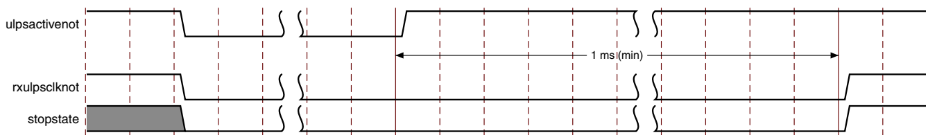
Figure 3-25: D-PHY RX (Slave) ULPS Mode Operation for Clock Lane
