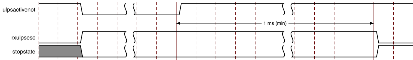
Figure 3-24: D-PHY RX (Slave) ULPS Mode Operation for Data Lane
