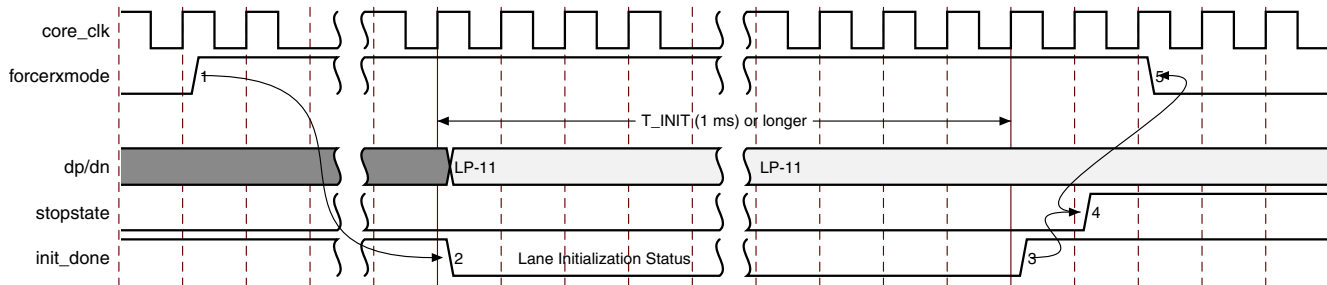
Figure 3-26: RX Data Lane Initialization Using forcexmode
