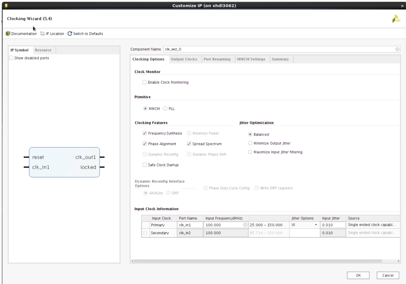
Figure 4-3: Clocking Options for 7 Series MMCM (Spread Spectrum Selected)
