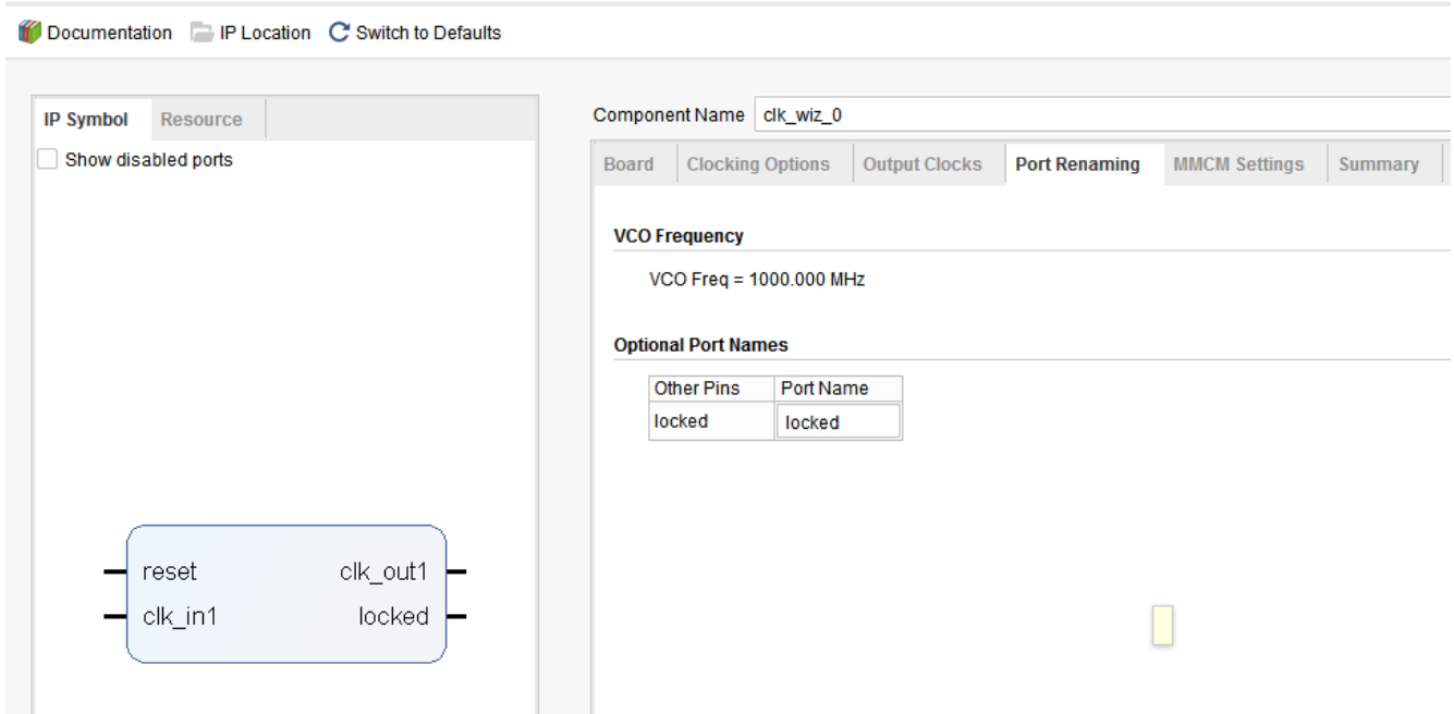
Figure 4-13: Port Renaming (Spread Spectrum Unselected)
