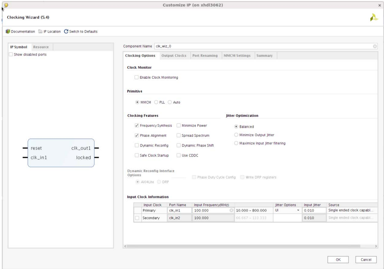
Figure 4-2: Clocking Options with Spread Spectrum Unselected for UltraScale and UltraScale+
