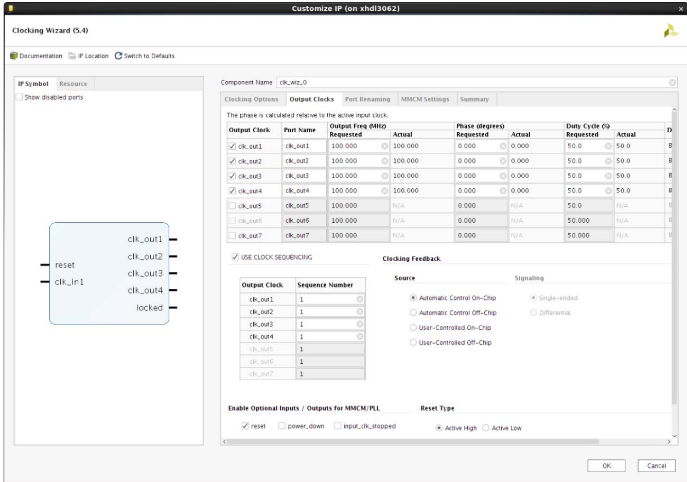
Figure 4-5: Output Clocks with Safe Clock Start Up and Clock Sequencing for 7 Series MMCM
