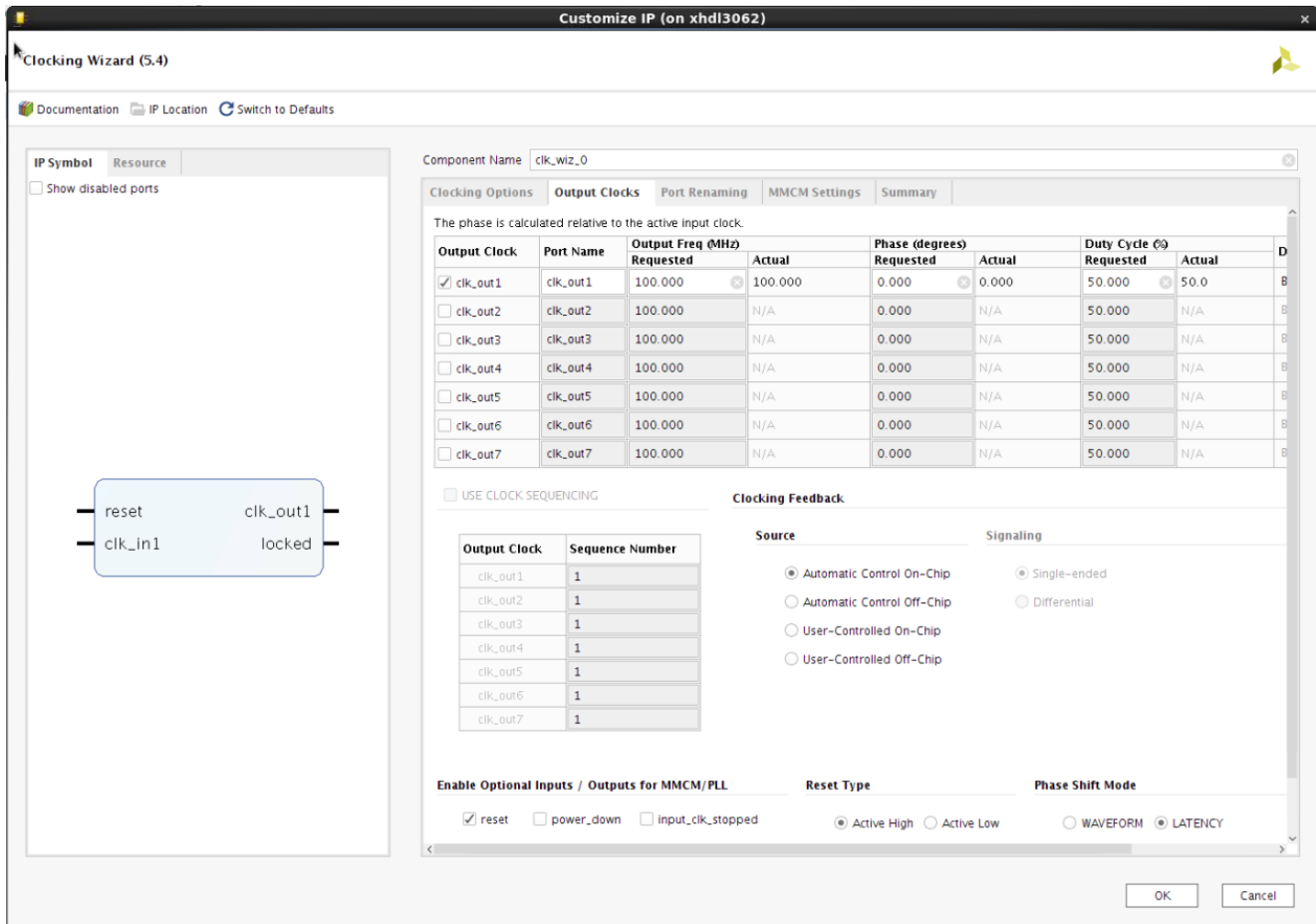
Figure 4-4: Output Clocks for MMCM (Spread Spectrum Unselected)
