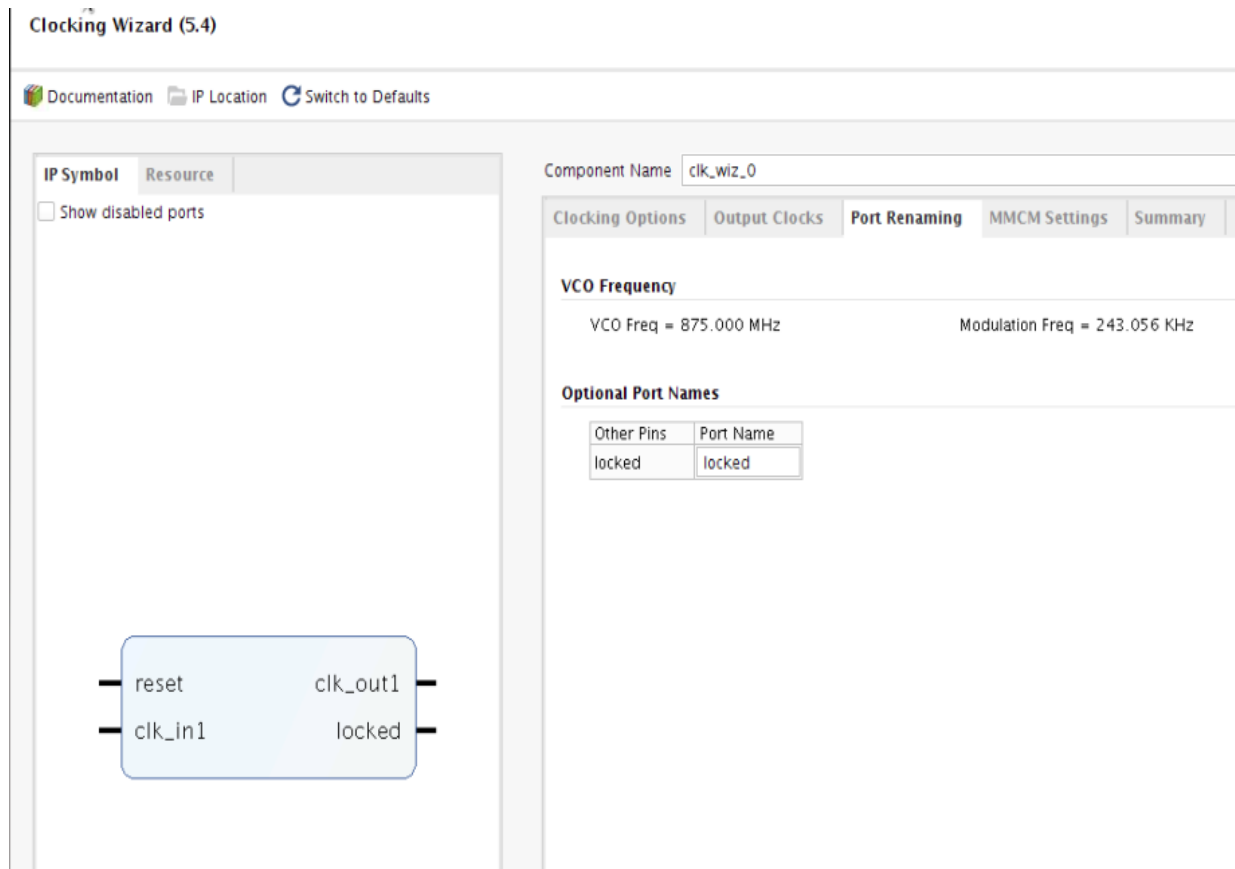
Figure 4-14: Port Renaming (Spread Spectrum Selected)
