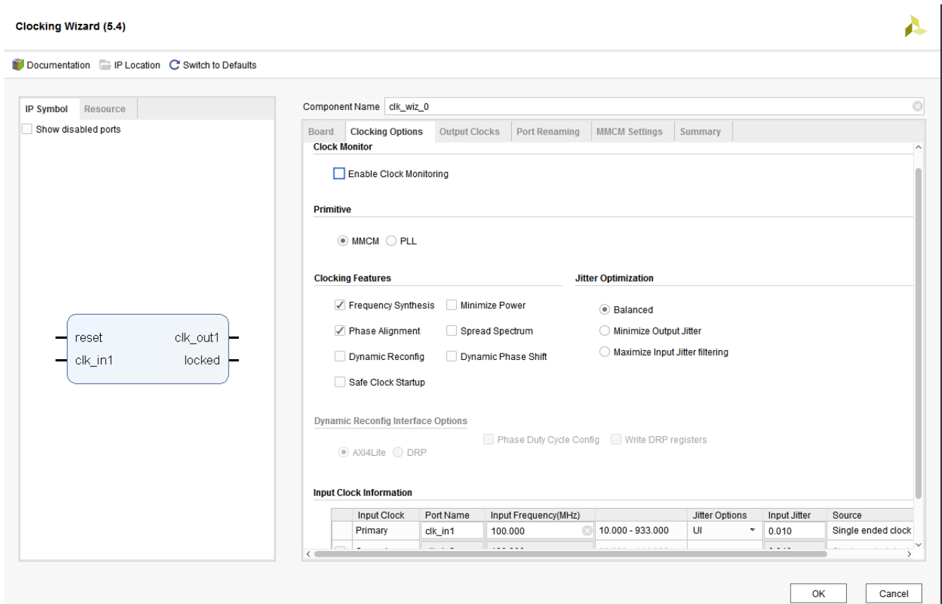
Figure 4-1: Clocking Options for 7 Series MMCM (Spread Spectrum Unselected)
