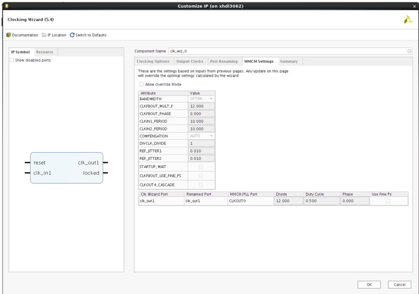
Figure 4-11: Primitive Override Screen (Spread Spectrum Unselected)
