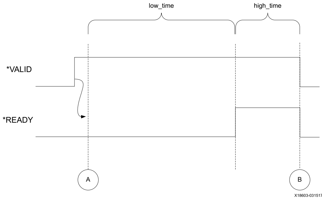
Figure C-9: GEN_AFTER_VALID_SINGLE/RAND_AFTER_VALID_SINGLE
