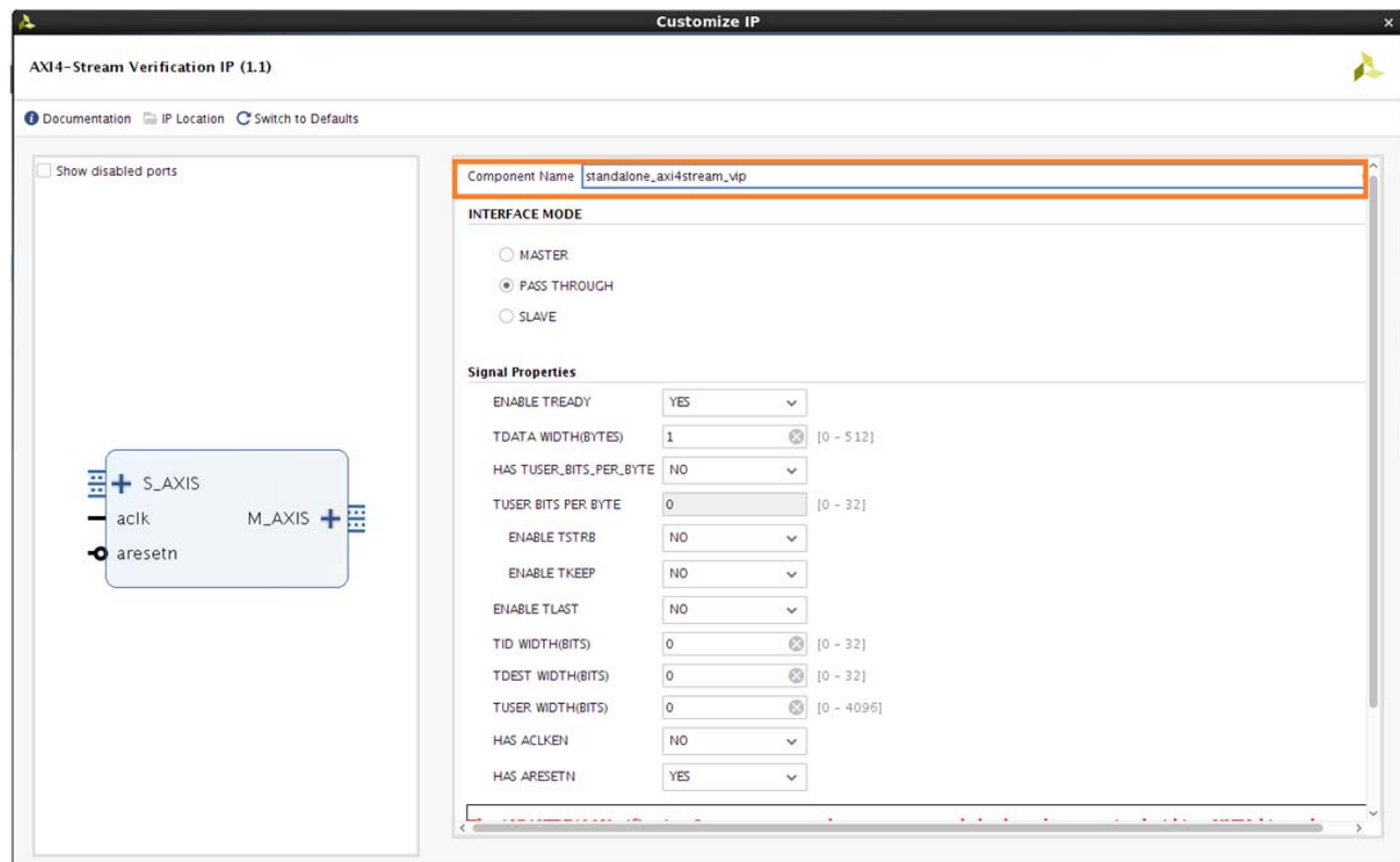
Figure 6-1: Standalone <component_name>_pkg
