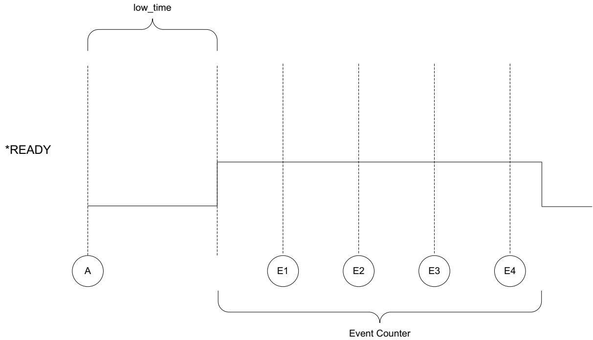
Figure C-8: GEN_EVENTS/RAND_EVENTS
