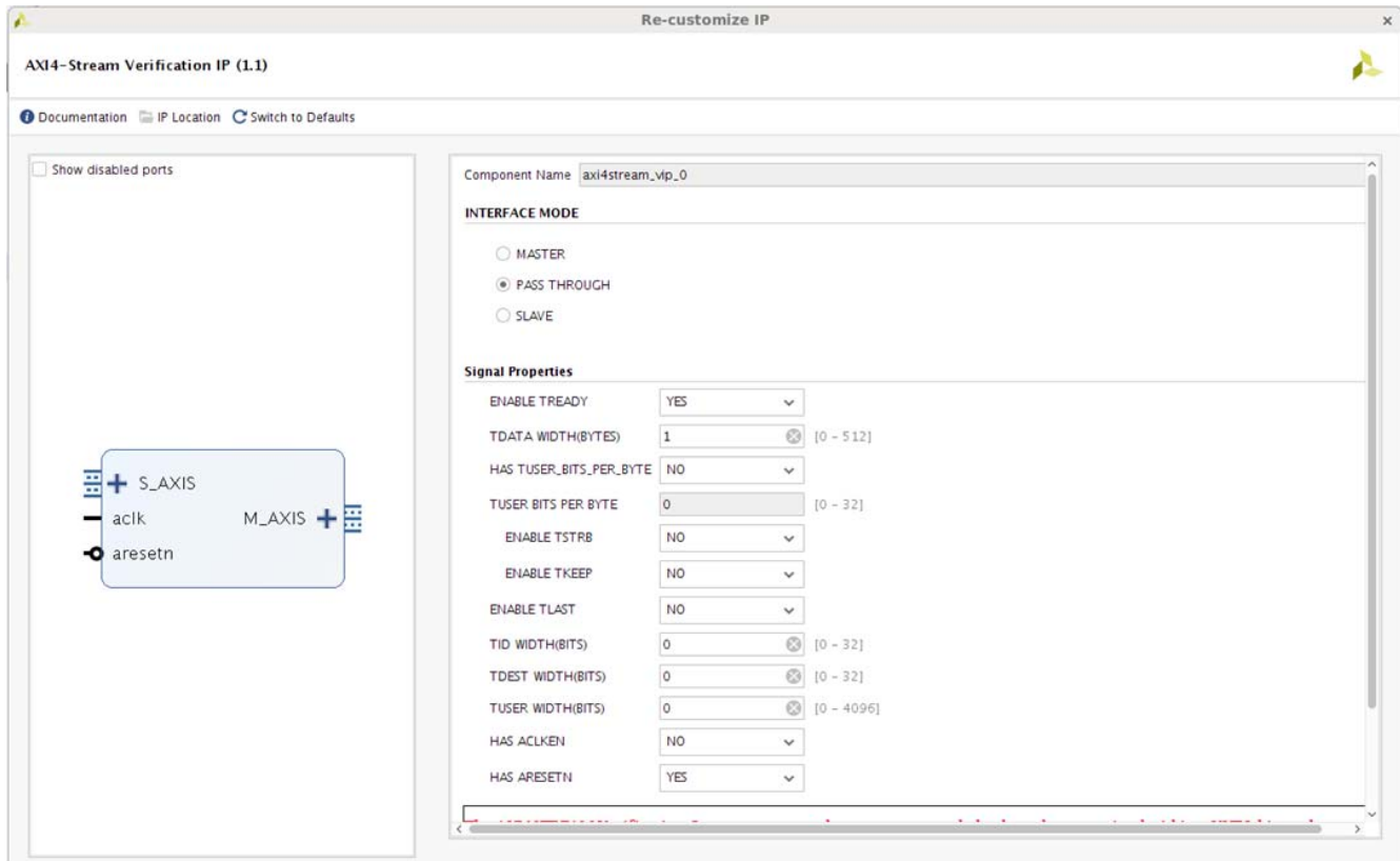
Figure 4-1: AXI4-Stream VIP Customize IP – Component Name Tab
