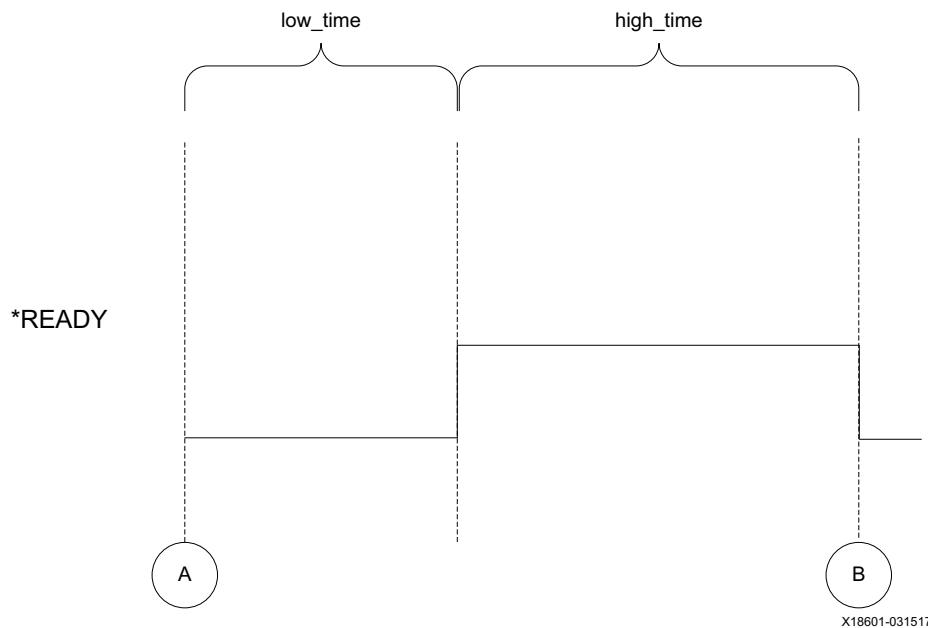
Figure C-7: GEN_OSC/RAND_OSC
