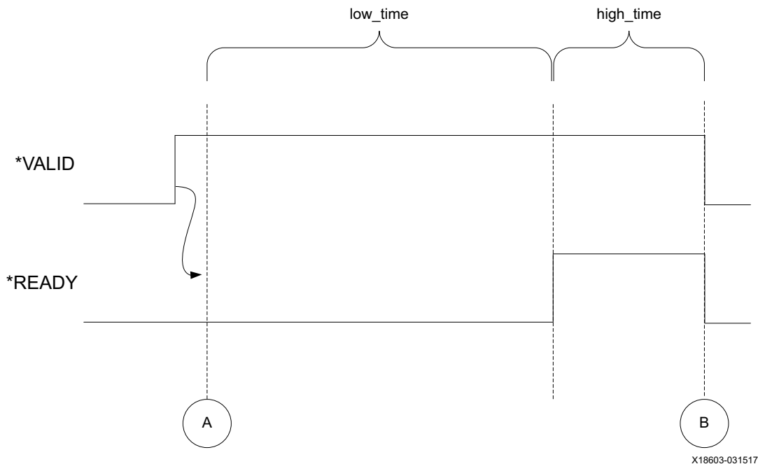
Figure C-6: GEN_SINGLE/RAND_SINGLE
