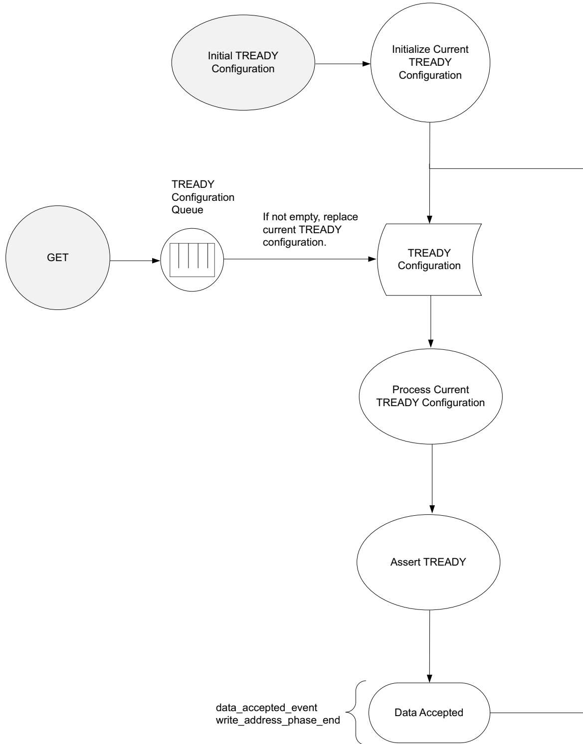
Figure C-4: TREADY Timing Flow
