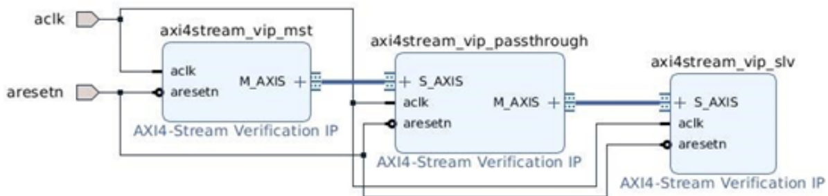
Figure 5-1: AXI4-Stream VIP Example Design
