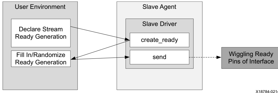
Figure 4-6: Ready Generation Flow
