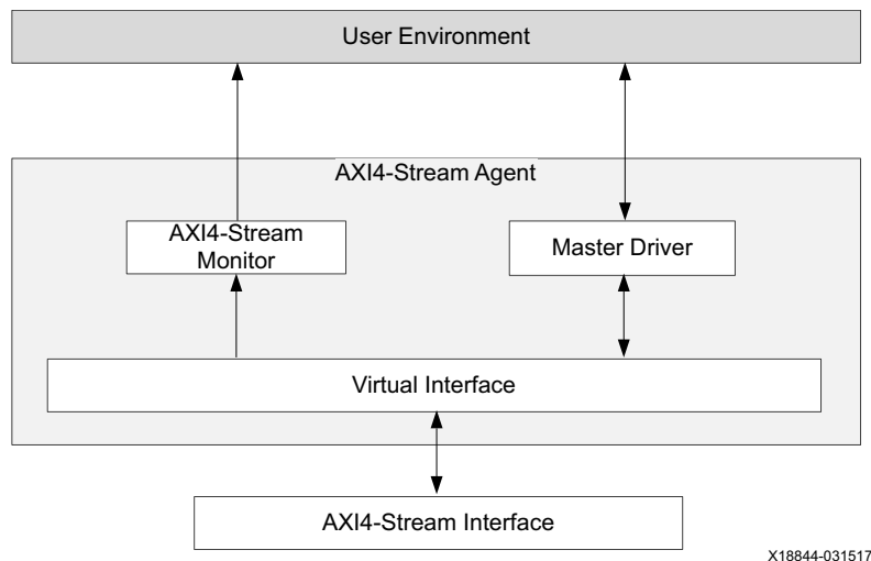
Figure C-1: AXI4-Stream Master VIP Agent
