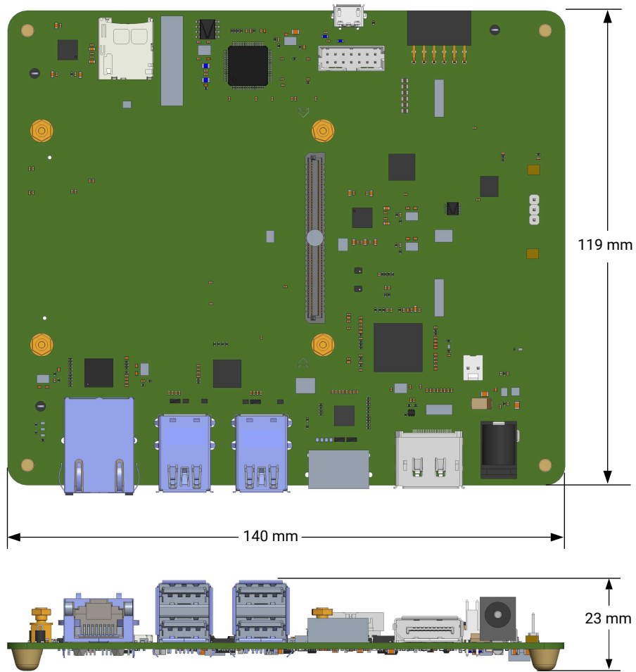
Figure 5: Kria KV260 Vision AI Starter Kit Carrier Card Mechanical Dimensions
