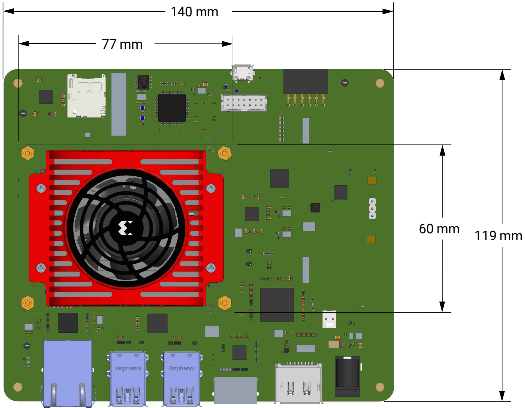
Figure 4: Kria KV260 Vision AI Starter Kit Mechanical Dimensions
