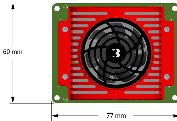
Figure 3: Kria K26 SOM and Thermal Solution Mechanical Dimensions
