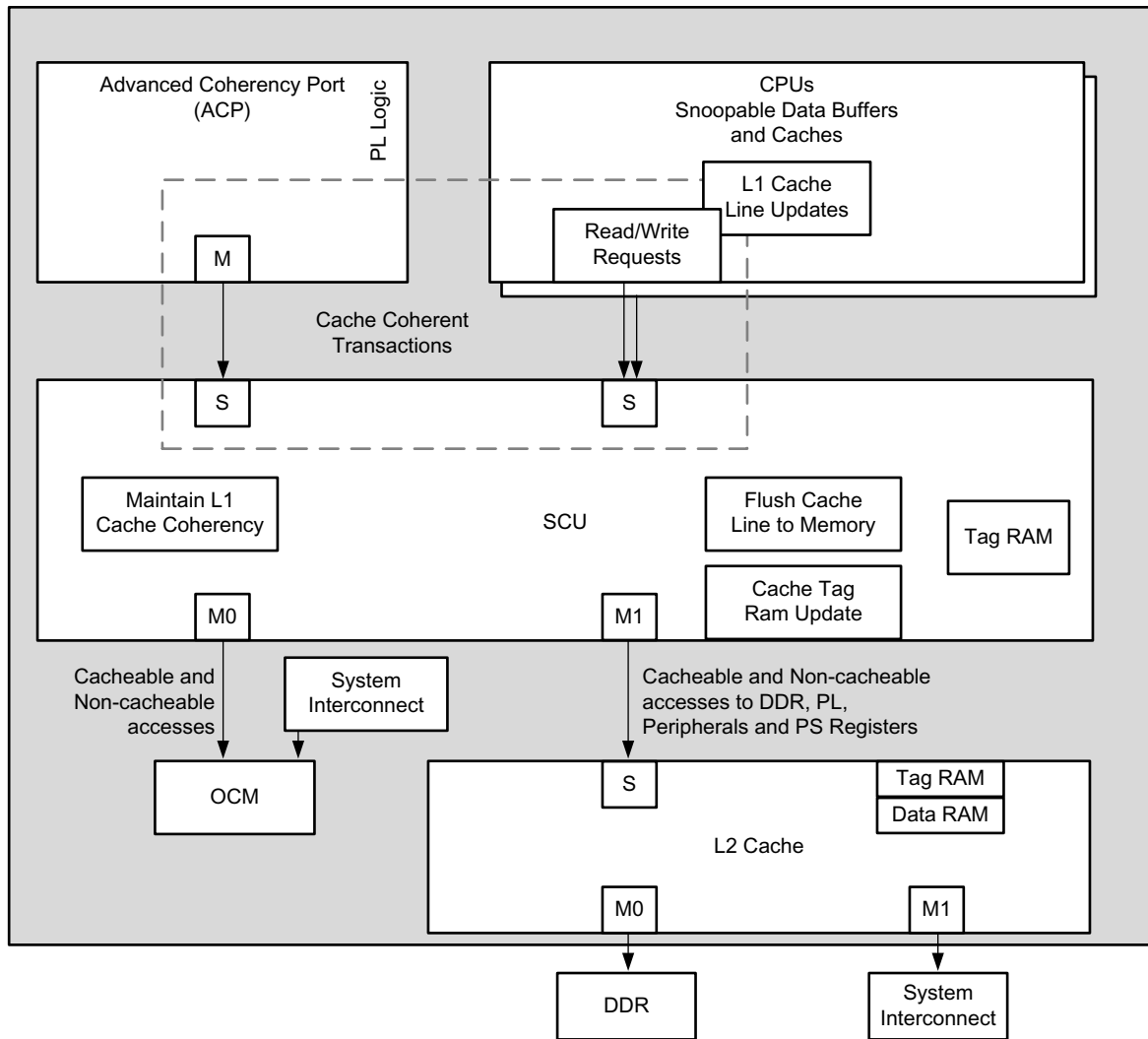
Figure 8: ARM Memories and ACP Connections
