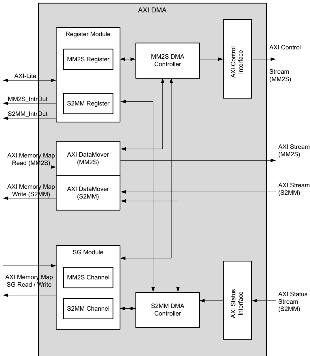
Figure 7: AXI DMA Core Block Diagram
