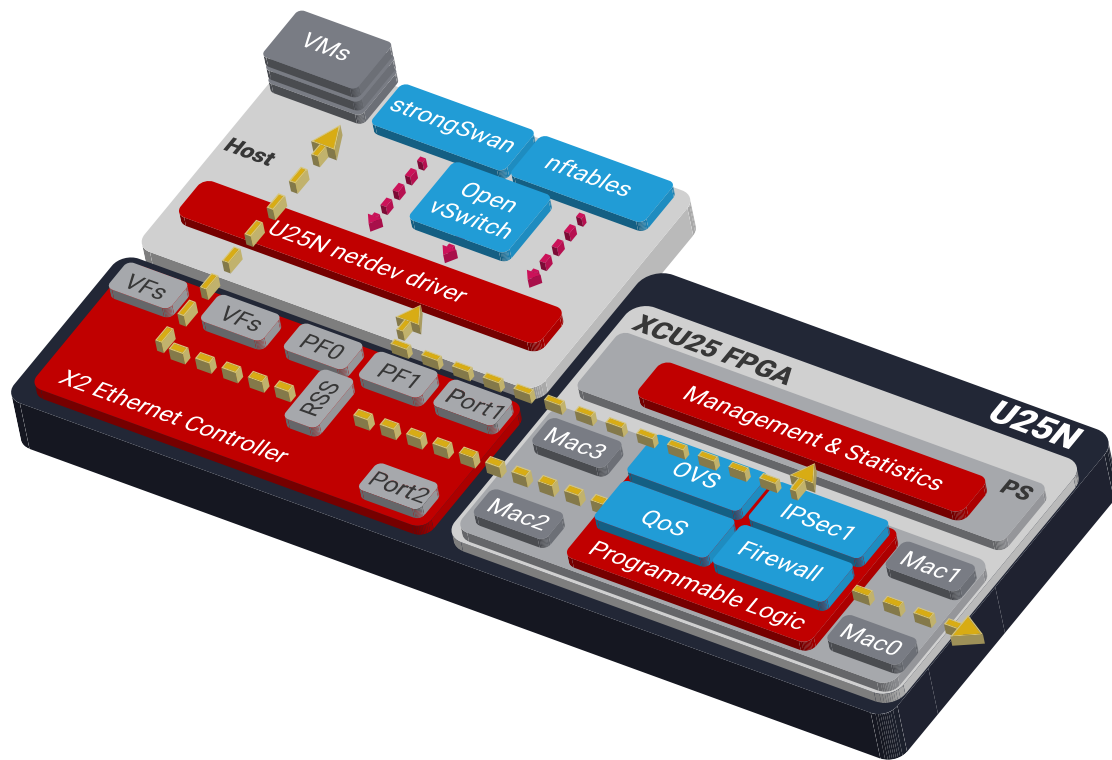
U25N Architectural Block Diagram
