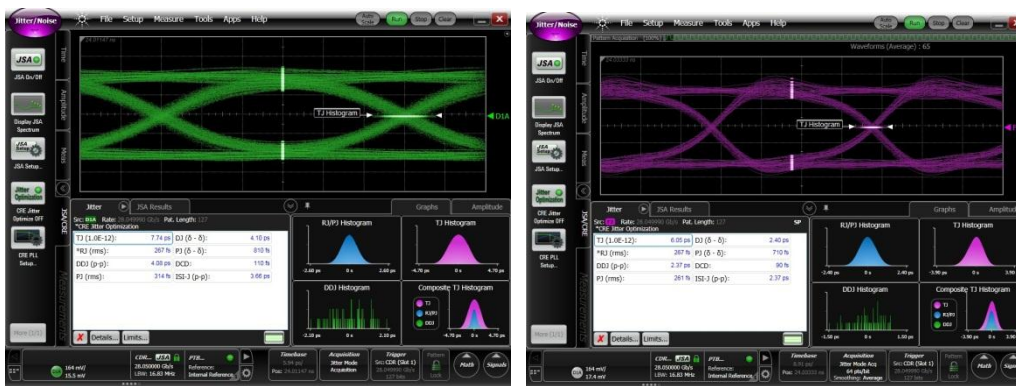
Figure 27: Jitter analysis results on raw signal (left) and de-embedded signal using 1-port AFR model (right).
